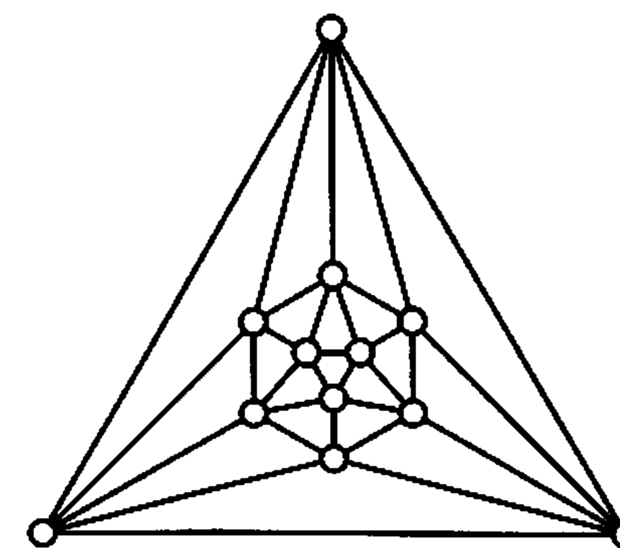
Figure 6.8. The icosahedron
