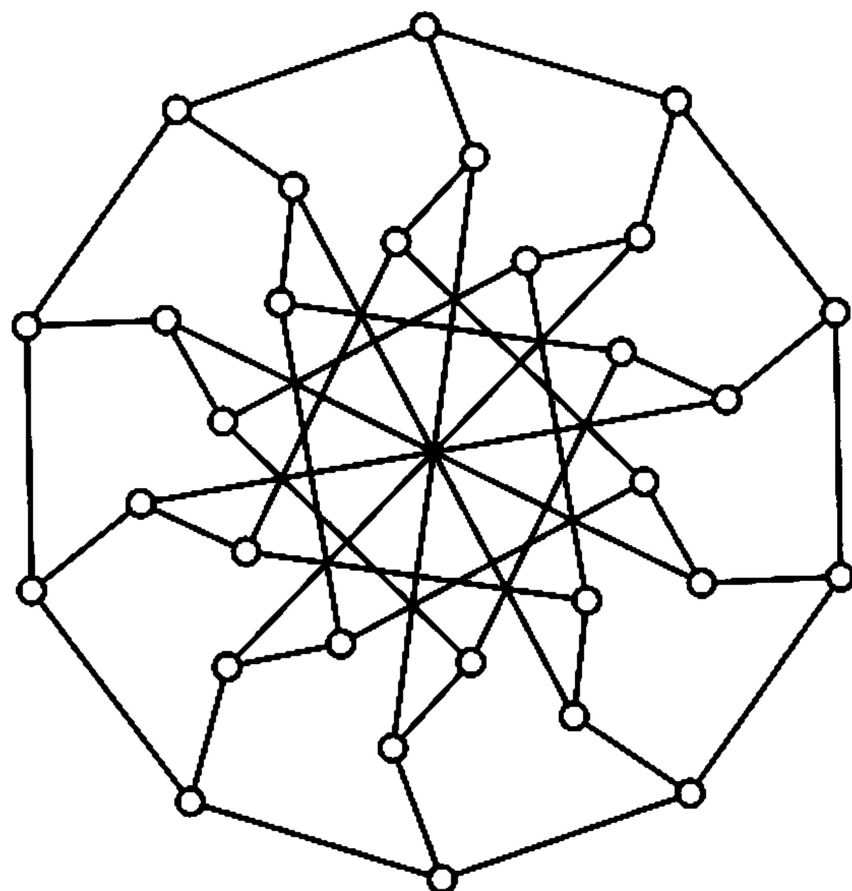
Figure 4.7. Tutte's 8-cage
