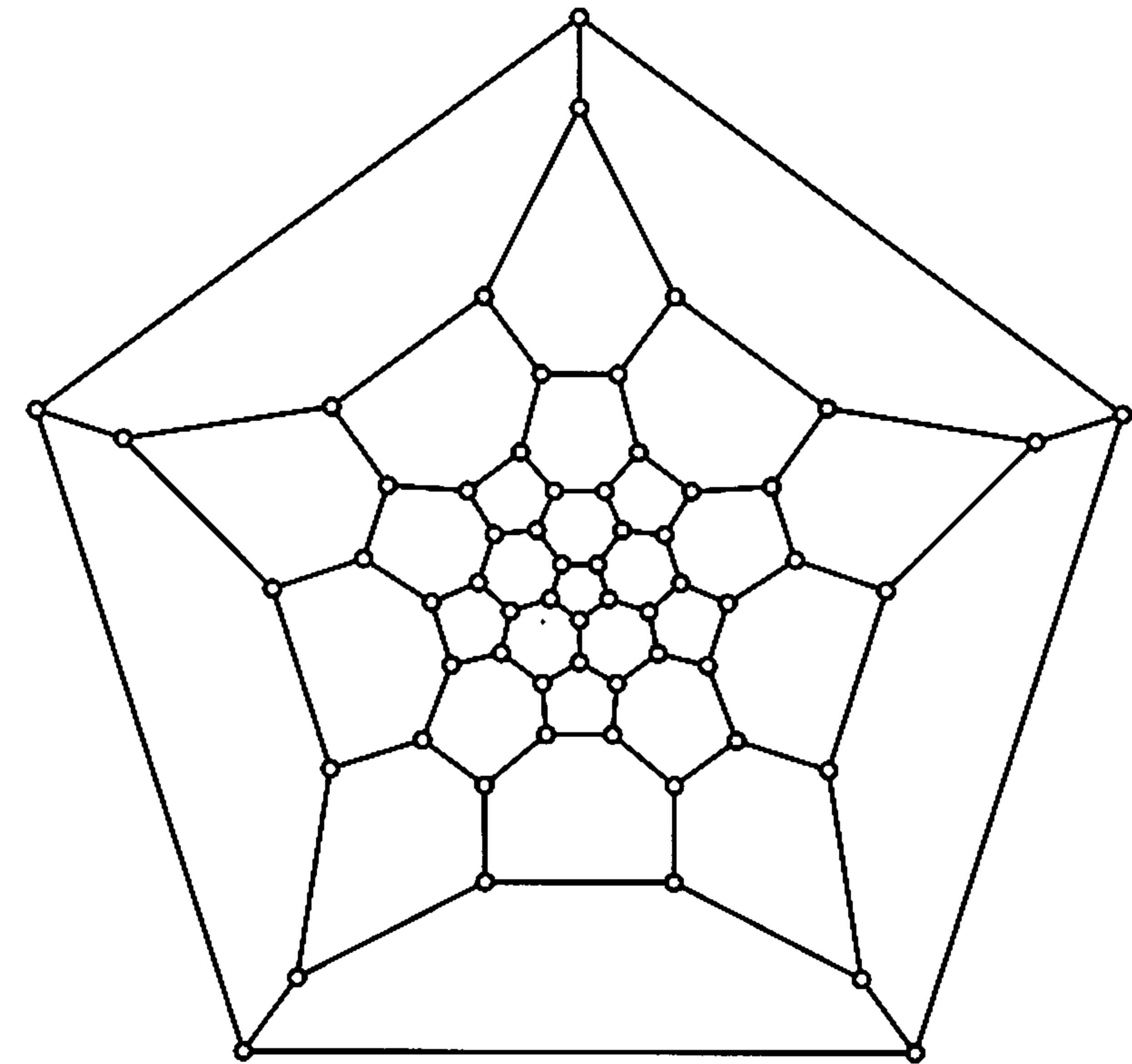
Figure 9.5. Buckminsterfullerene
