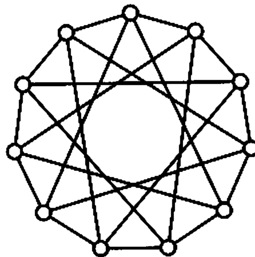
Figure 6.2. \text{And}(4) = X(\mathbb{Z}_{11}, \{1, 4, 7, 10\})
