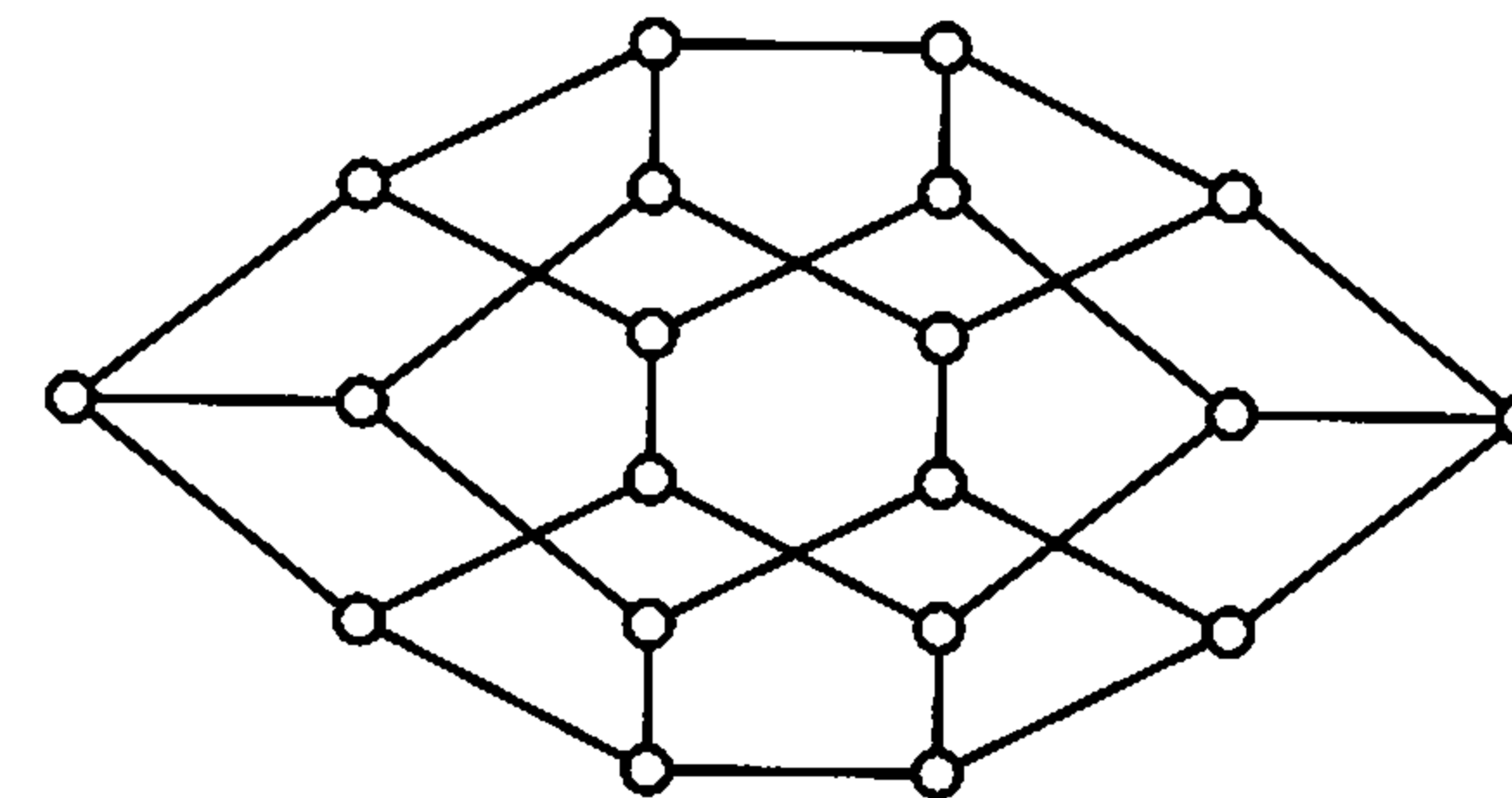
Figure 4.5. The dodecahedron
