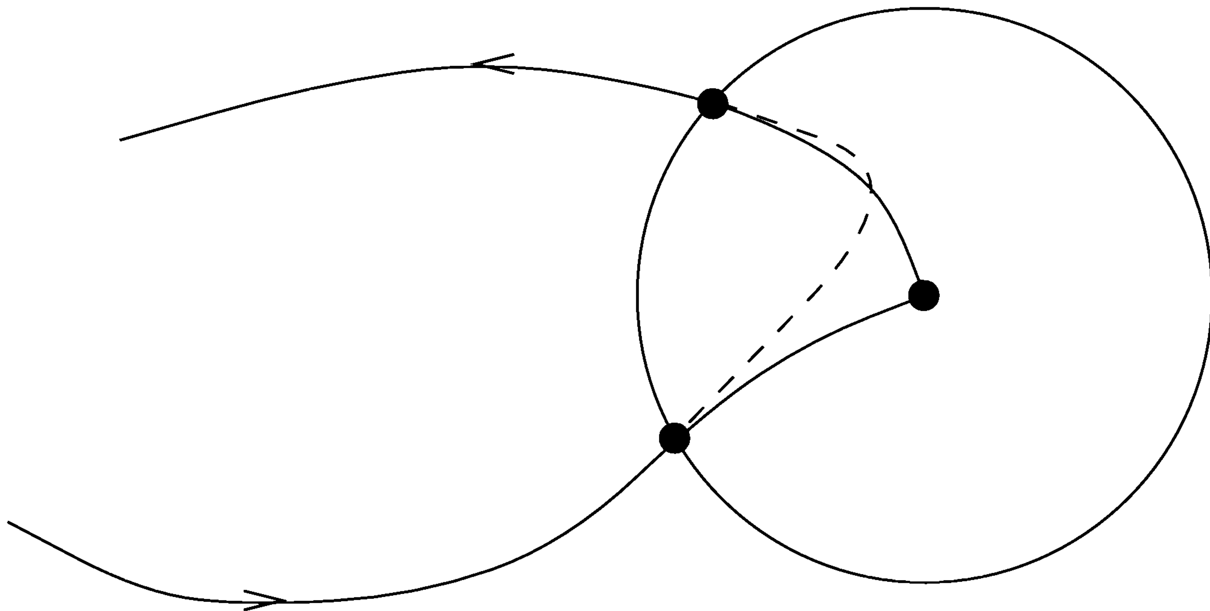
FIGURE 9.11. Rounding a corner.
