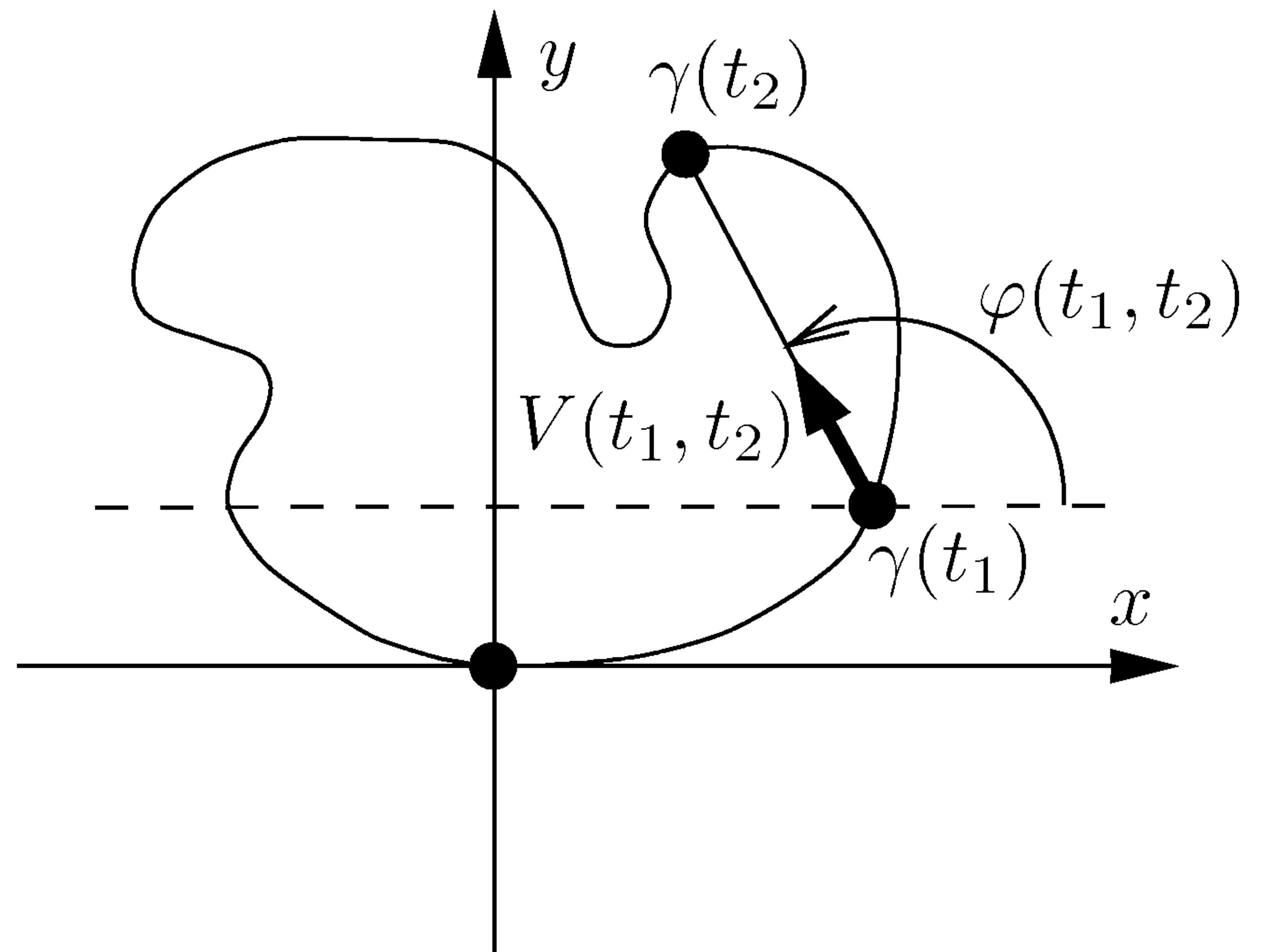
FIGURE 9.9. The secant angle.
