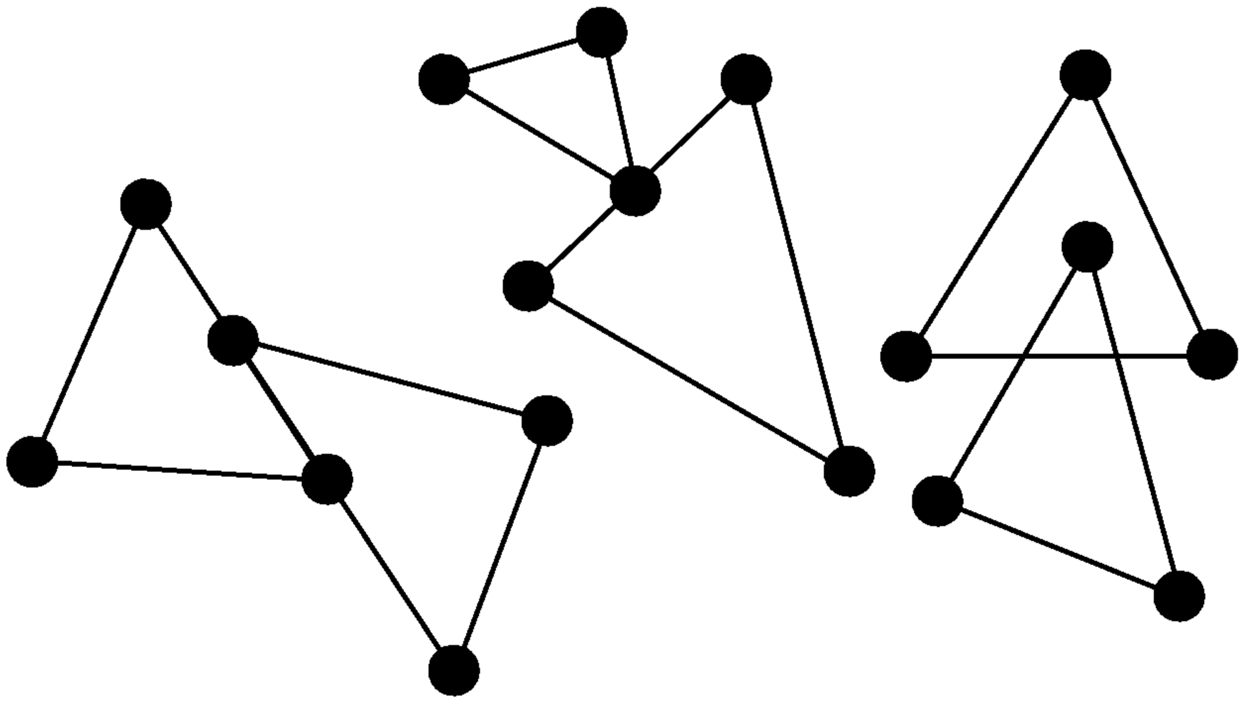
FIGURE 9.14. Illegal intersections of triangles in a triangulation.
