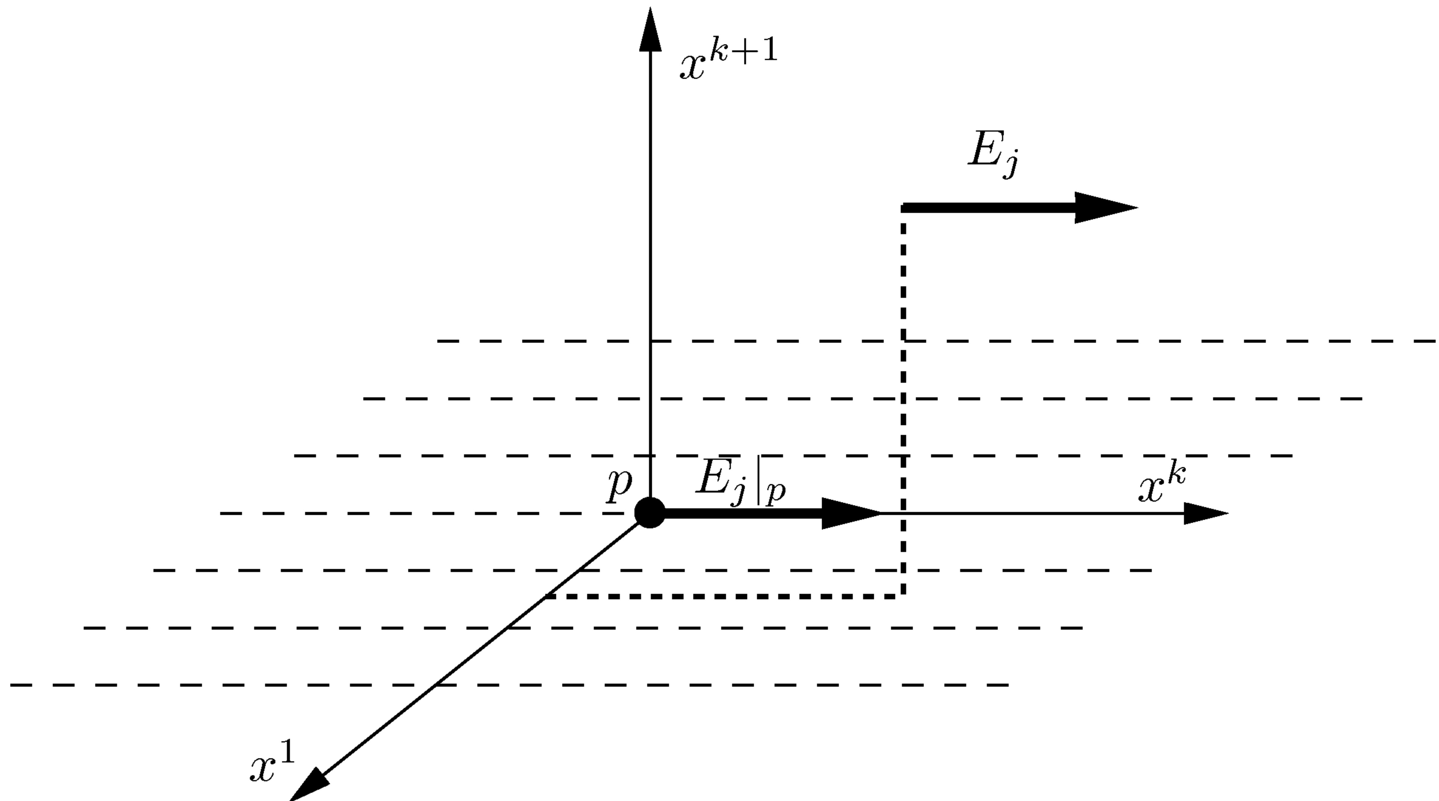
FIGURE 7.2. Proof that zero curvature implies flatness.
