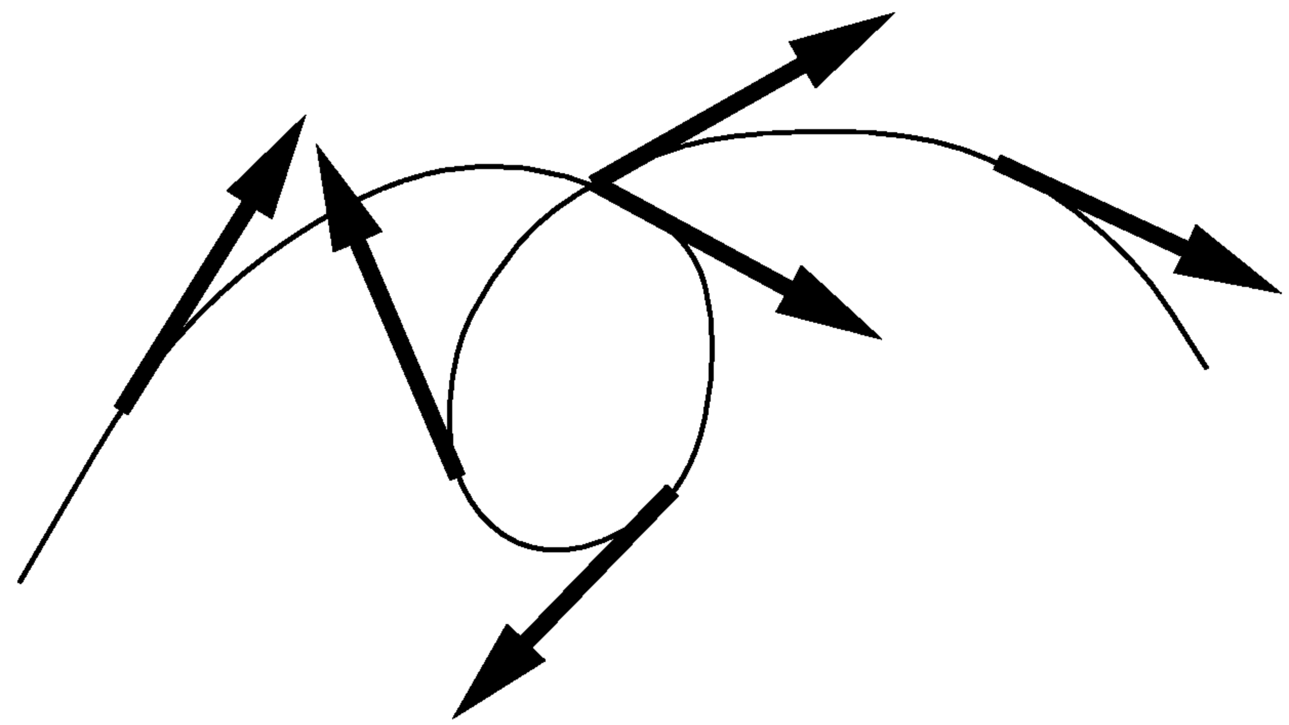
FIGURE 4.5. Nonextendible vector field.
