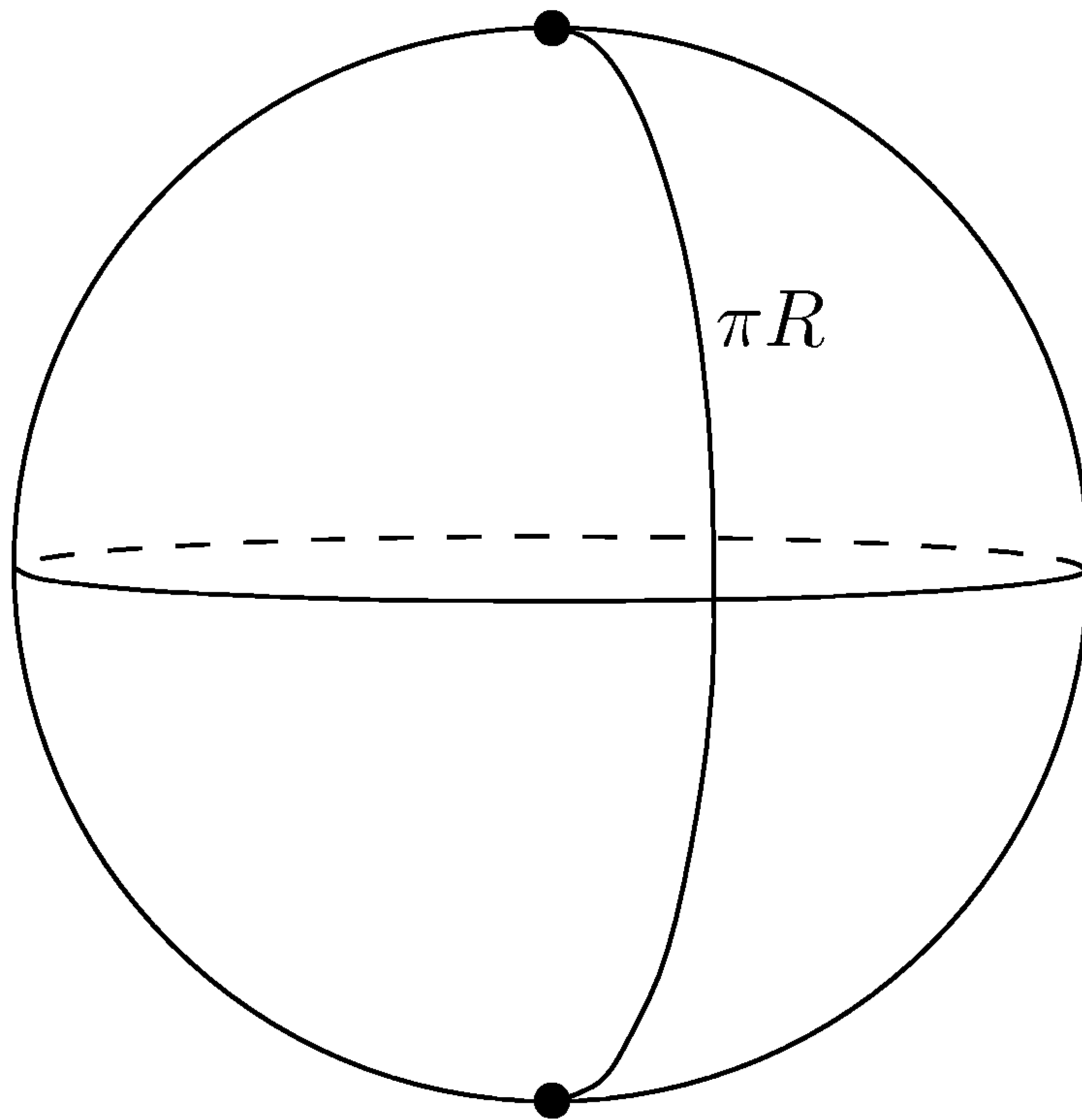
FIGURE 11.4. The diameter of S_R^n is \pi R .
