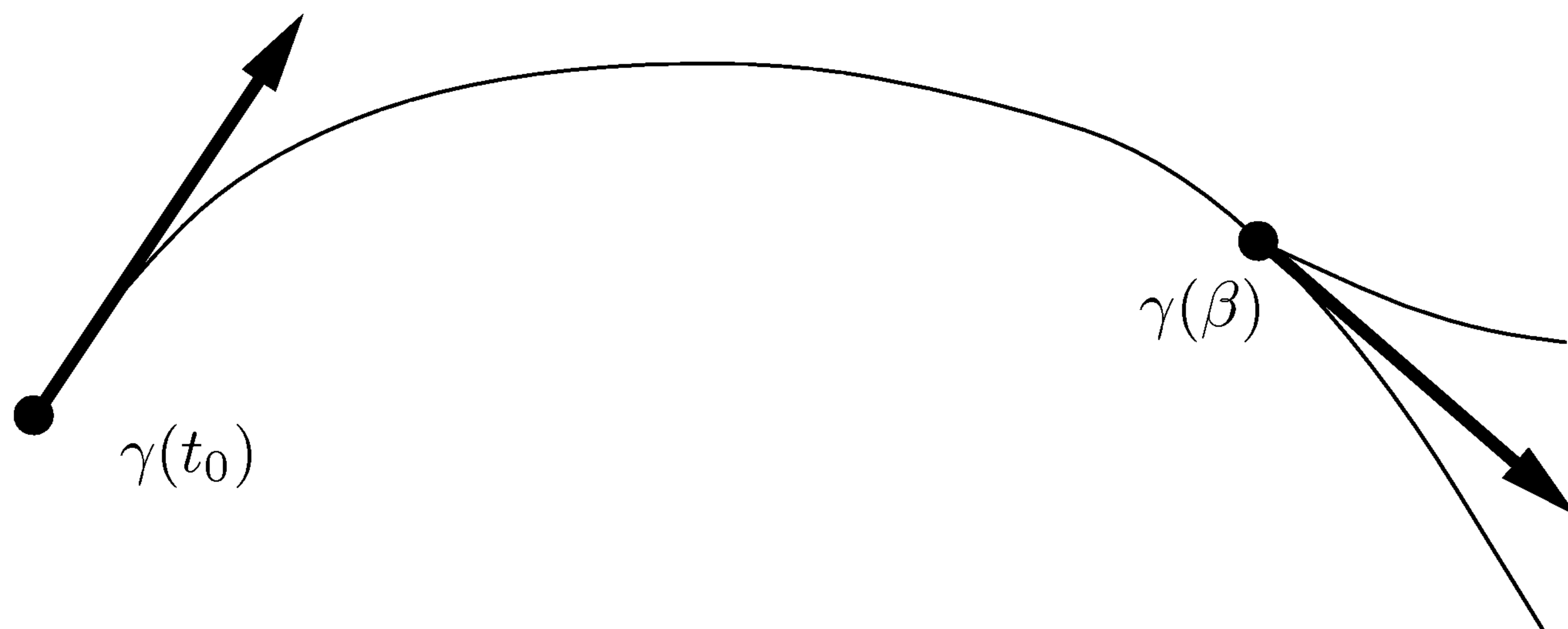
FIGURE 4.6. Uniqueness of geodesics.
