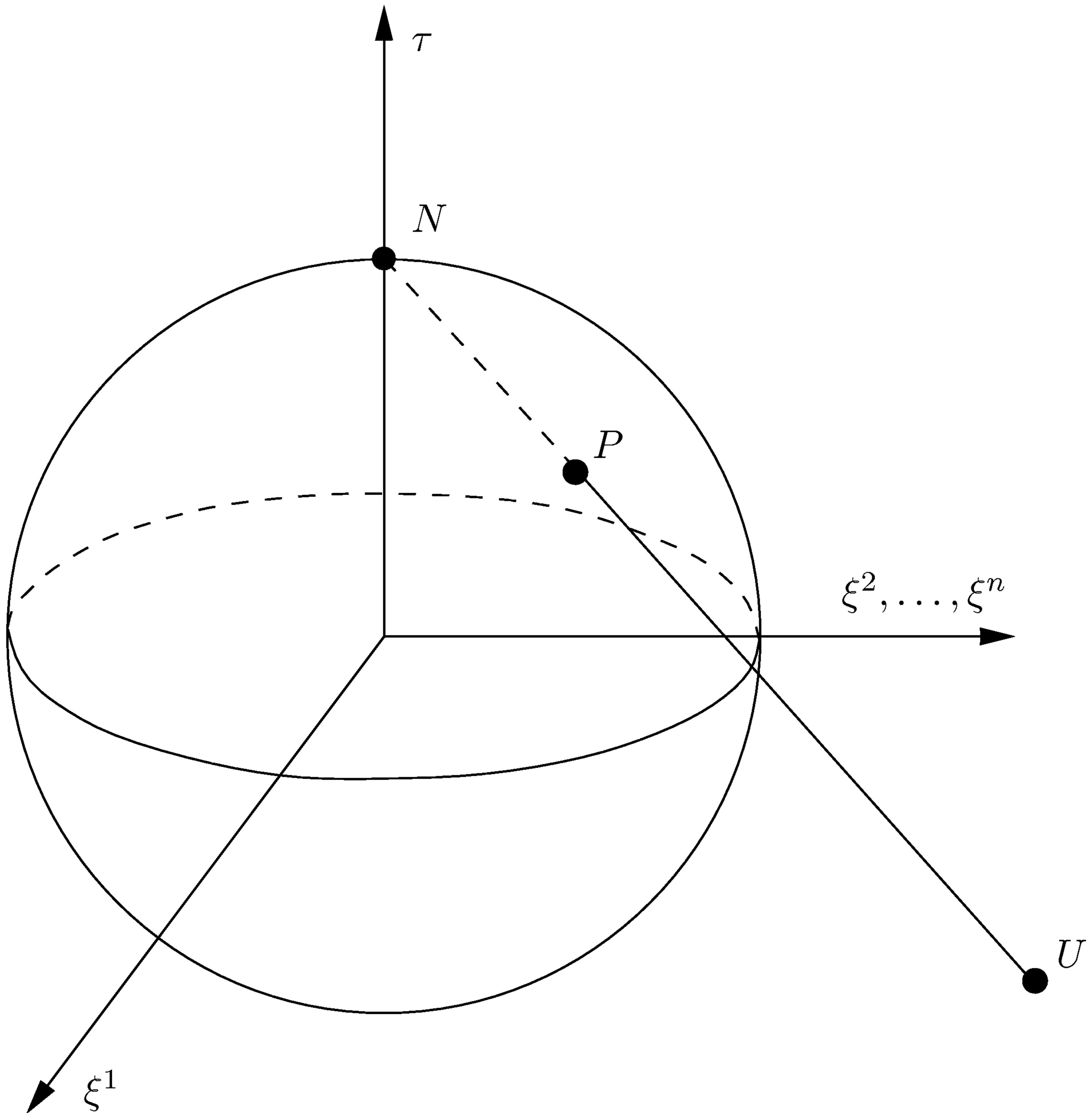
FIGURE 3.3. Stereographic projection.
