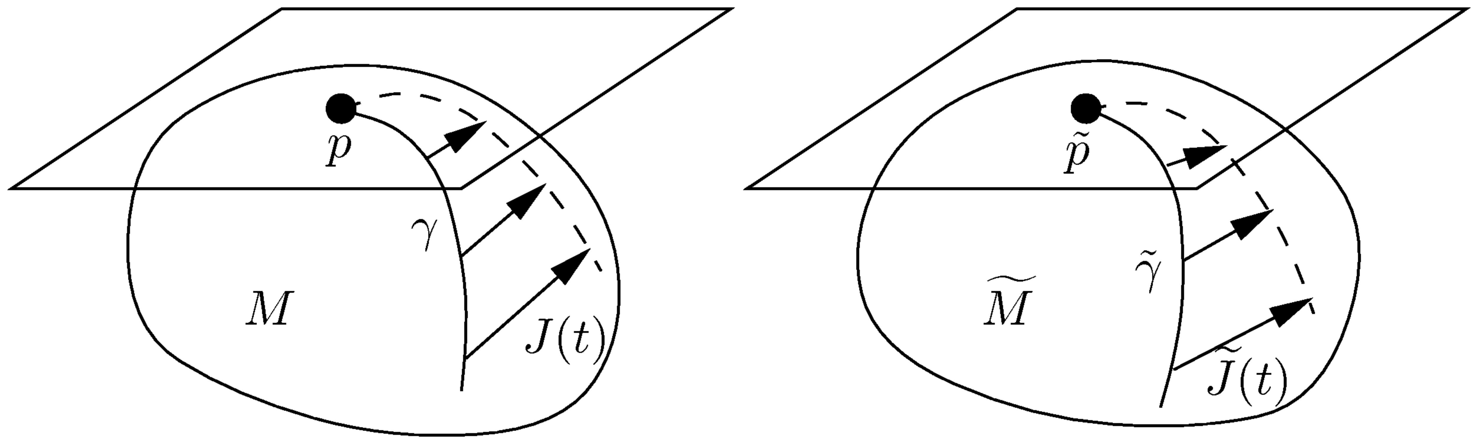
FIGURE 11.5. Setup for the Rauch comparison theorem.
