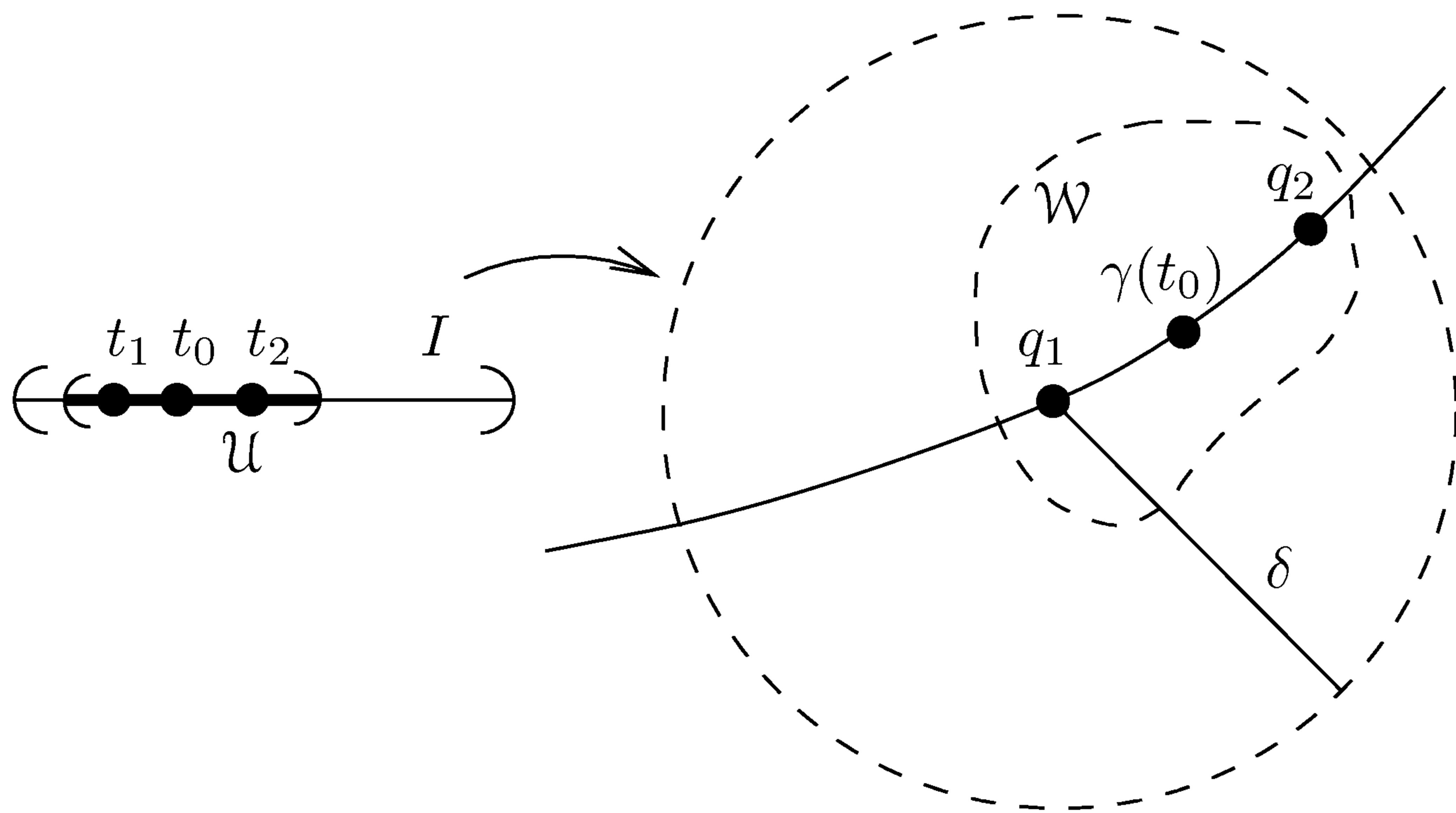
FIGURE 6.13. Geodesics are locally minimizing.
