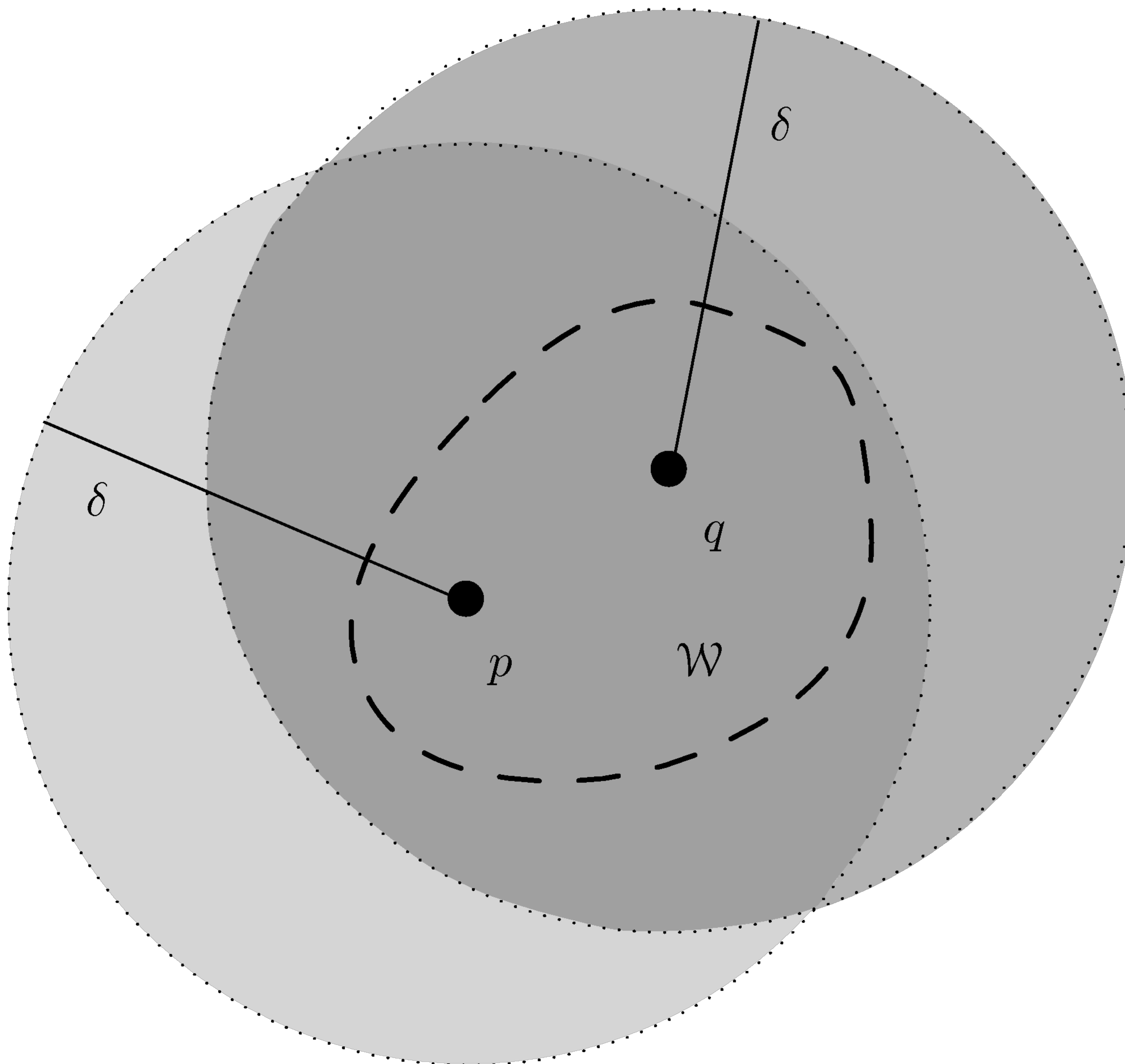
FIGURE 5.4. Uniformly normal neighborhood.
