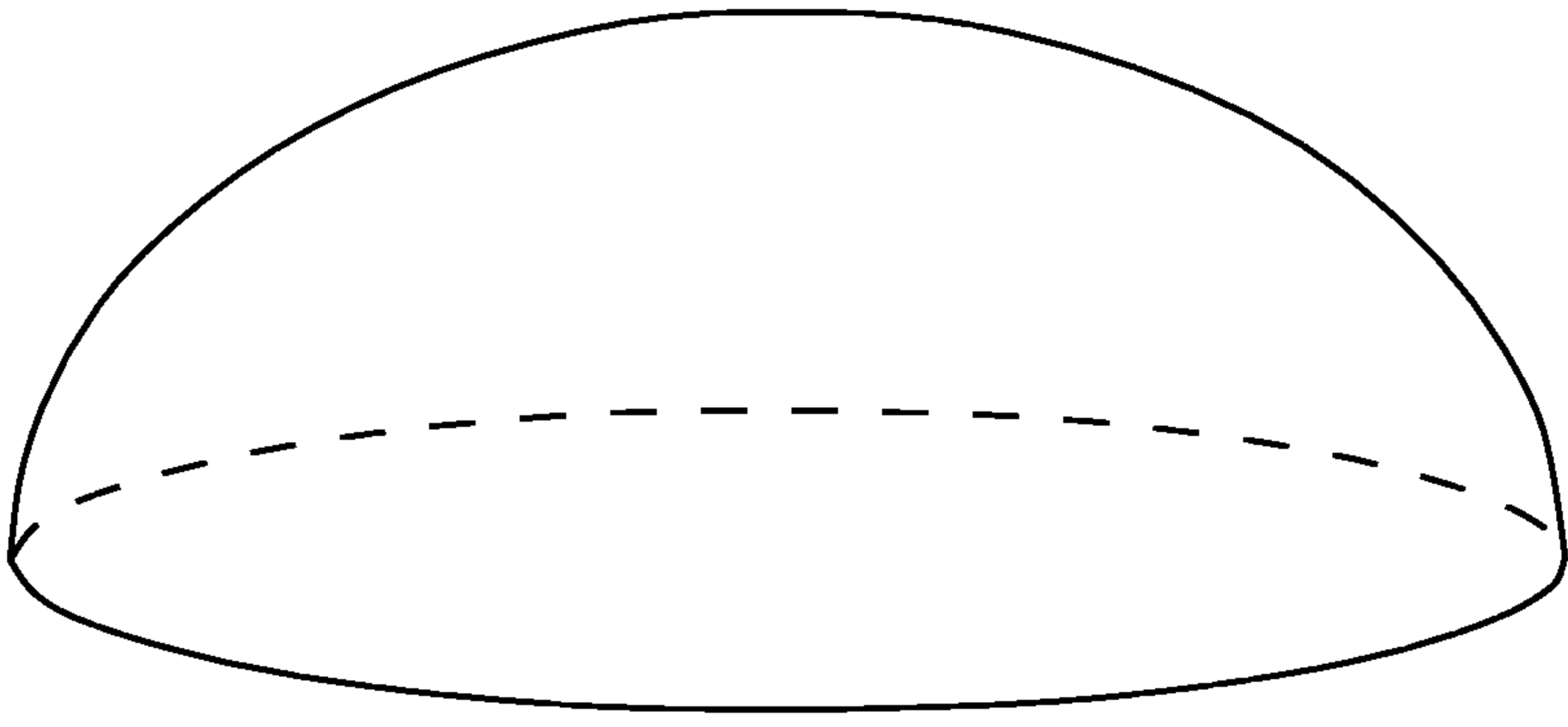
FIGURE 1.5. K > 0 .
