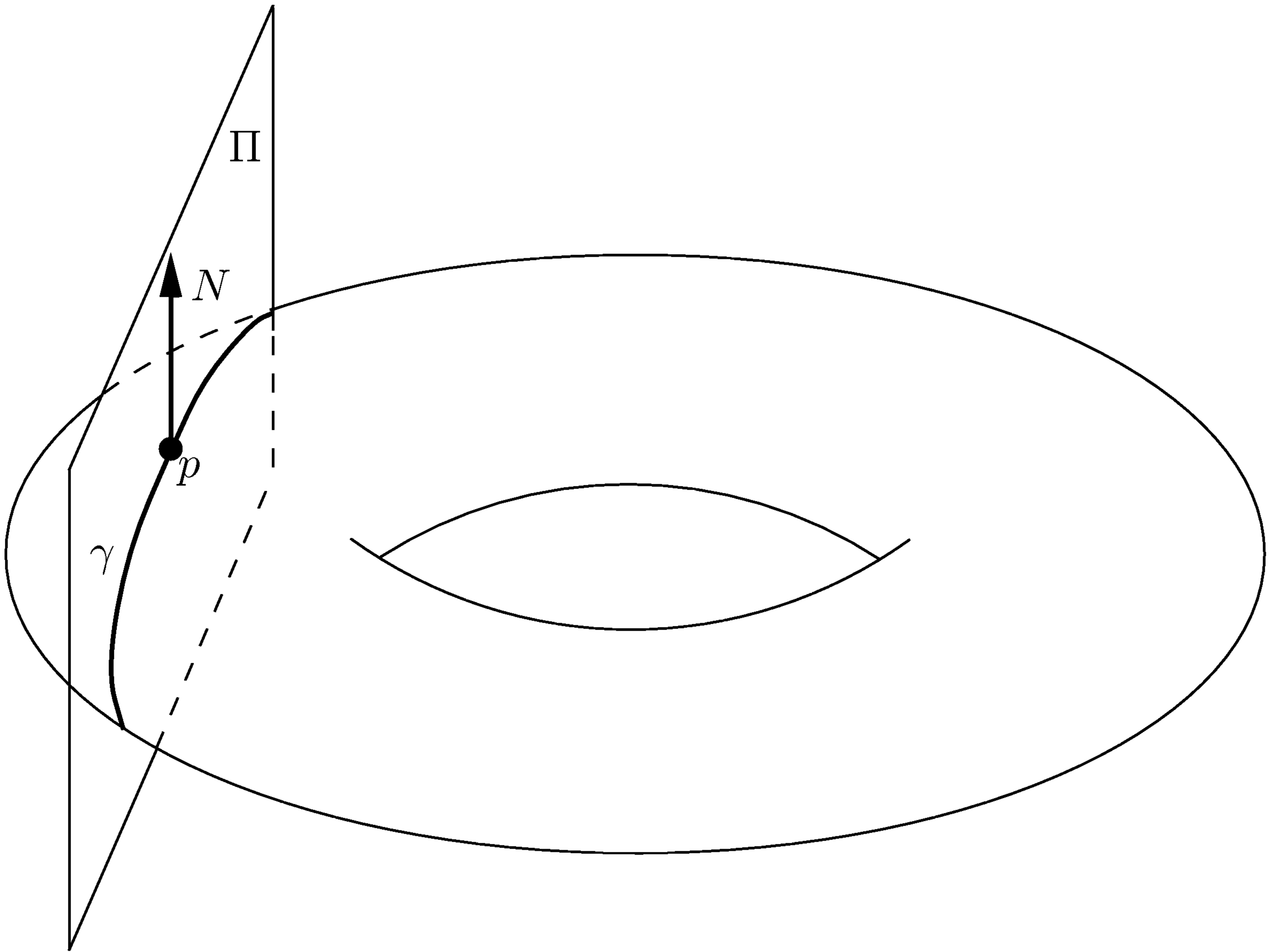
FIGURE 1.2. Computing principal curvatures.
