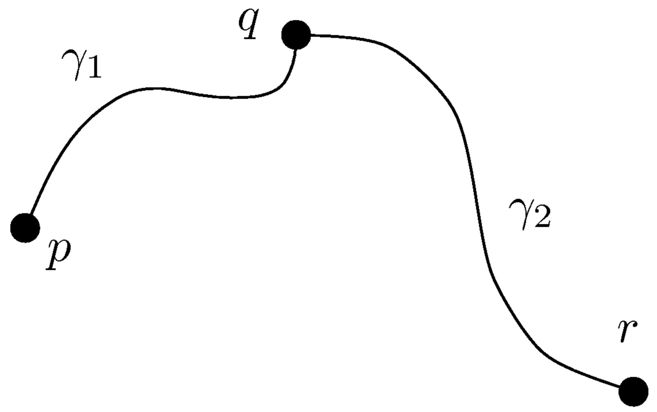
FIGURE 6.2. The triangle inequality.
