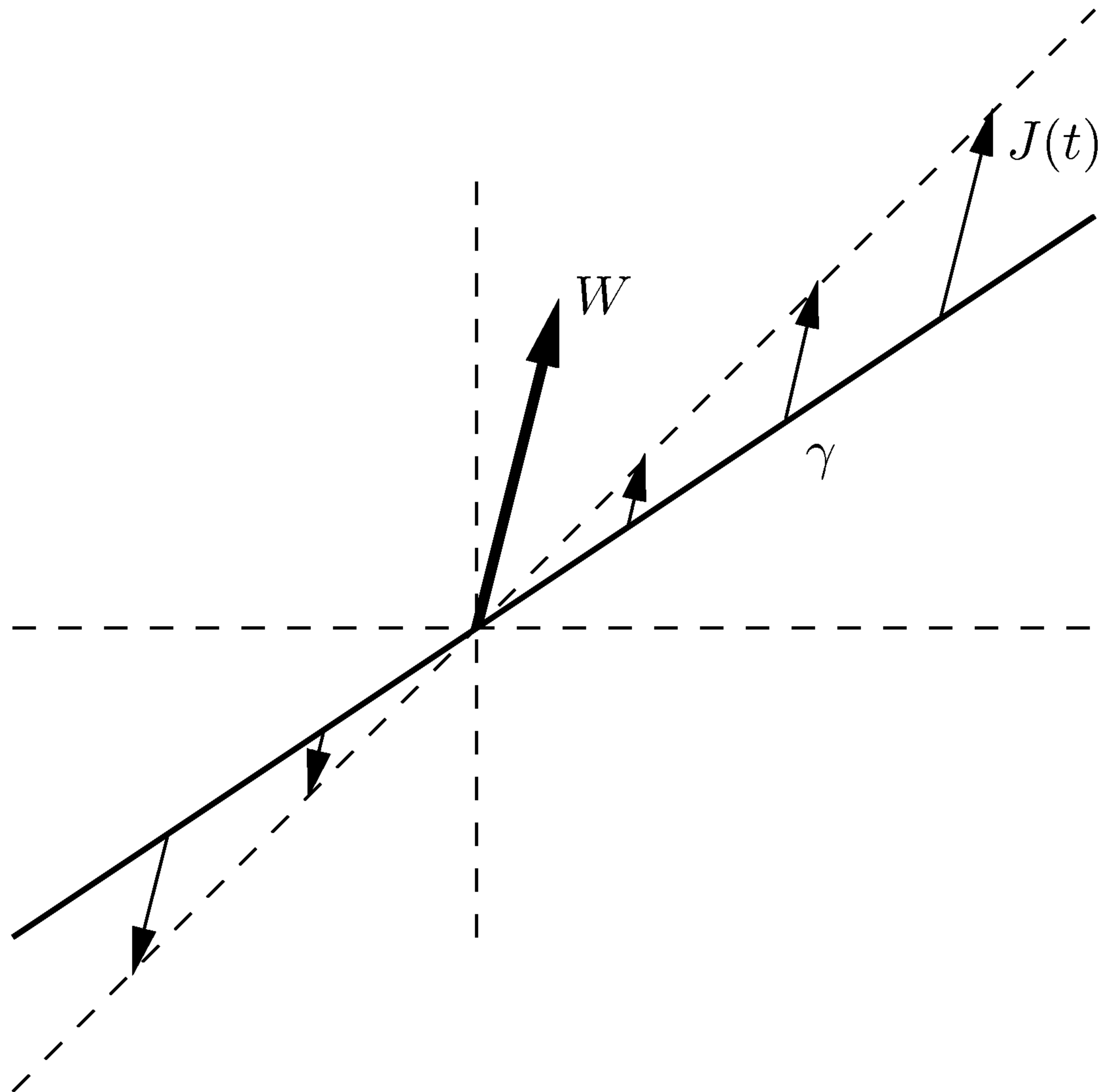
FIGURE 10.4. A Jacobi field in normal coordinates.
