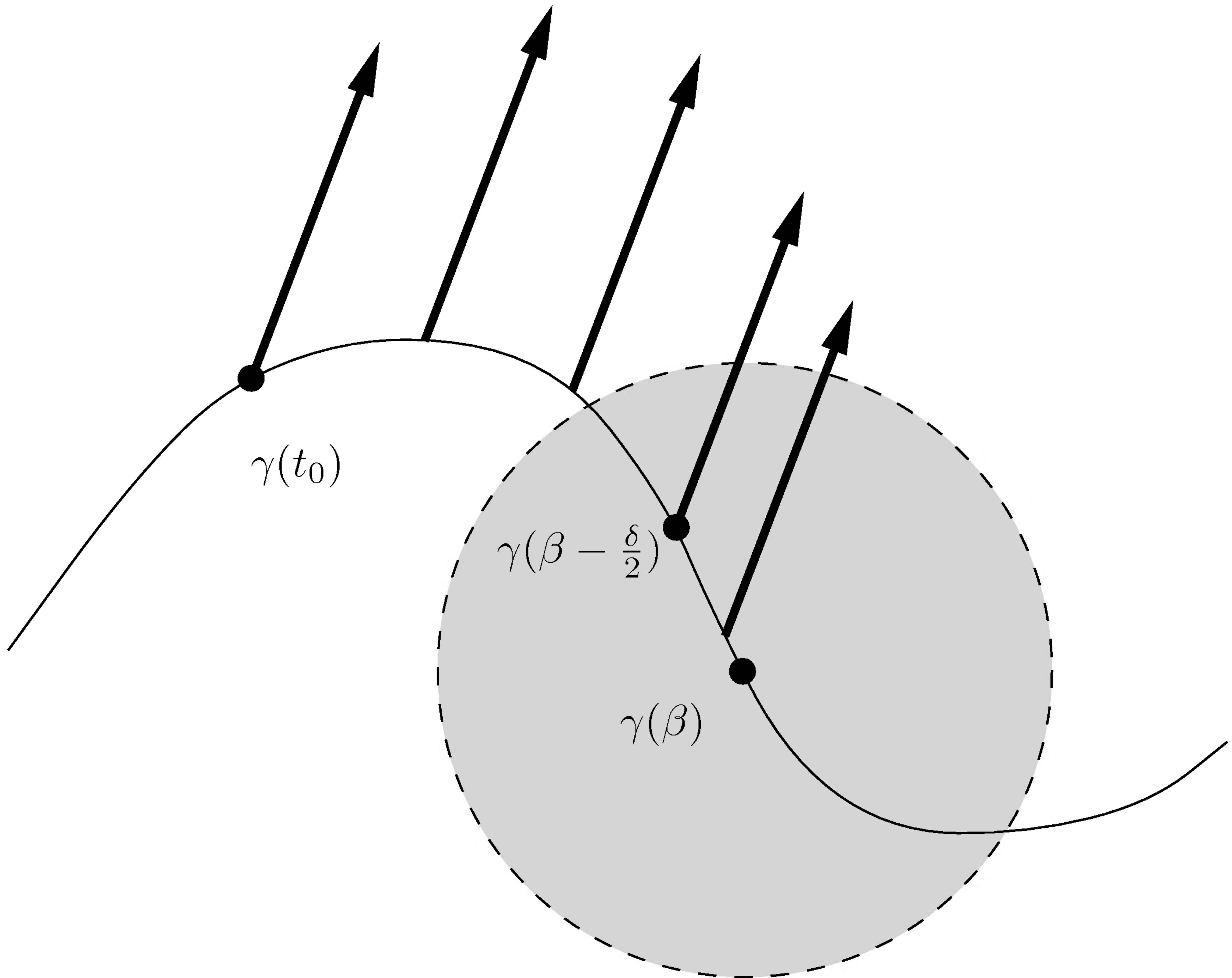
FIGURE 4.8. Existence and uniqueness of parallel translates.
