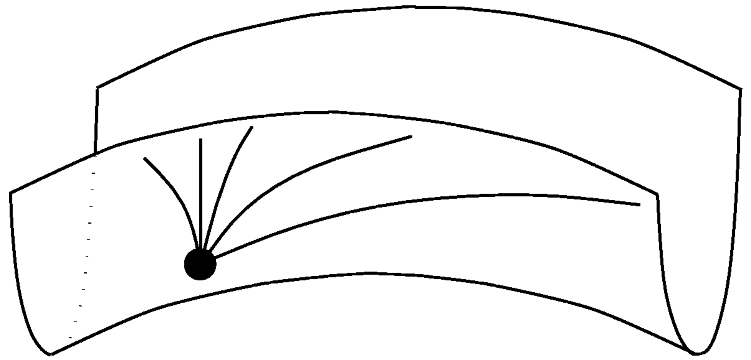
FIGURE 10.2. Negative curvature causes geodesics to spread out.
