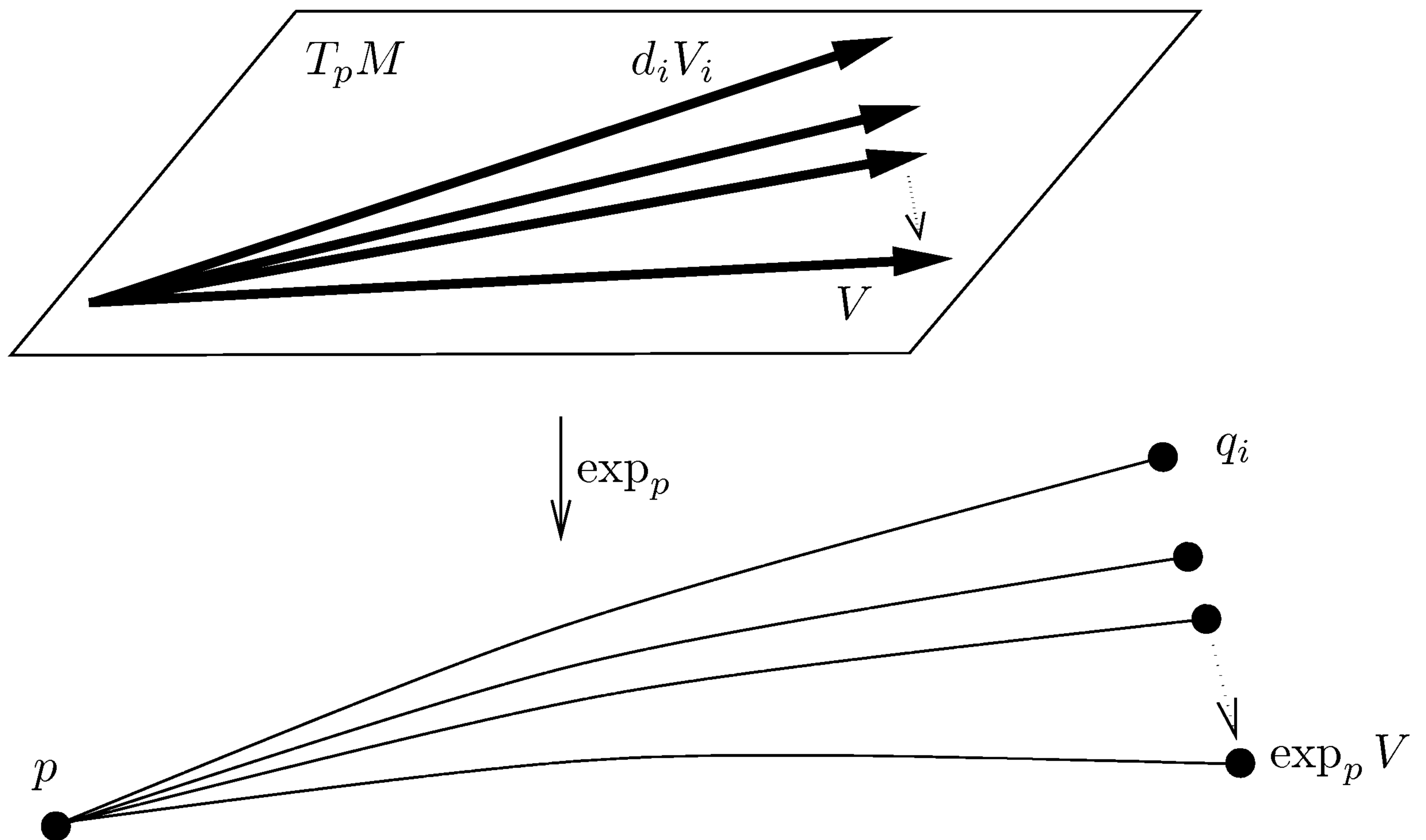
FIGURE 6.17. Cauchy sequences converge.
