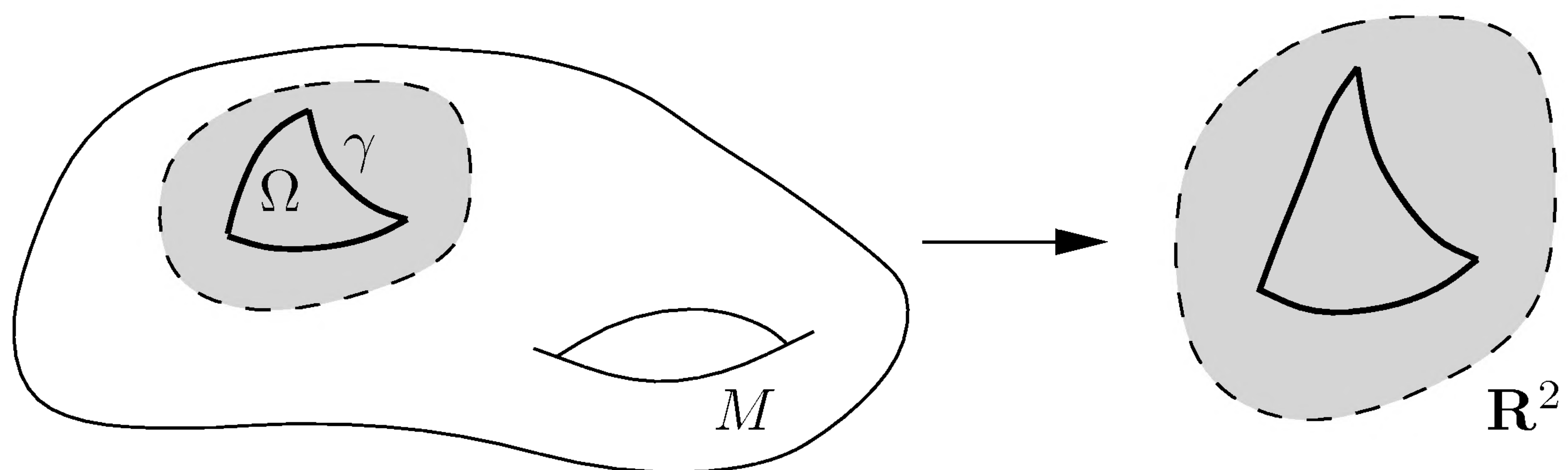
FIGURE 9.12. A curved polygon on a surface.
