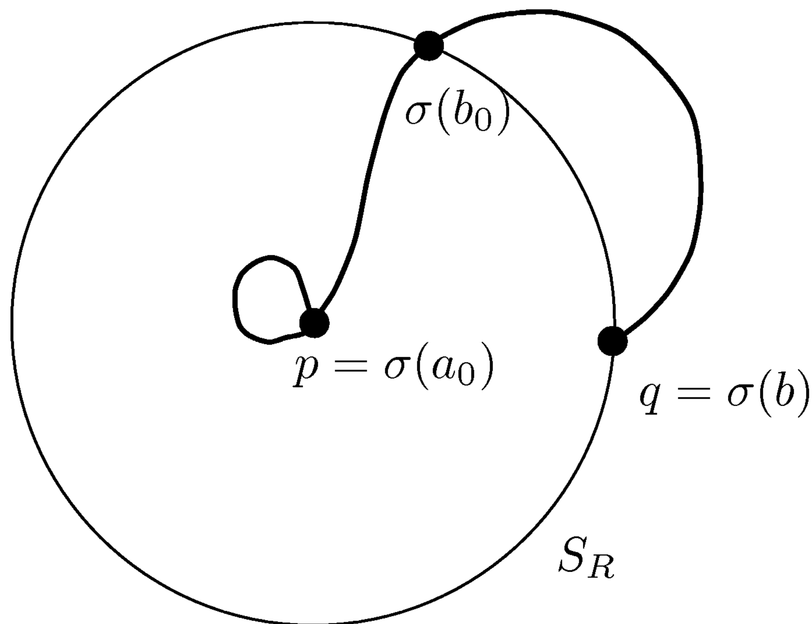
FIGURE 6.12. Radial geodesics are minimizing.
