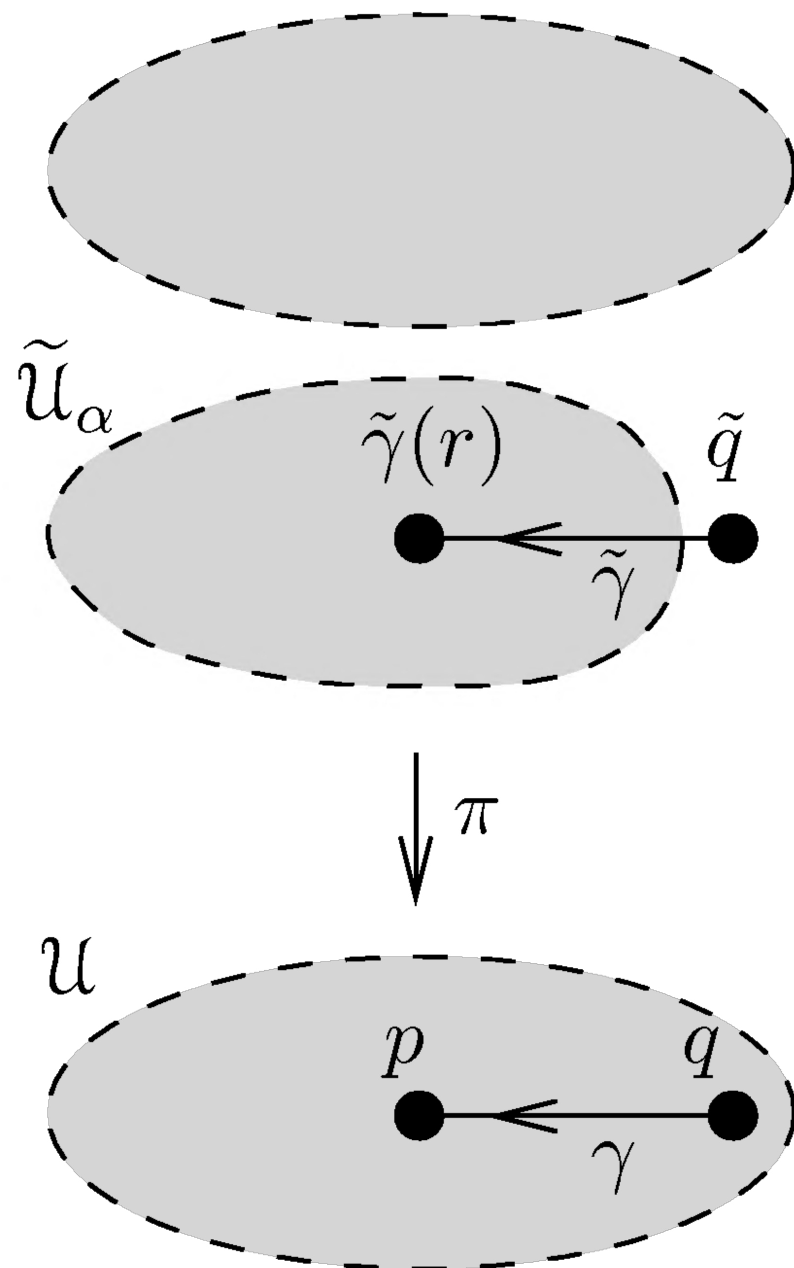
FIGURE 11.3. Proof that \pi^{-1}(\mathcal{U}) \subset \bigcup_{\alpha} \tilde{\mathcal{U}}_{\alpha} .
