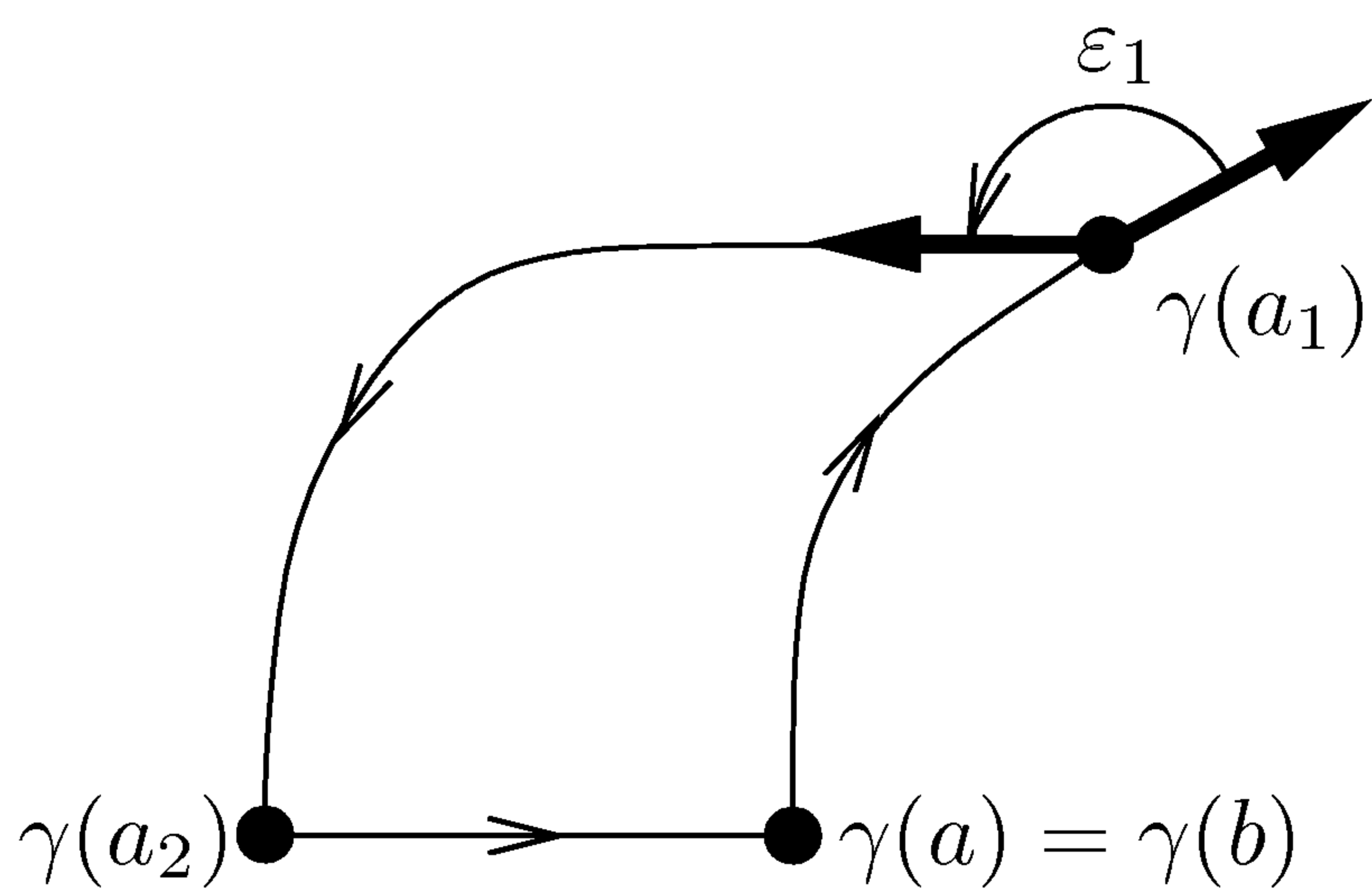
FIGURE 9.5. Defining the tangent angle at a vertex.
