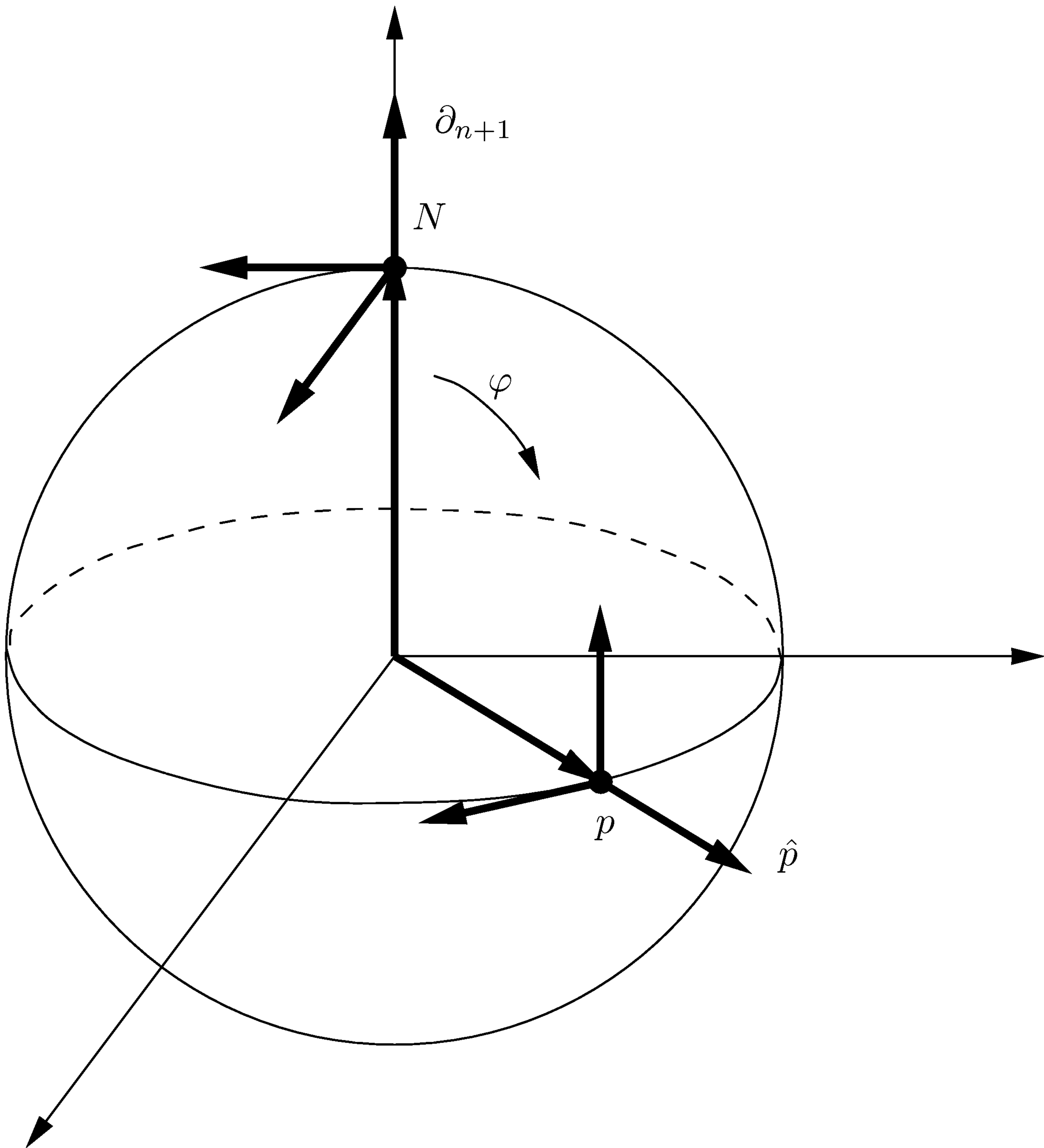
FIGURE 3.2. Transitivity of O(n + 1) on orthonormal bases.
