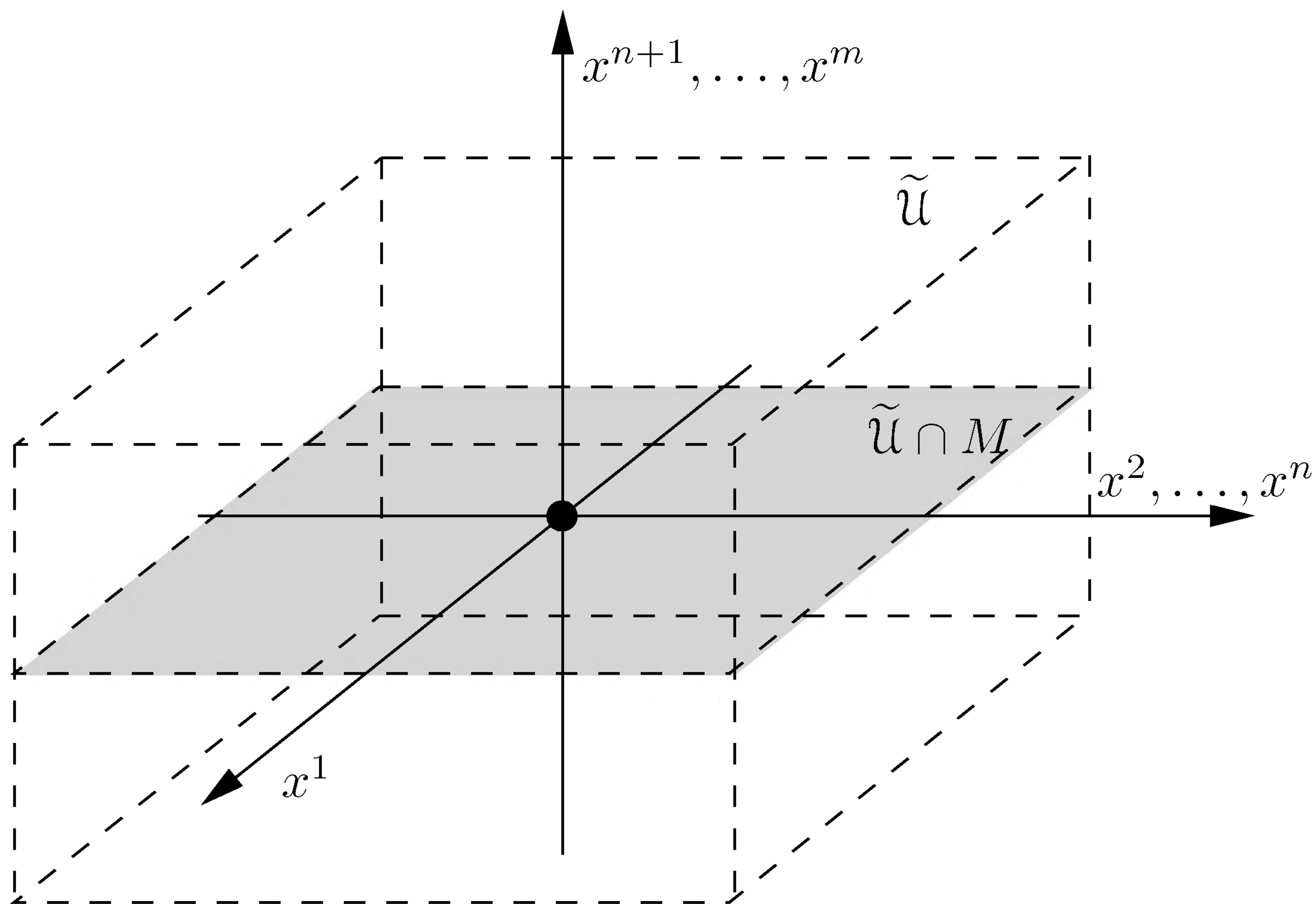
FIGURE 2.1. Slice coordinates.
