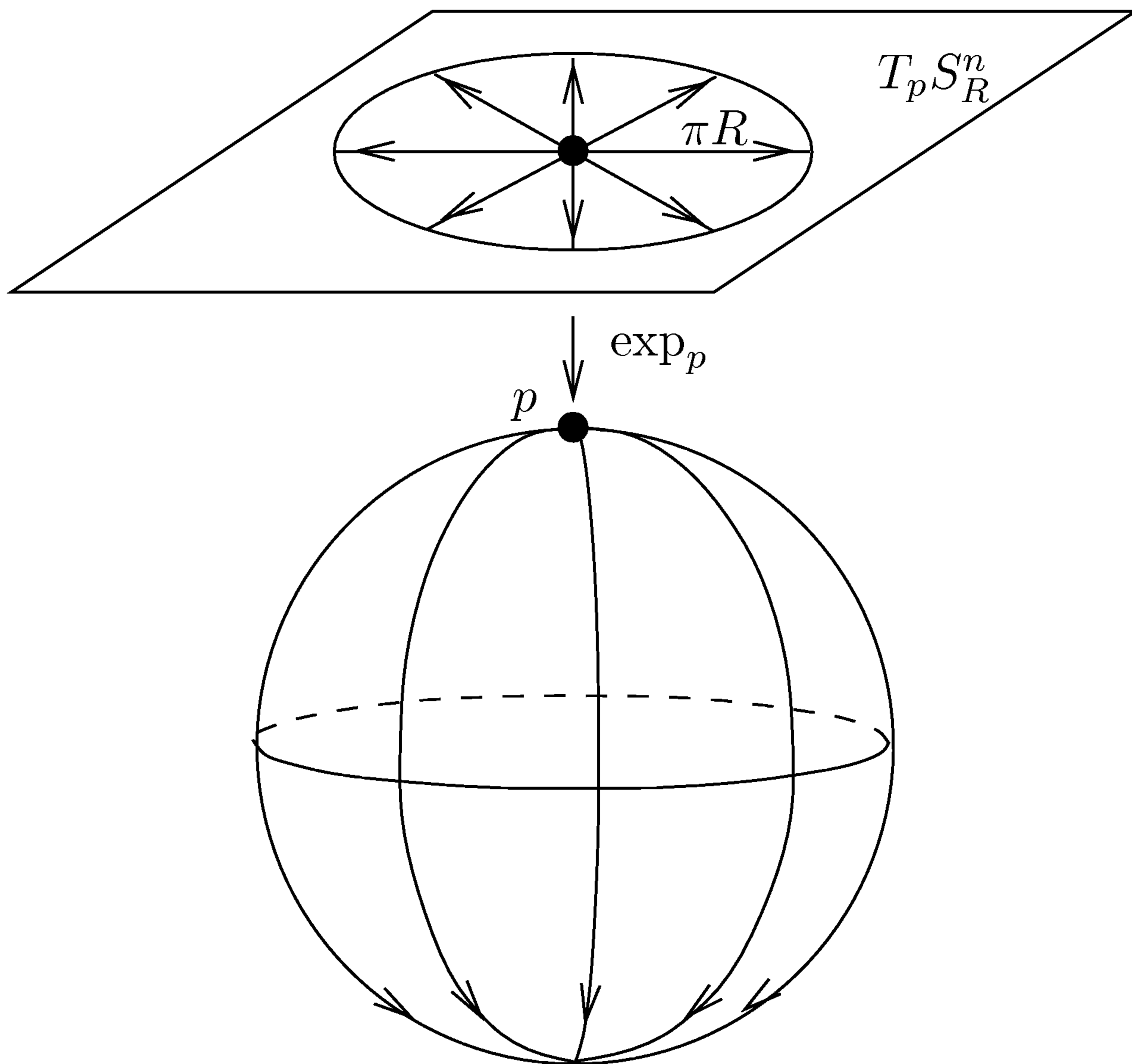
FIGURE 10.7. The exponential map of the sphere.
