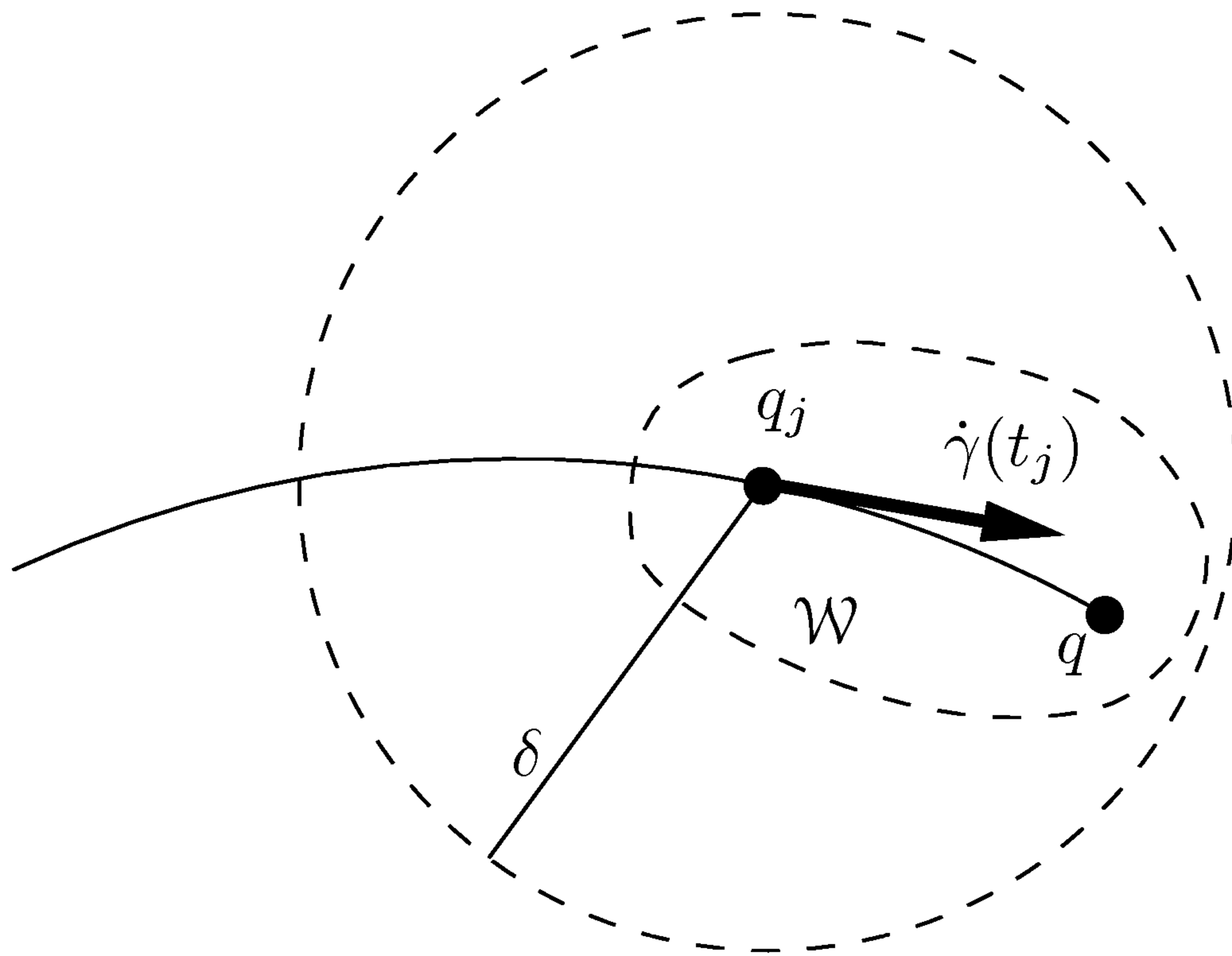
FIGURE 6.14. \gamma extends past q .
