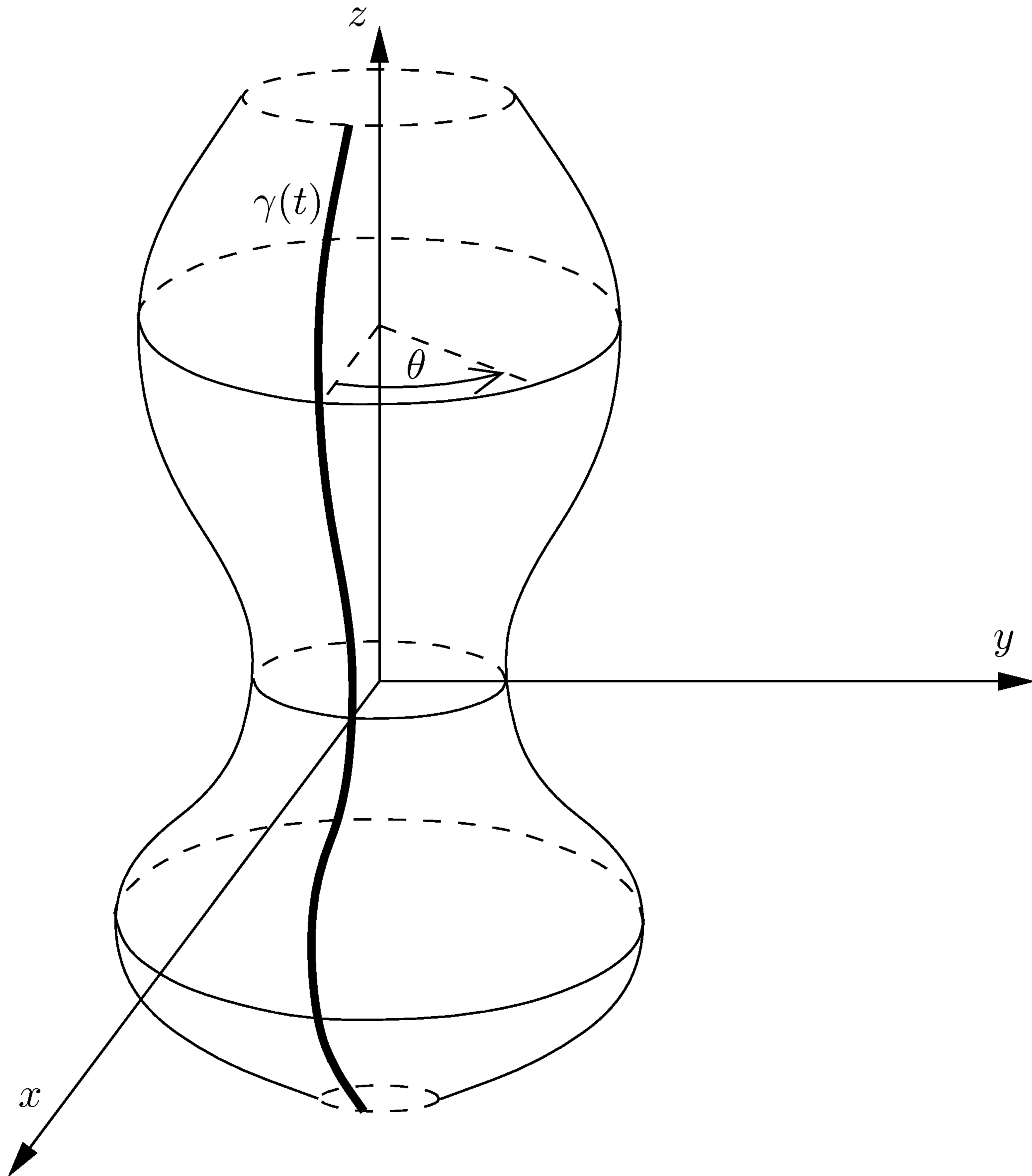
FIGURE 3.1. A surface of revolution.
