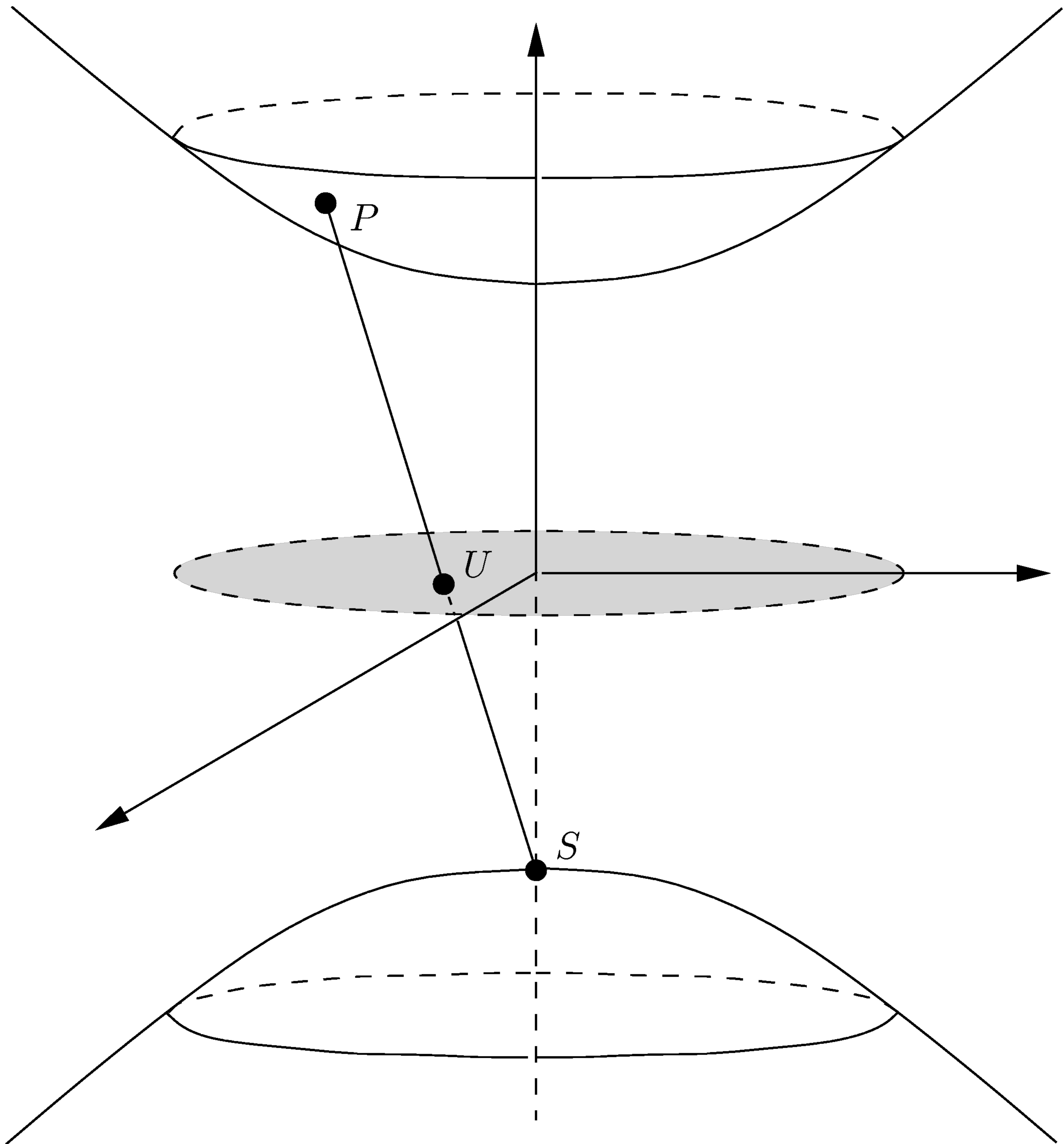
FIGURE 3.4. Hyperbolic stereographic projection.
