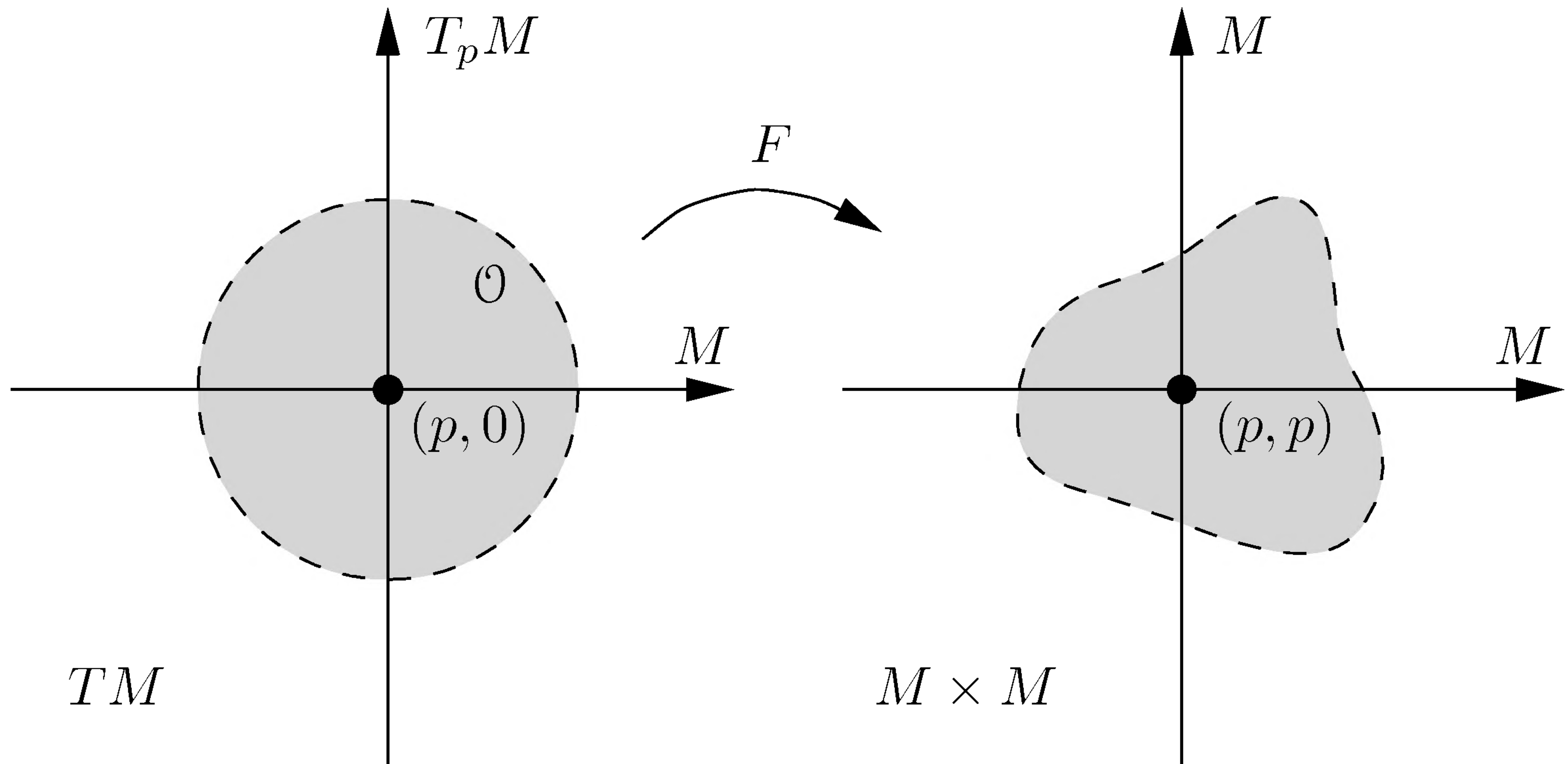
FIGURE 5.5. F is a diffeomorphism near (p, 0) .
