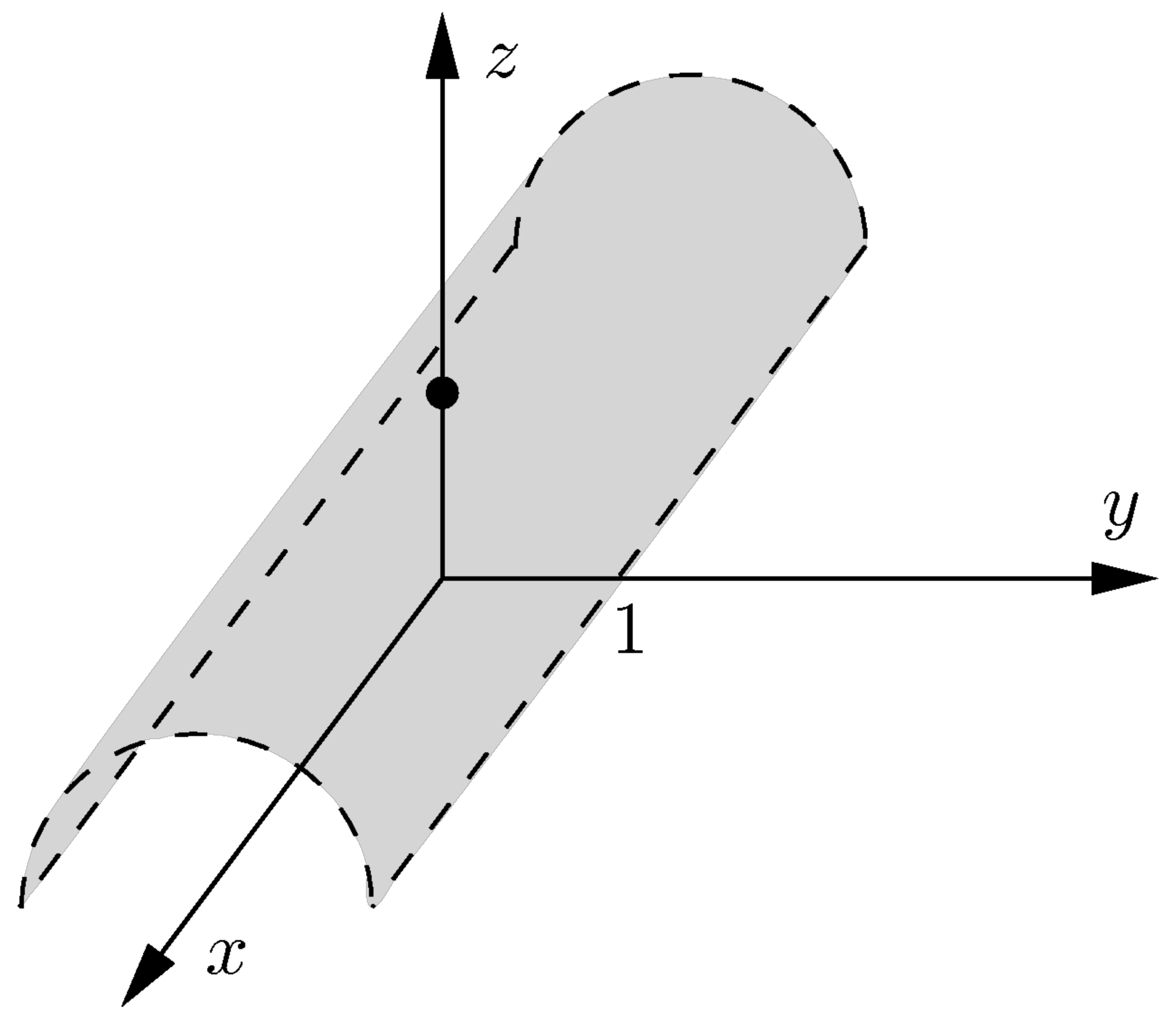
FIGURE 1.4. S_2 .
