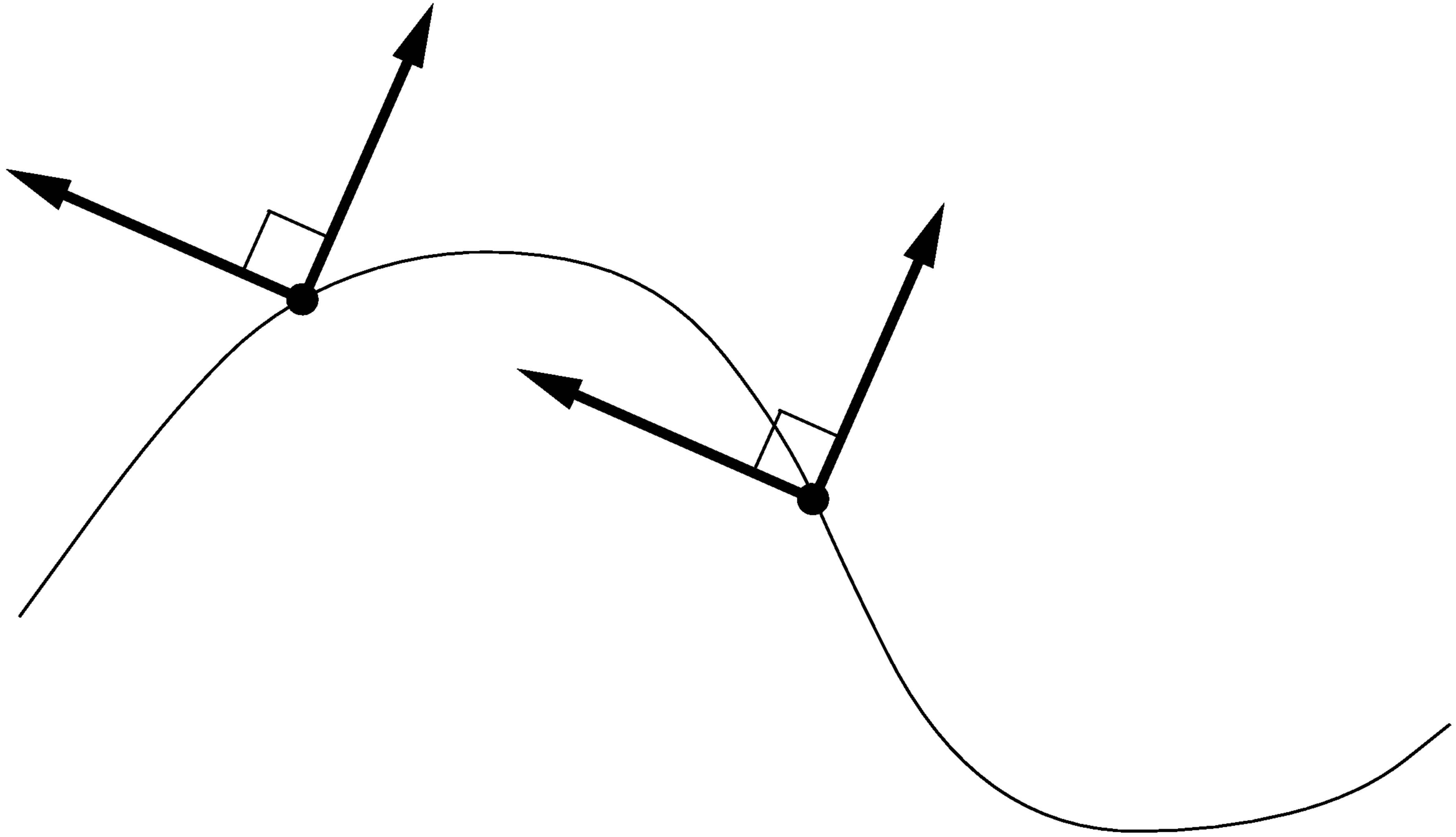
FIGURE 5.1. Parallel translation is an isometry.
