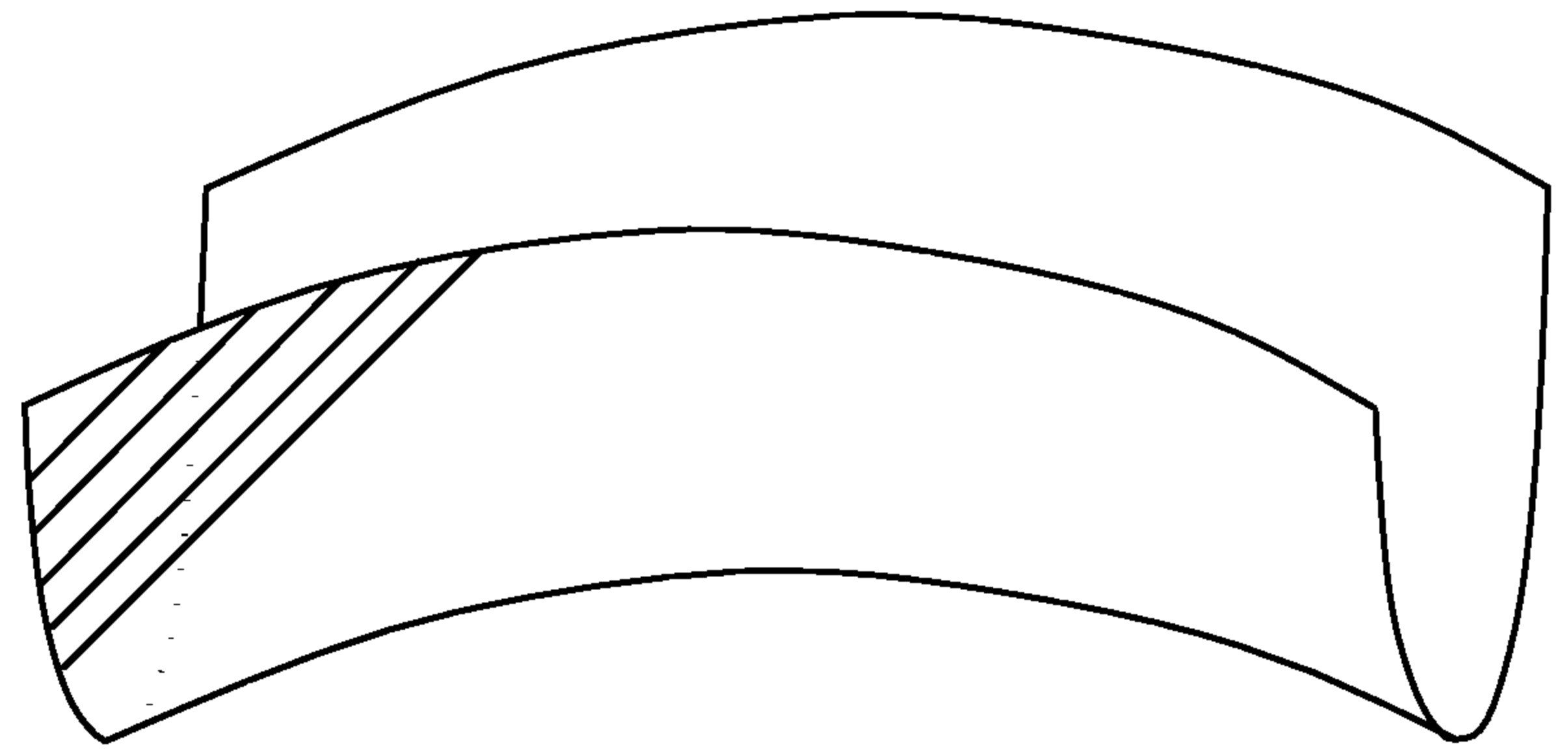
FIGURE 1.6. K < 0 .
