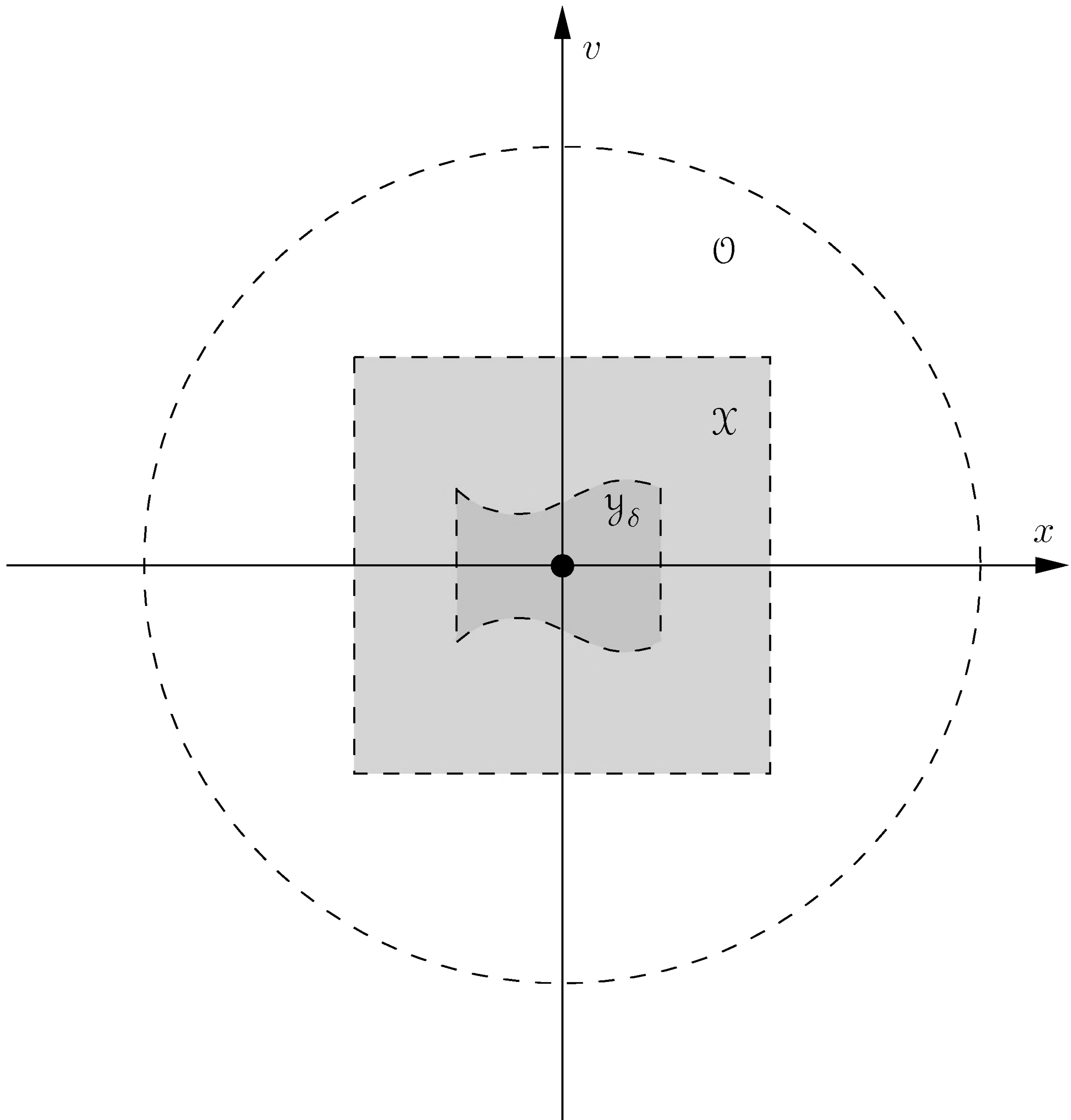
FIGURE 5.6. The sets \mathcal{Y}_\delta \subset \mathcal{X} \subset \mathcal{O} .
