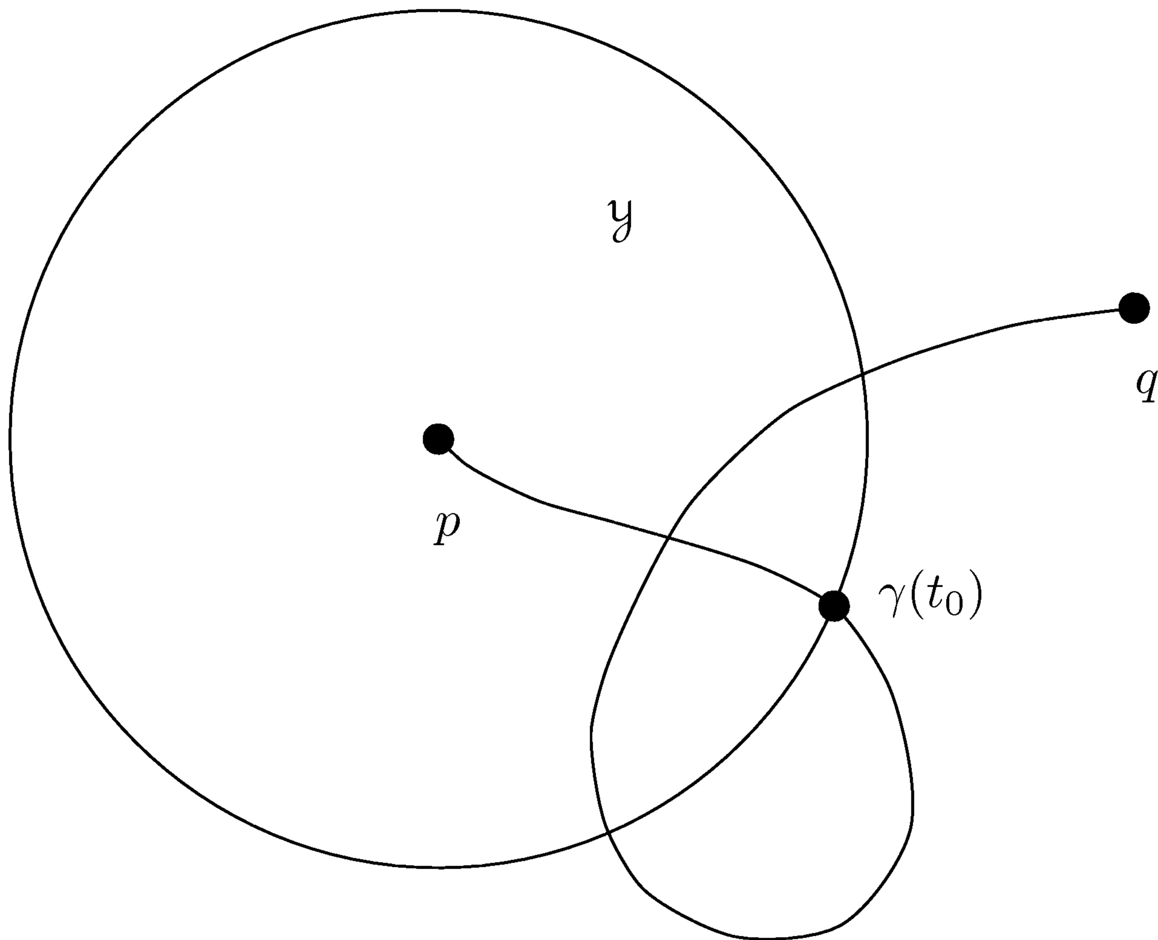
FIGURE 6.3. d(p, q) > 0 .
