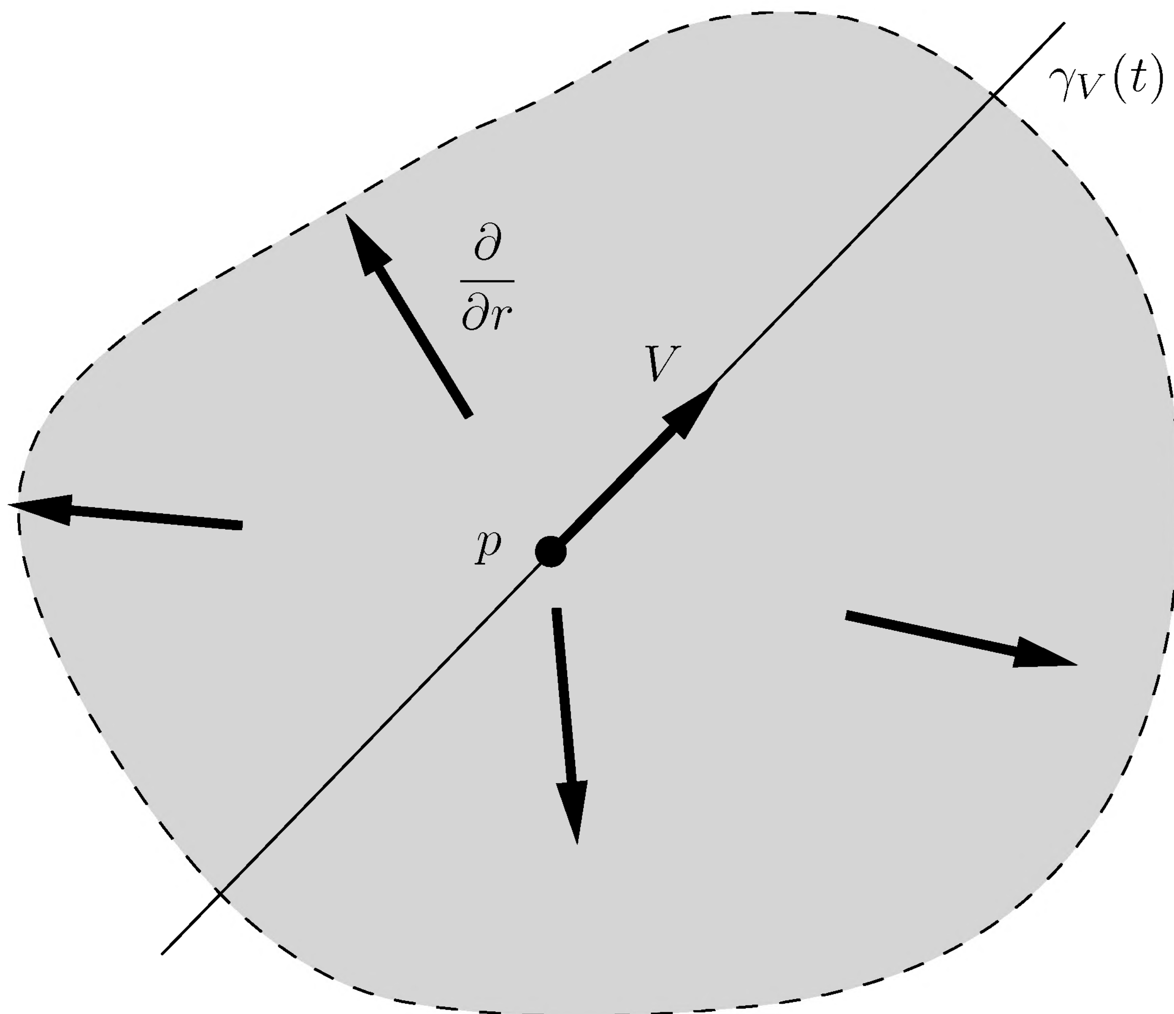
FIGURE 5.3. Riemannian normal coordinates.
