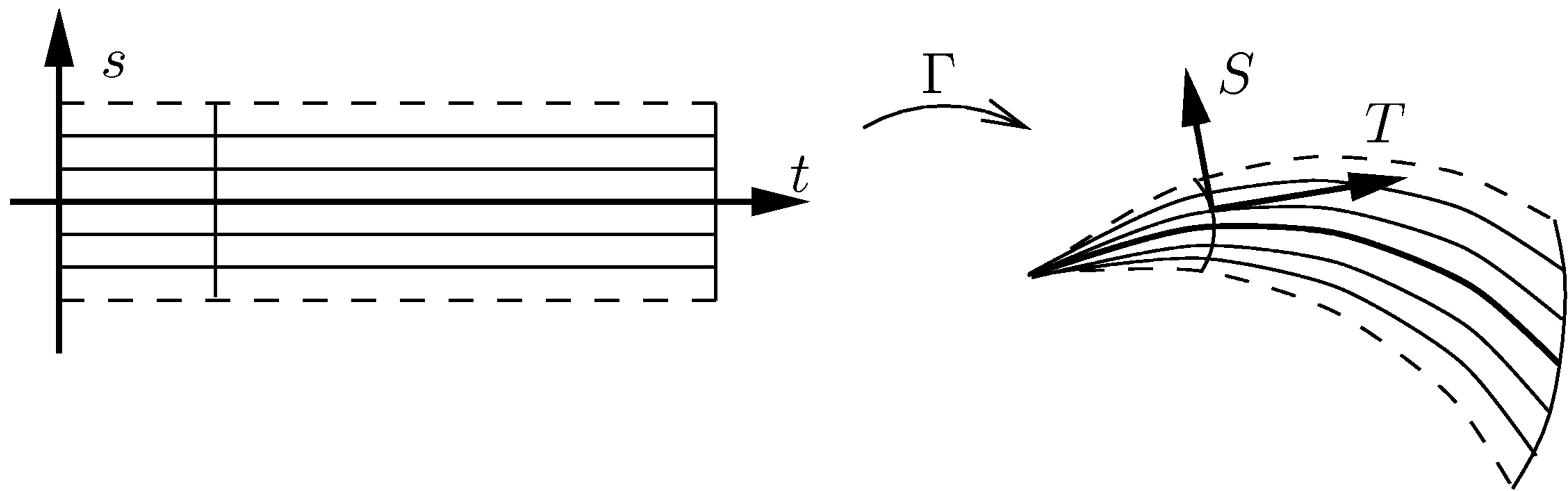
FIGURE 6.10. The variation \Gamma .
