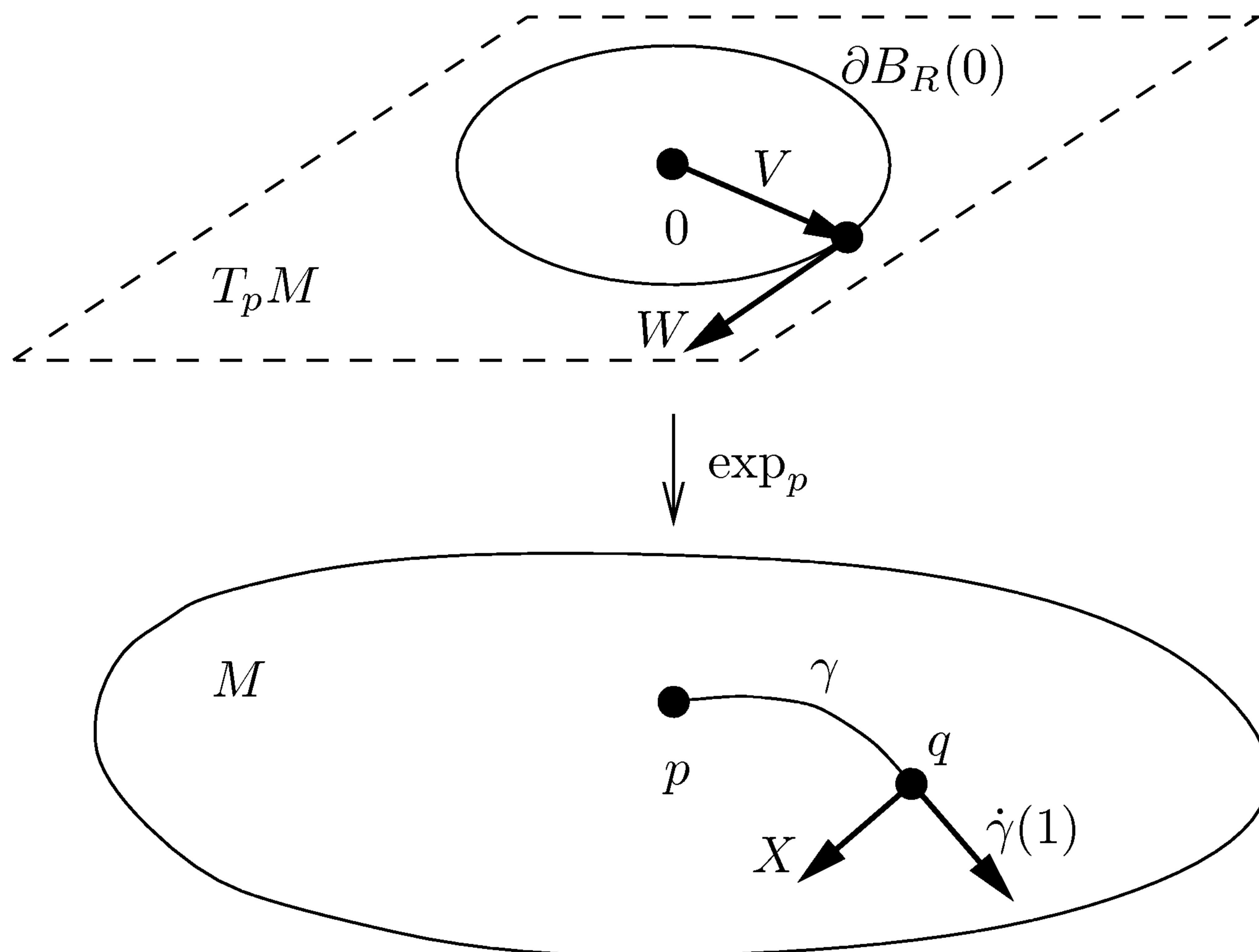
FIGURE 6.9. Proof of the Gauss lemma.
