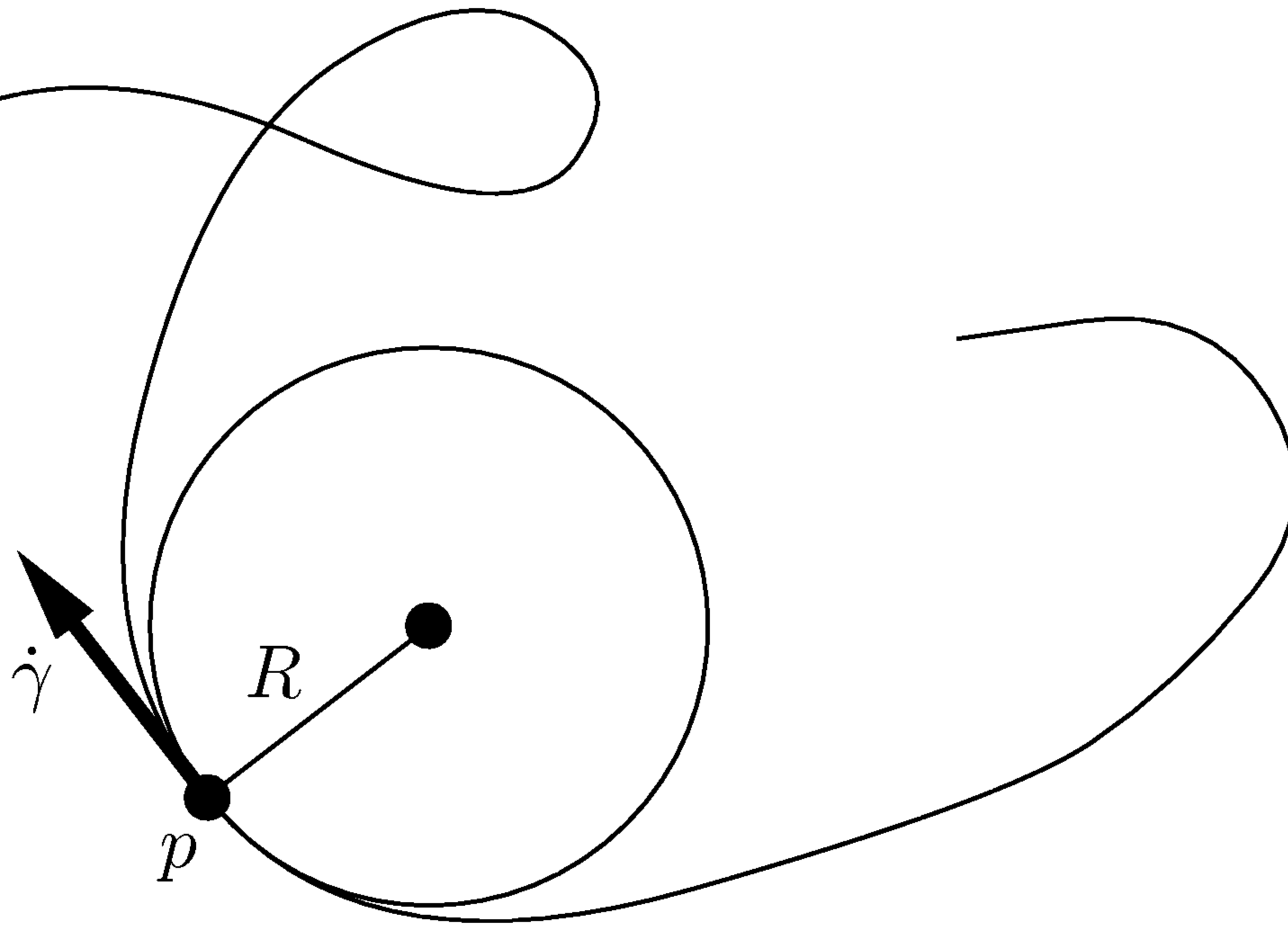
FIGURE 1.1. Osculating circle.
