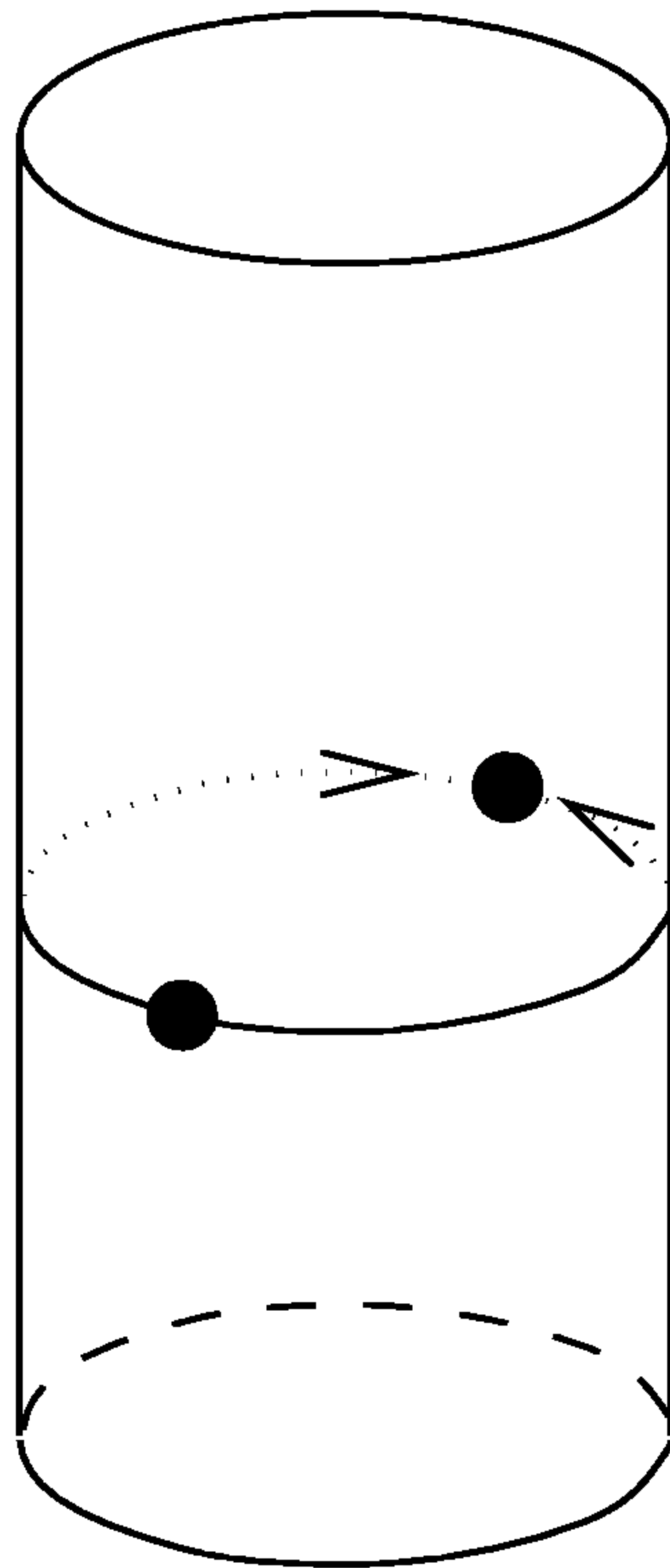
FIGURE 10.11. Geodesics on the cylinder.
