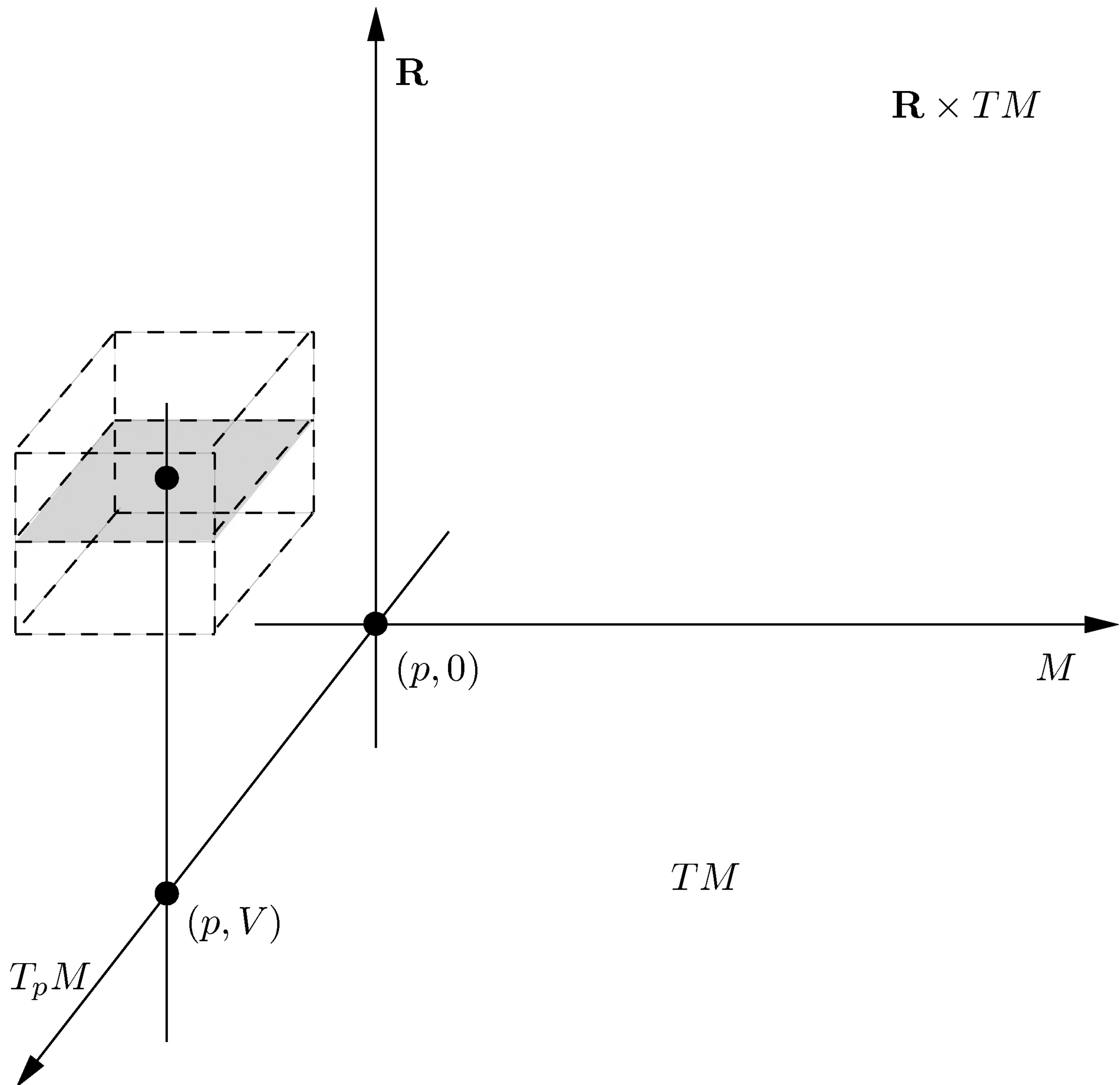
FIGURE 5.2. \mathcal{E} is open.
