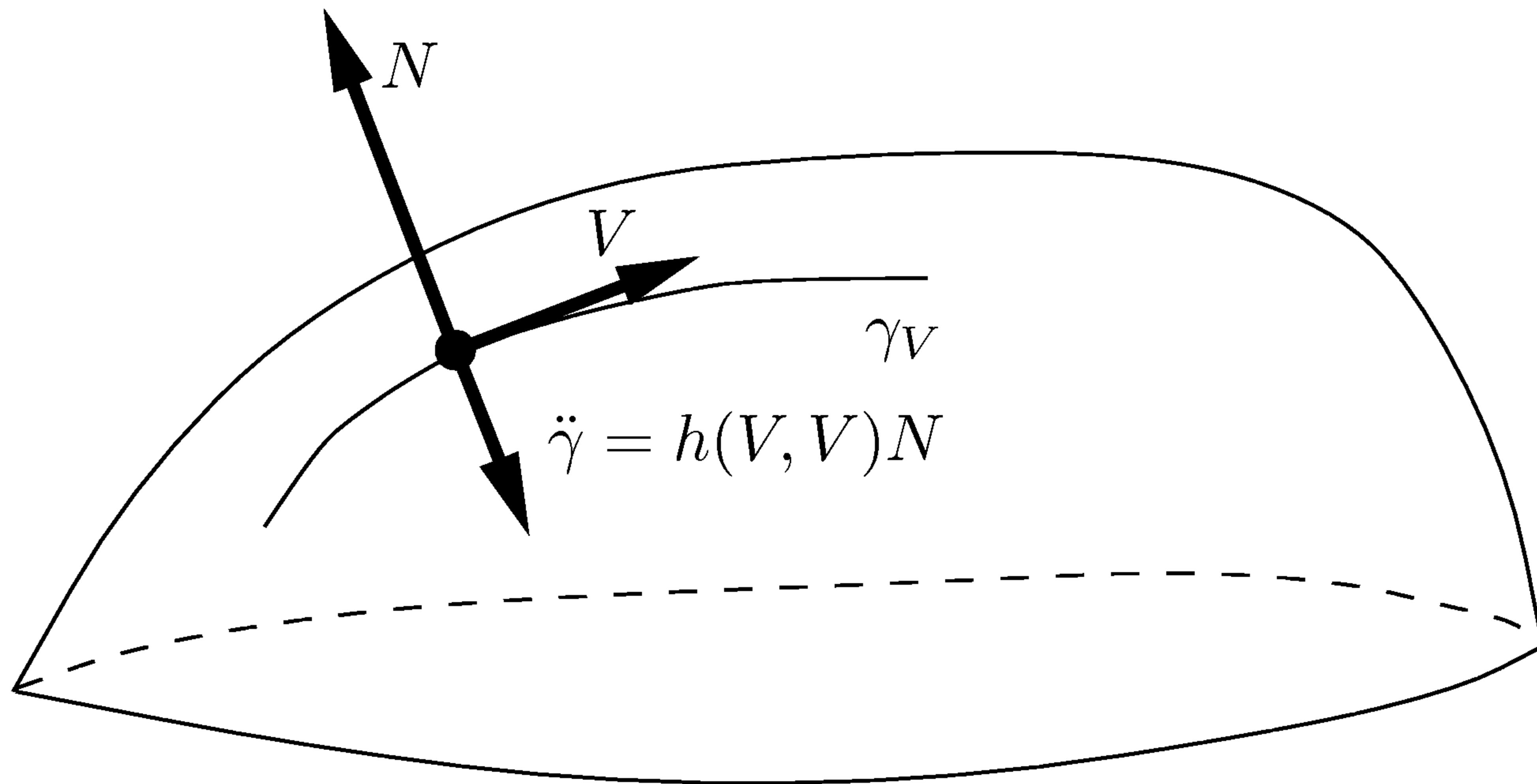
FIGURE 8.3. Geometric interpretation of h(V, V) .
