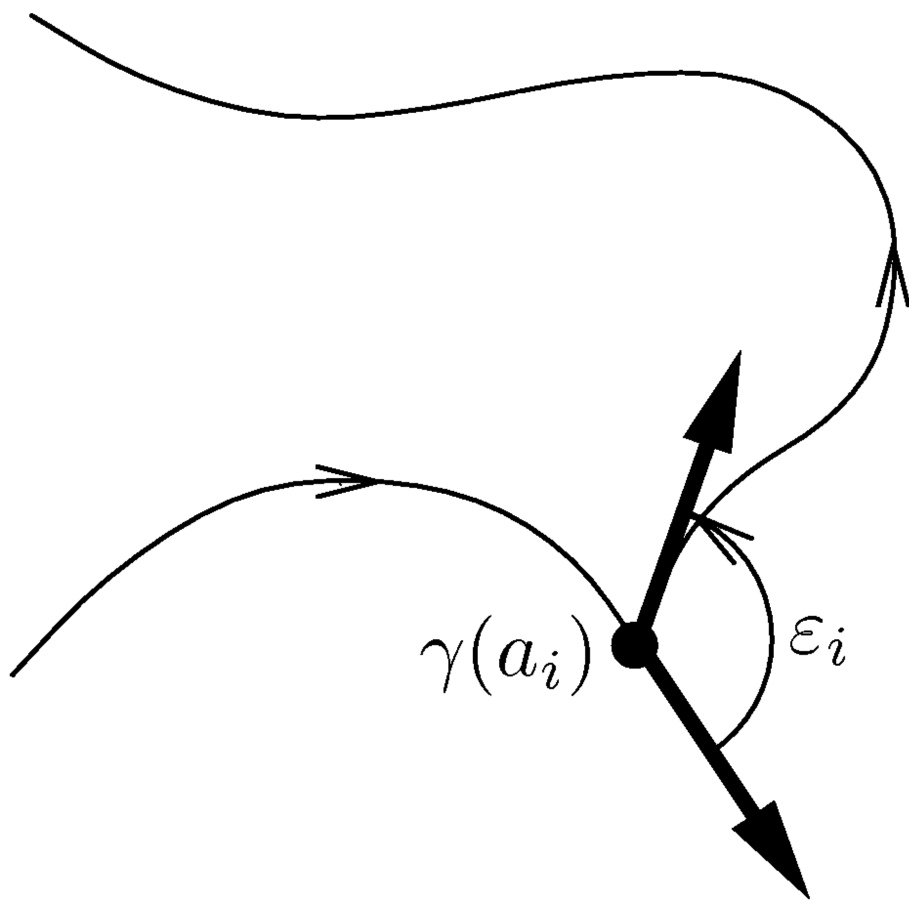
FIGURE 9.2. An exterior angle.
