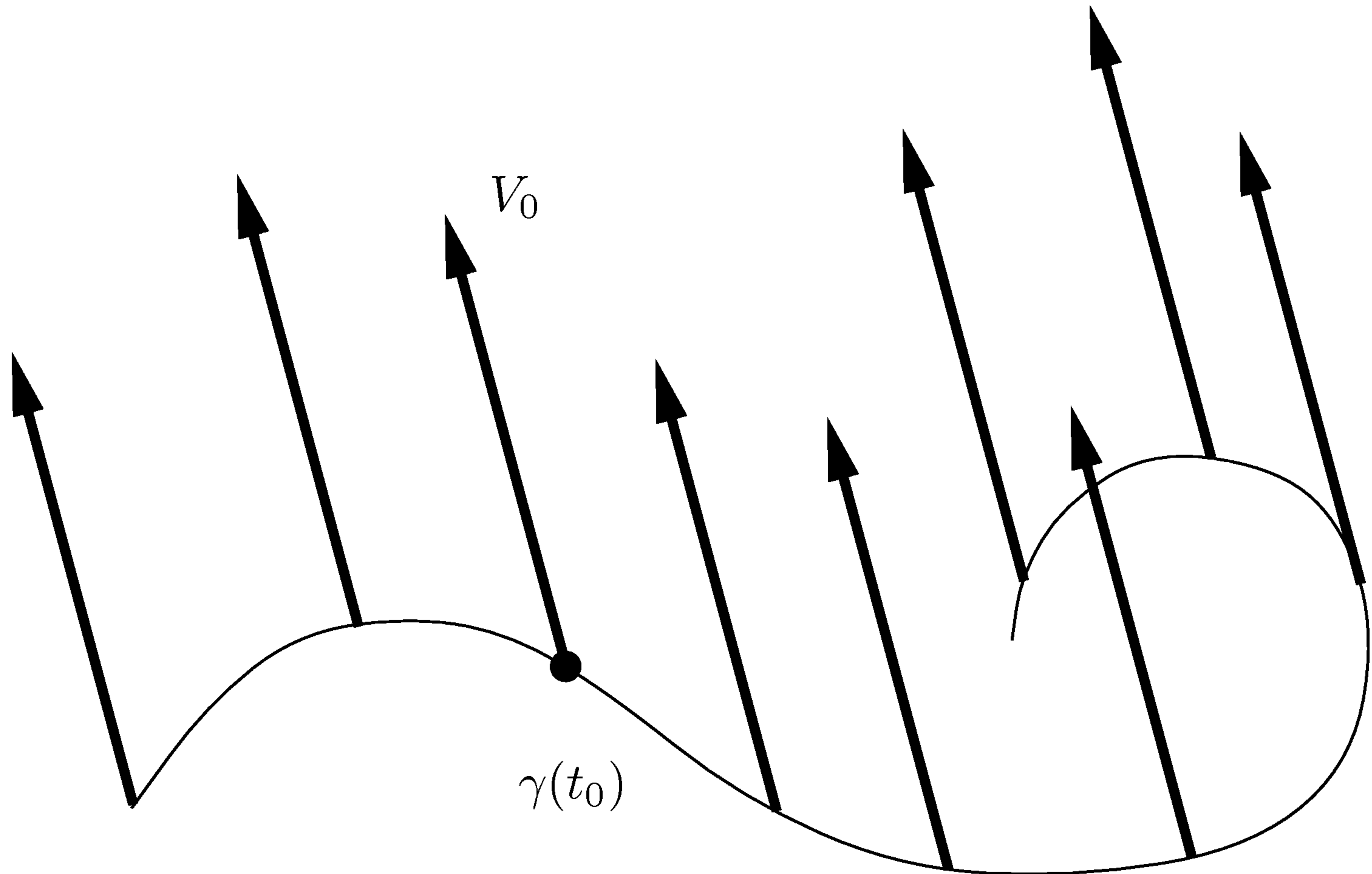
FIGURE 4.7. Parallel translate of V_0 along \gamma .
