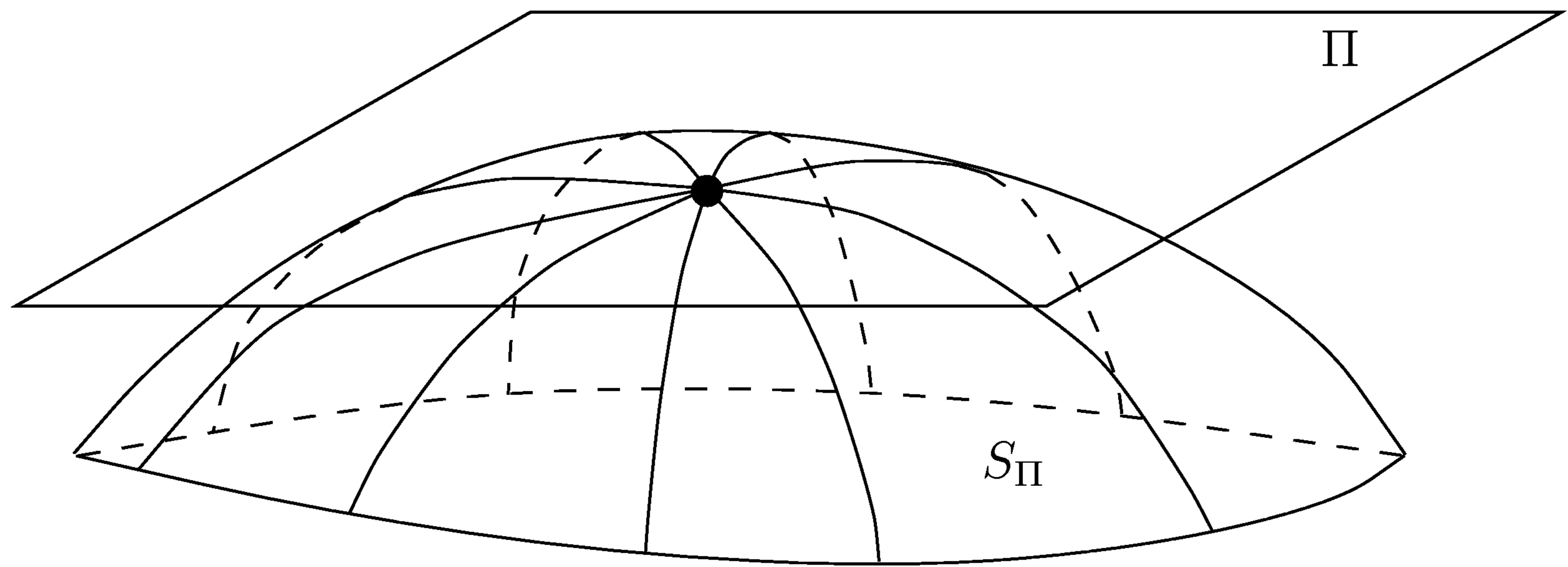
FIGURE 8.4. A plane section.
