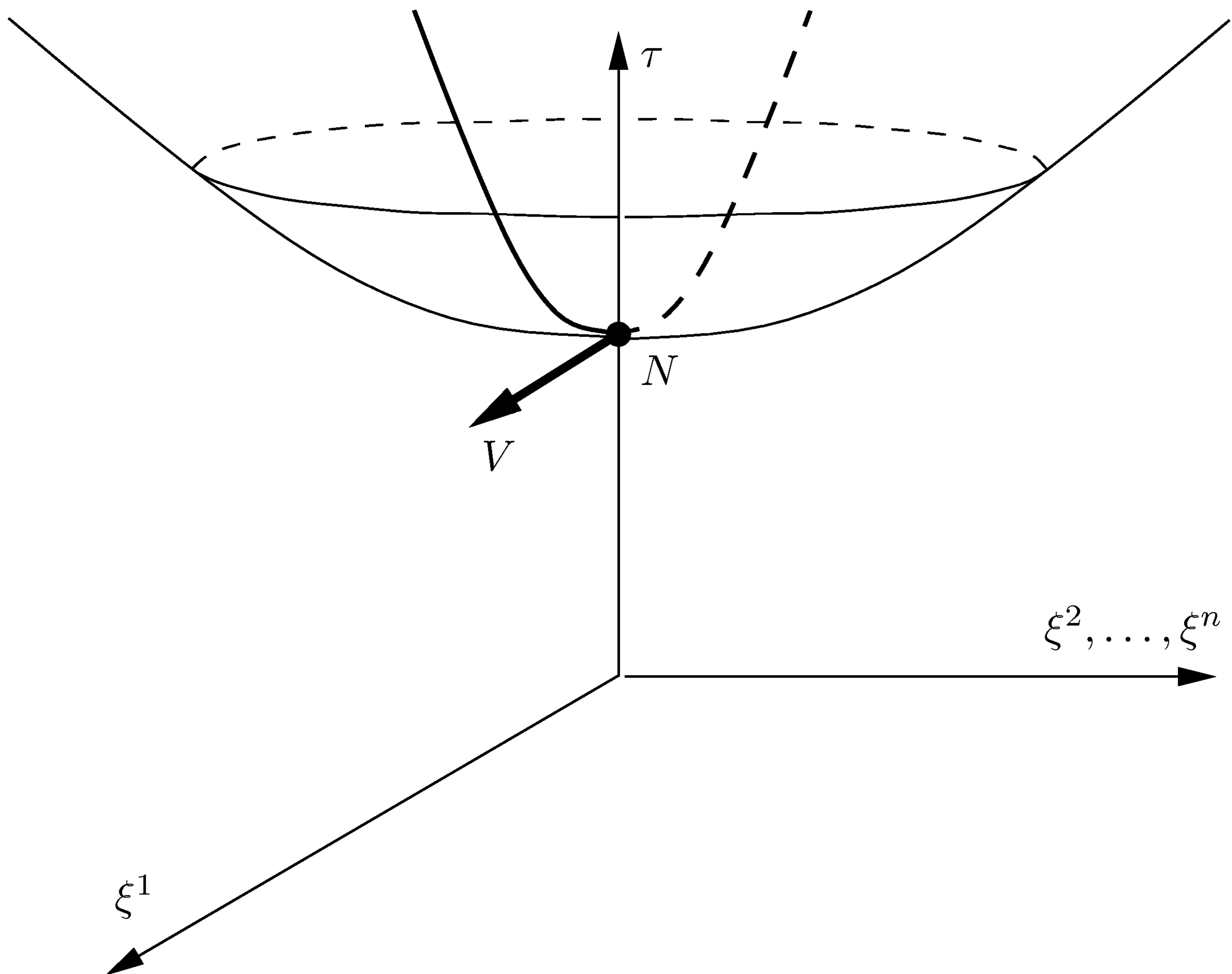
FIGURE 5.10. A great hyperbola.
