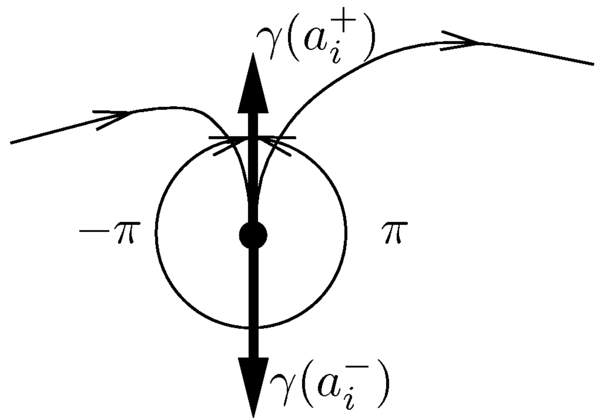
FIGURE 9.3. A cusp.
