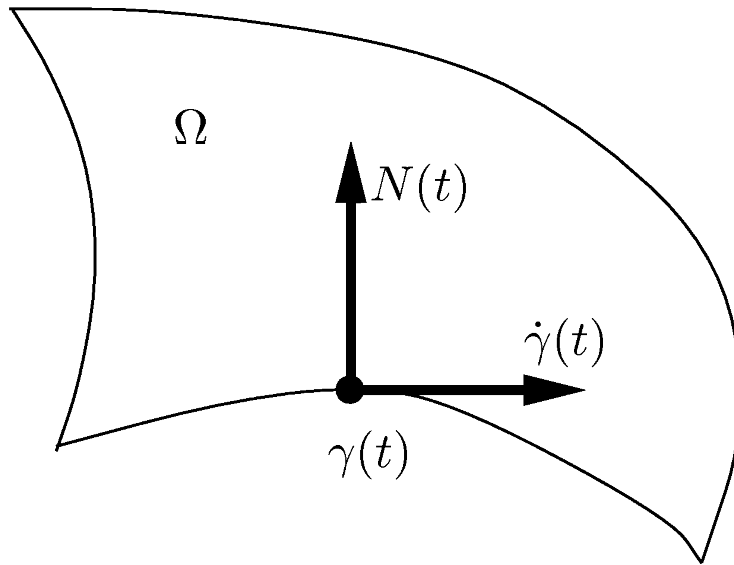
FIGURE 9.13. N(t) is the inward-pointing normal.
