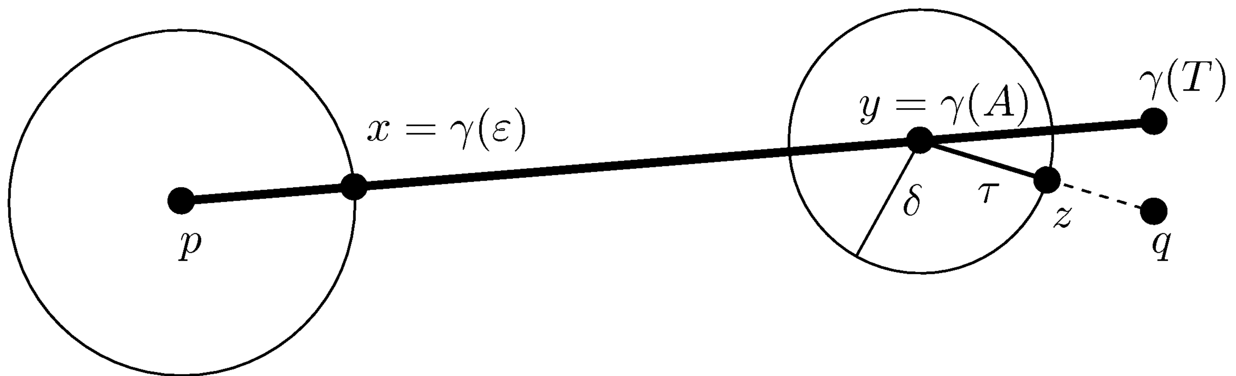
FIGURE 6.16. Proof that A = T .
