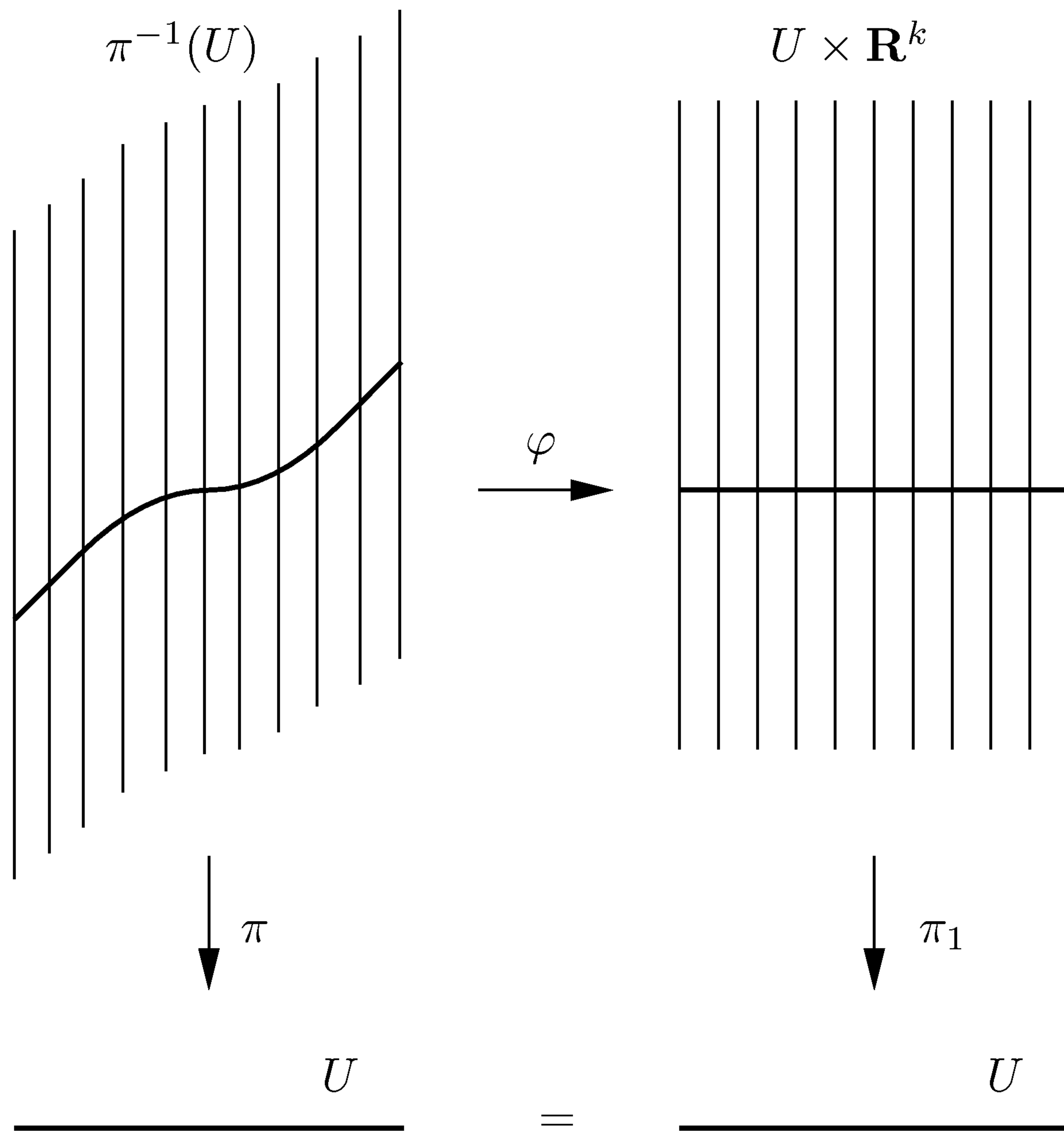
FIGURE 2.2. A local trivialization.
