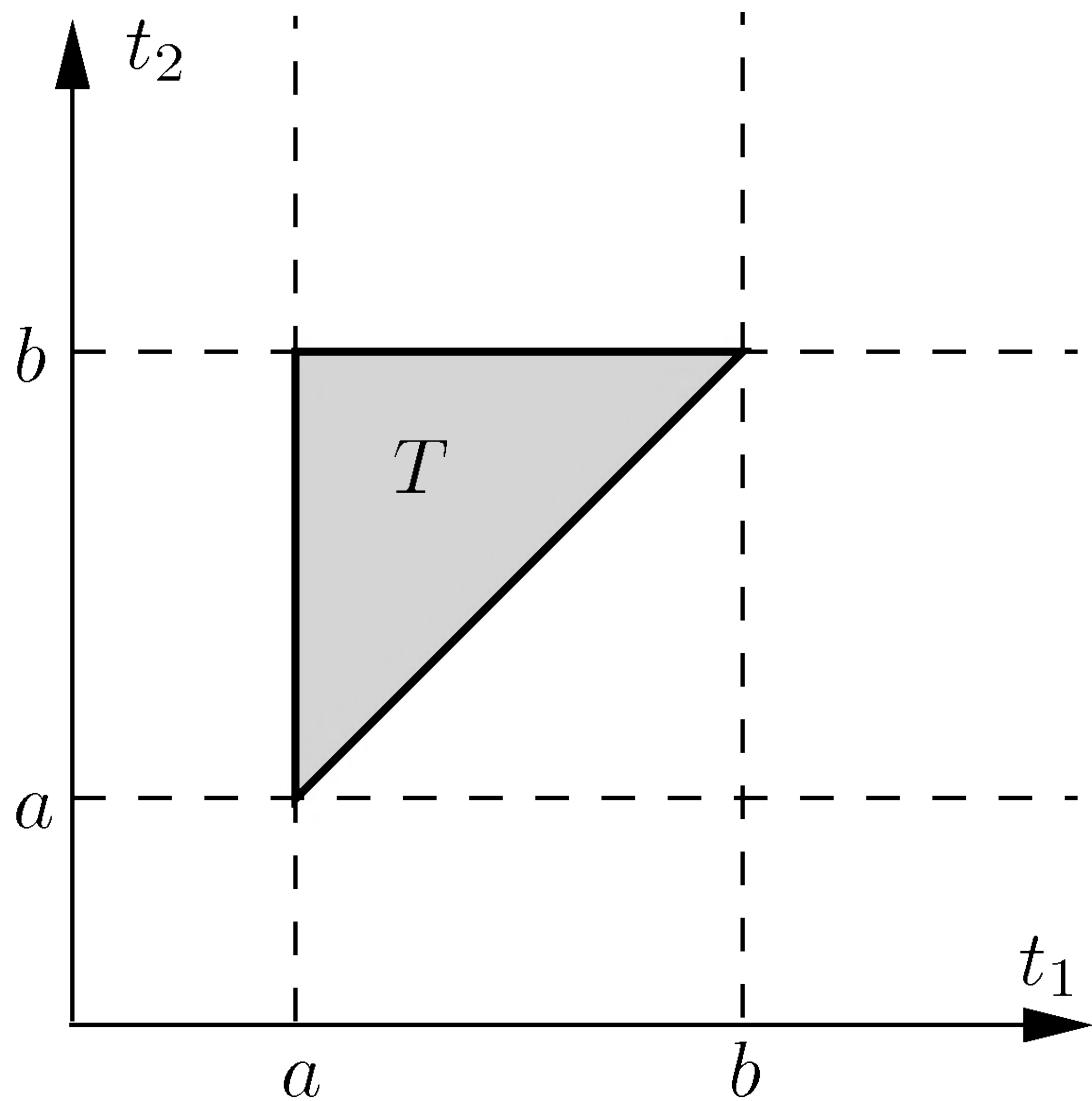
FIGURE 9.8. The domain of the secant angle function.
