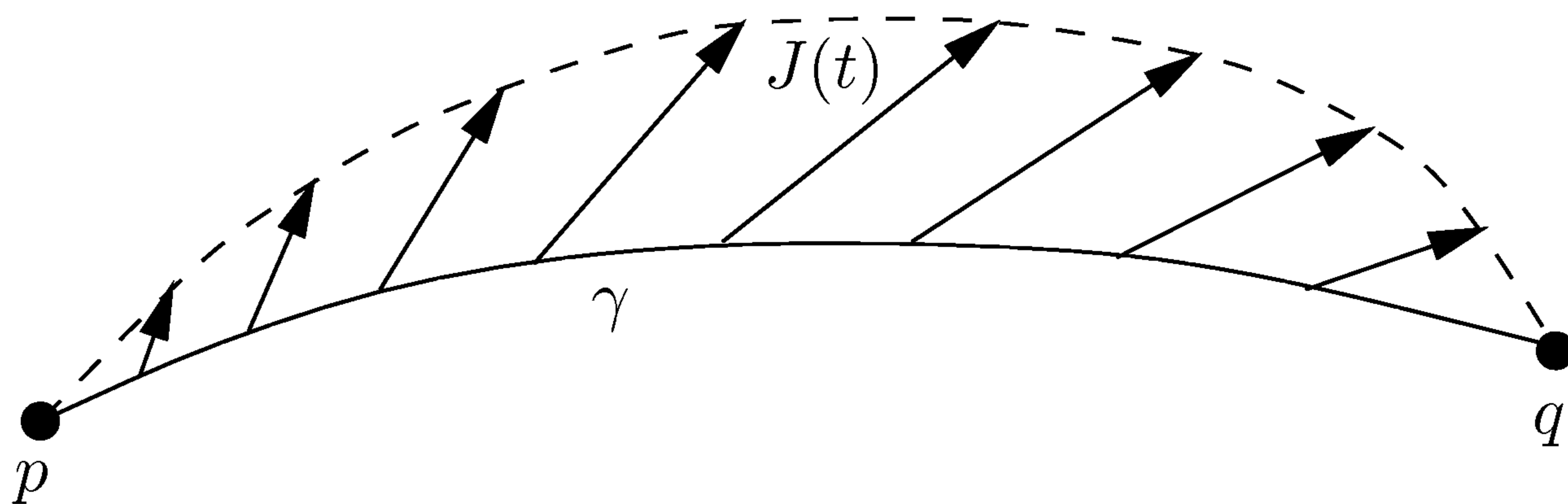
FIGURE 10.8. Conjugate points.
