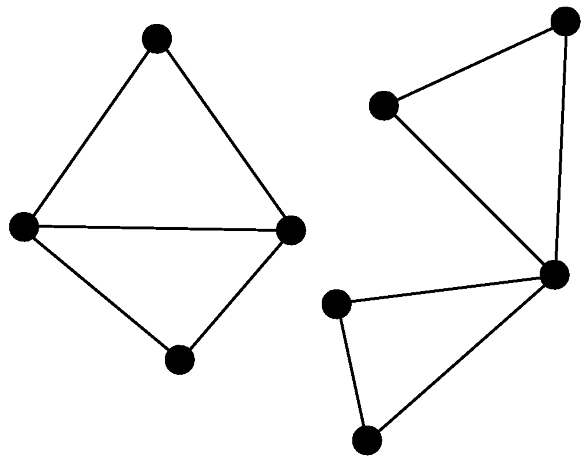
FIGURE 9.15. Valid intersections.
