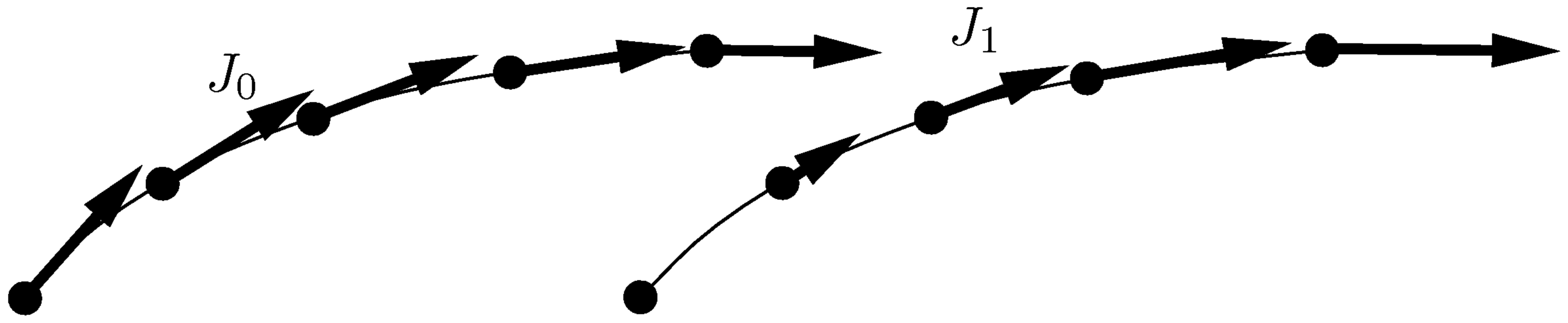
FIGURE 10.3. Trivial Jacobi fields.
