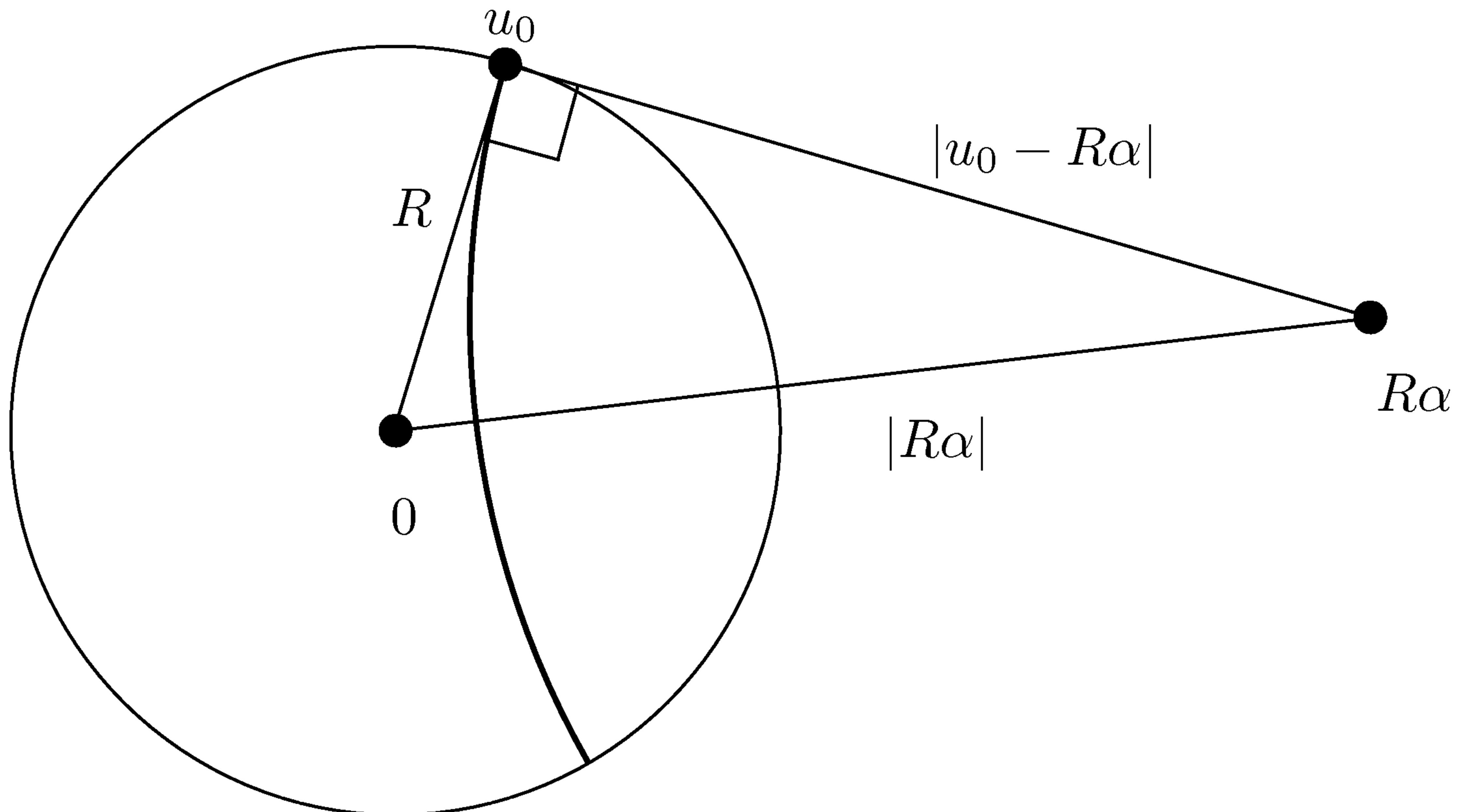
FIGURE 5.11. Geodesics are arcs of circles orthogonal to the boundary.
