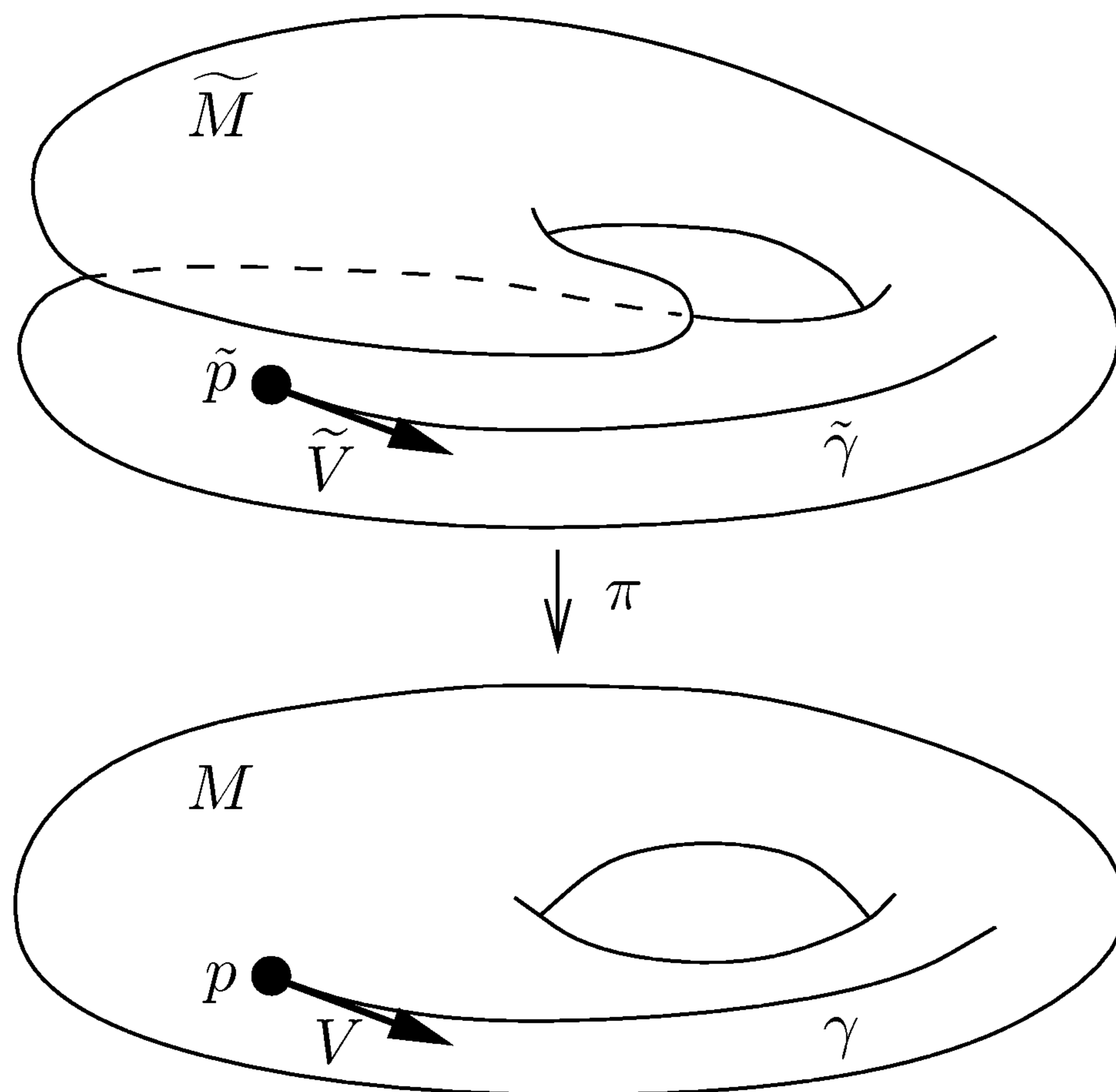
FIGURE 11.1. Lifting geodesics.
