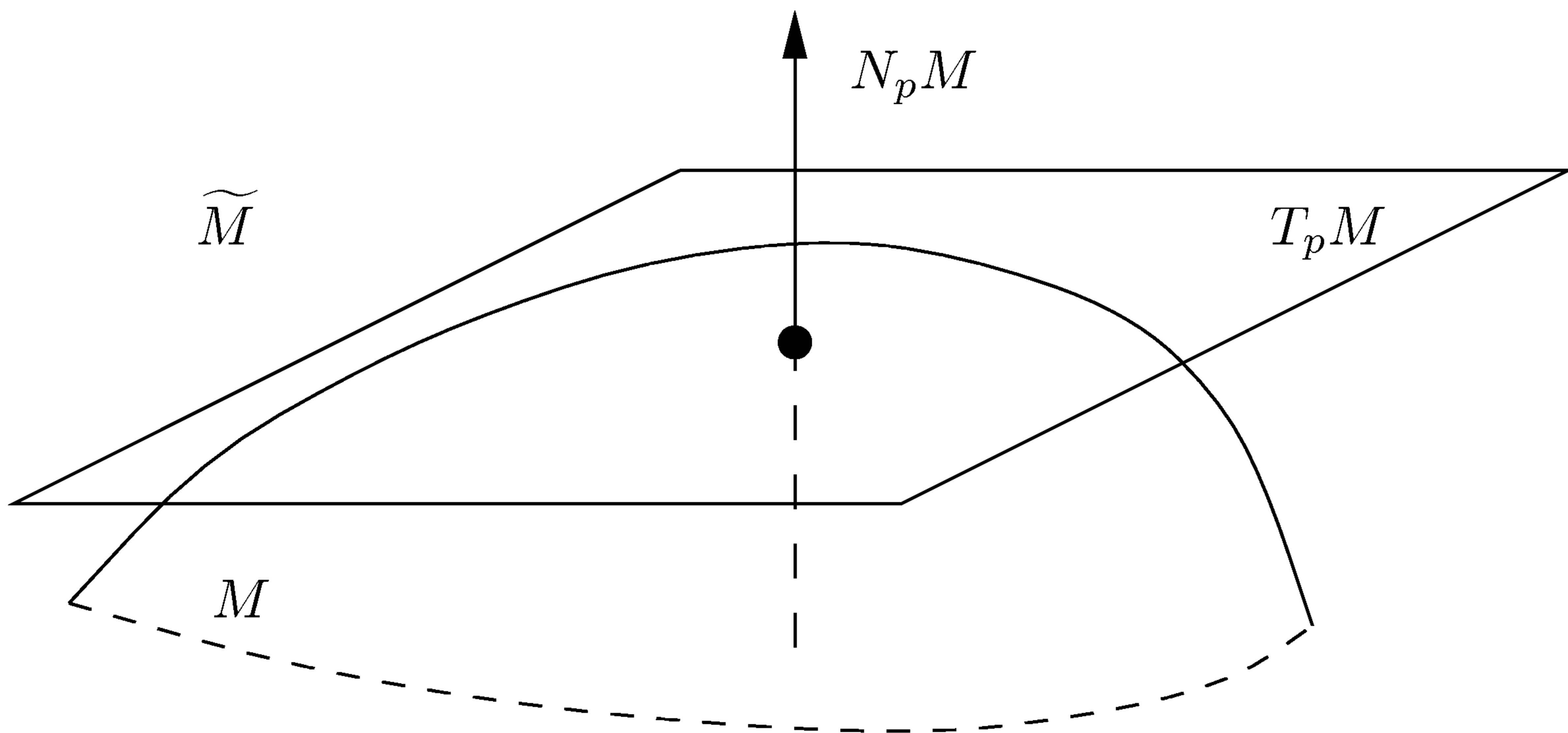
FIGURE 8.1. The normal space at p .
