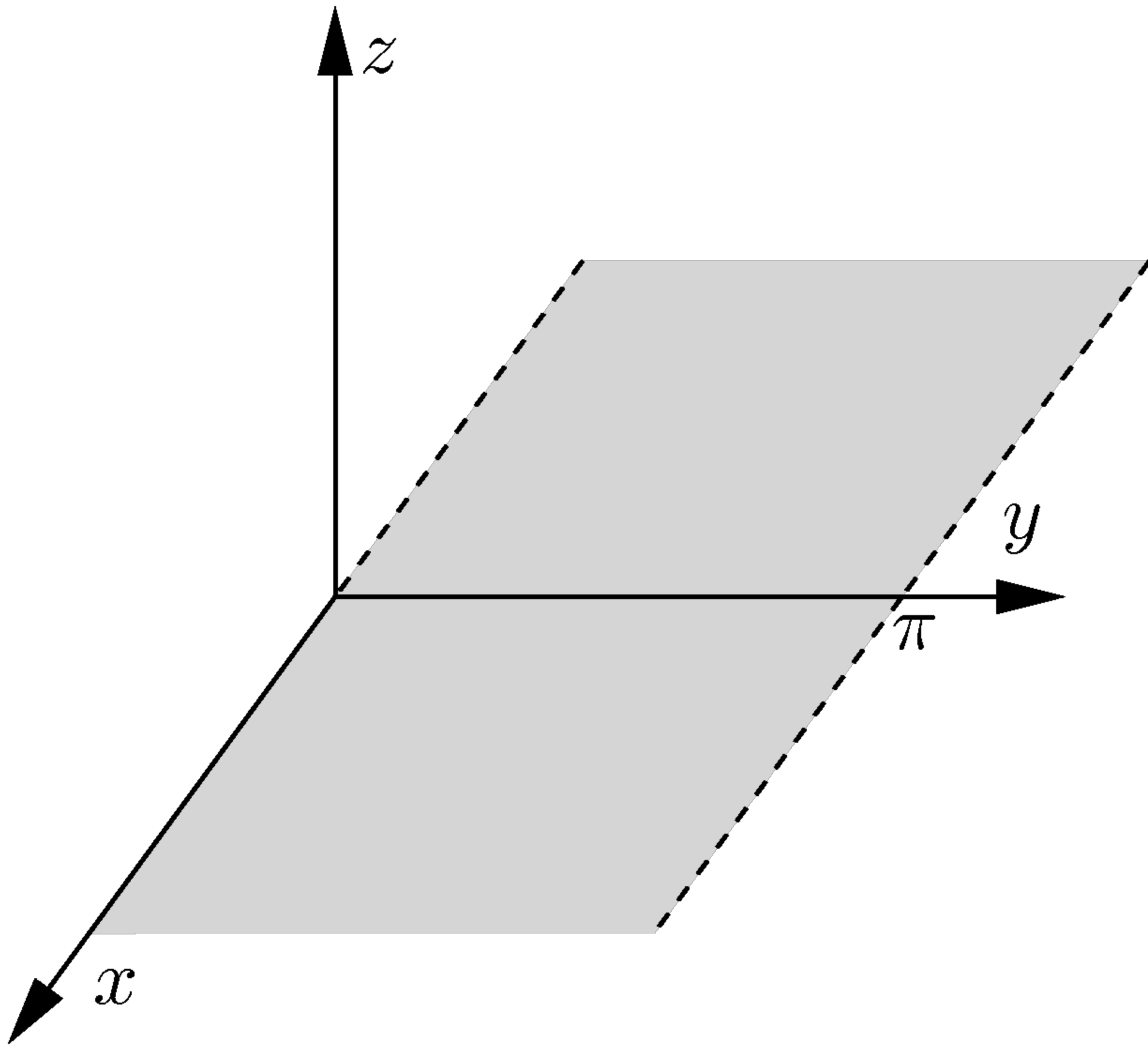
FIGURE 1.3. S_1 .
