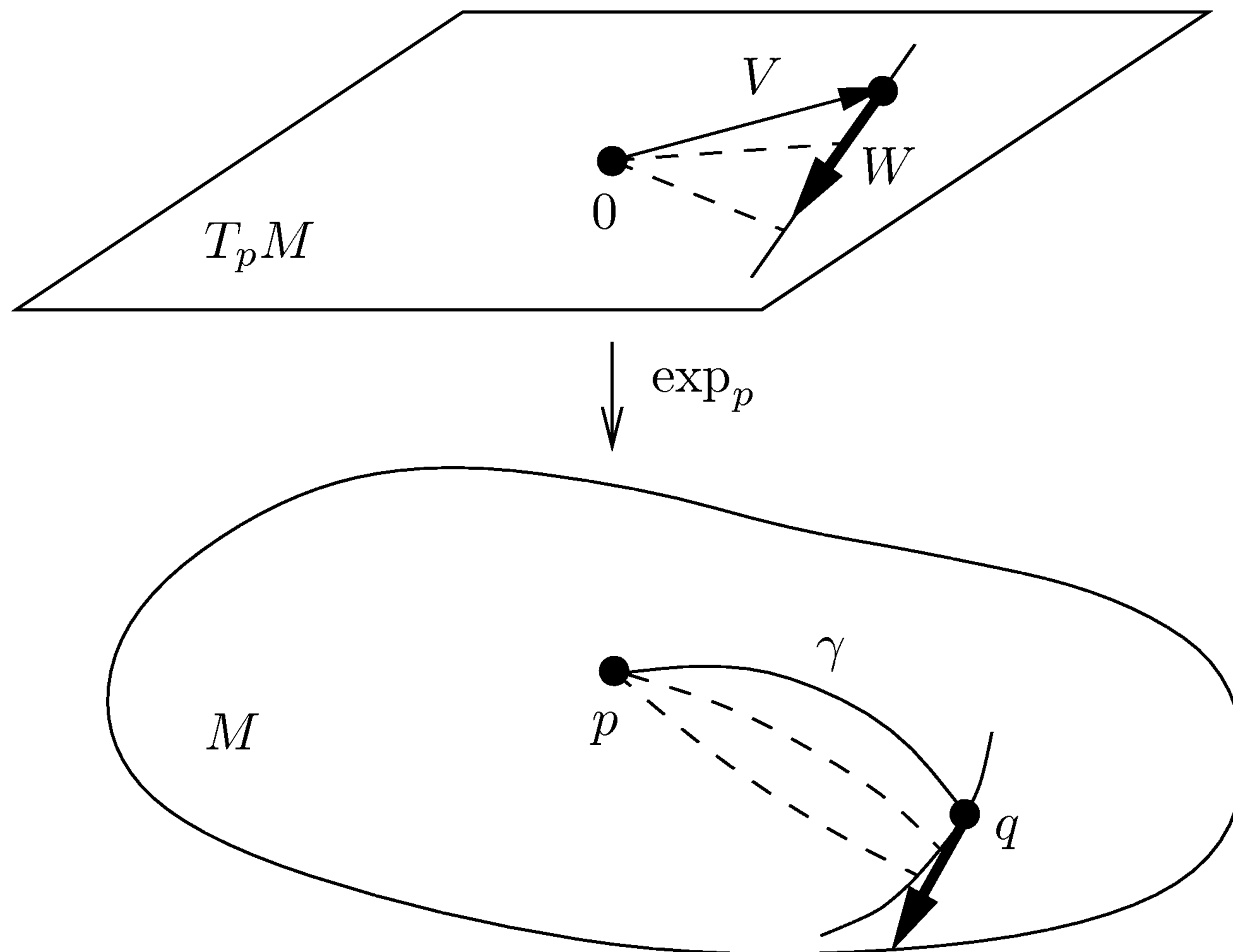
FIGURE 10.9. Computing (\exp_p)_*W .
