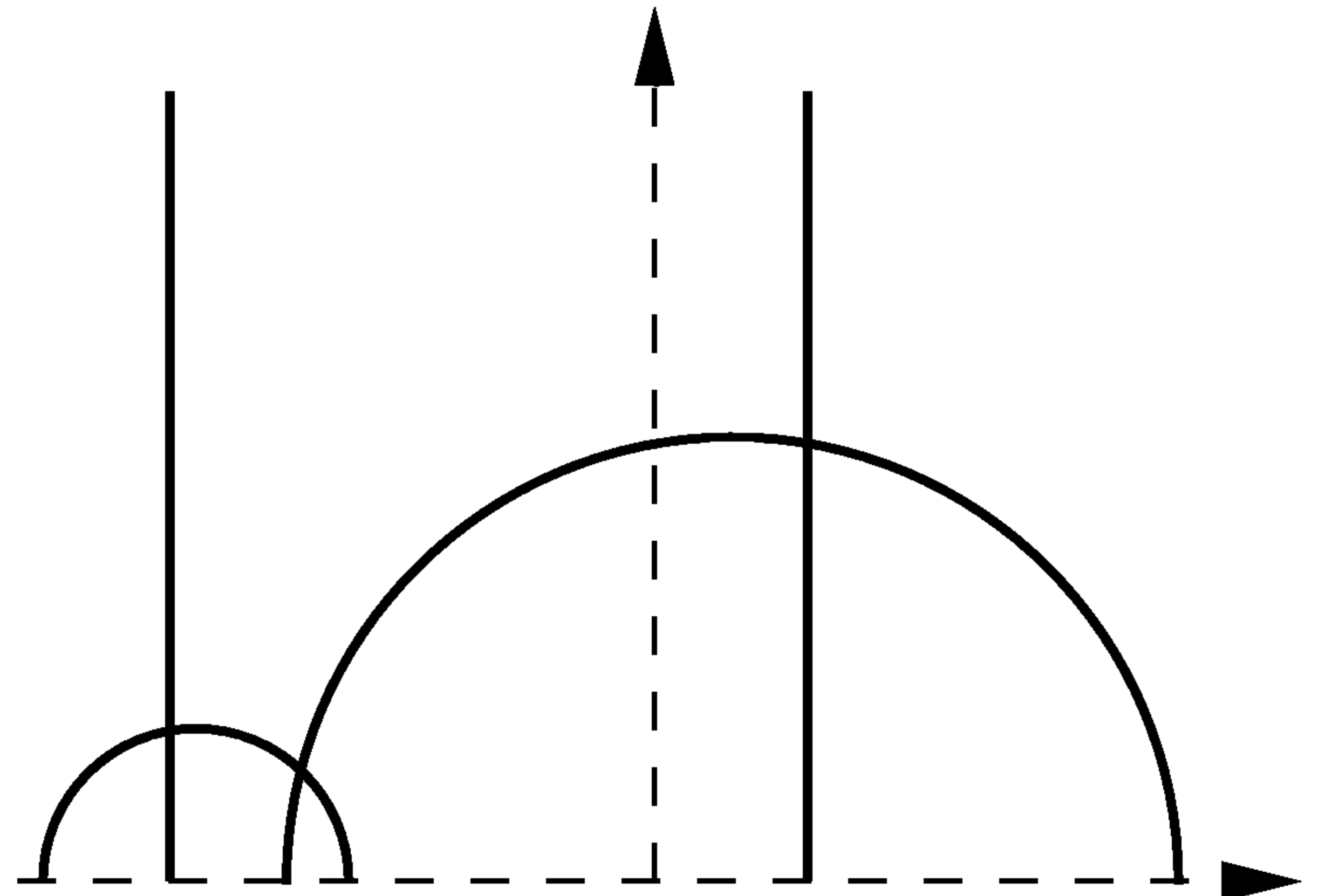
FIGURE 5.9. Geodesics of the Poincaré half-space.
