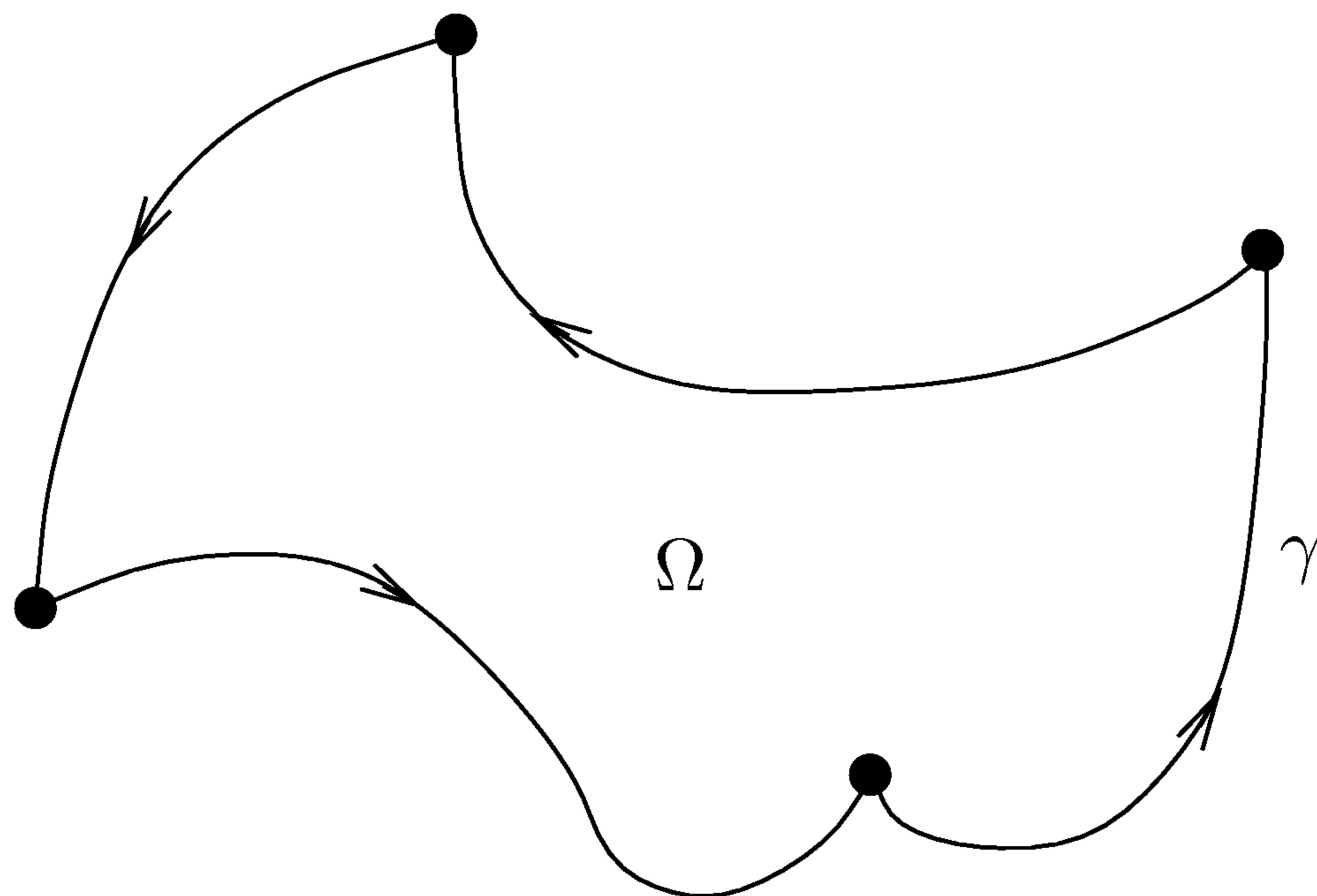
FIGURE 9.4. A positively oriented curved polygon.
