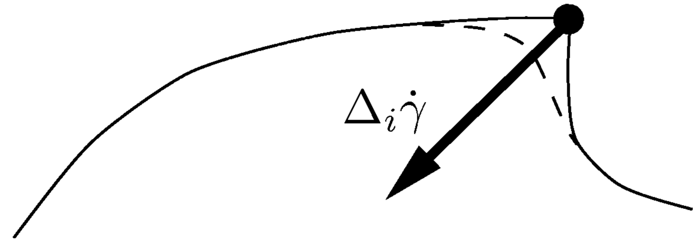
FIGURE 6.8. Rounding the corner.
