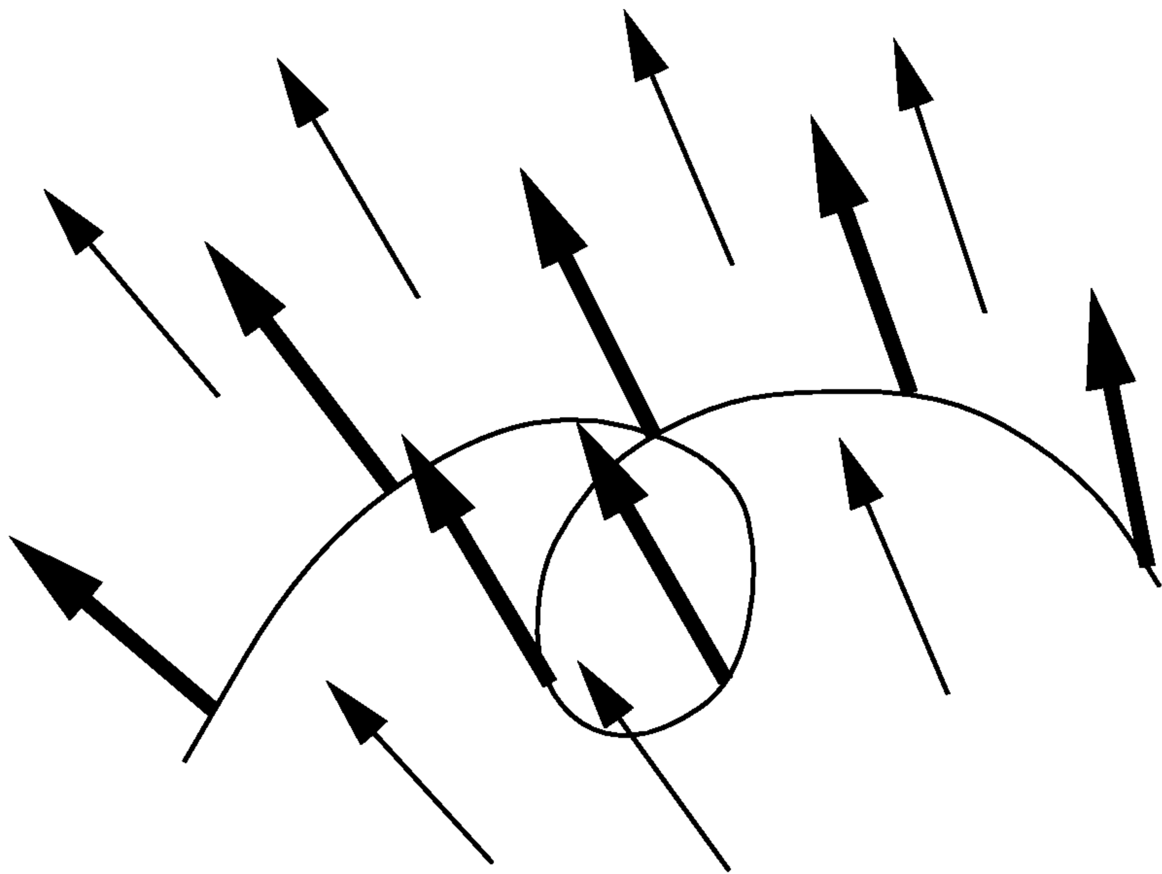
FIGURE 4.4. Extendible vector field.
