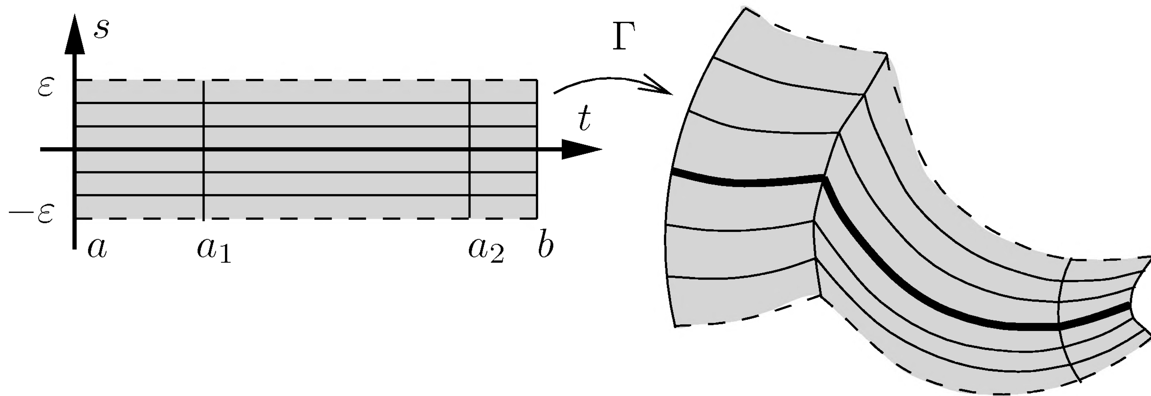
FIGURE 6.4. An admissible family.
