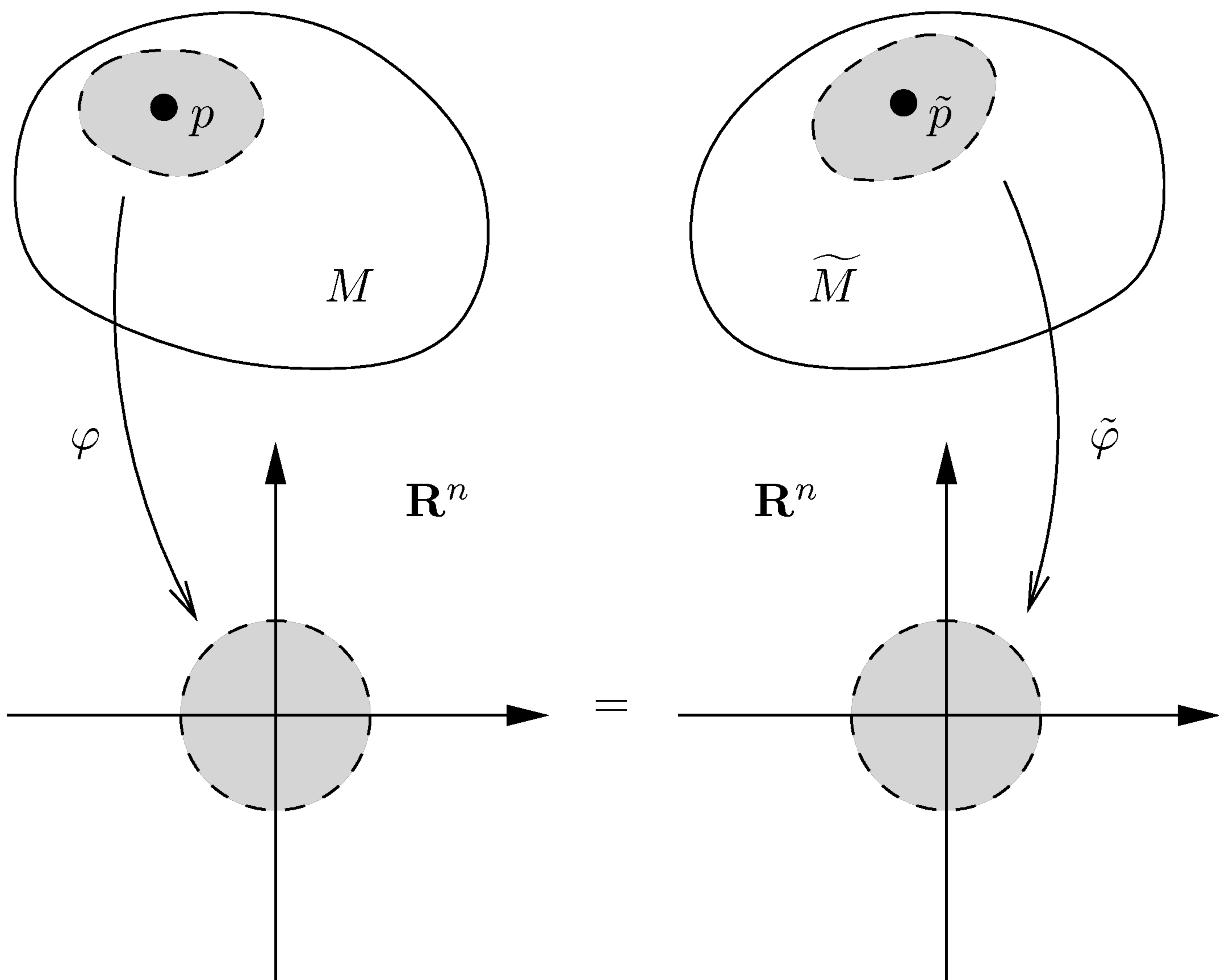
FIGURE 10.6. Local isometry constructed from normal coordinate charts.
