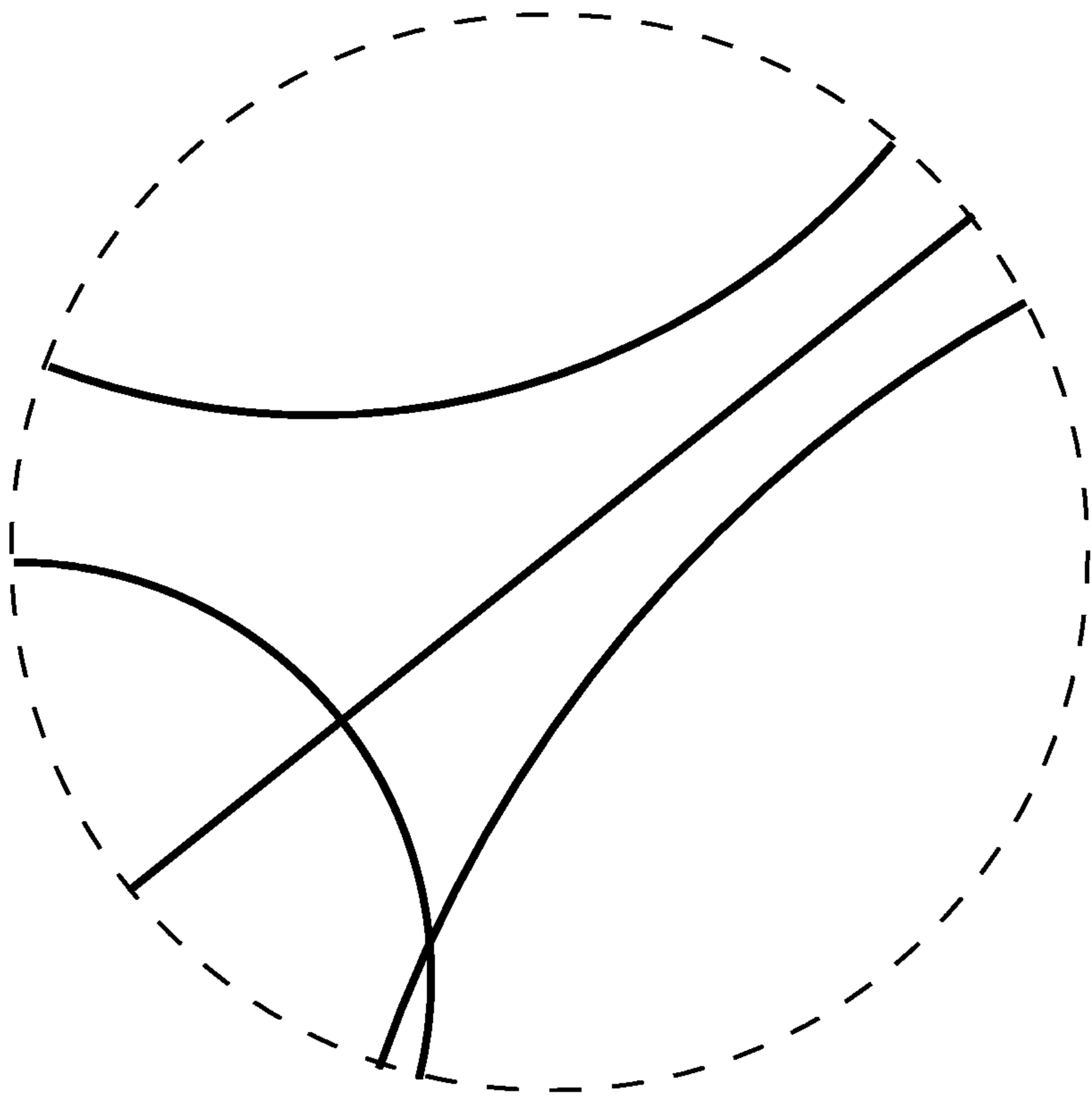
FIGURE 5.8. Geodesics of the Poincaré ball.
