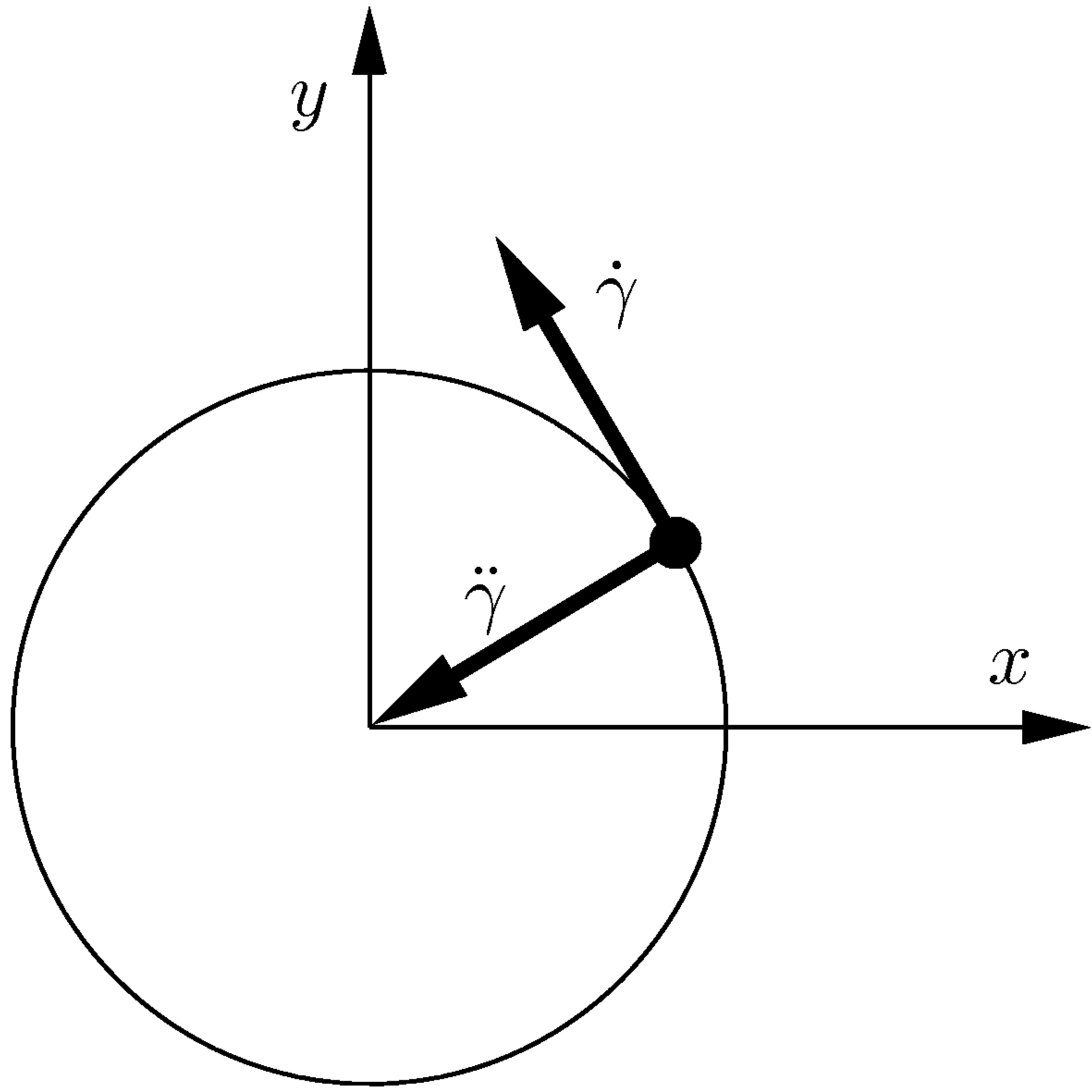
FIGURE 4.1. Euclidean coordinates.
