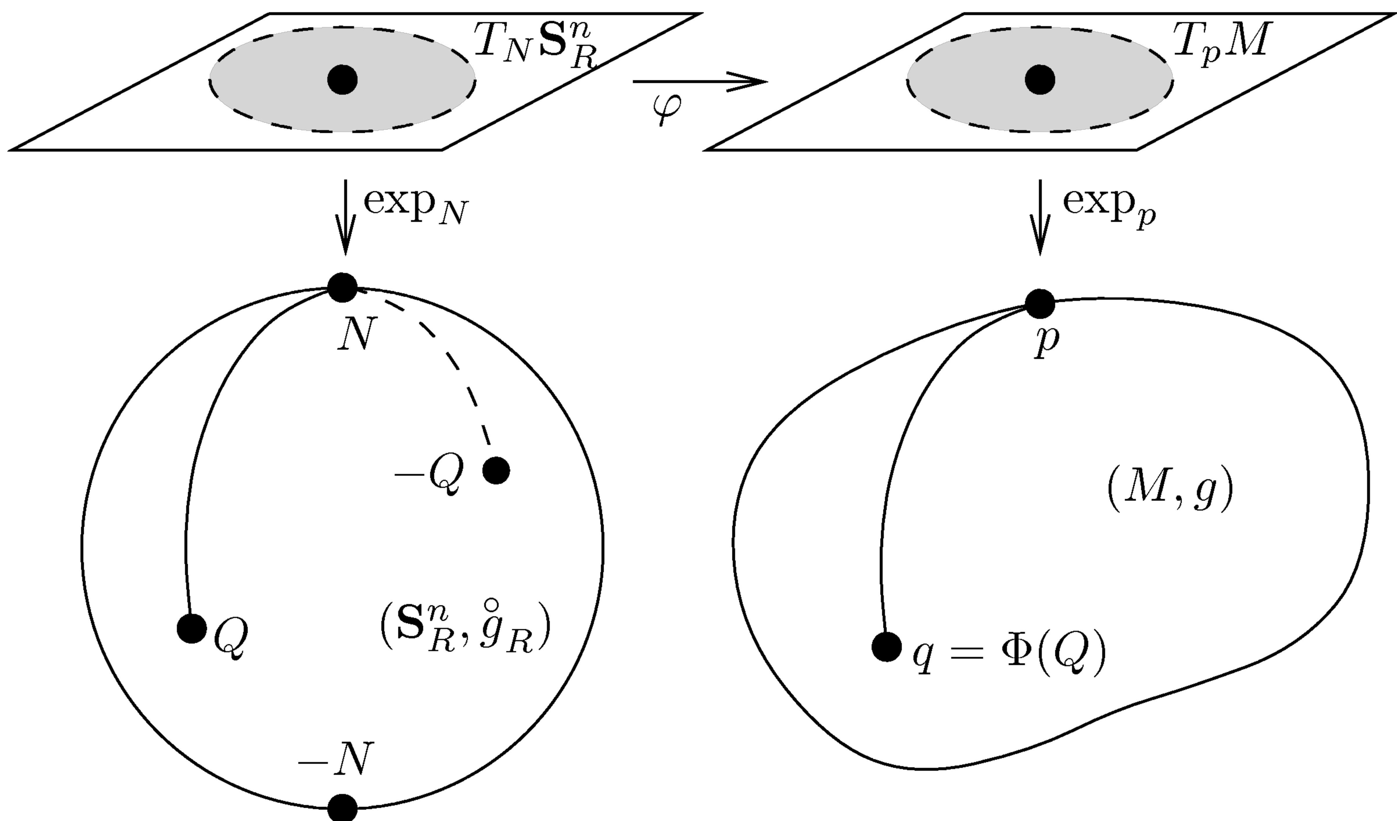
FIGURE 11.6. Constructing an isometry when C > 0 .
