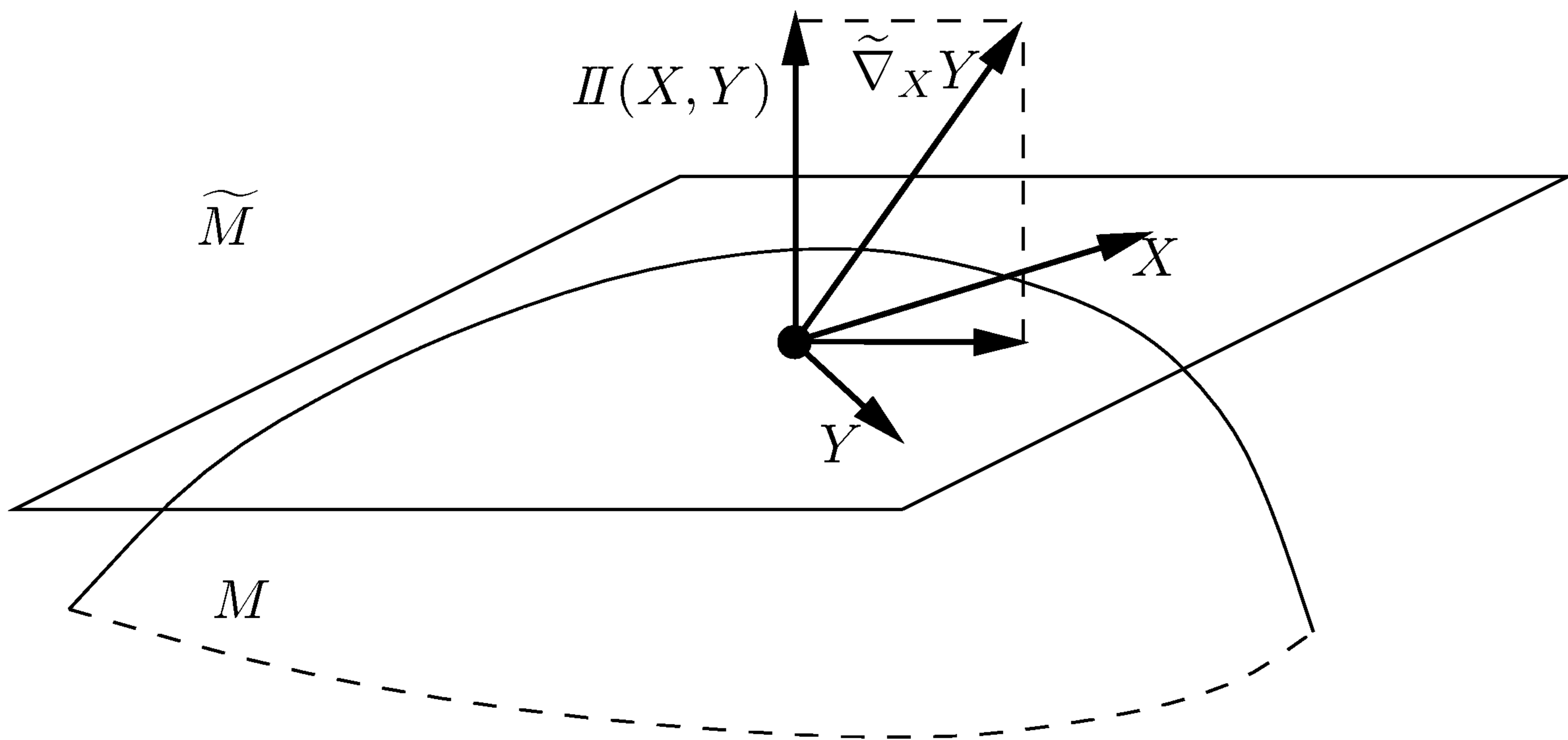
FIGURE 8.2. The second fundamental form.
