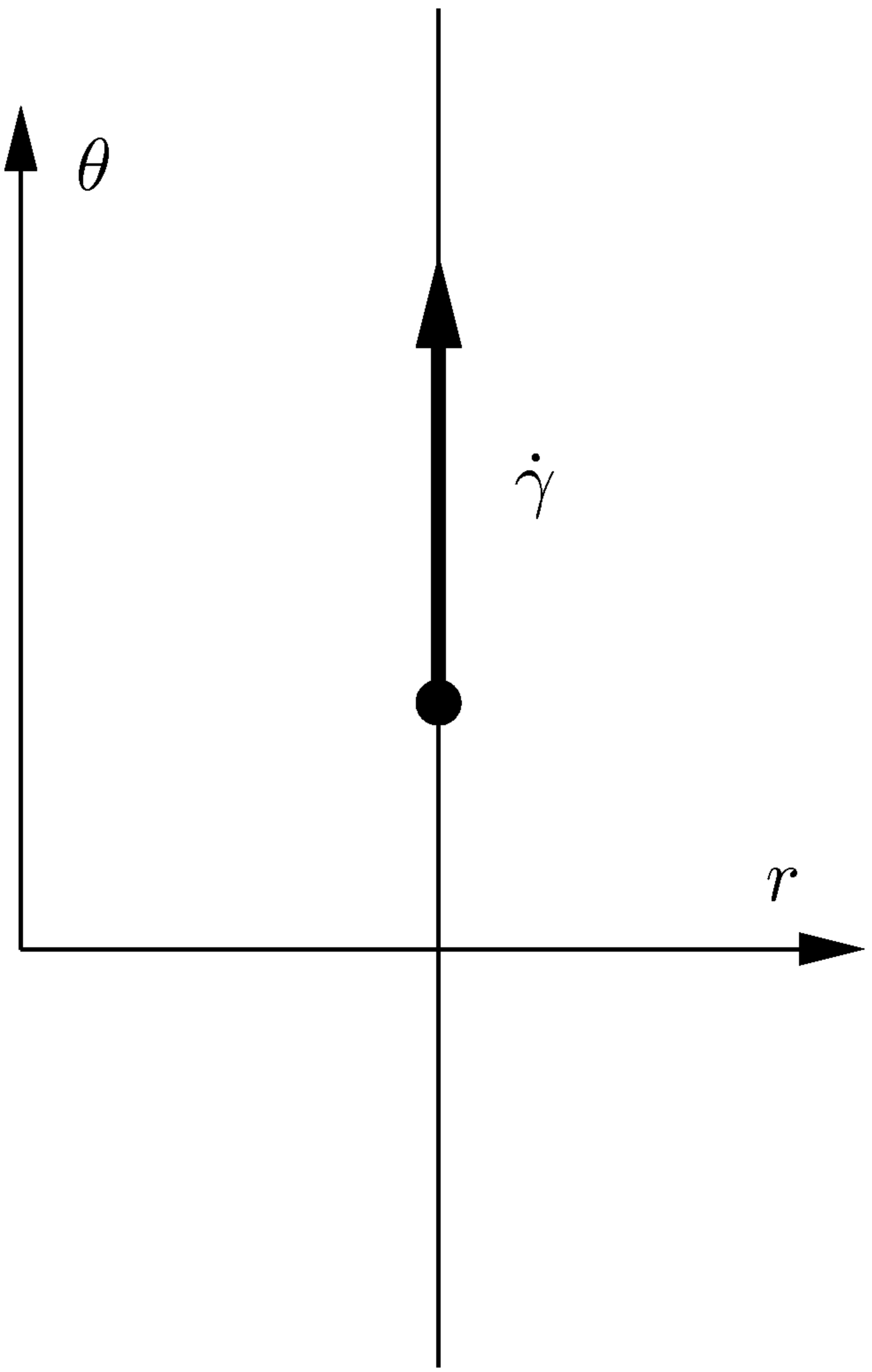
FIGURE 4.2. Polar coordinates.
