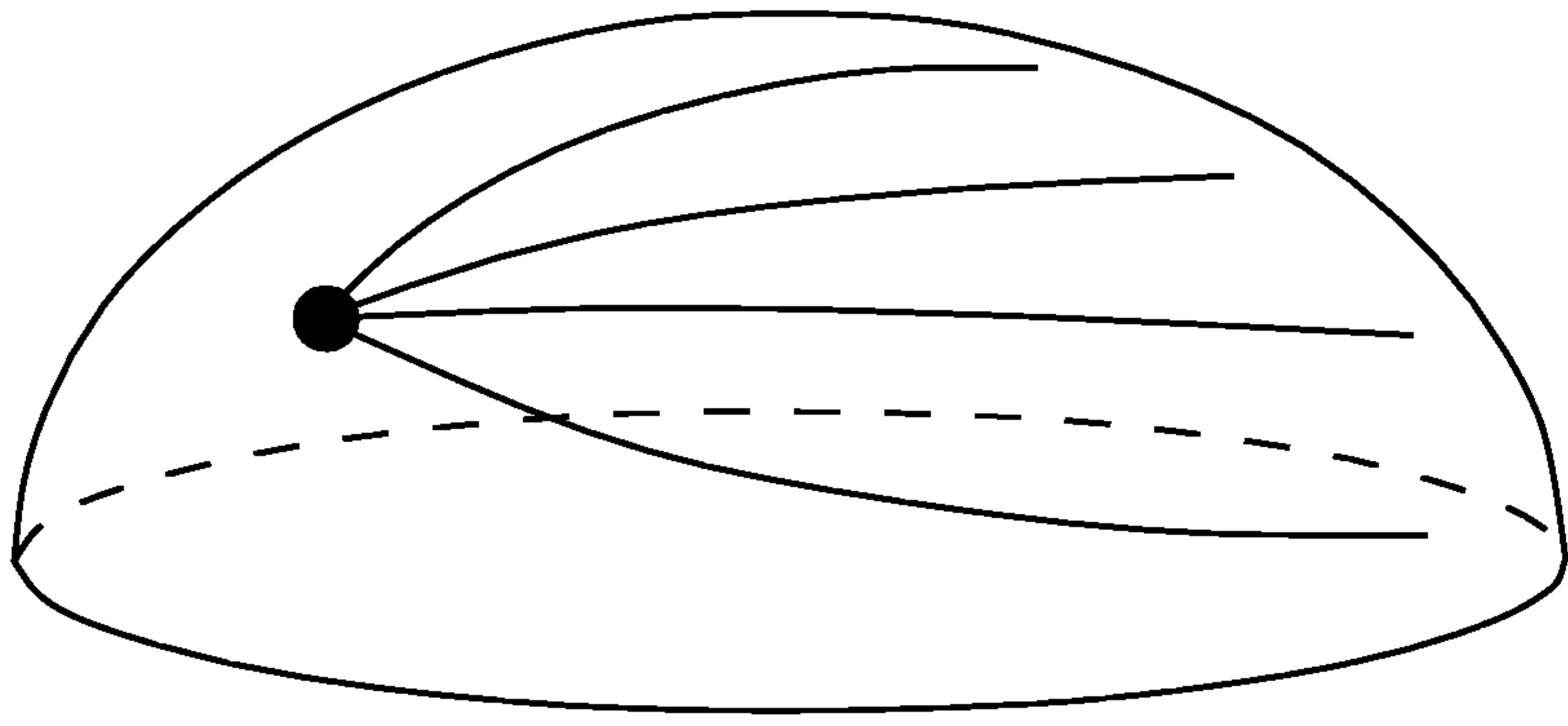
FIGURE 10.1. Positive curvature causes geodesics to converge.
