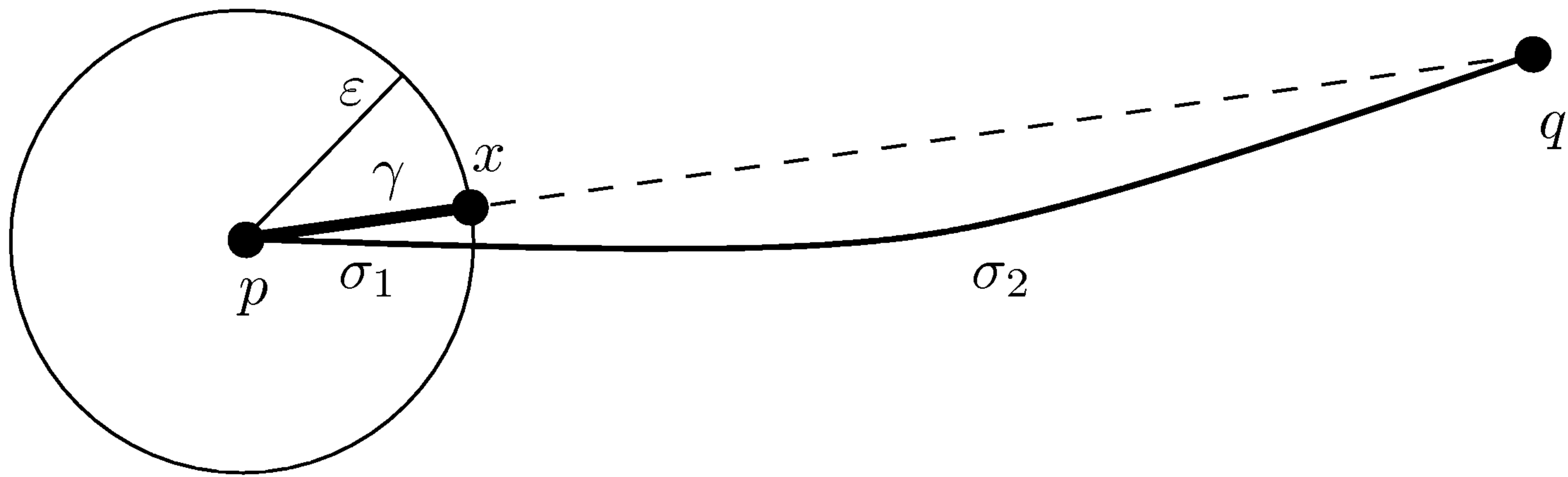
FIGURE 6.15. Proof that \gamma|_{[0,\varepsilon]} aims at q .
