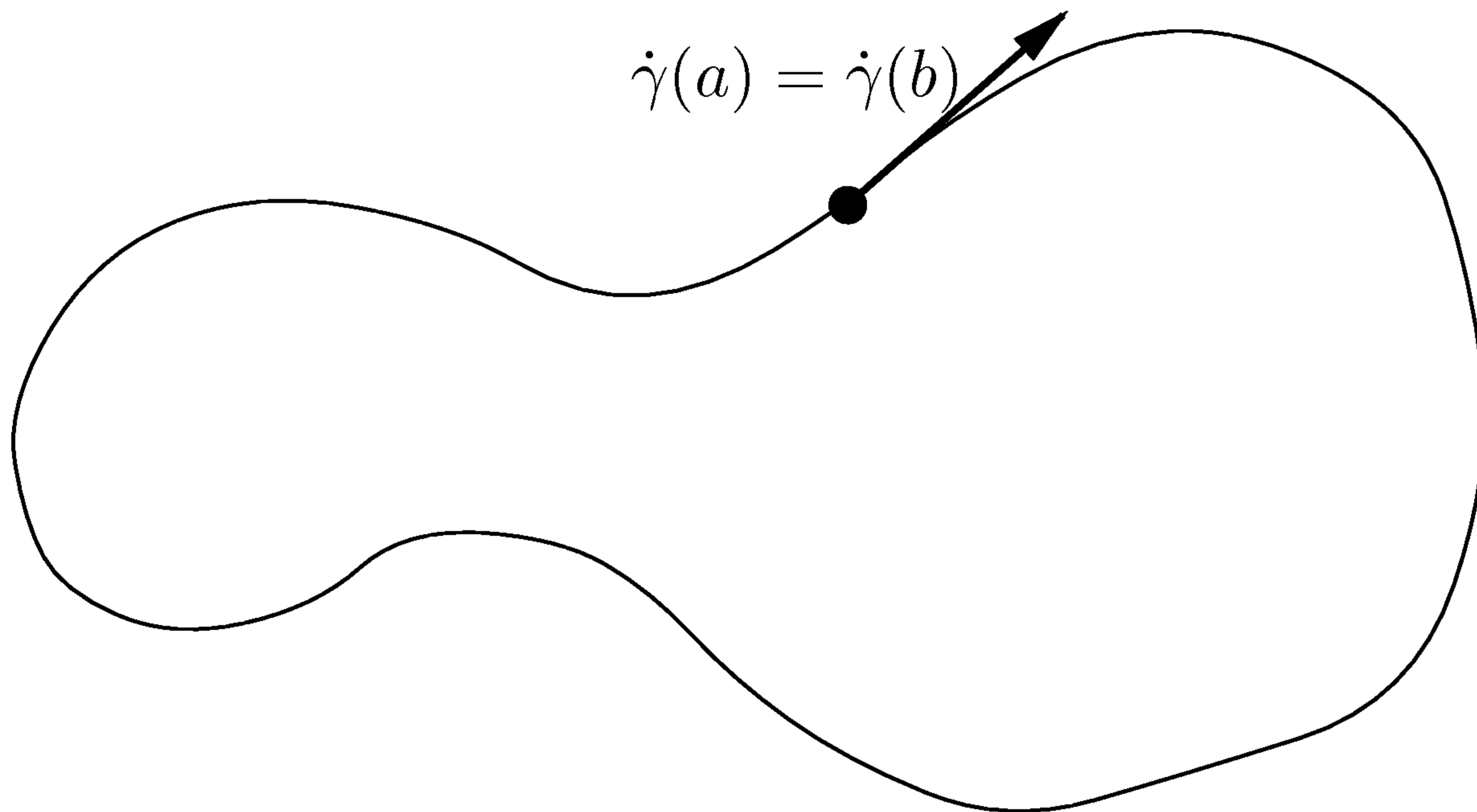
FIGURE 9.1. A closed curve with \dot{\gamma}(a) = \dot{\gamma}(b) .
