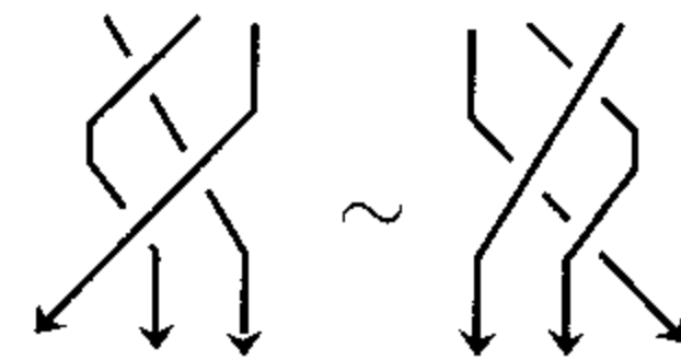
Figure 2.6. Relation (2.5)
