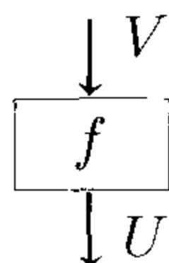
Figure 1.1. A morphism f : U \rightarrow \mathbf{V}
