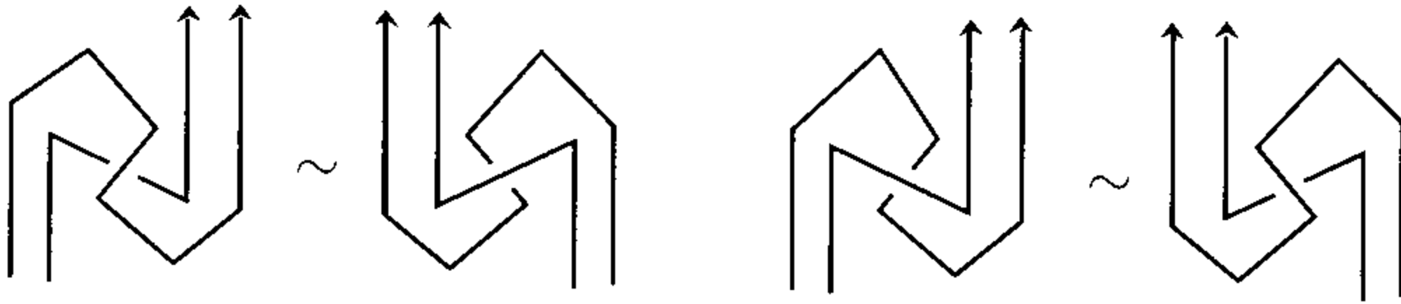
Figure 2.4. Relation, (2.3)
