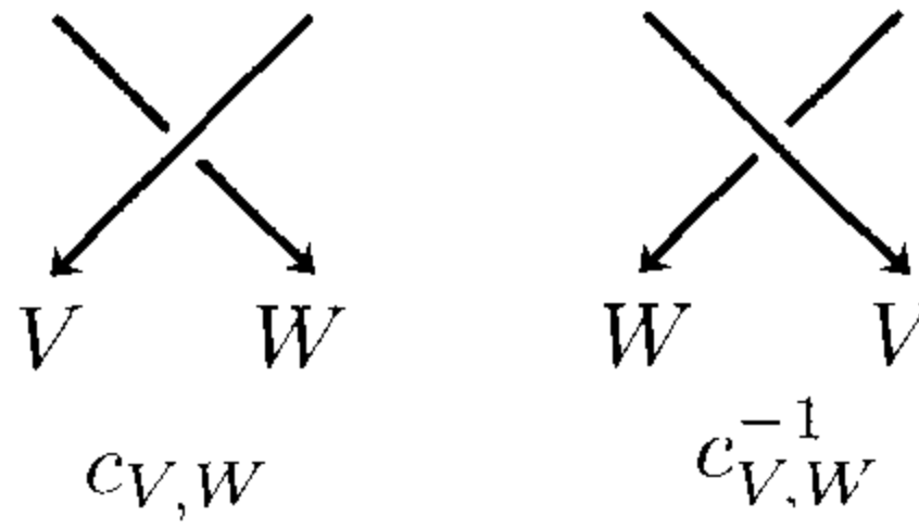
Figure 1.7. c_{V,W} and its inverse
