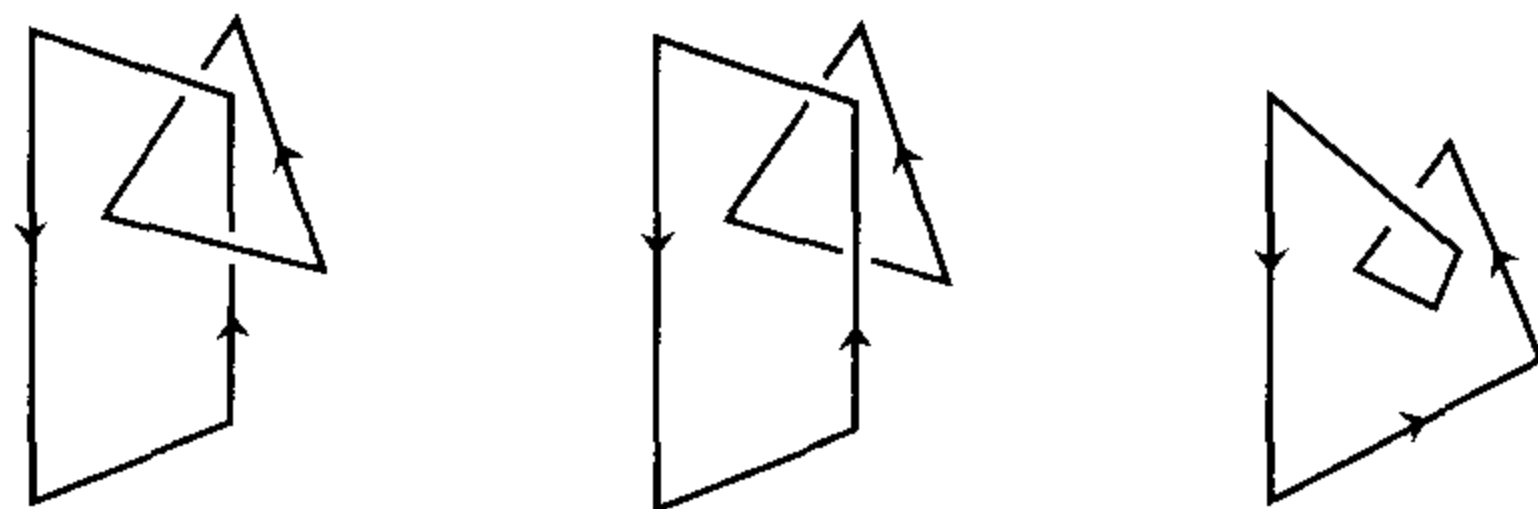
Figure 4.3.
