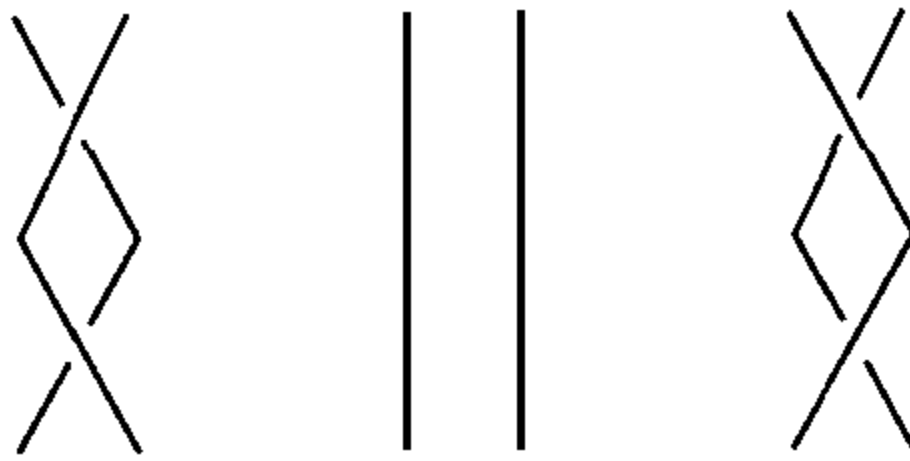
Figure 3.3. Reidemeister move (II)
