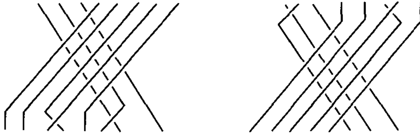
Figure 2.2.
