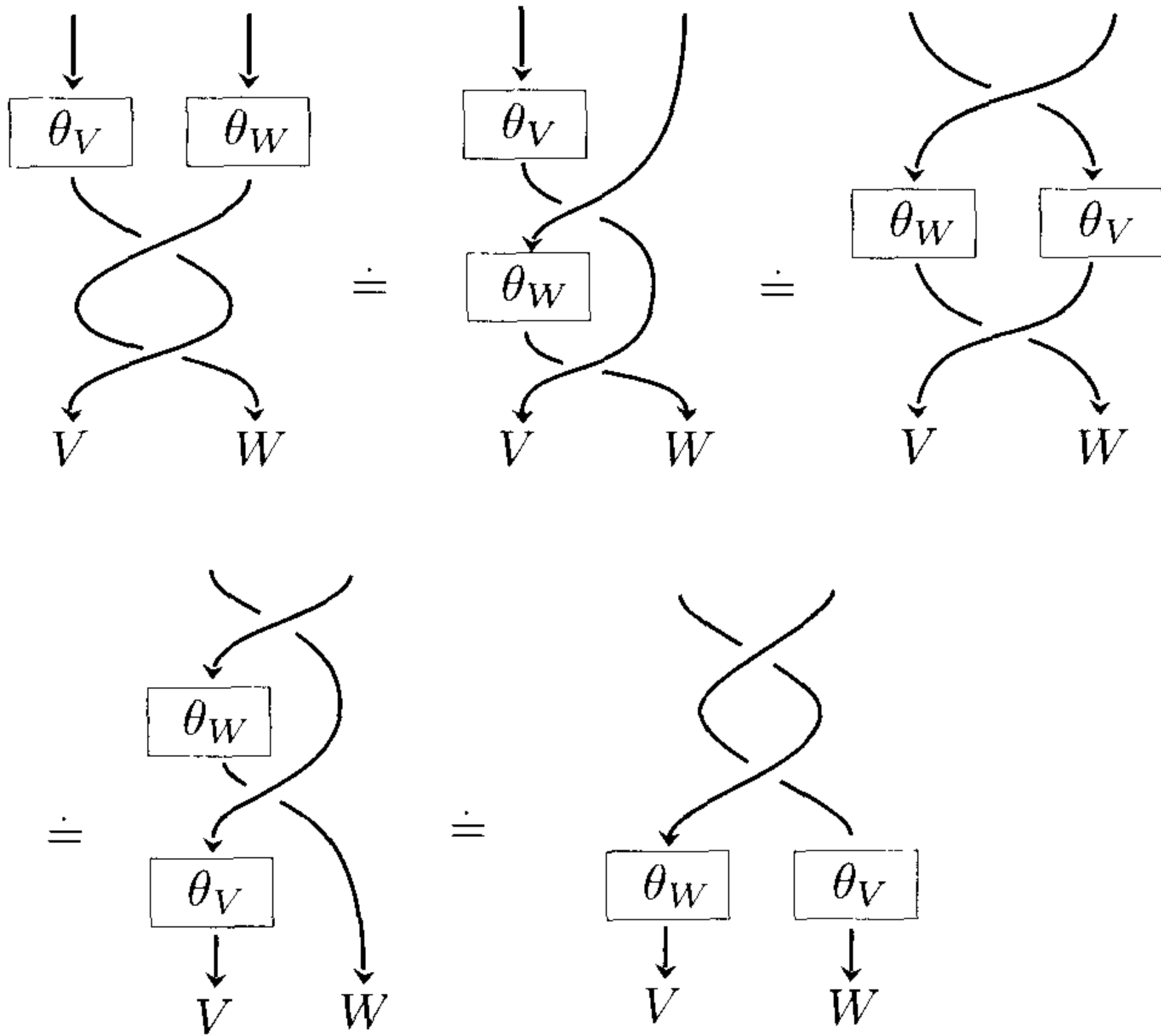
Figure 3.6. Proof of Lemma 3.3 (a)
