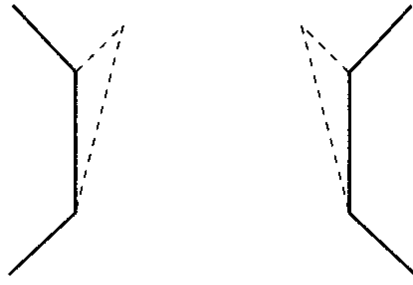
Figure 3.5. (0 projected)
