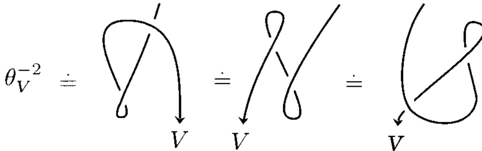
Figure 3.8. The equalities of Lemma 3.4
