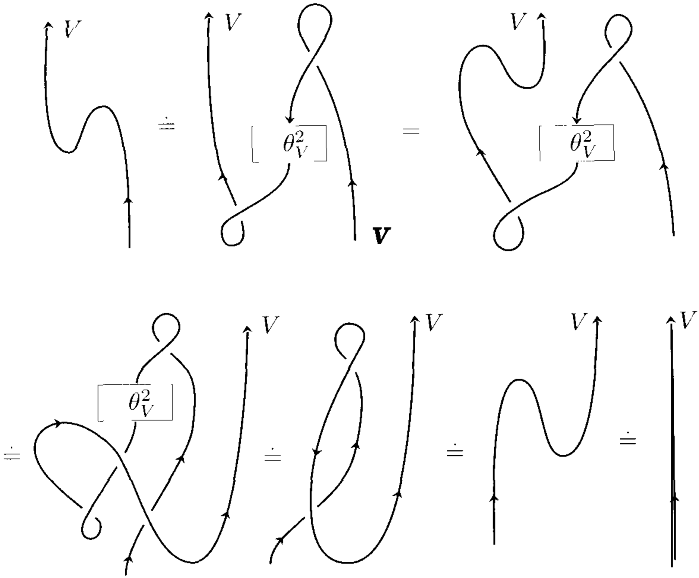
Figure 3.10. Proof of Relation (3.8)
