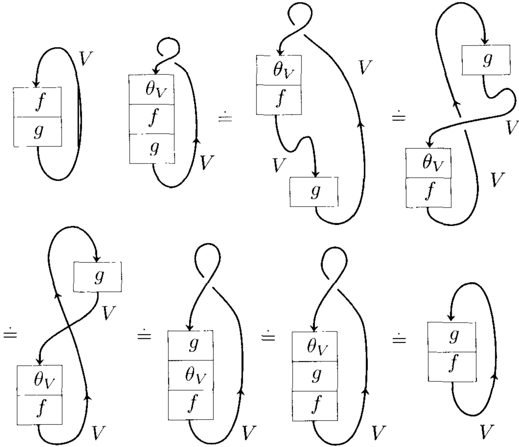
Figure 4.2. The proof of \text{tr}_q(fg) = \text{tr}_q(gf)
