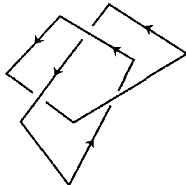
Figure 2.1. A right-handed trefoil knot
