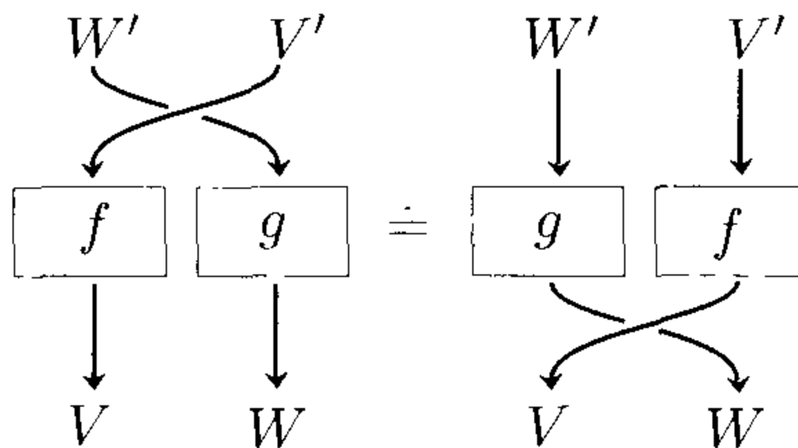
Figure 1.9. Naturality of c_{V,W}
