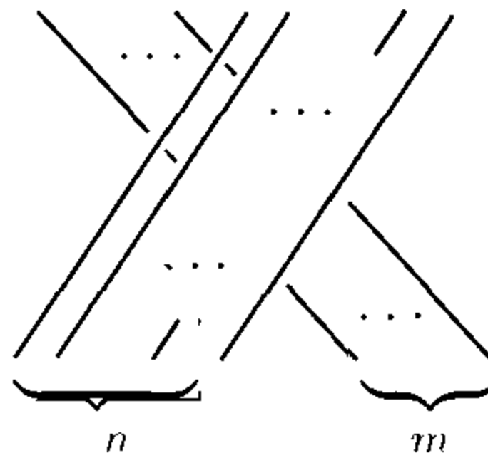
Figure 2.1. The braid c_{n,m}
