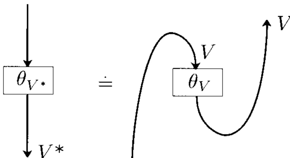
Figure 3.5. Relation (3.2)
