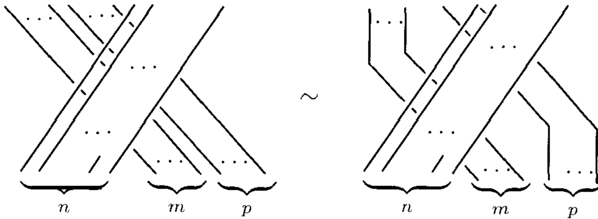
Figure 2.3. Proof of Relation 1.5
