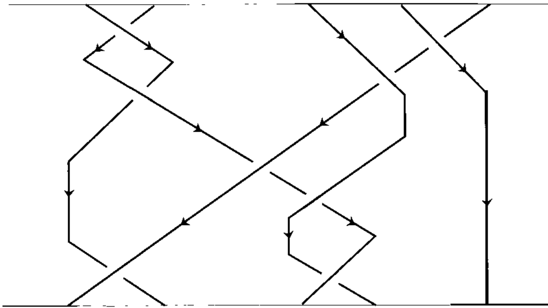
Figure 6.1. A braid
