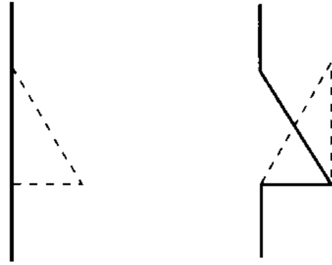
Figure 3.6. (I projected)
