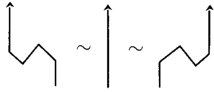
Figure 2.3. Relation (2.2)
