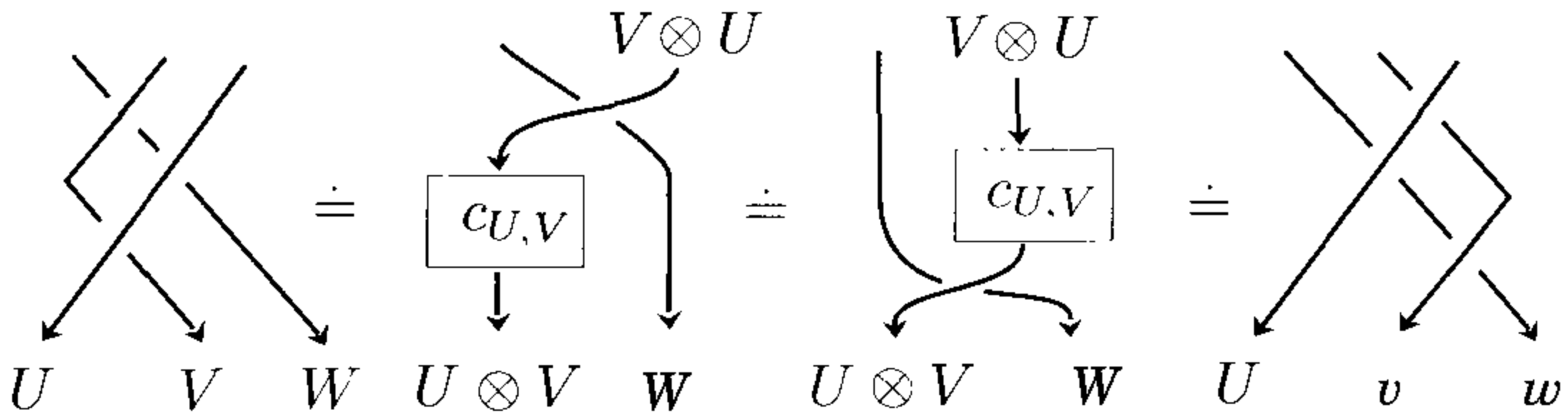
Figure 1.11. Proof of Theorem X111.1.3
