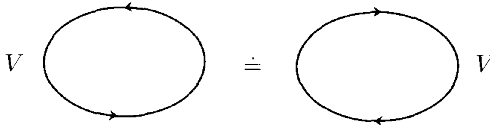
Figure 4.5. The quantum dimension of V
