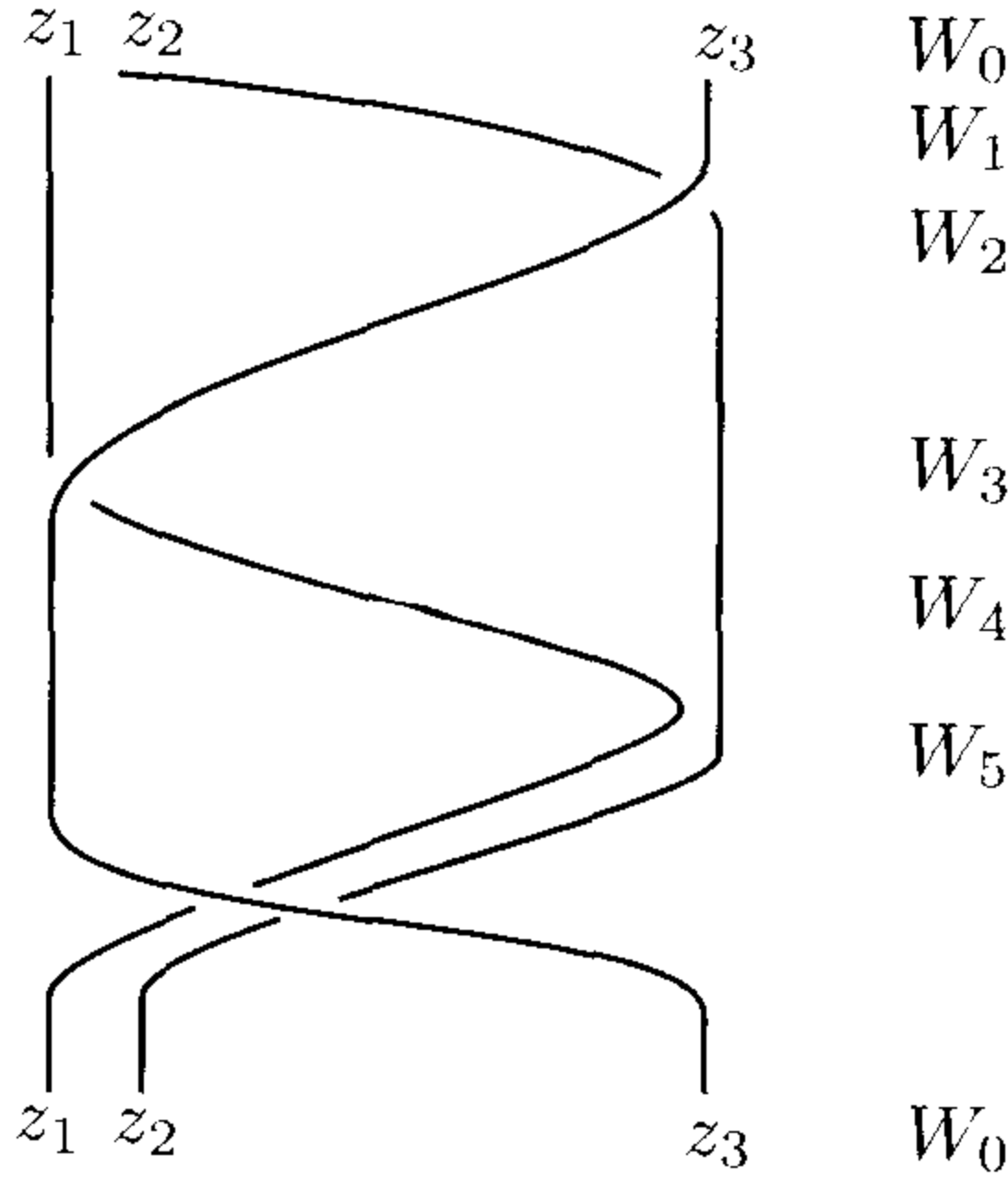
Figure 8.1. The movements of z_1, z_2, and z_3
