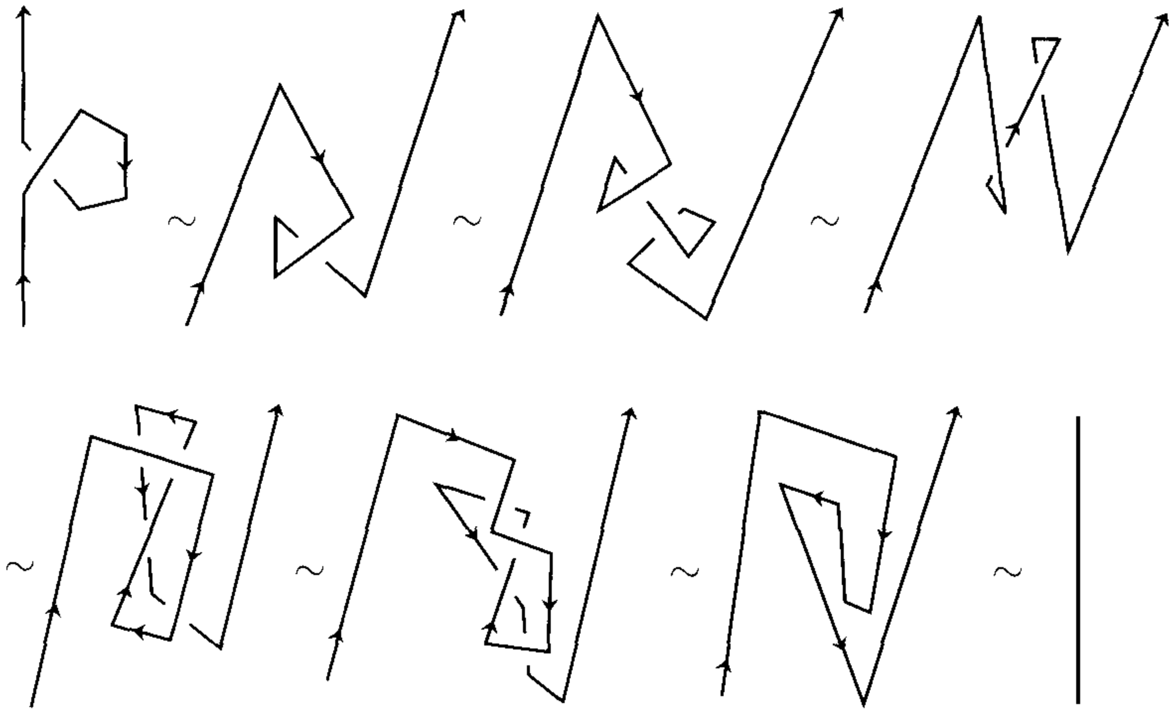
Figure 3.4. Proof for Transformation (I) “upwards”
