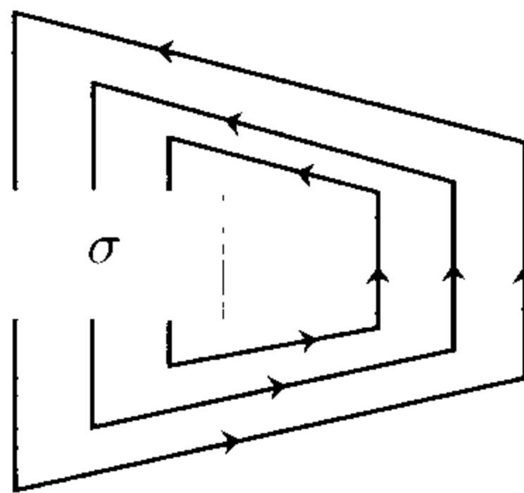
Figure 8.4. Closure of a braid
