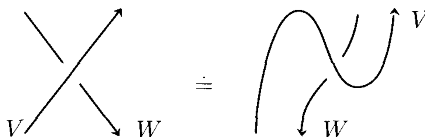
Figure 3.2. The equality of Proposition 3.1
