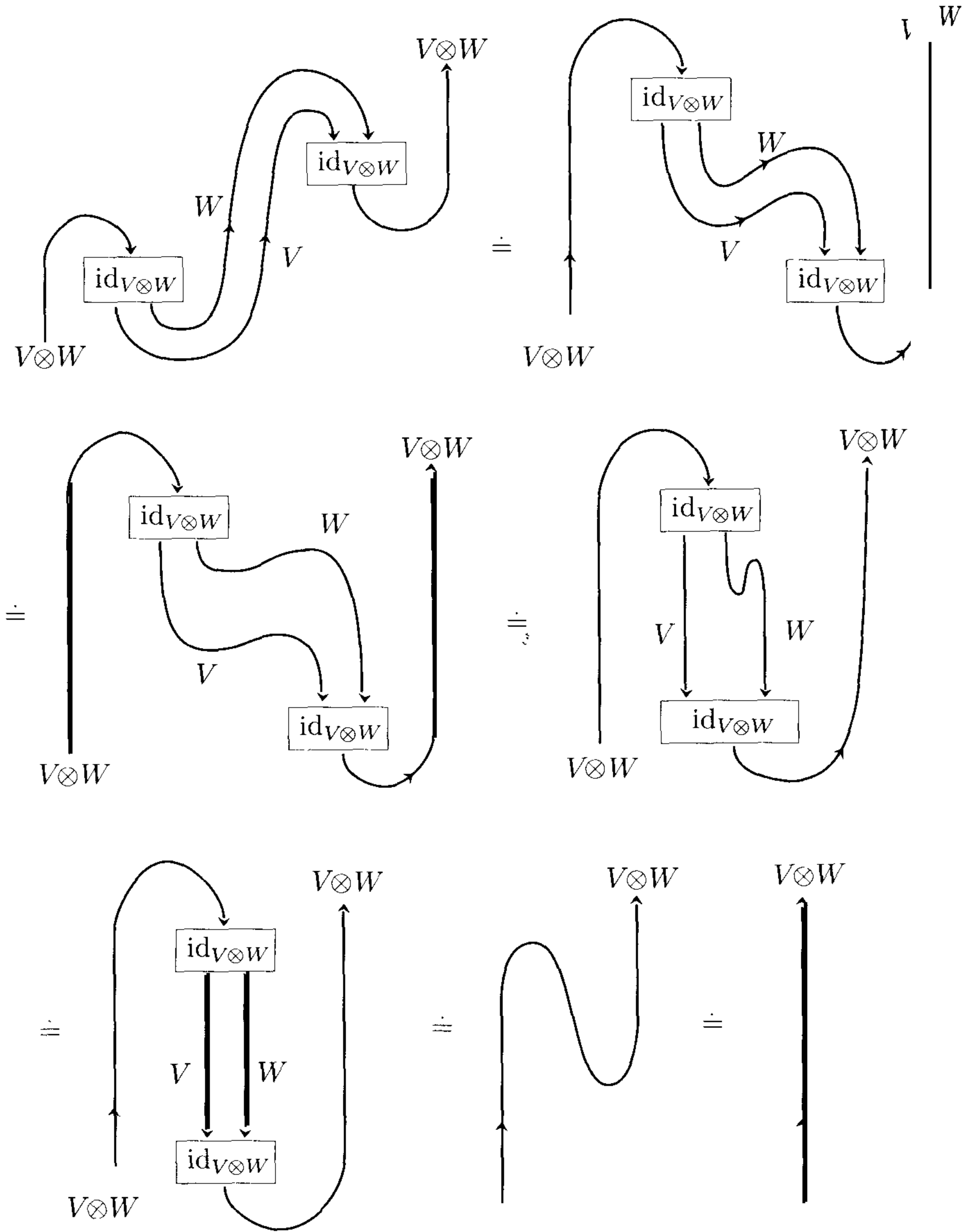
Figure 2.7. Proof of \lambda_{V,W} \circ \lambda_{V,W}^{-1} = \text{id}_{(V \otimes W)^*}
