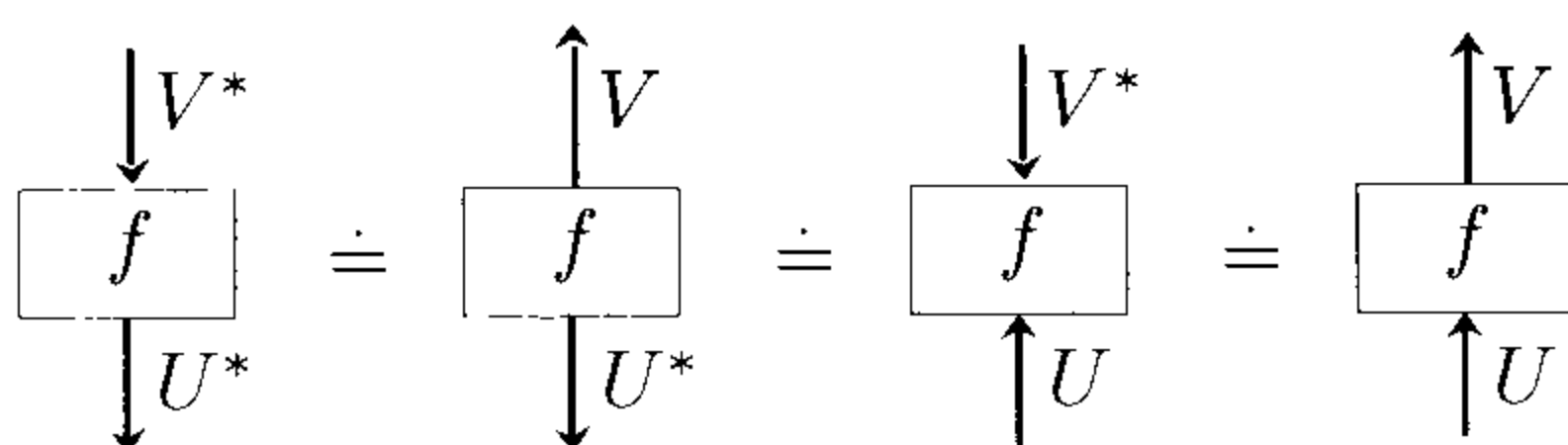
Figure 2.1. A morphism f:U^* \rightarrow V^*
