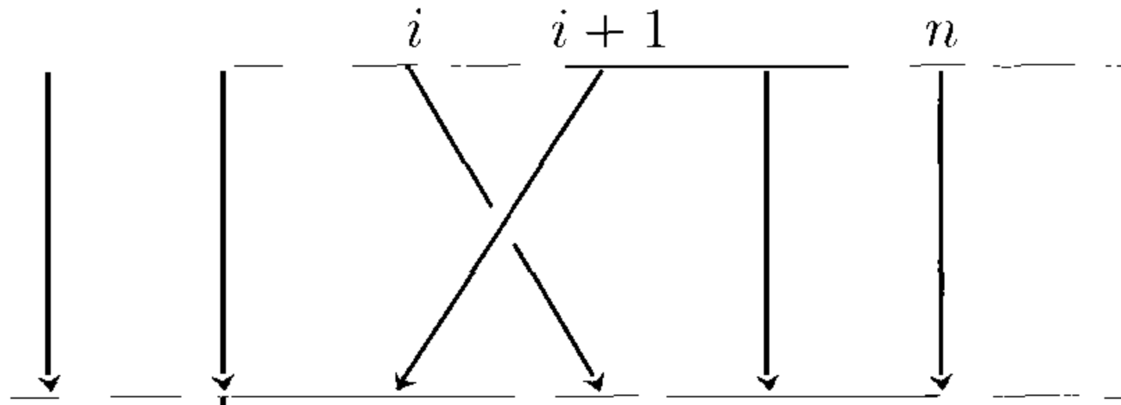
Figure 6.2. The braid \sigma_i
