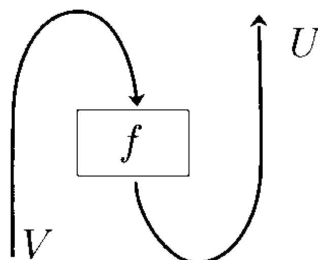
Figure 2.4. The transpose f^*
