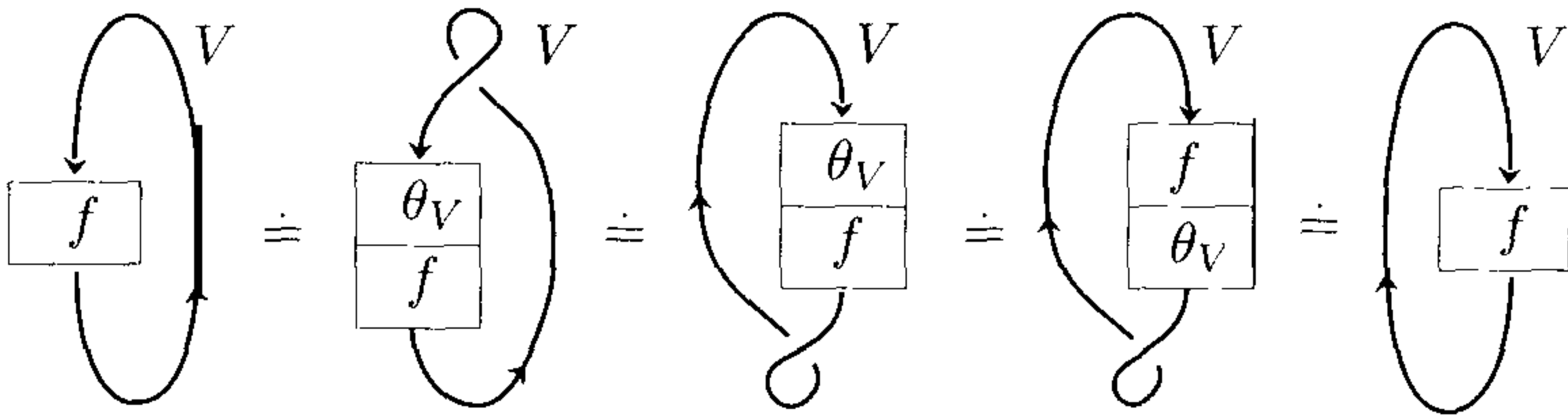
Figure 4.1. The quantum trace of f
