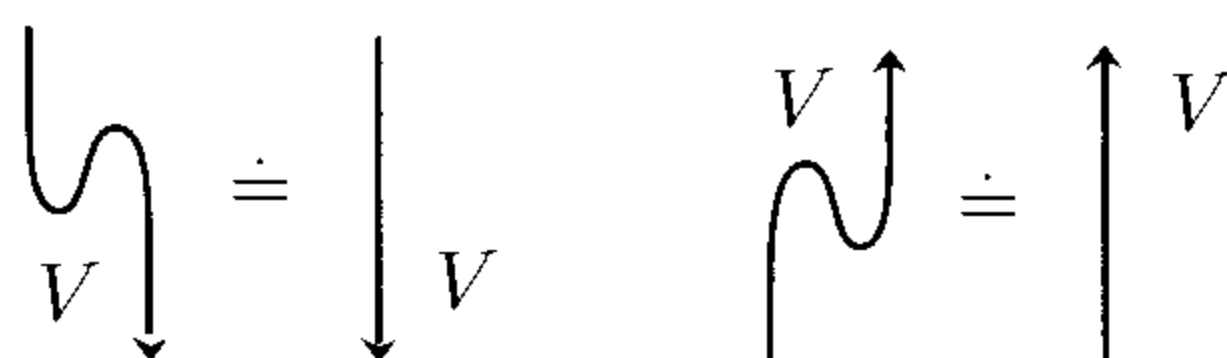
Figure 2.3. Relations (2.1)
