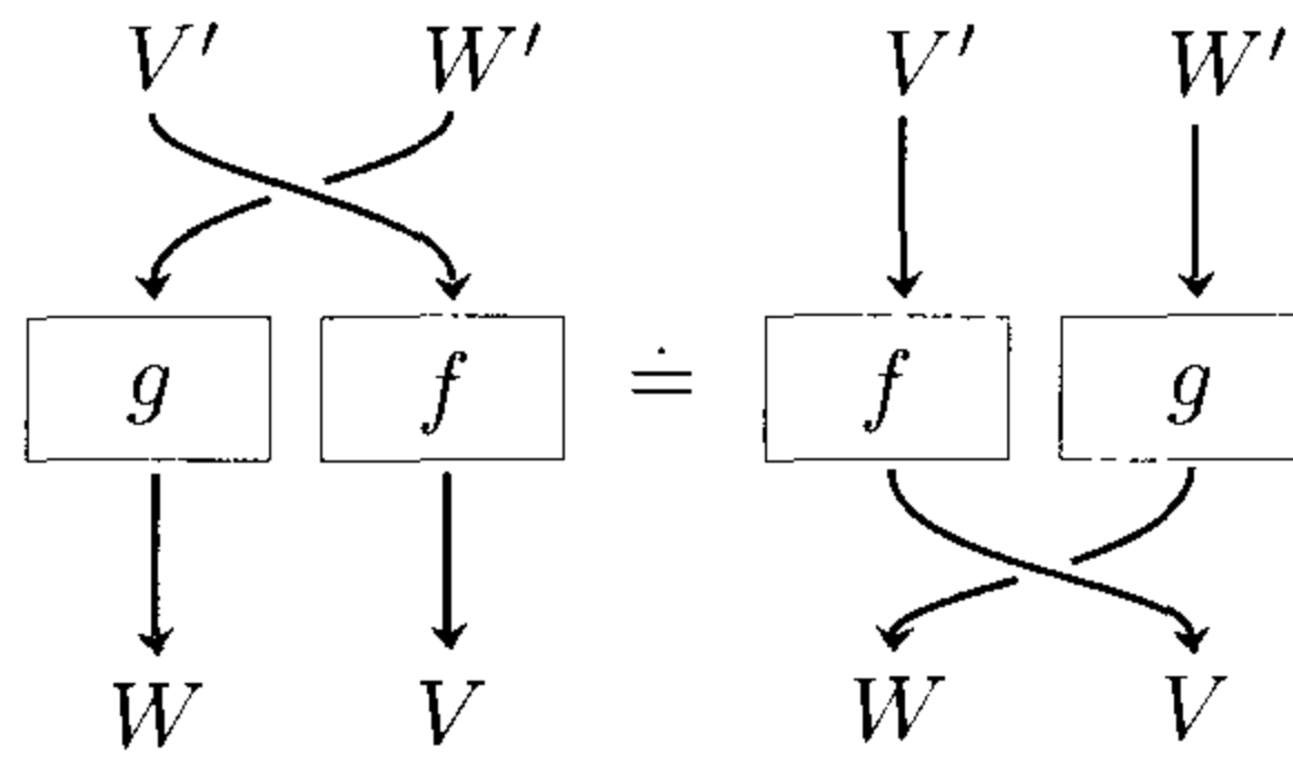
Figure 1.10. Naturality of c_{V,W}^{-1}
