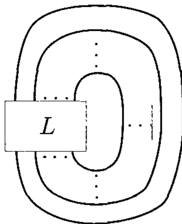
Figure 5.2. The quantum trace \text{tr}_q(L)
