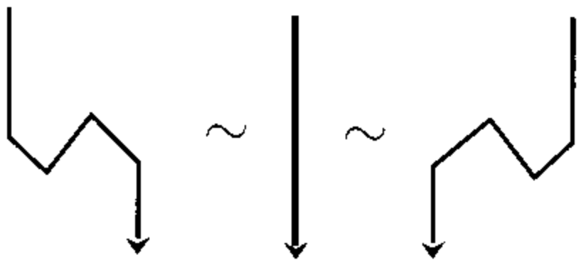
Figure 2.2. Relation (2.1)
