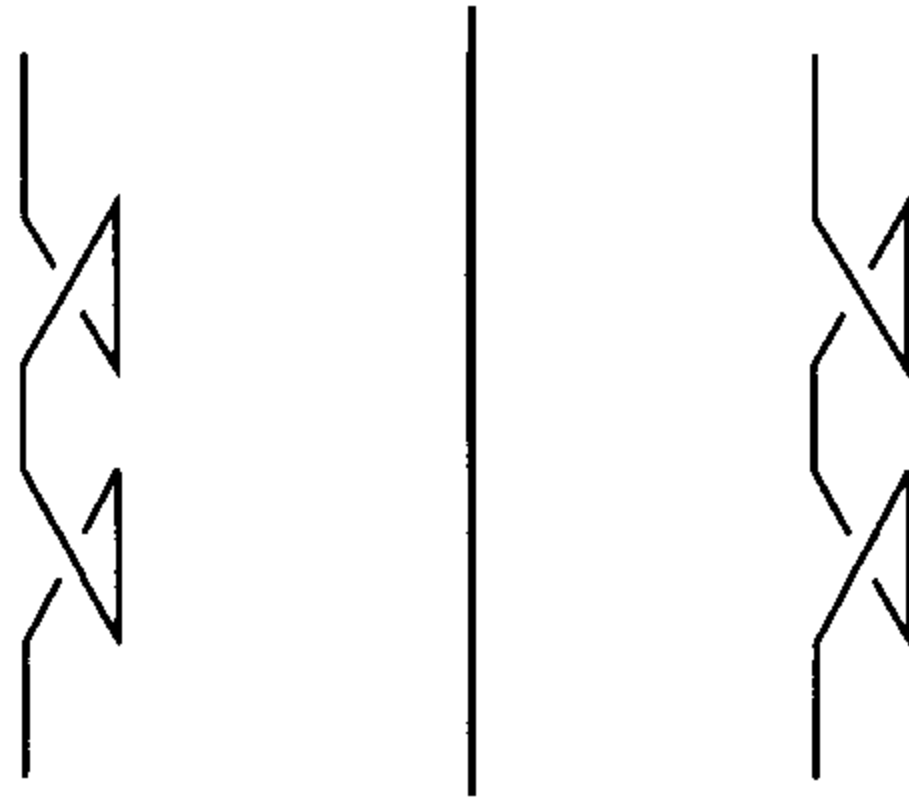
Figure 8.3. Reidemeister move (I)
