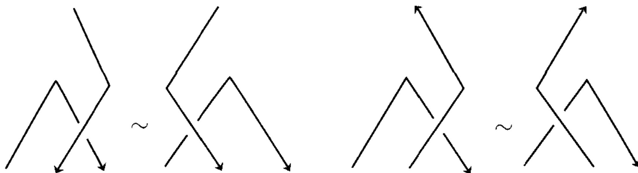
Figure 3.9. An isotopy in the neighbourhood of a local maximum
