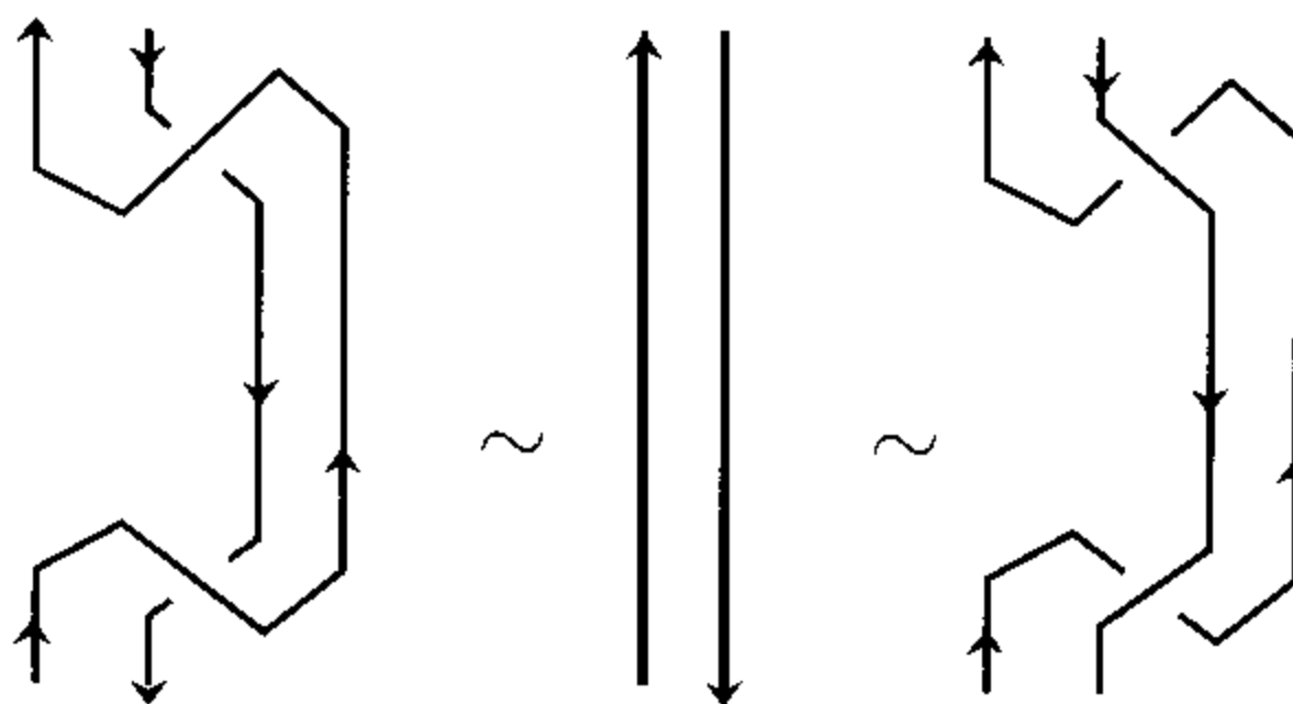
Figure 2.9. Relation (2.8)
