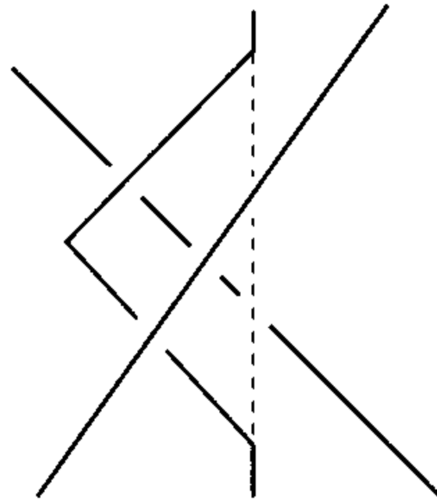
Figure 3.8. (III projected)
