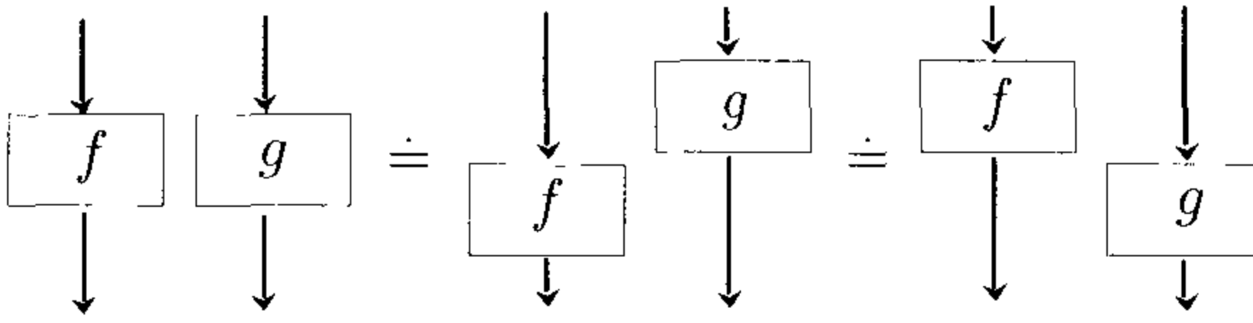
Figure 1.6. The identity (XI.2.3)
