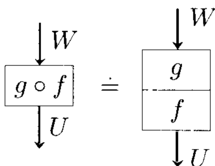
Figure 1.2. Composition of morphisms
