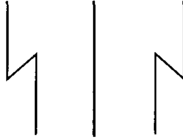
Figure 3.1. Reidemeister move (0)
