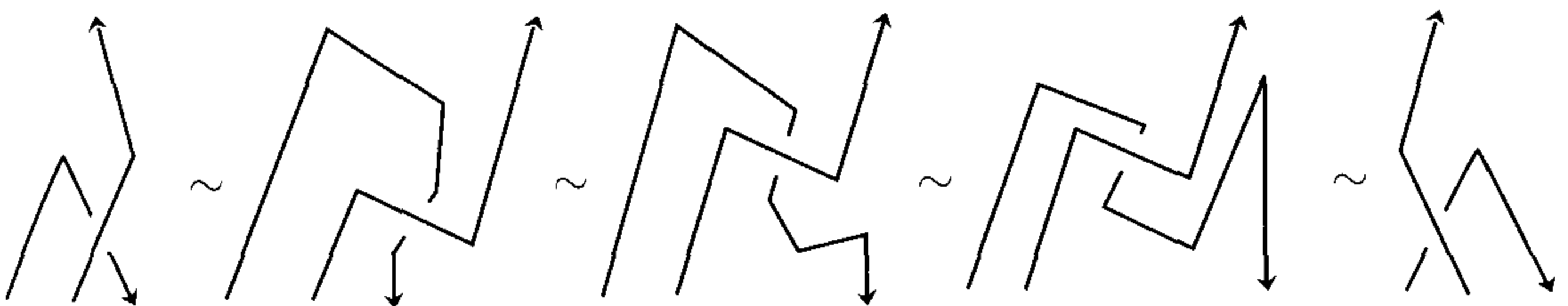
Figure 3.12.
