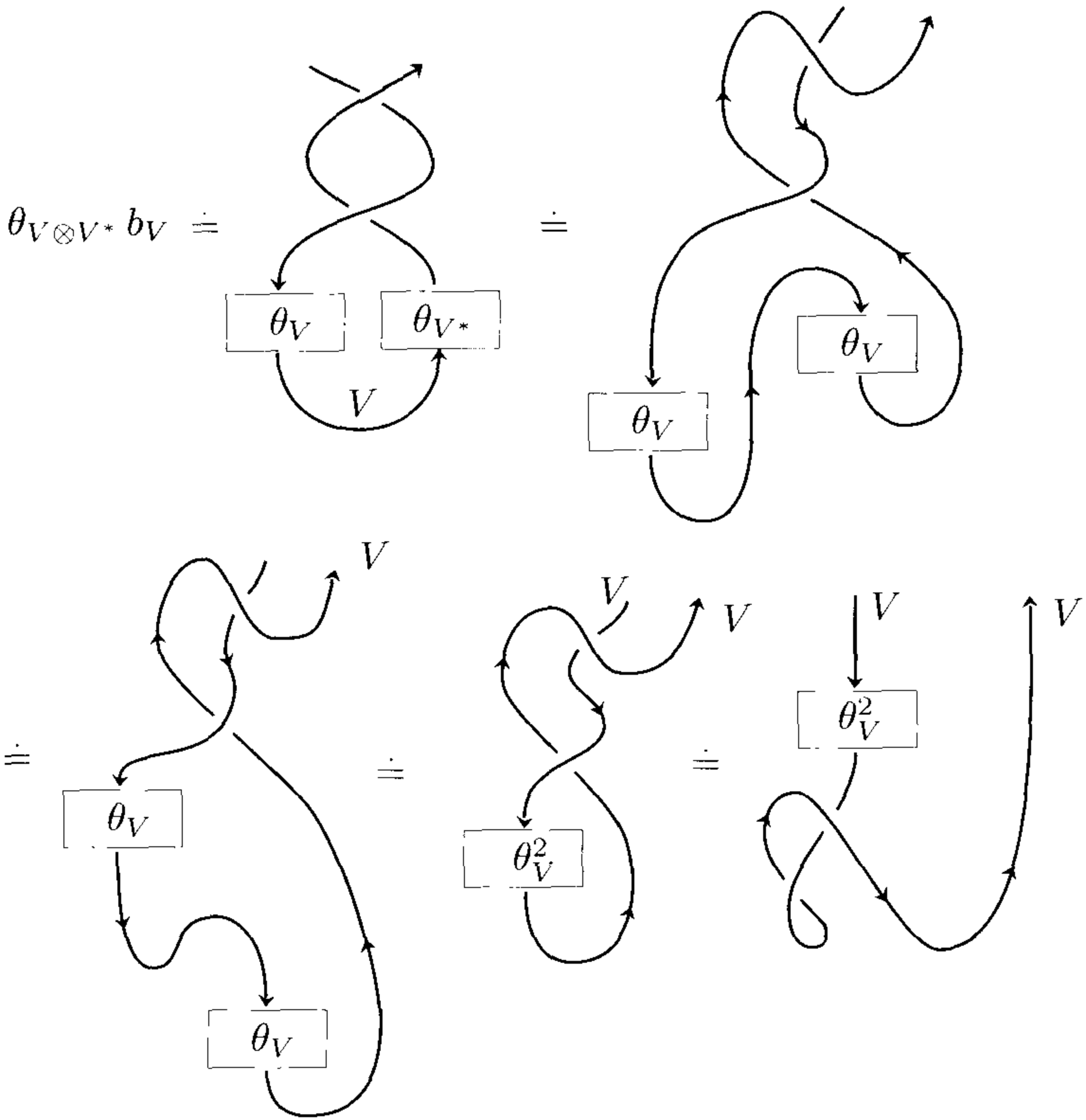
Figure 3.9. Proof of \theta_{V \otimes V^*} b_V = (\theta_V^2 f \otimes id_{V^*}) b_V
