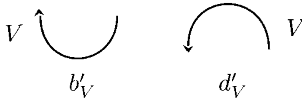
Figure 3.7. The morphisms b'_V and d'_V
