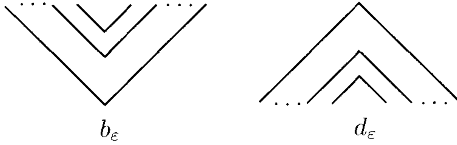
Figure 5.1. The framed tangles b_\varepsilon and d_\varepsilon
