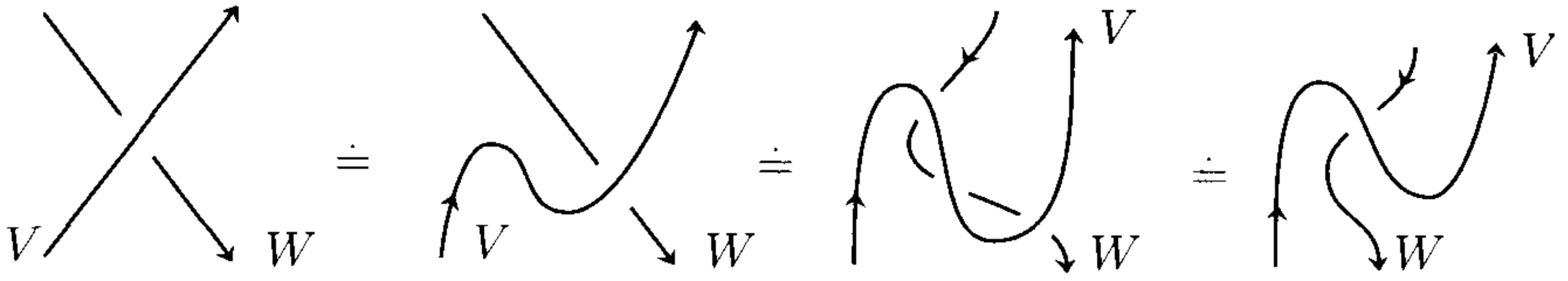
Figure 3.3. Proof of Proposition 3.1
