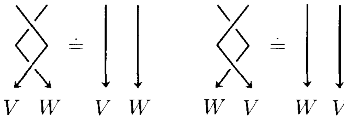
Figure 1.8. Invertibility of c_{V,W}
