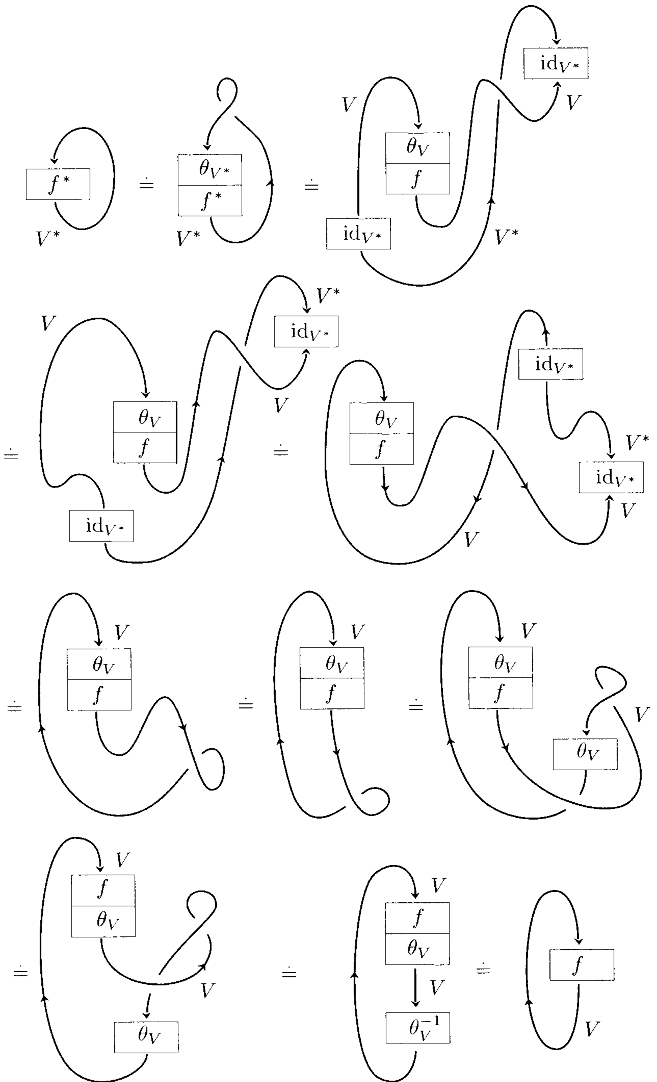
Figure 4.4. The proof of \text{tr}_q(f) = \text{tr}_q(f^*)
