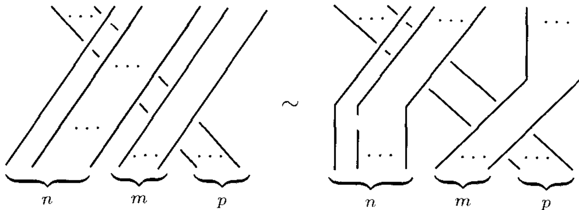
Figure 2.4. Proof of Relation 1.6
