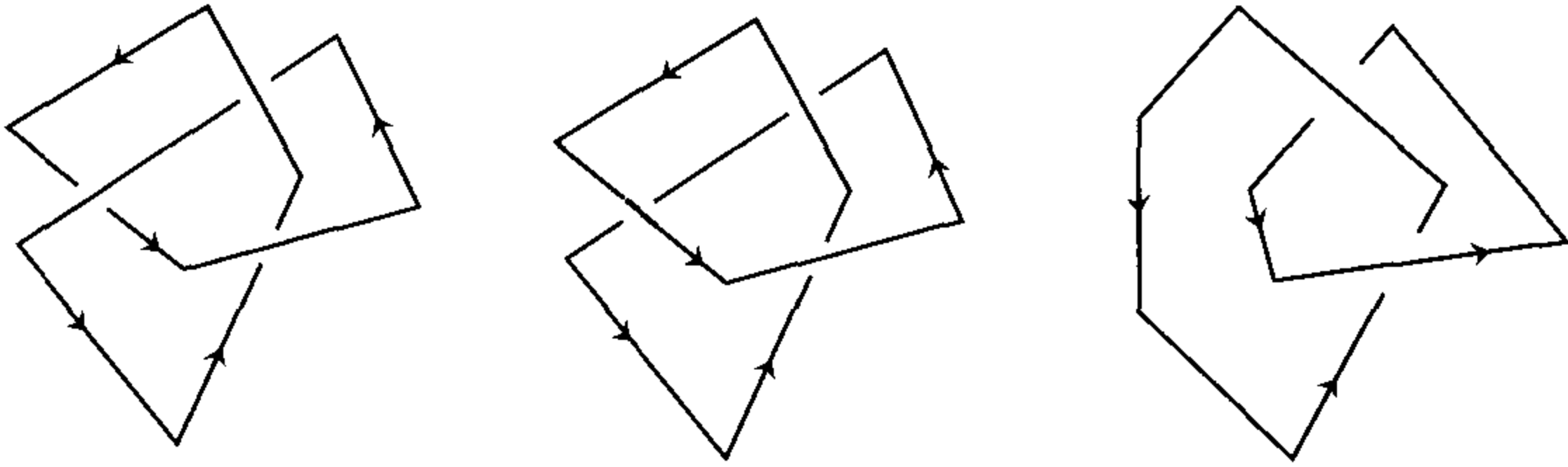
Figure 4.4.
