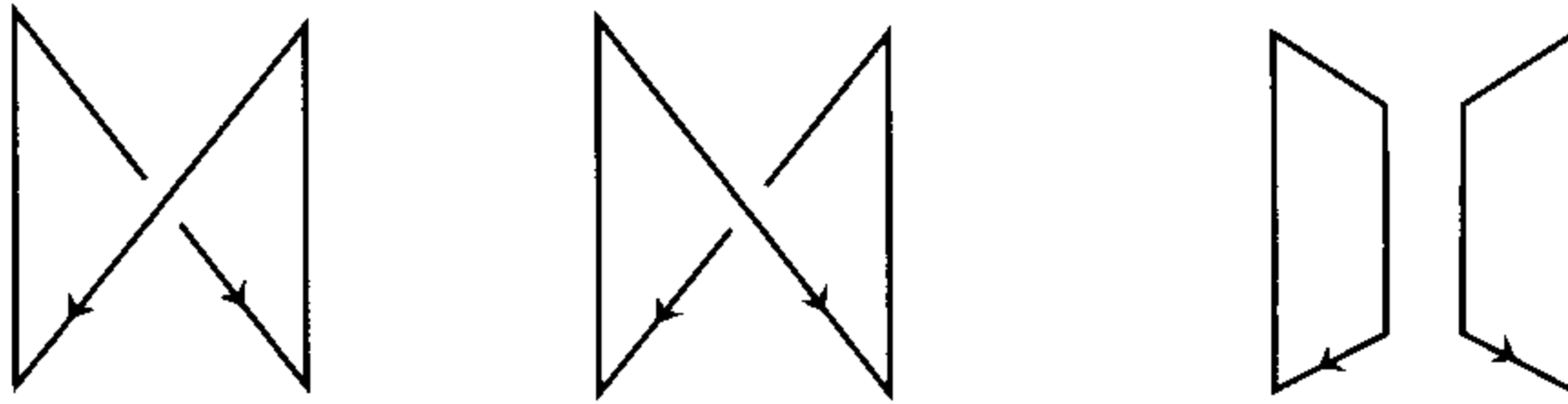
Figure 4.2. A Conway triple
