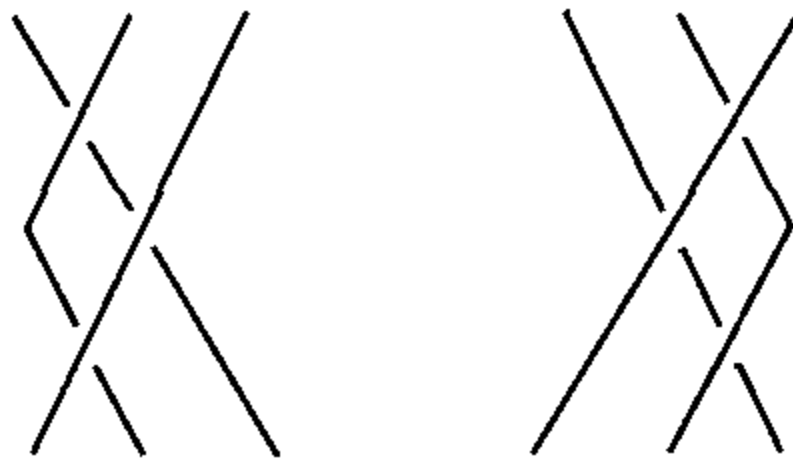
Figure 3.4. Reidemeister move (III)
