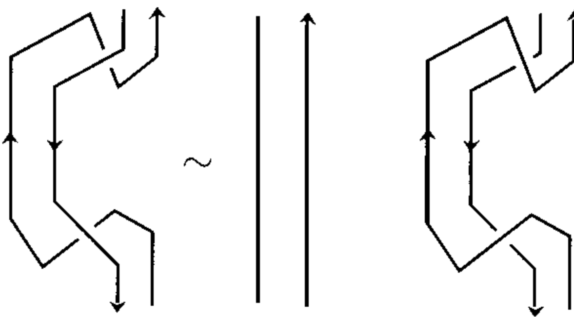
Figure 2.8. Relation (2.7)
