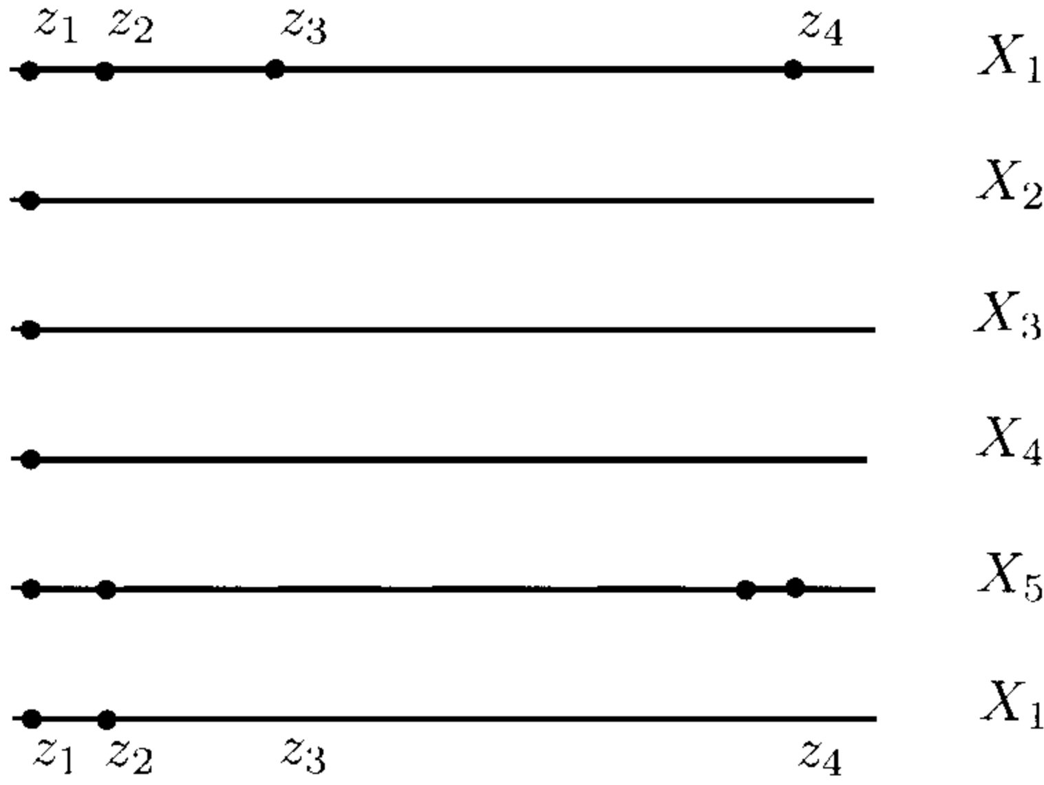
Figure 8.2. Five configurations of four particles
