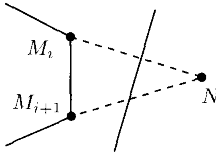
Figure 1.1. A n -operation
