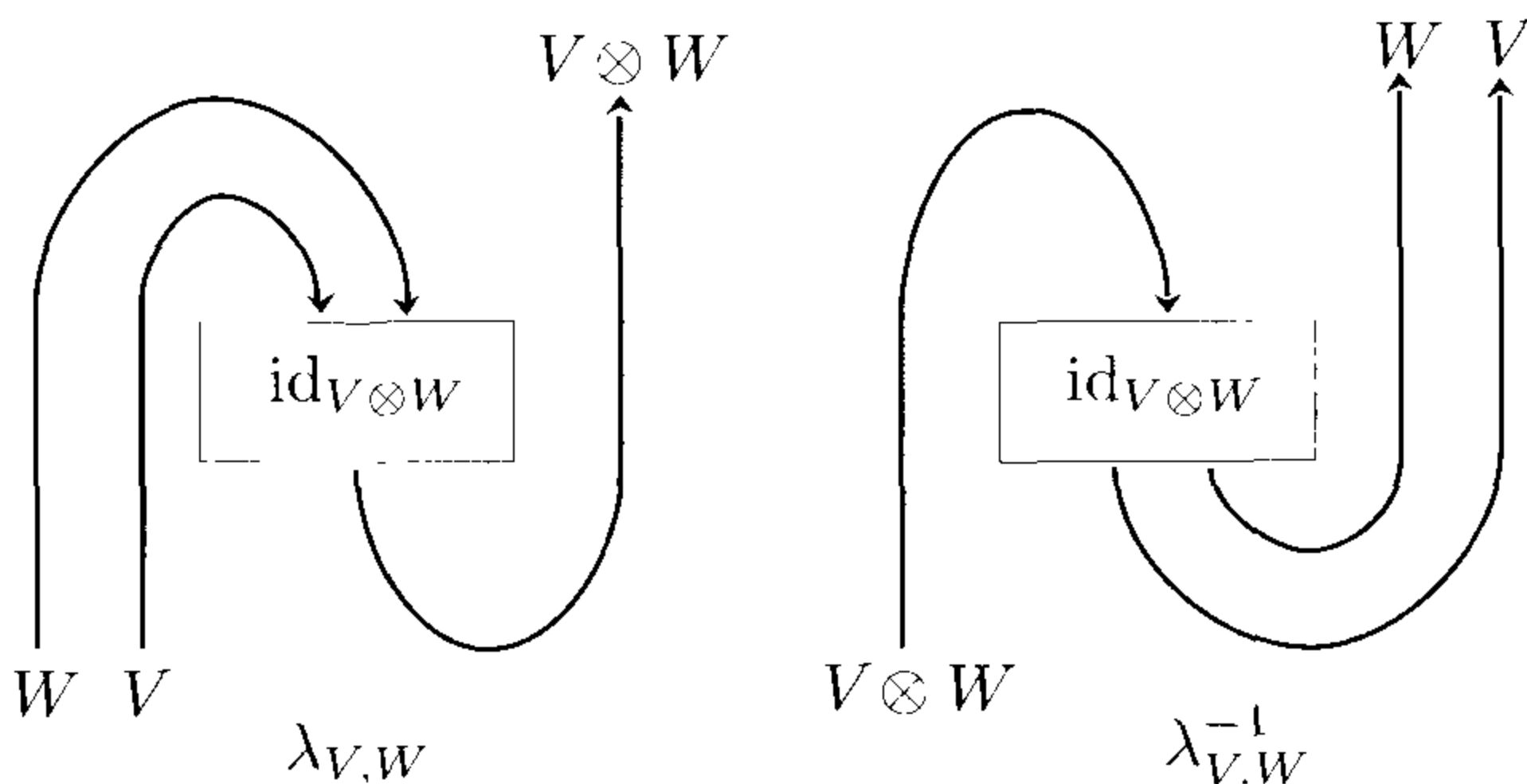
Figure 2.5. The morphisms \lambda_{V,W} and \lambda_{V,W}^{-1}
