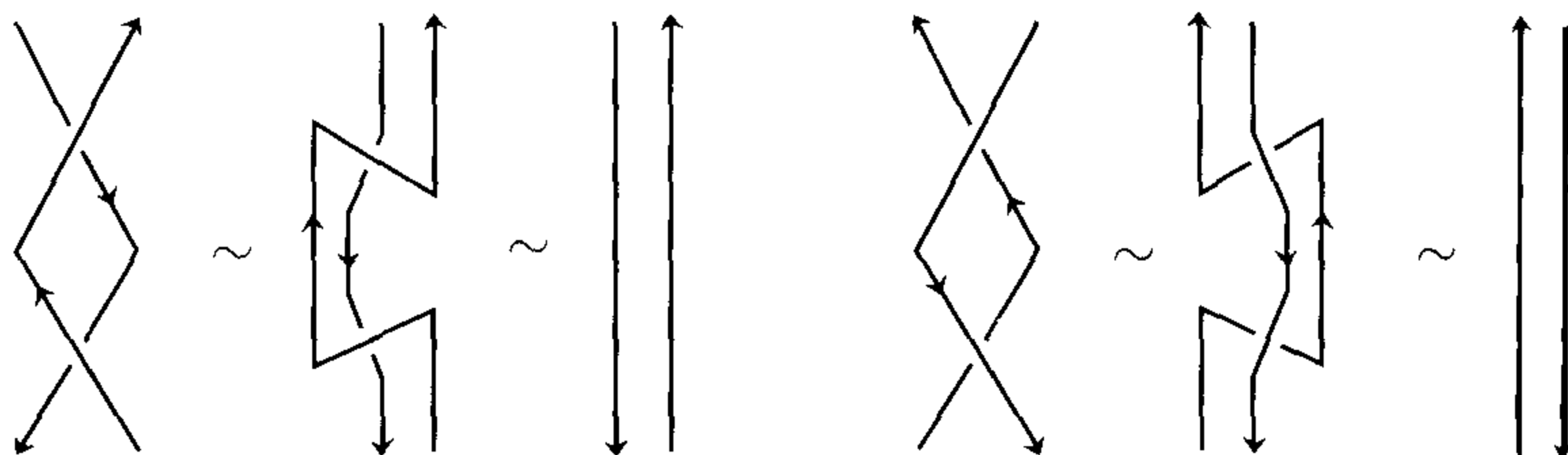
Figure 3.3. Congruence when L = Y or T
