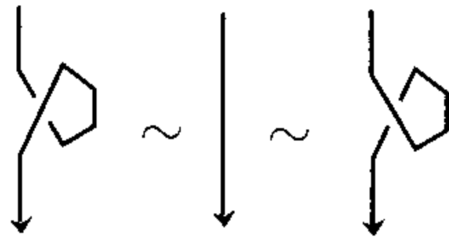
Figure 2.7. Relation (2.6)
