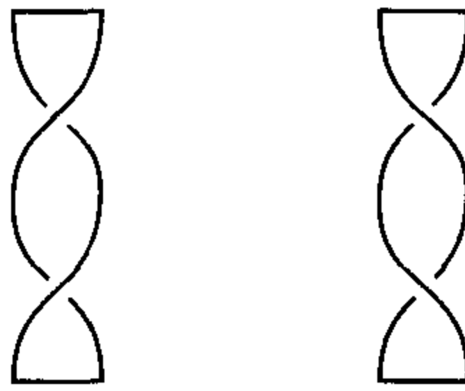
Figure 8.1
