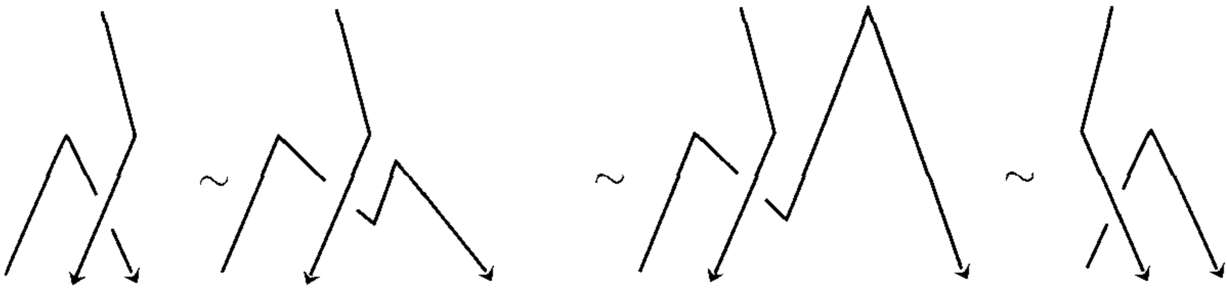
Figure 3.11
