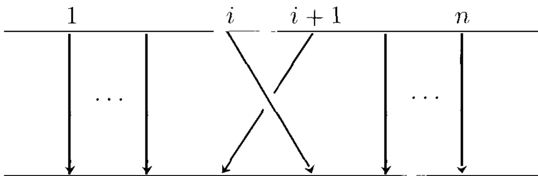
Figure 6.3. The braid \sigma_i^{-1}
