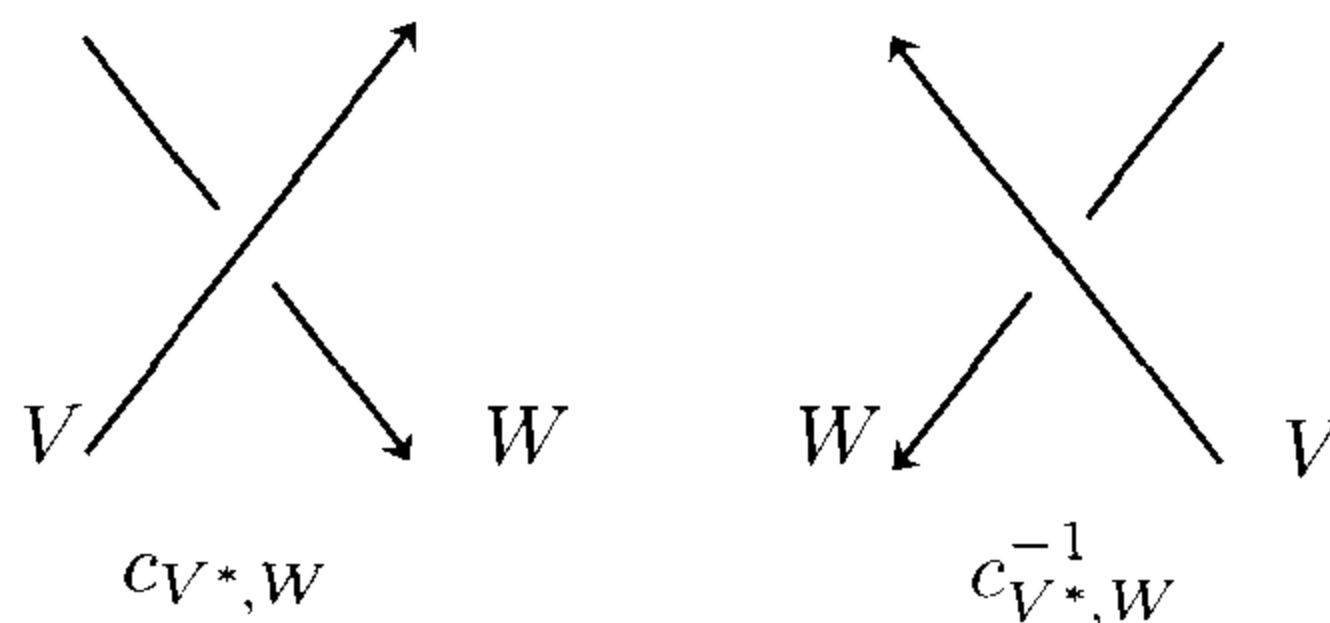
Figure 3.1. c_{V^*,W} and its inverse
