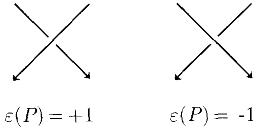
Figure 2.2. The linking number
