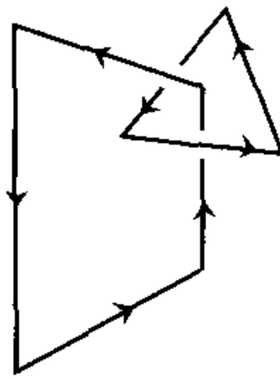
Figure 2.3. The Hopf link
