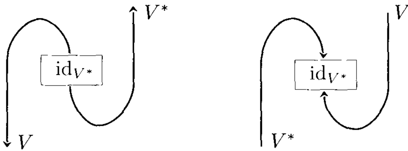
Figure 3.11. Isomorphisms between V and V^{**}
