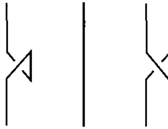
Figure 3.2. Reidemeister move (I)
