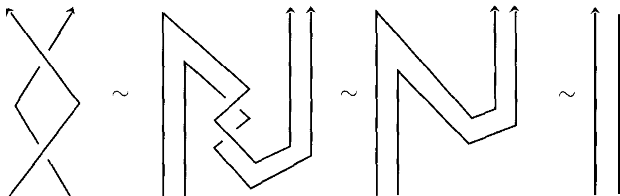
Figure 3.2. Congruence when L = Z
