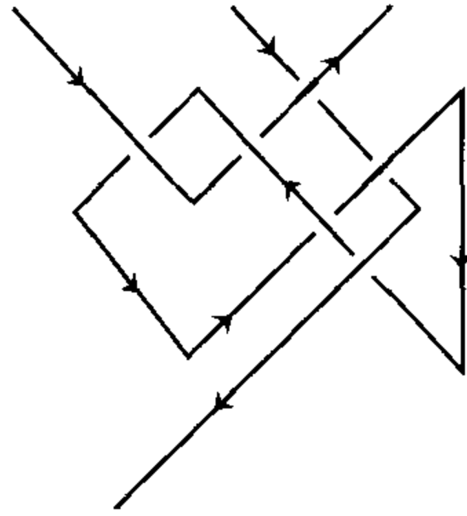
Figure 5.1. A tangle
