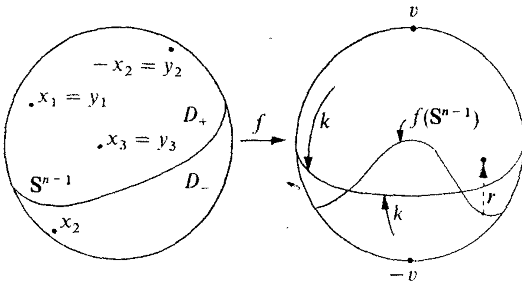
Figure IV-14. Proof of Theorem 20.6.
