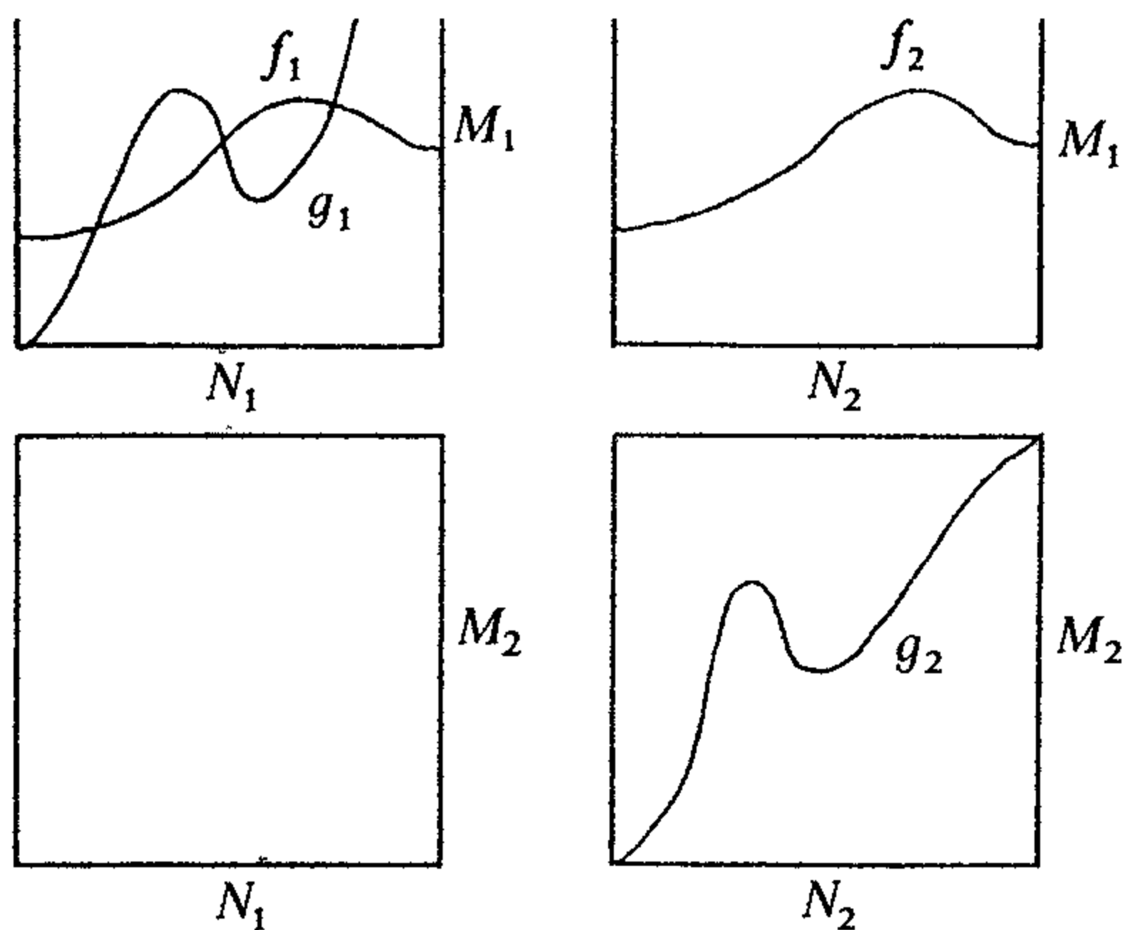
Figure VI-11. Coincidence doubling.
