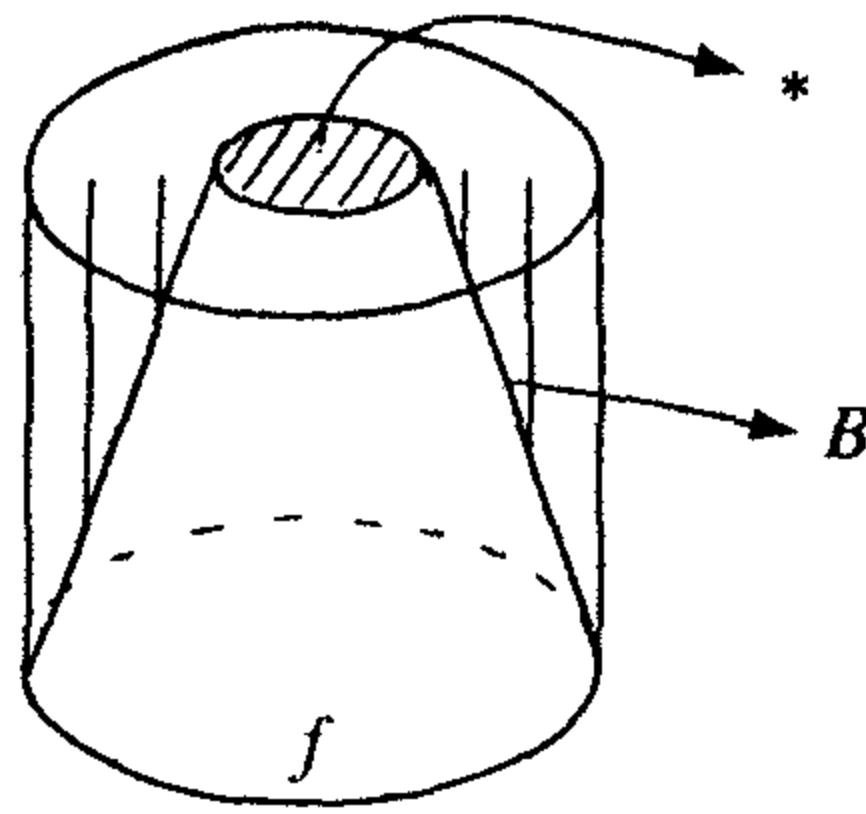
Figure VII-5. A relative homotopy.
