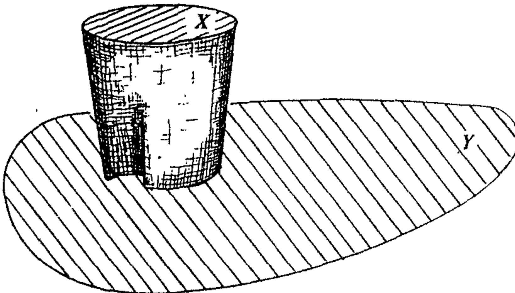
Figure I-2. Mapping cylinder.
