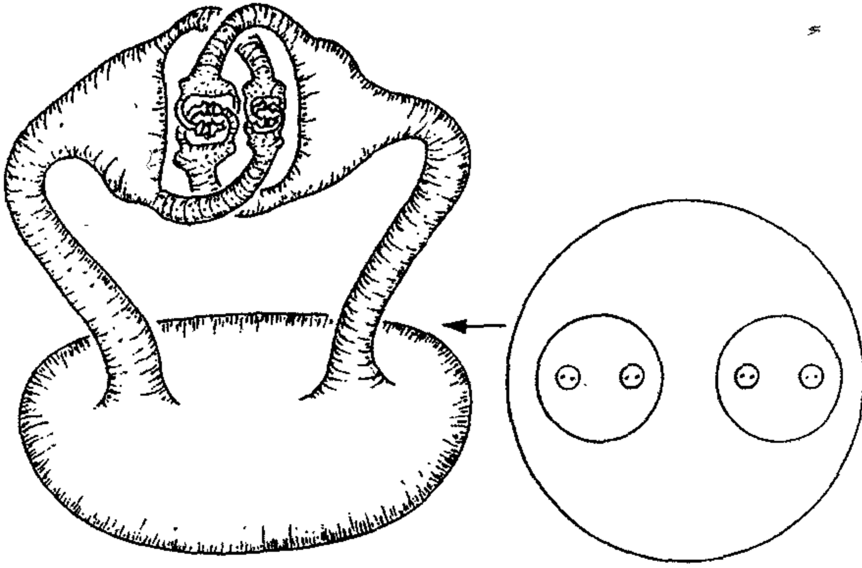
Figure IV-9. The Alexander horned disk.
