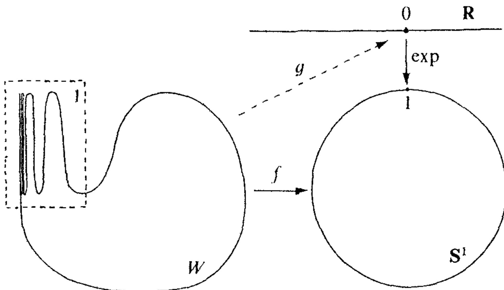
Figure III-6. Discontinuous lifting.
