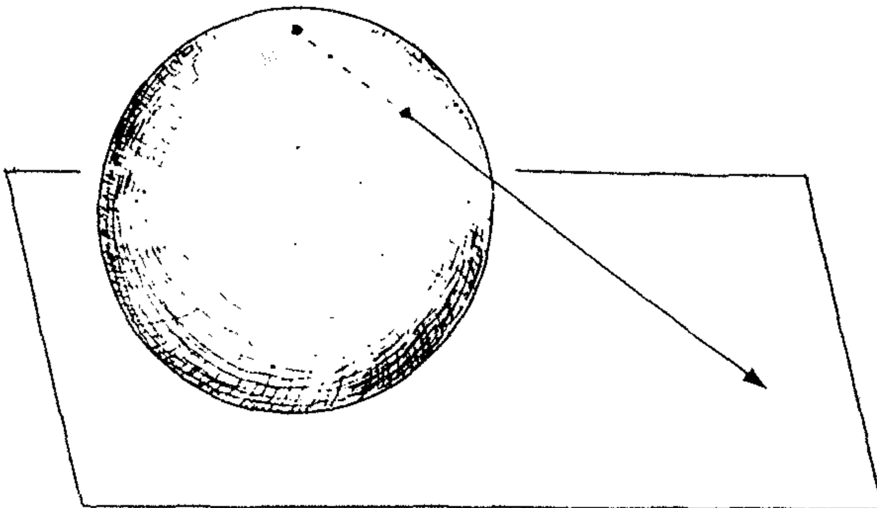
Figure II-2. Stereographic projection.
