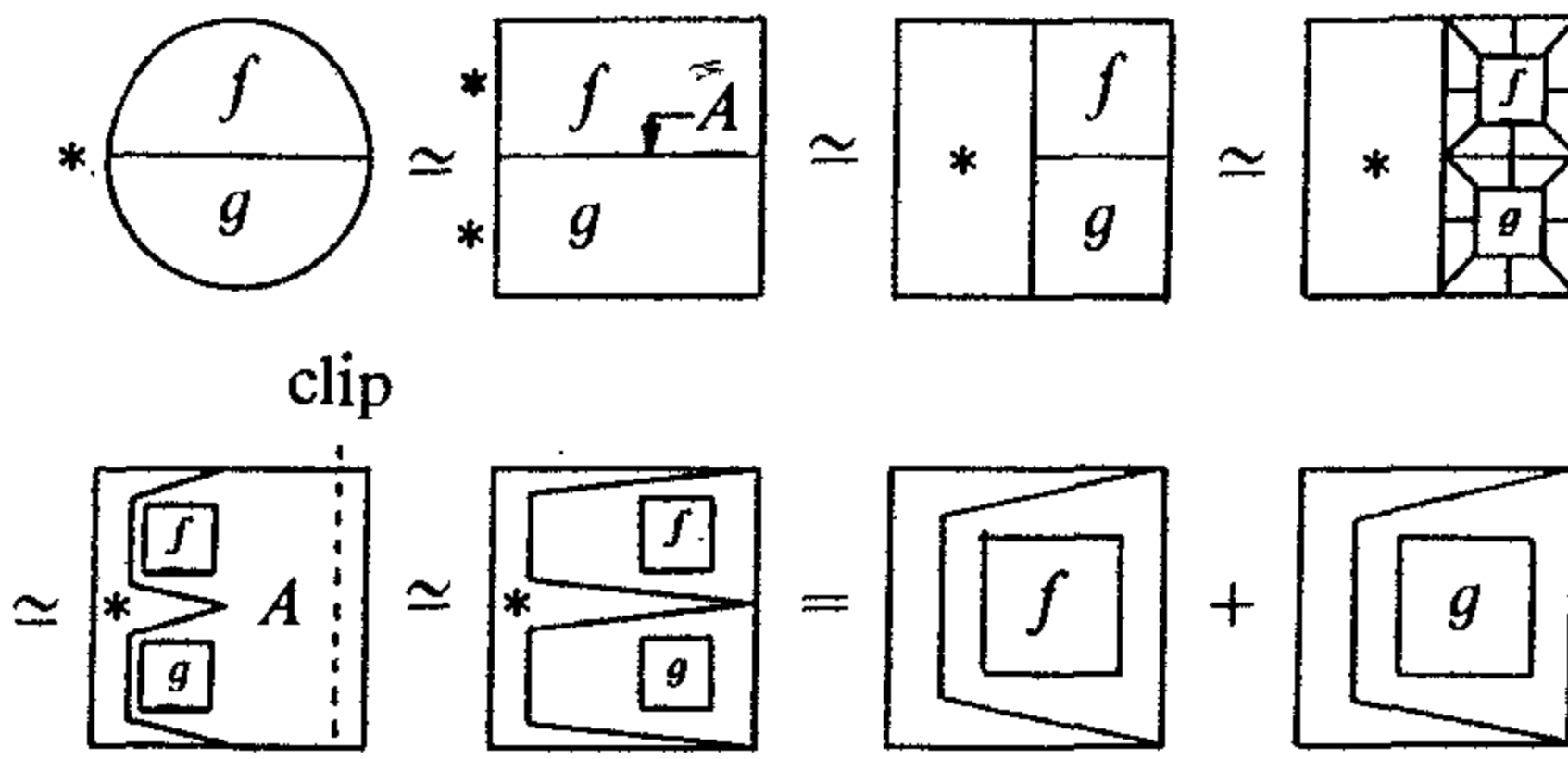
Figure VII-8. Case k = 2 of the Homotopy Addition Theorem.
