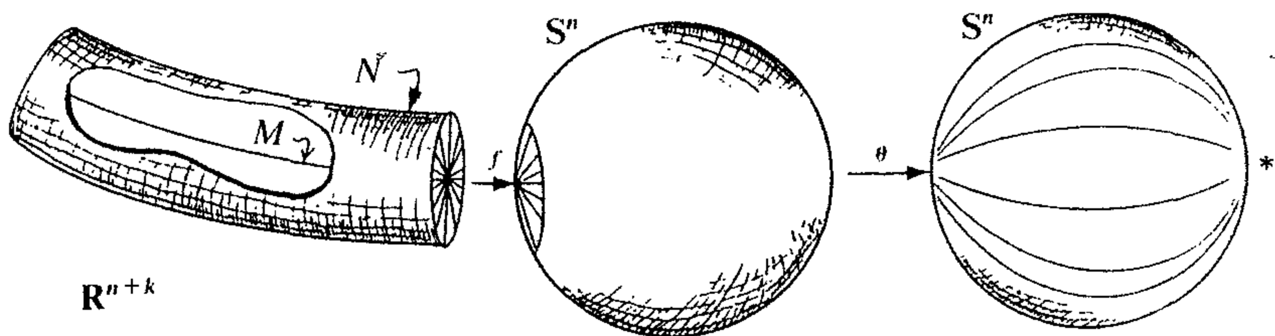
Figure II-13. Thom-Pontryagin construction.
