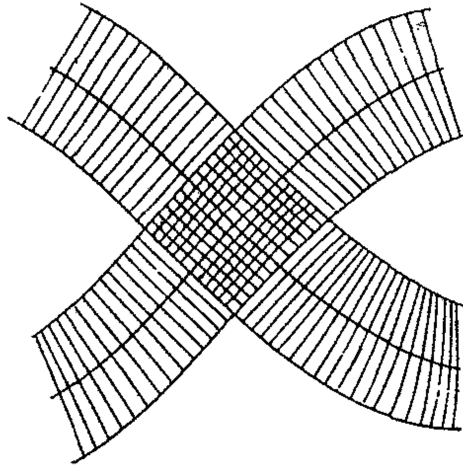
Figure VI-12. Simple plumbing.
