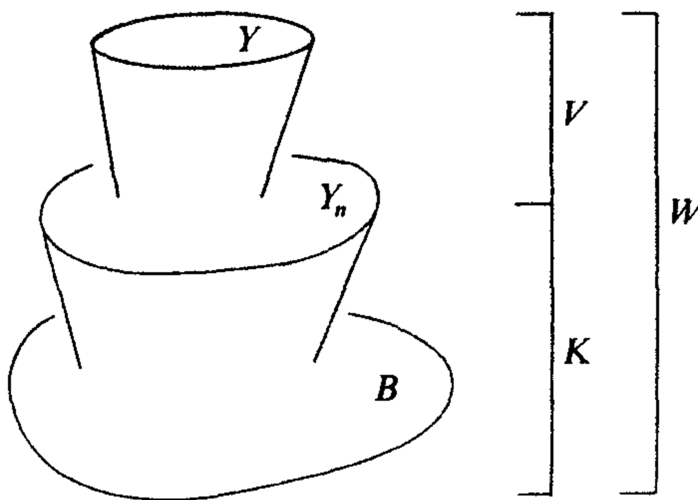
Figure VII-12. Mapping cylinders.
