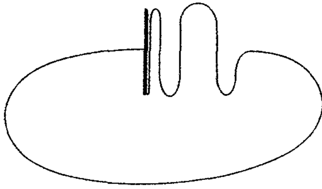
Figure VII-2. A pseudo-circle.
