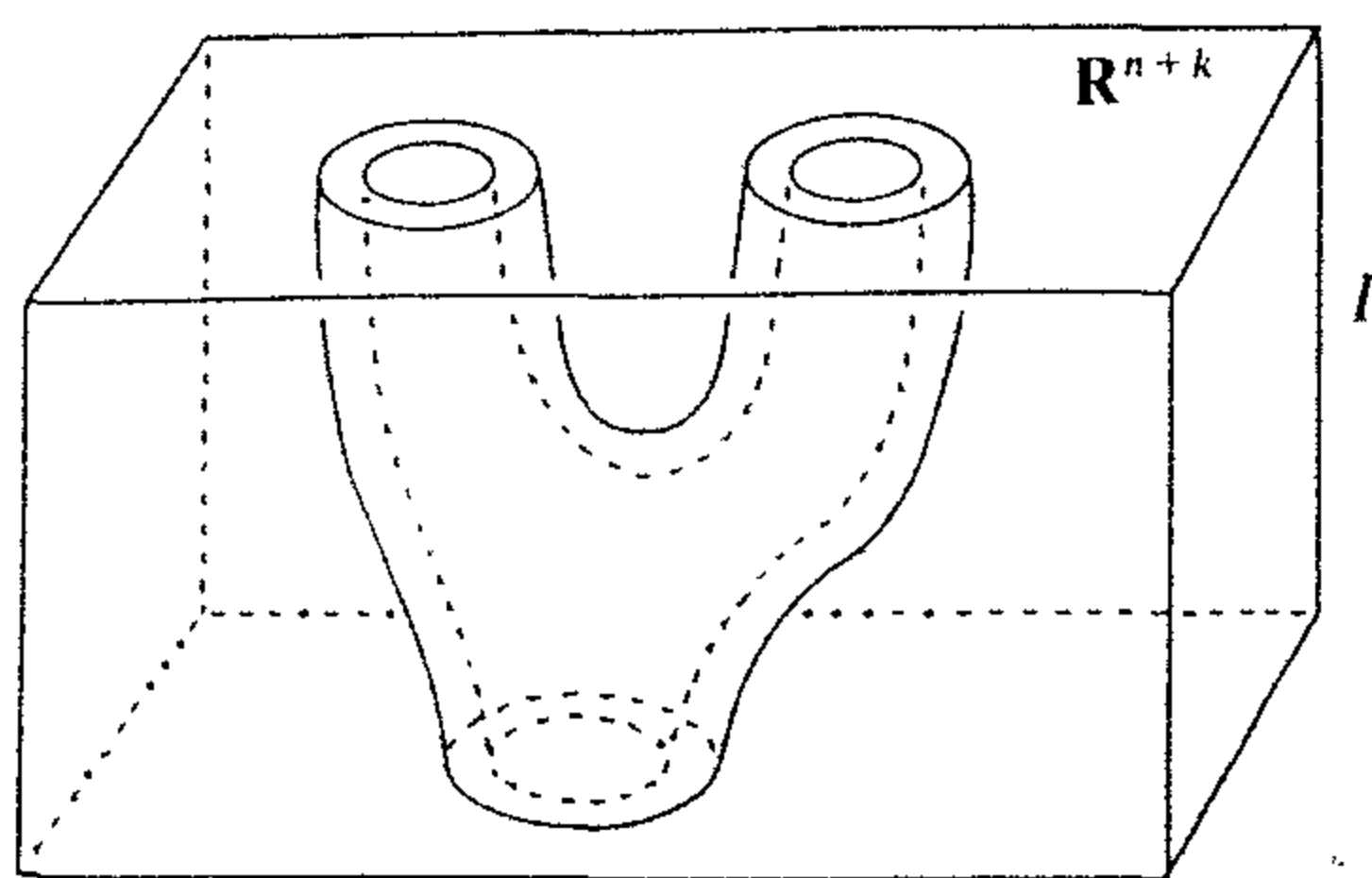
Figure II-14. A cobordism.
