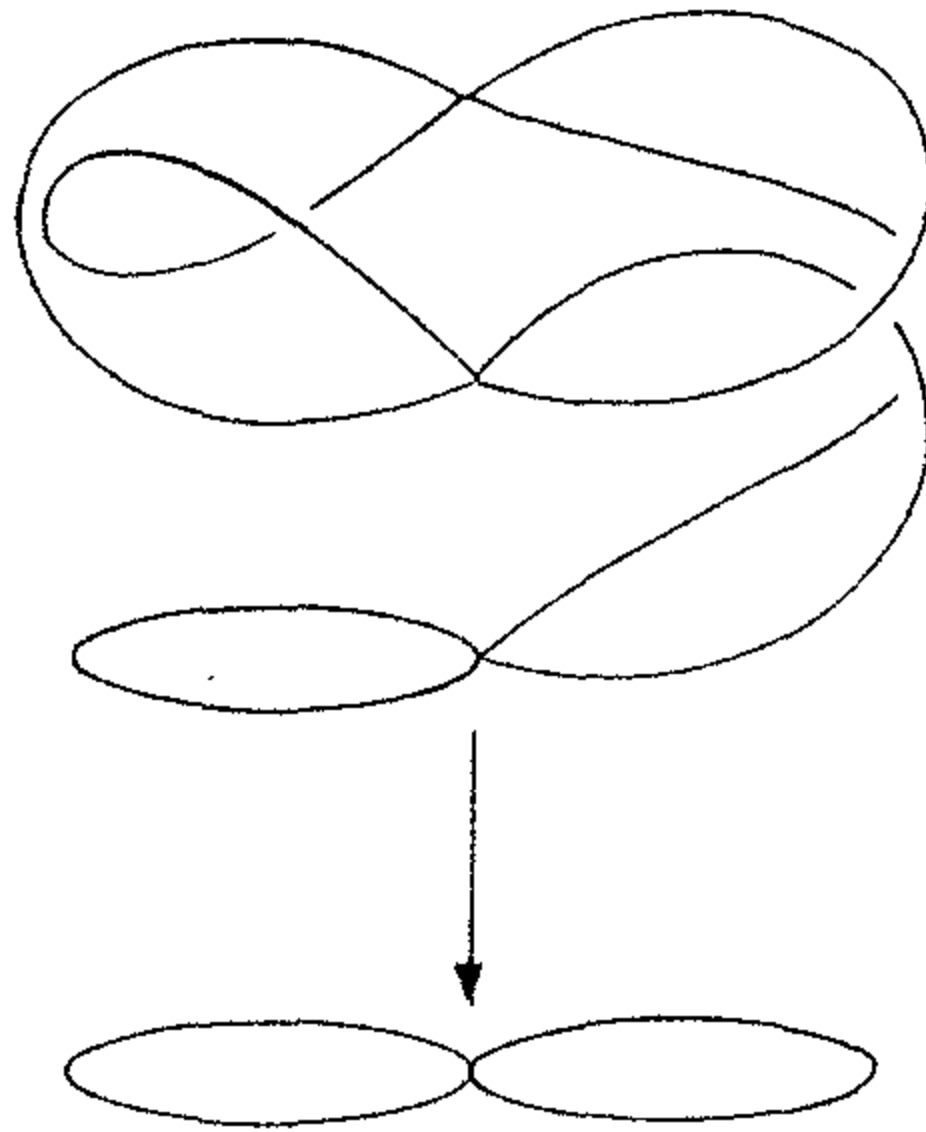
Figure III-5. A threefold covering space.
