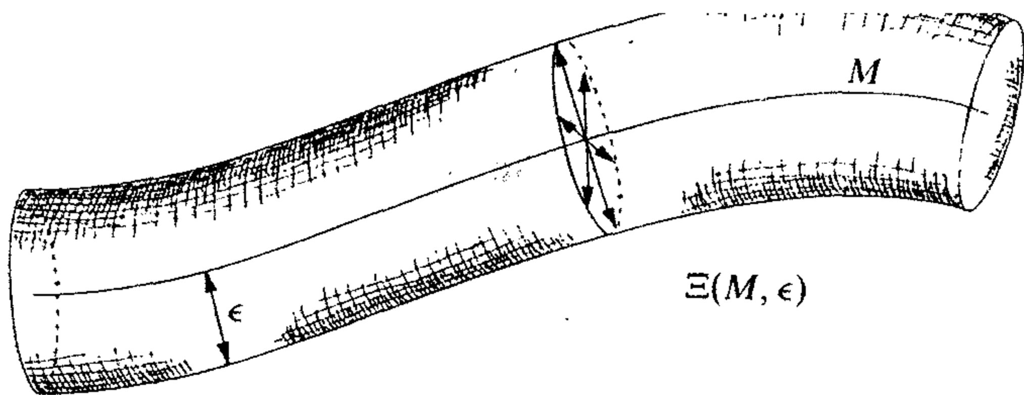
Figure II-7. Tubular neighborhood.
