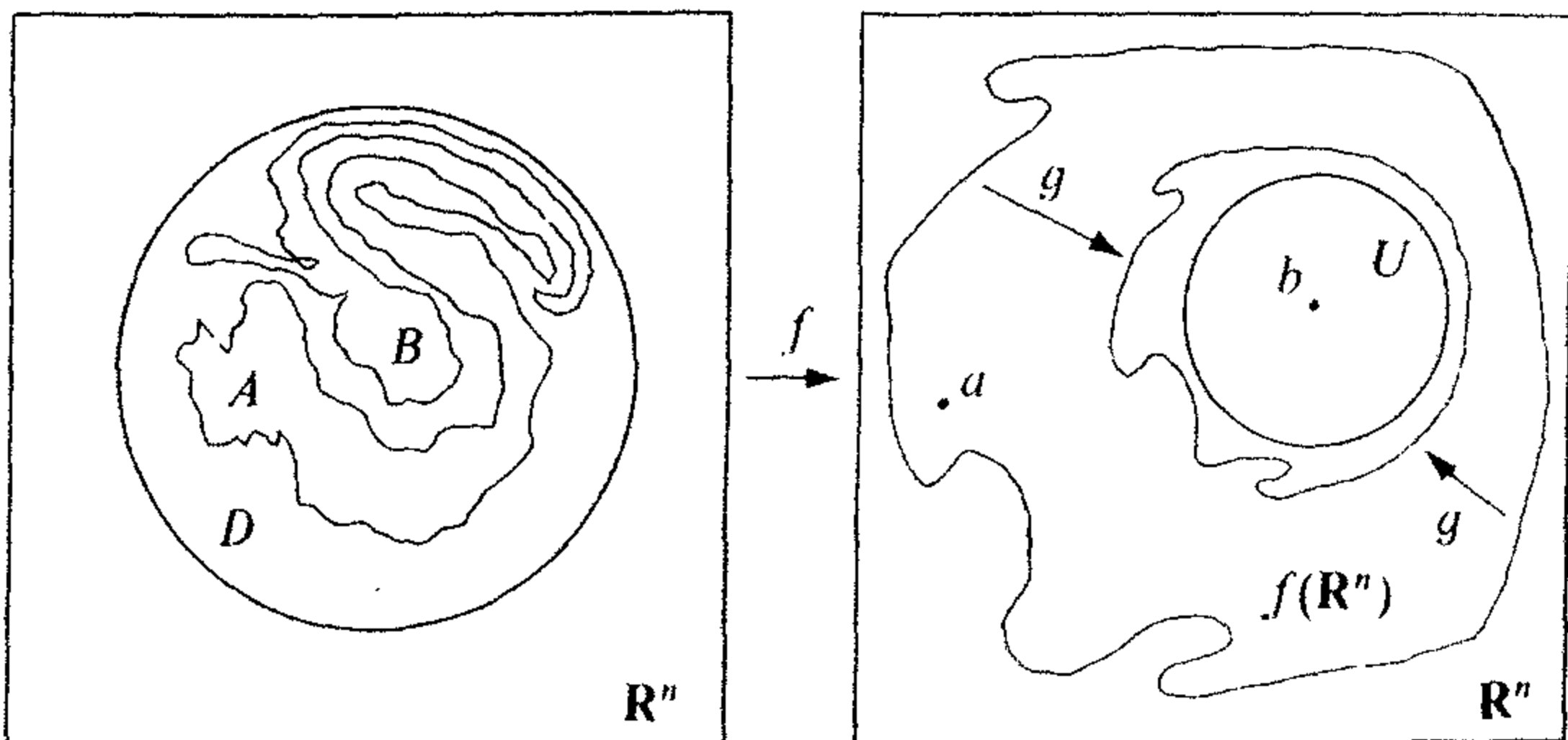
Figure IV-10. Avoiding B.
