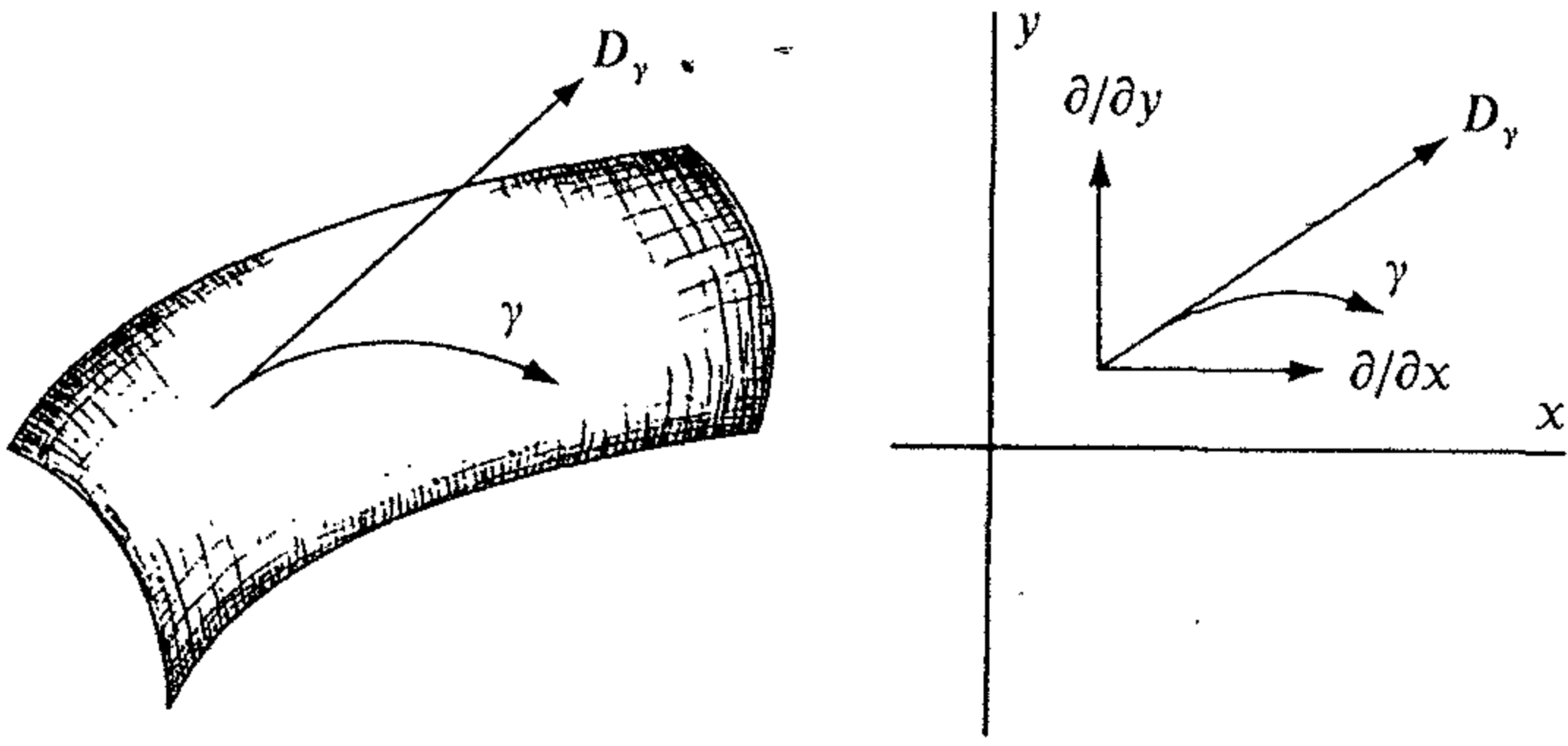
Figure II-4. Tangent vectors.
