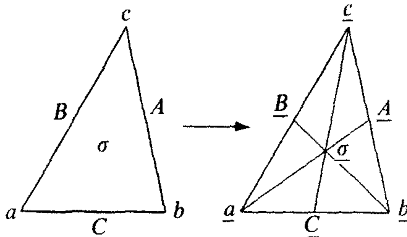
Figure IV-7. Barycentric subdivision.
