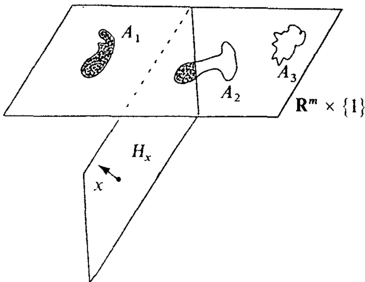
Figure IV-13. Ham sandwich.
