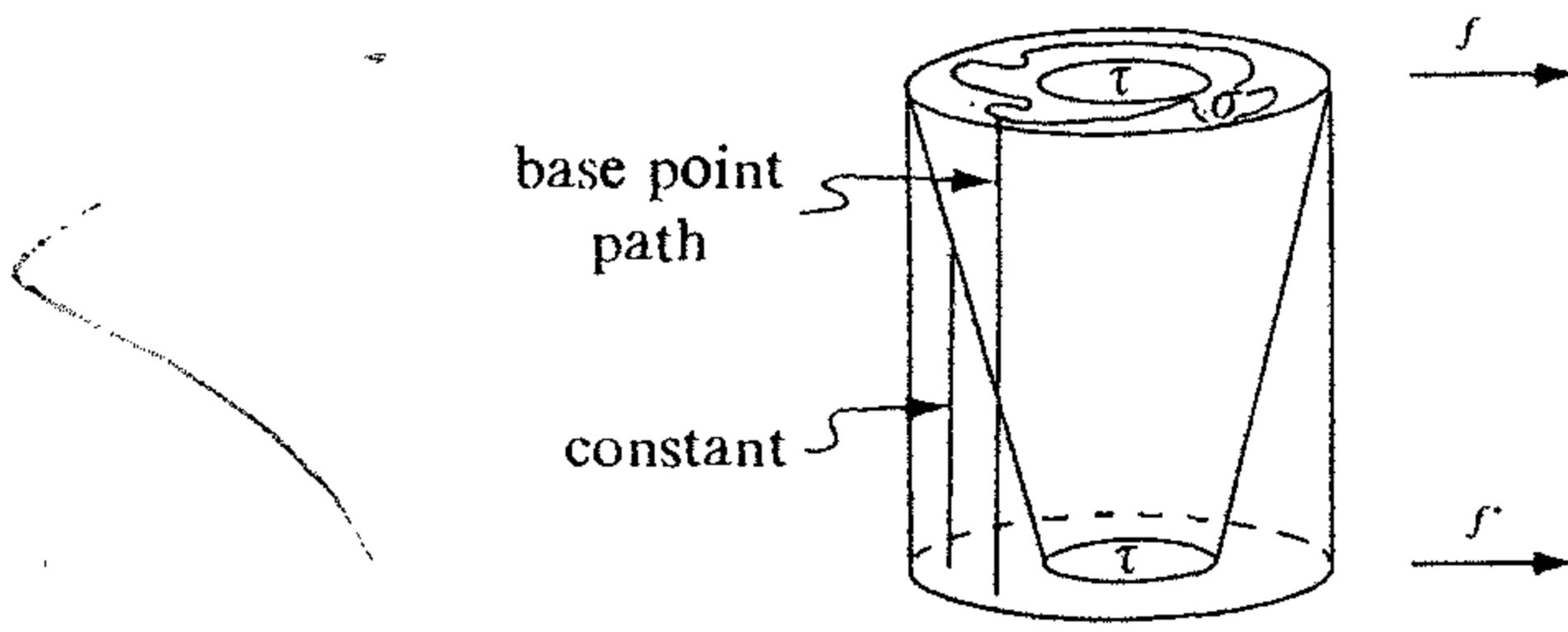
Figure VII-10. Stage 2 homotopy.
