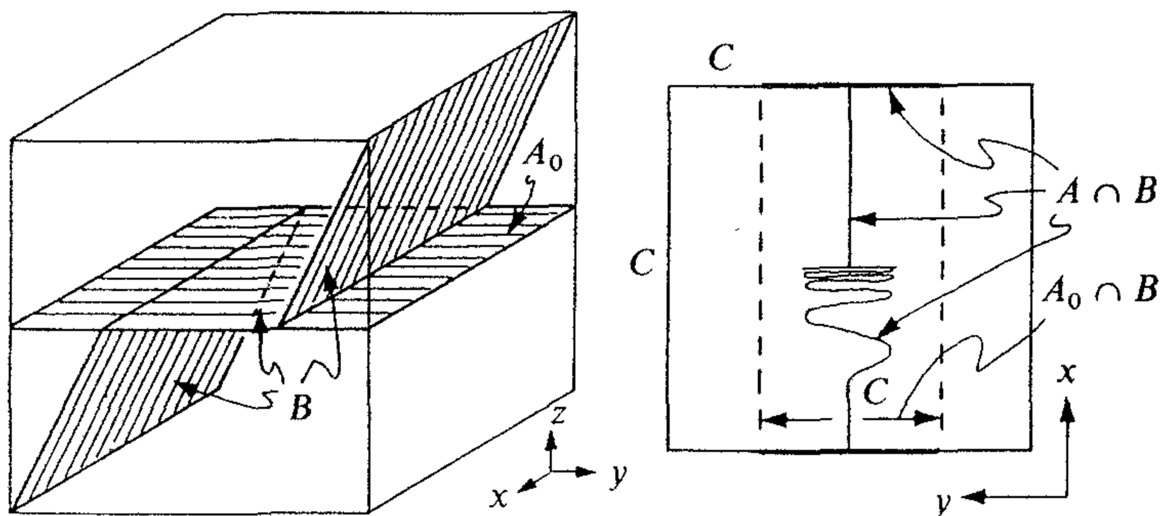
Figure VI-8. Wild intersection in 3-torus.
