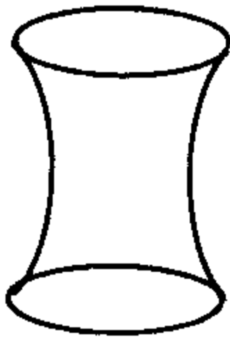
smooth quadric (rank 4)
