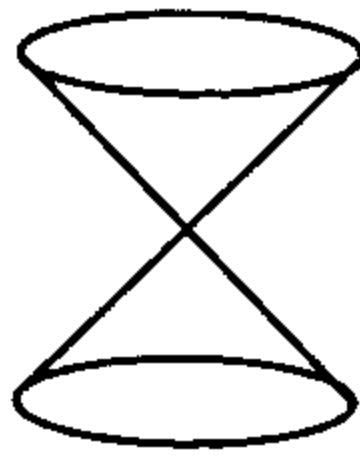
quadric cone (rank 3)
