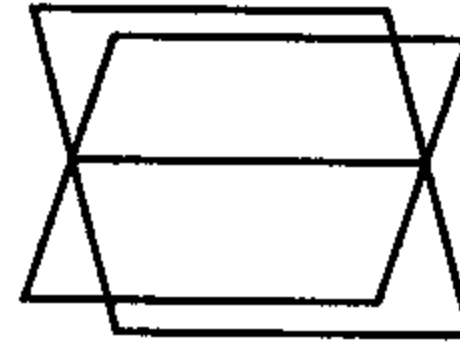
pair of planes (rank 2)
