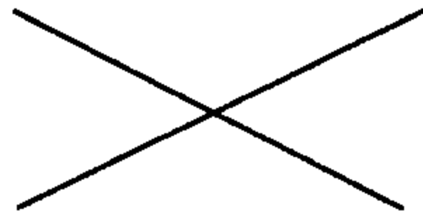
pair of lines (rank 2)
