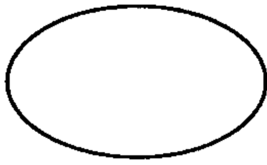
smooth conic (rank 3)
