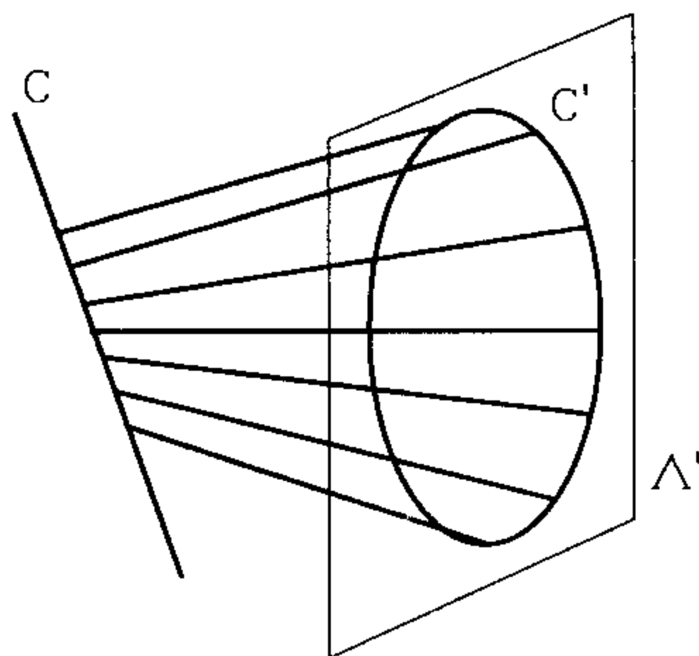
the scroll S_{2,1} \subset \mathbb{P}^4
