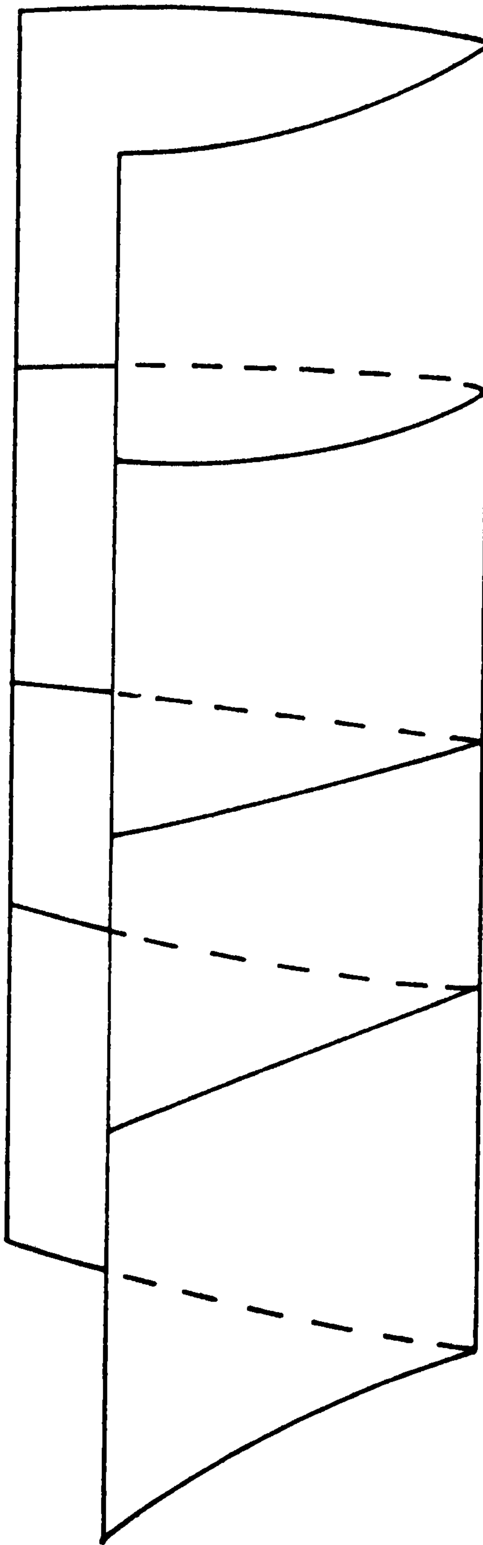
Figure 10: The Hyperbolic Umbilic
