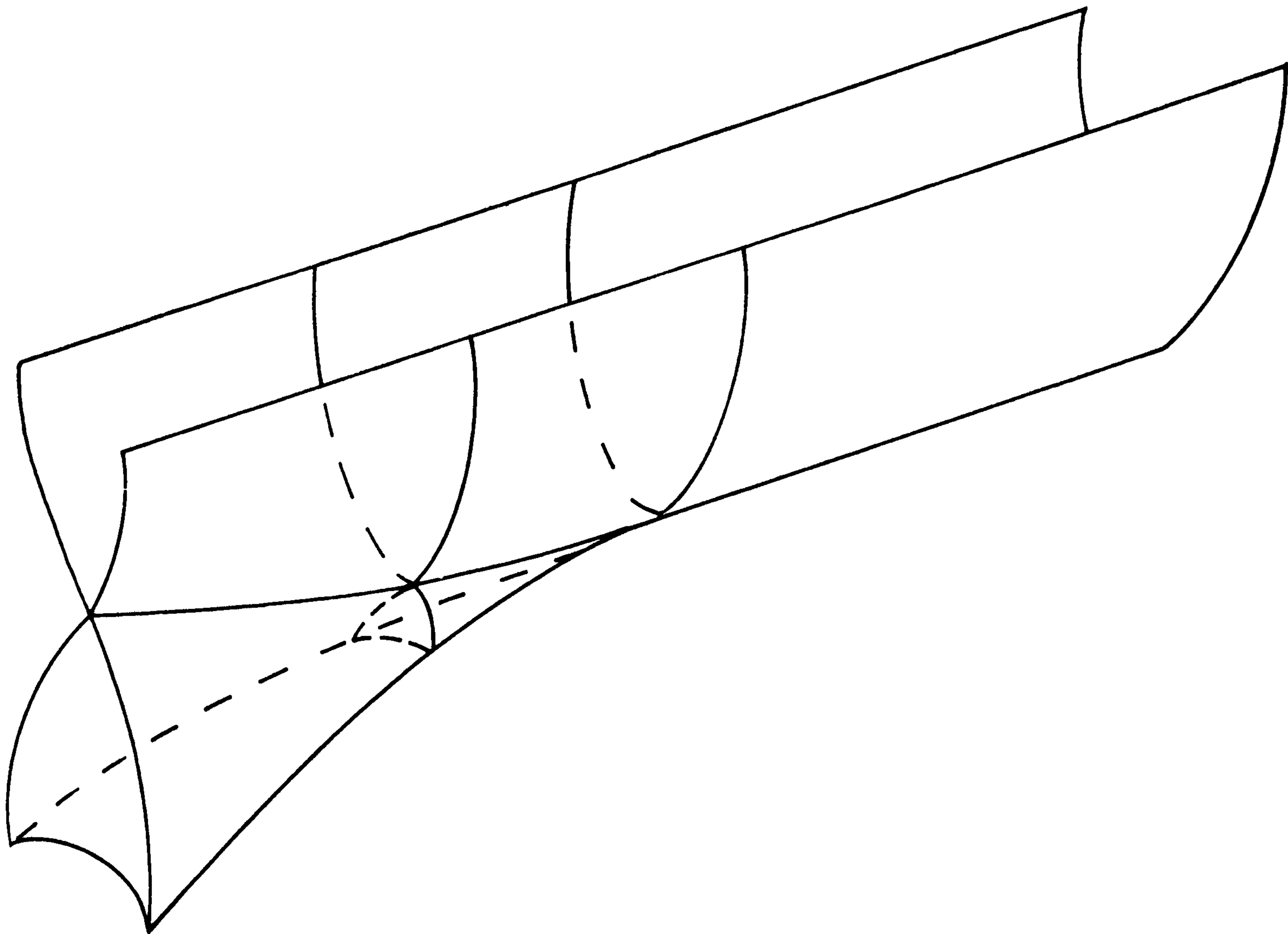
Figure 5: The Swallow's Tail
