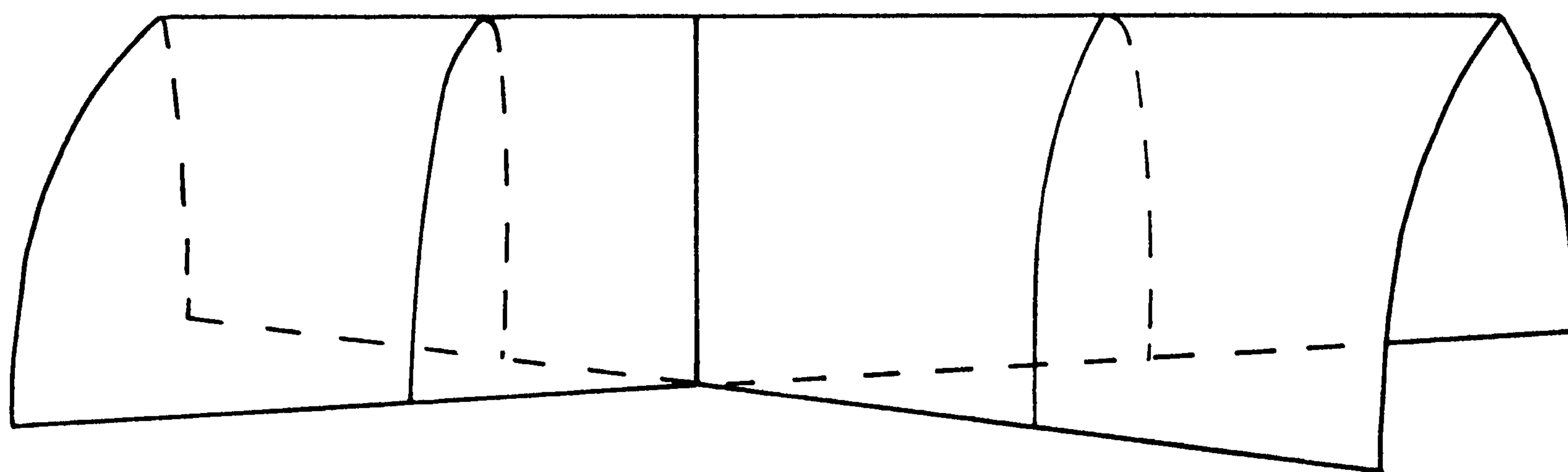
Figure 6: The Cross Cap
