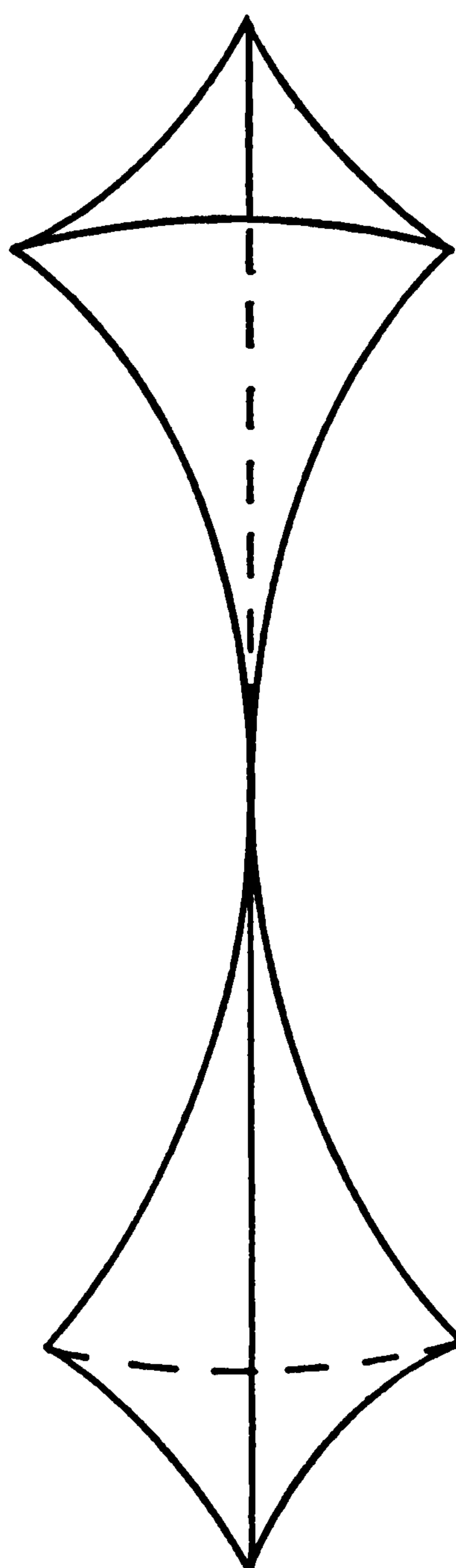
Figure 9: The elliptic Umbilic
