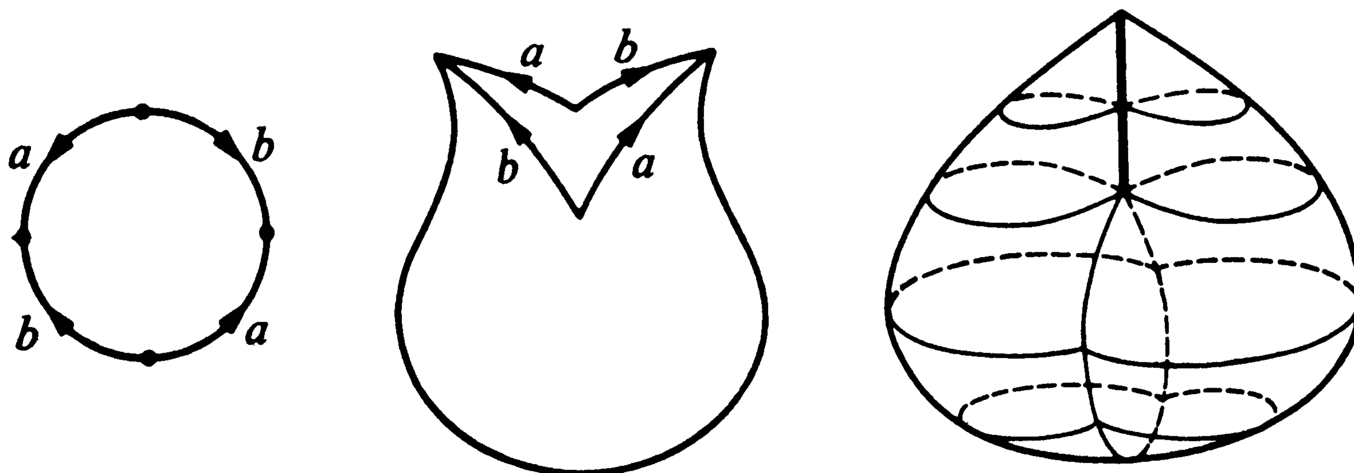
Figure 7: The Topological Cross Cap
