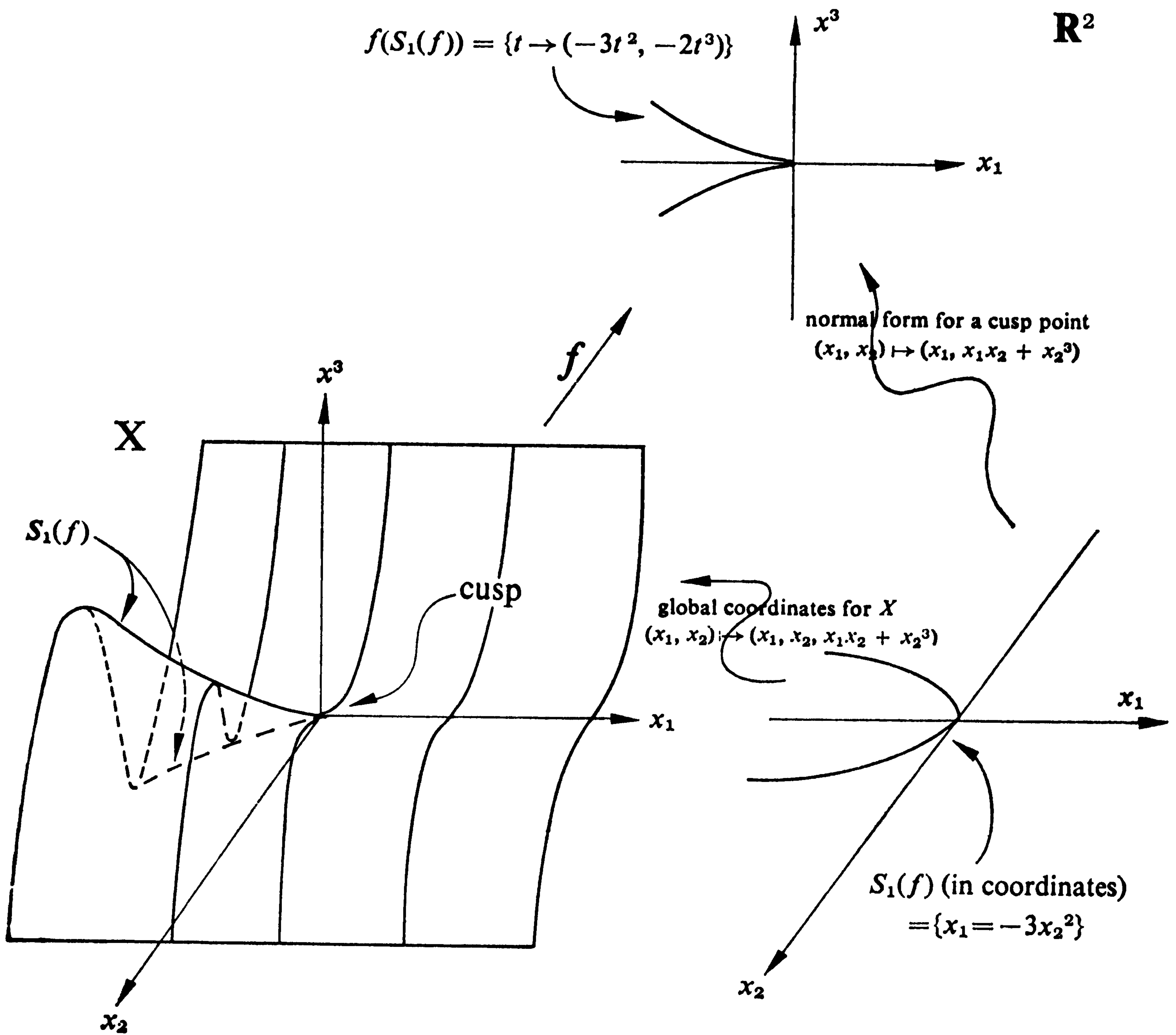
Figure 3: The Simple Cusp
