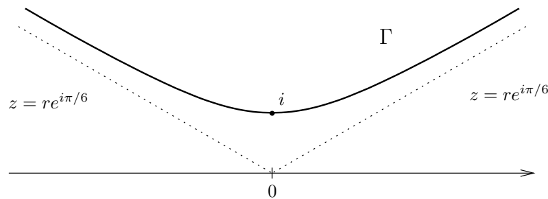
Figure 4. The curve of steepest descent
