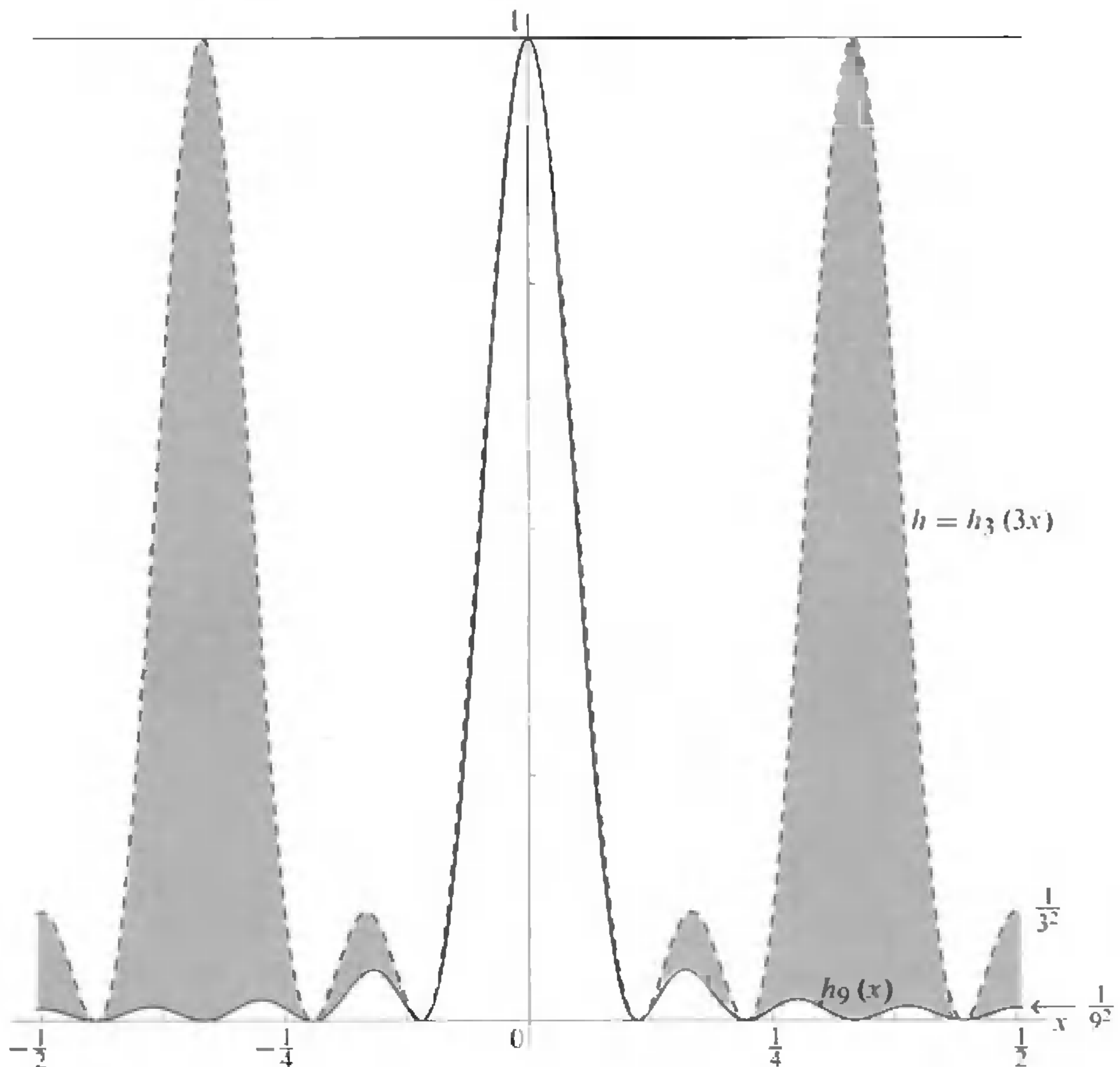
Fig. 6.2. Solutions to the eigenvalue problem (6.2.19).
