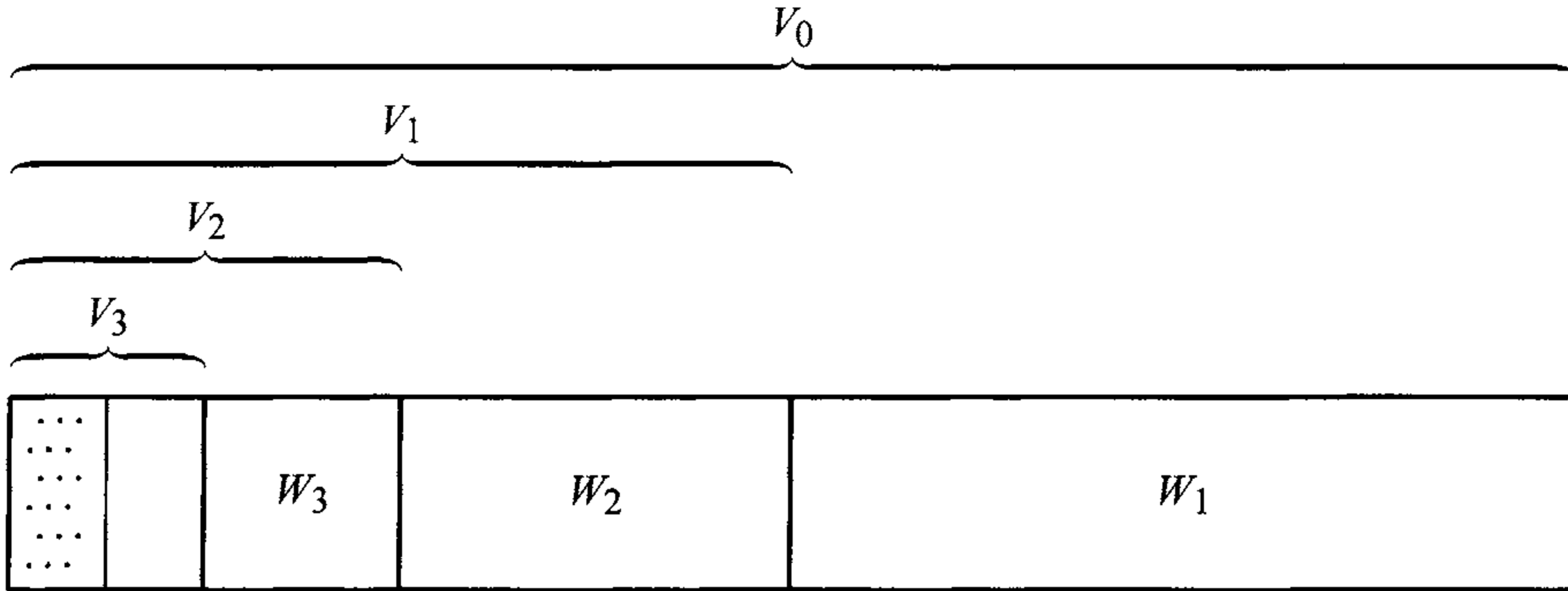
Fig. 7.6. A decreasing family of resolution subspaces V_0 \supset V_1 \supset V_2 \supset \dots , and corresponding detail spaces W_1, W_2, \dots . Dyadic wavelets. V_n = V_{n+1} + W_{n+1}, n = 0, 1, \dots
