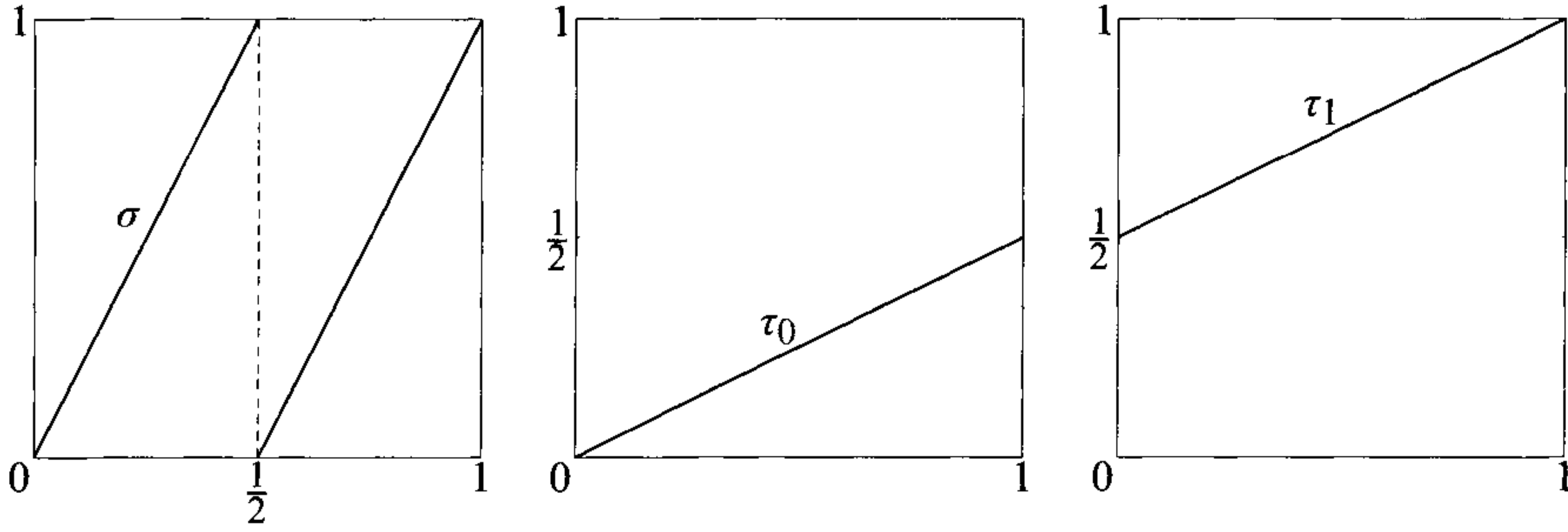
Fig. 5.1. The 2-adic fractions.
