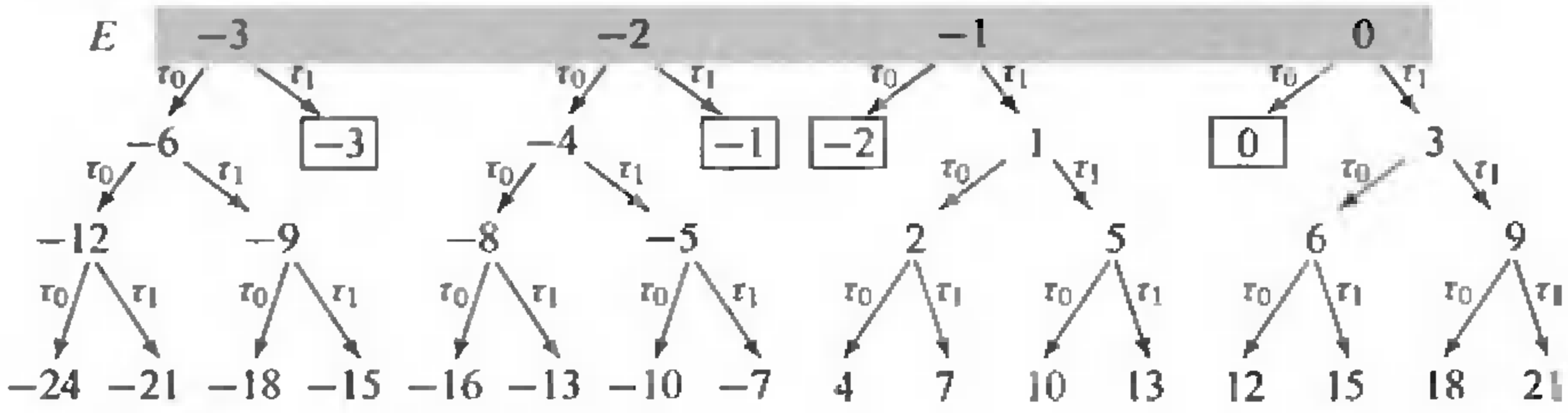
Fig. 8.2. Branching with step size 3.
