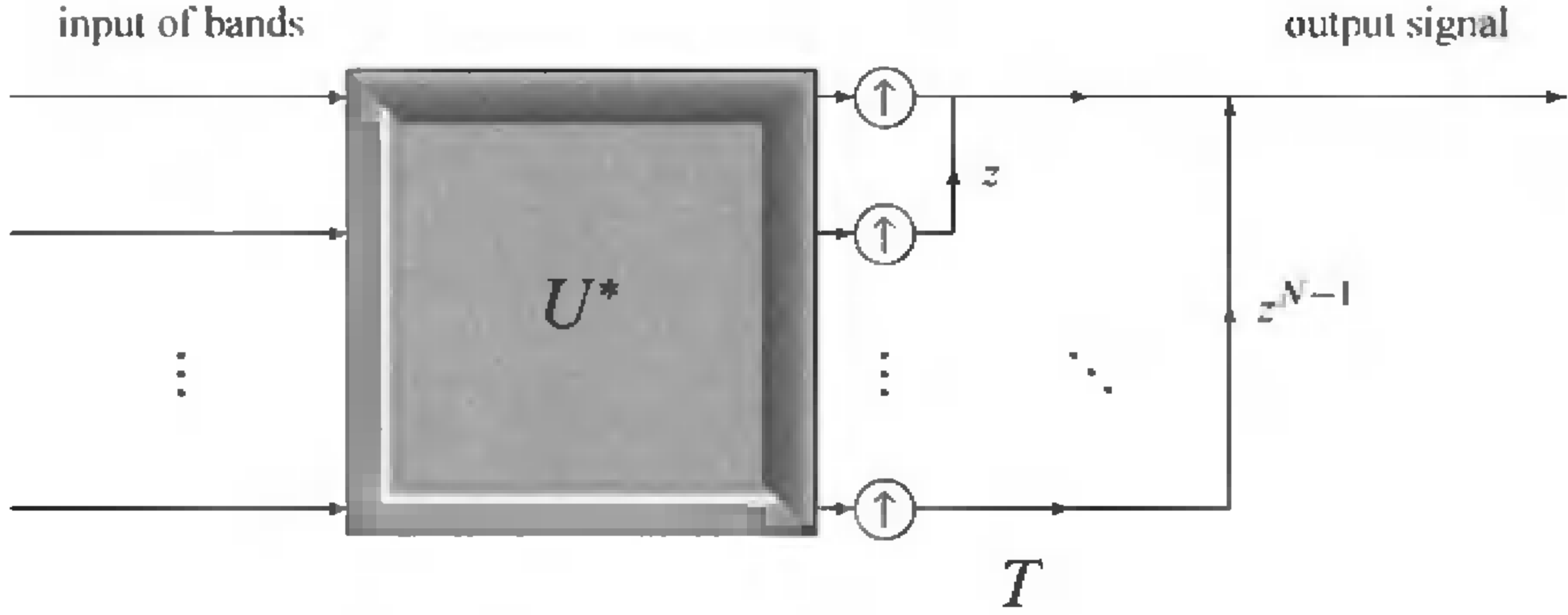
Fig. C.1. Representation of S = TU^* . This and the next diagram illustrate the use of the operator relations from Appendix C in synthesis of subbands of a signal, or of a subdivision of an image. The two diagrams form a pair. The present first one represents a matrix action transforming one band-configuration into another. This is followed by up-sampling applied to each strand. There is then a system of translations before the strands are merged and added. This diagram is a natural dual version of the next one, Figure C.2, i.e., the analysis step which begins with subdivision, or breaking apart an input signal.
