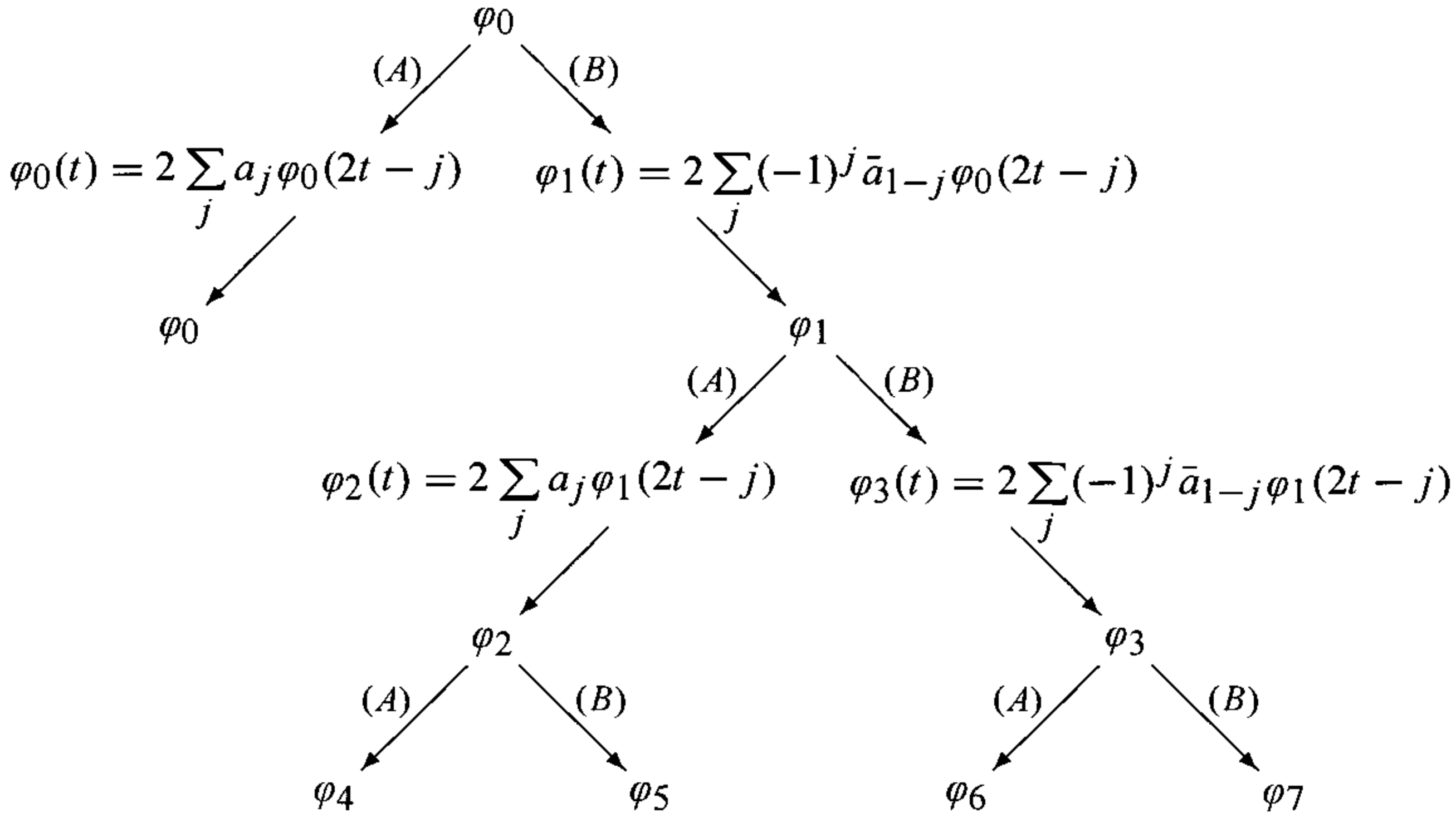
Fig. 7.2. The generation of the basis functions \varphi_0, \varphi_1, \varphi_2, \dots by use of the algorithm (7.5.5) initiated with \varphi_0 = \varphi such that \varphi(t) = 2 \sum_j a_j \varphi(2t - j) , the functional equation by which, in the first (A) branch, \varphi_0 “re-generates” itself.
