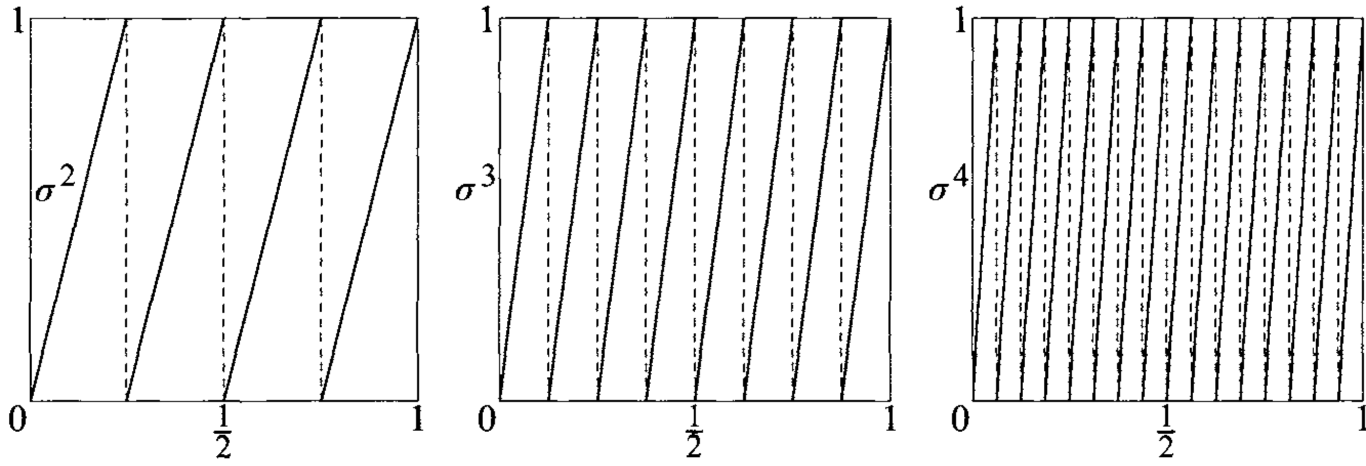
Fig. 5.2. Powers of \sigma .
