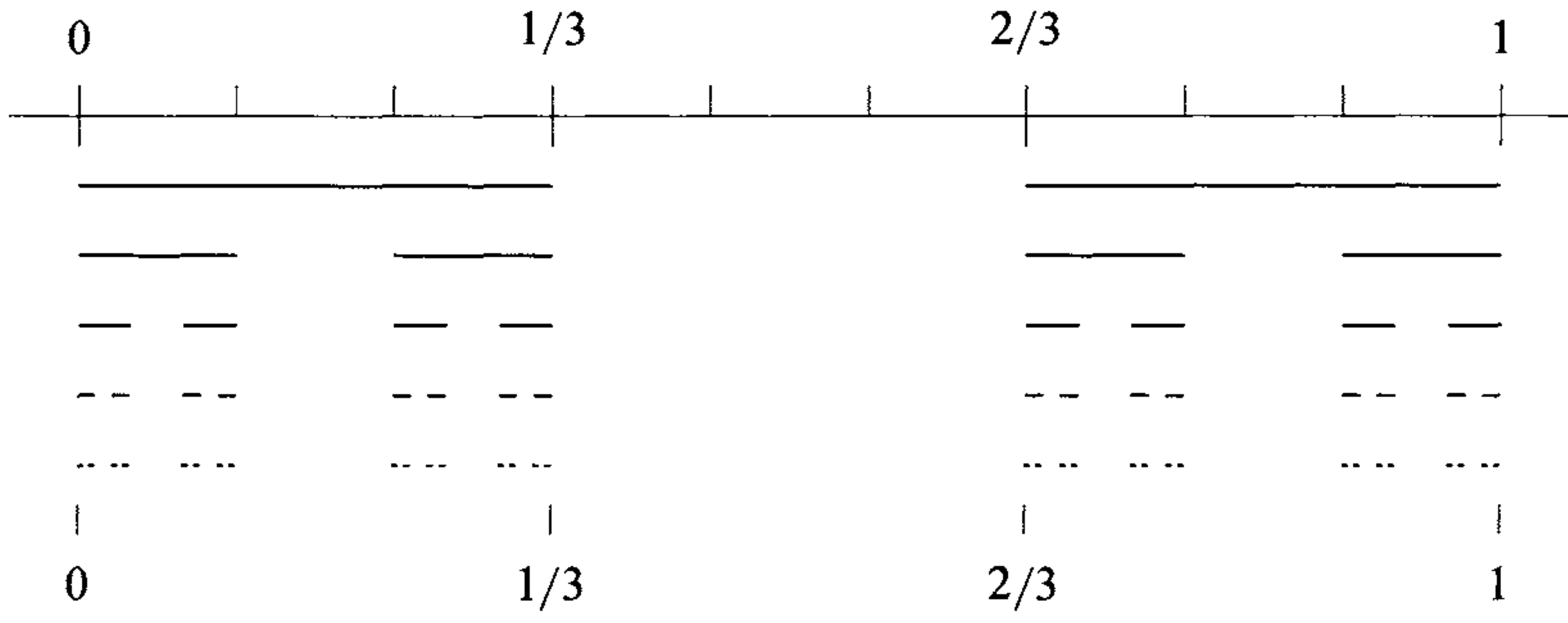
(a) X_3 : middle-third Cantor set.
