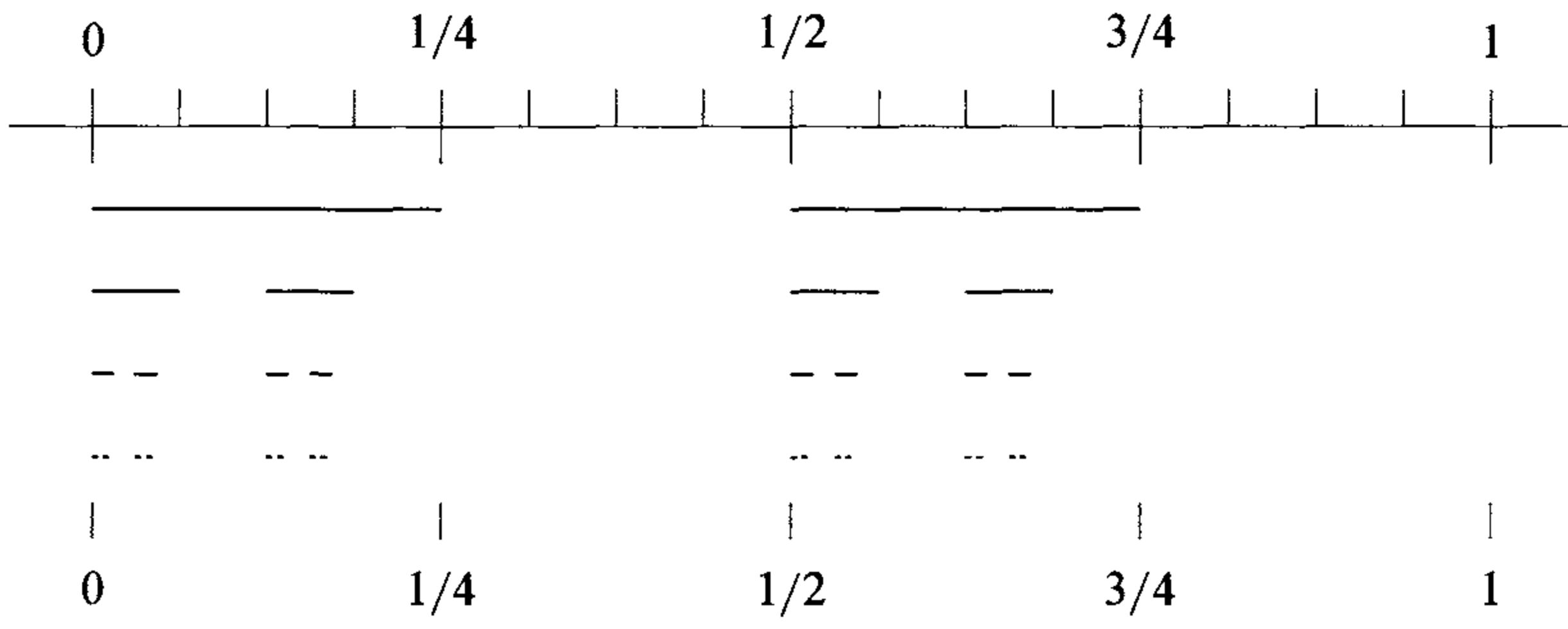
(b) X_4 : the quarter Cantor set.
