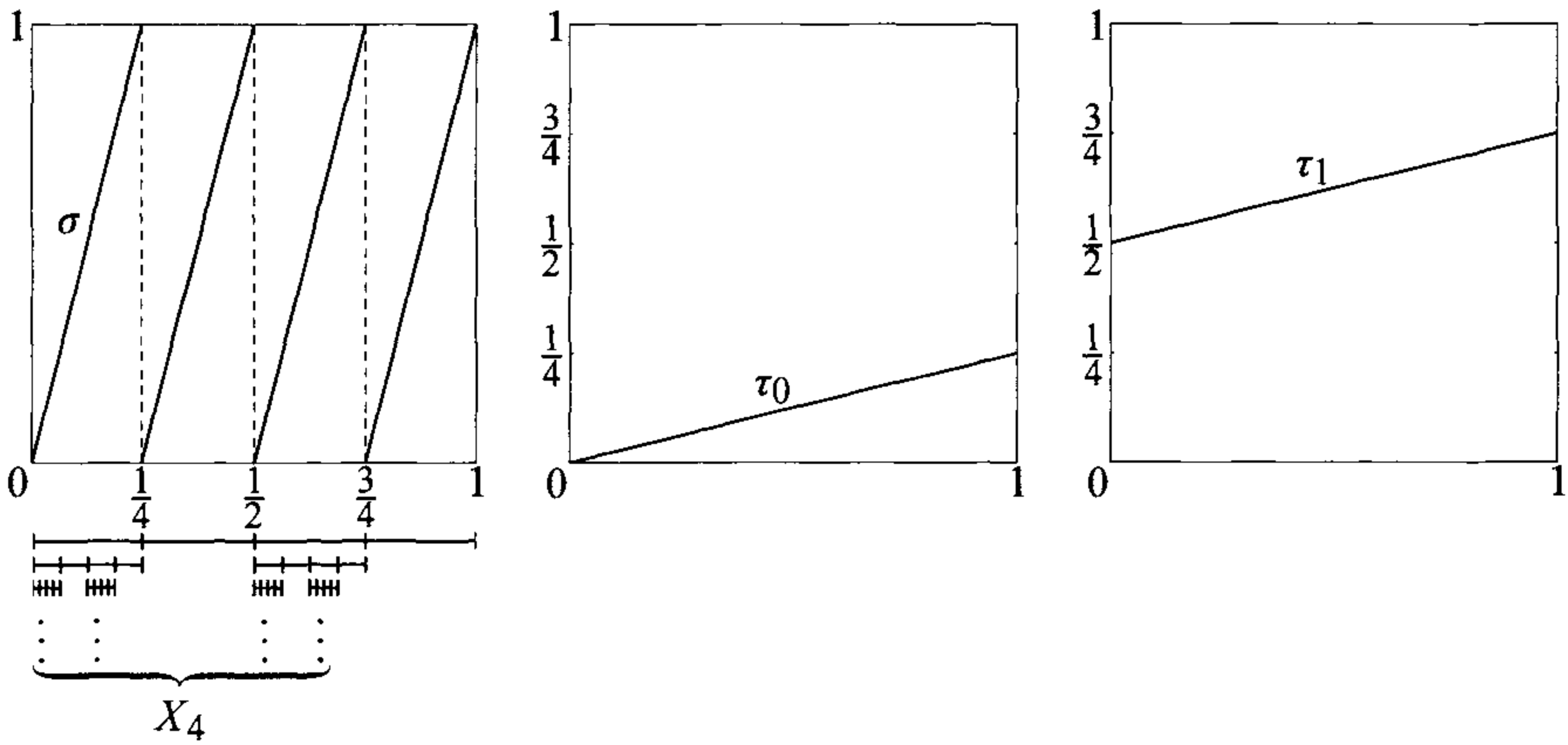
Fig. 4.3. The quarter Cantor set X_4 .
