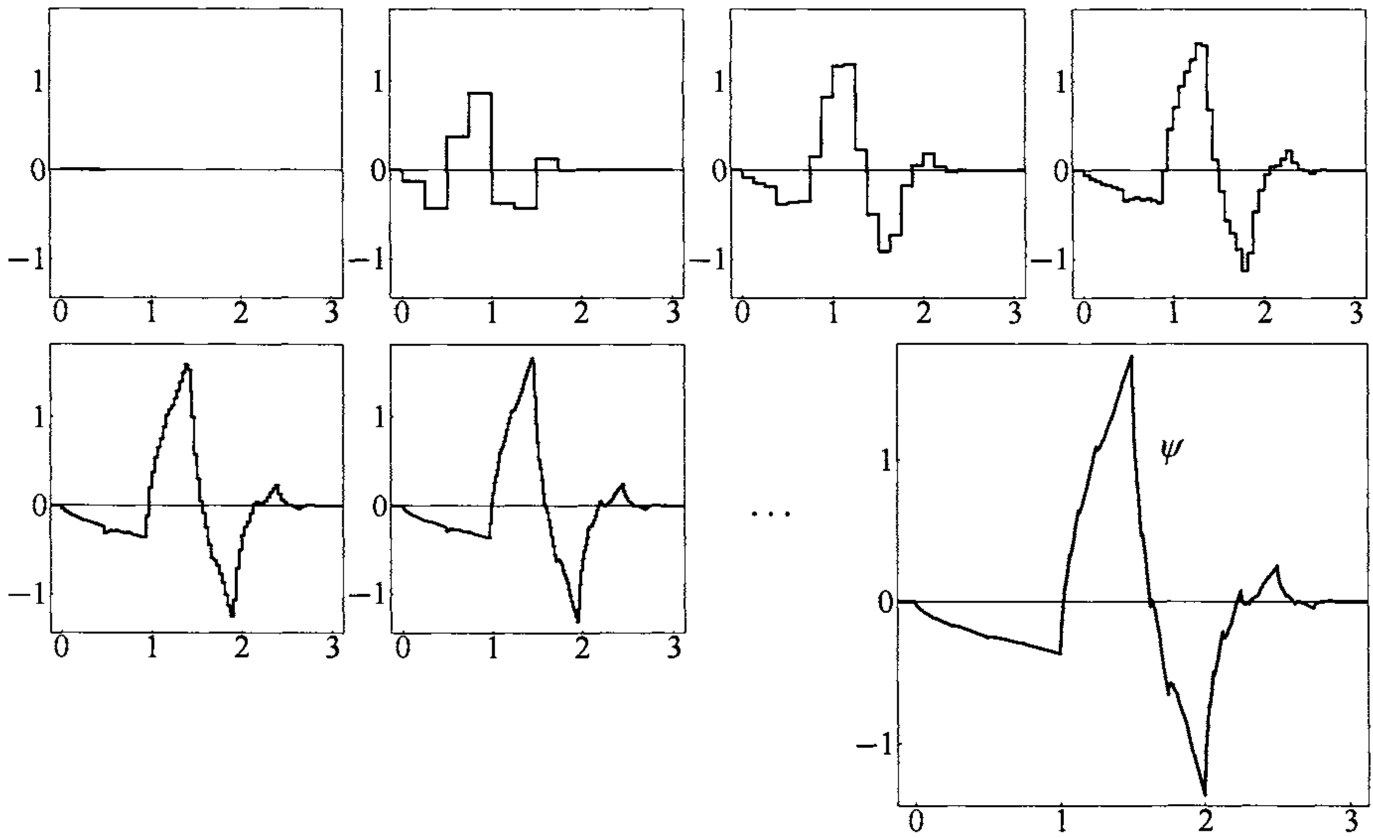
(b): Mother function
