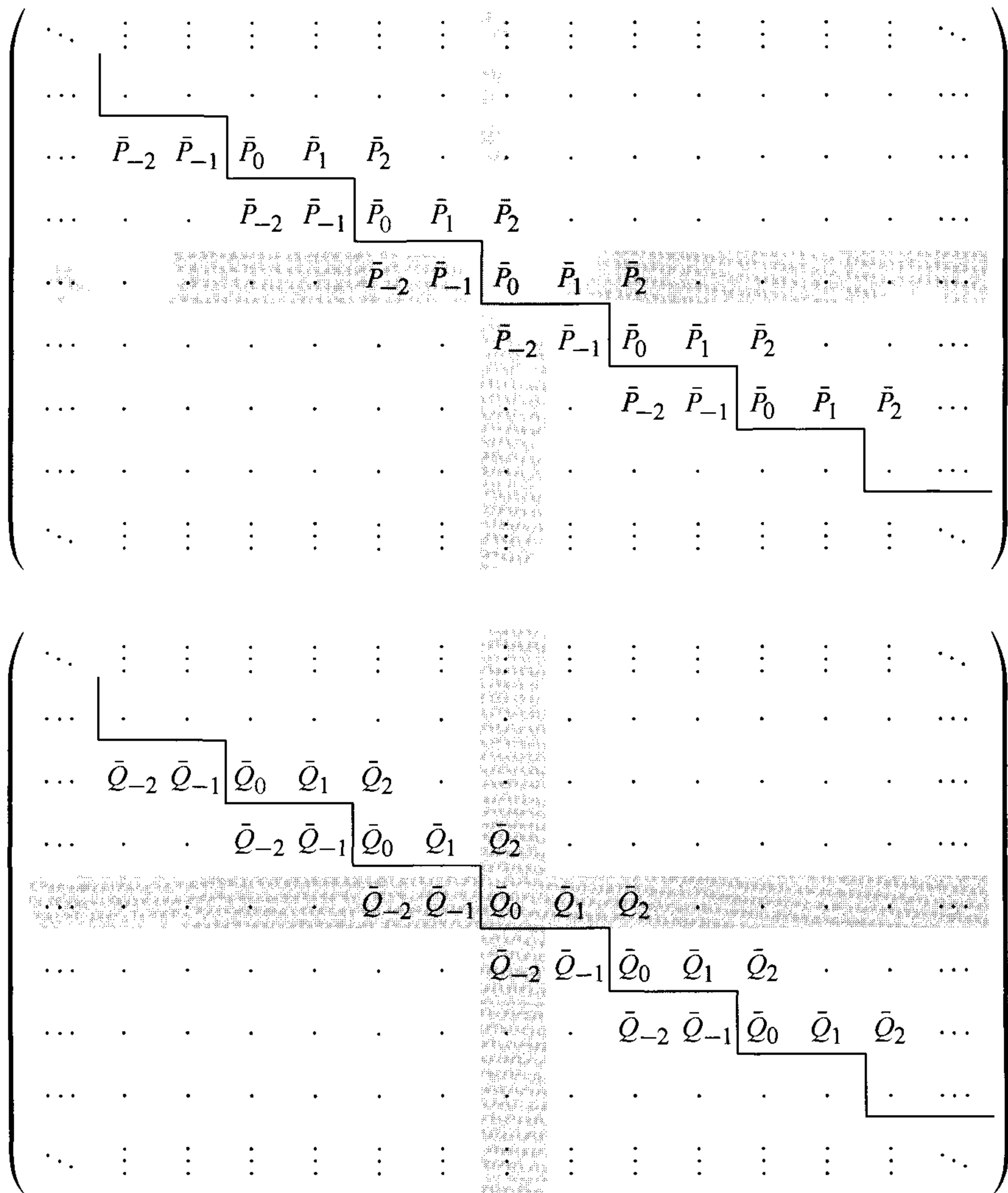
Fig. 1.3. The slanted matrices F and G of (1.7.2).
