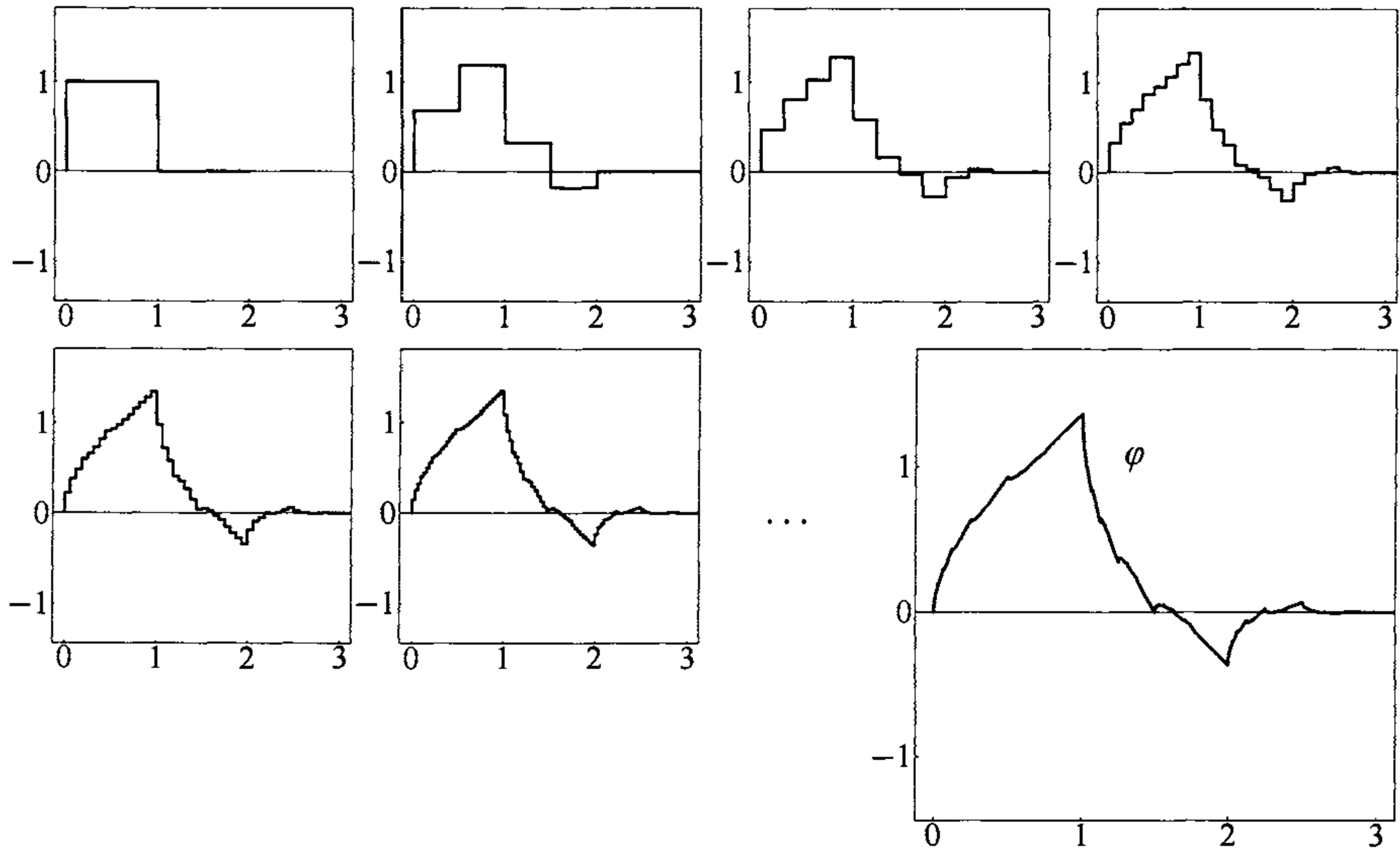
(a): Father function
