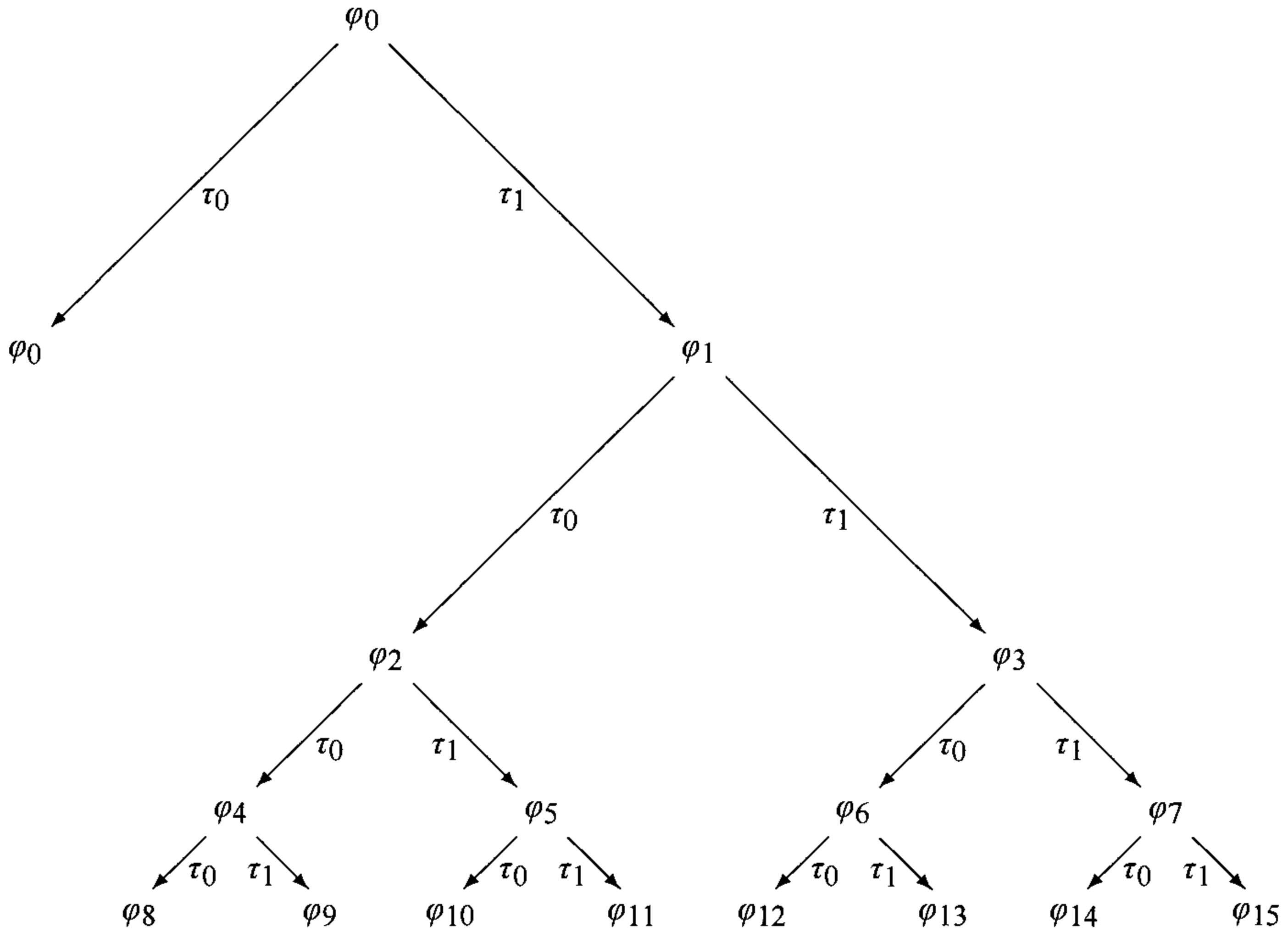
Fig. 8.1. The fundamental dyadic pyramid.
