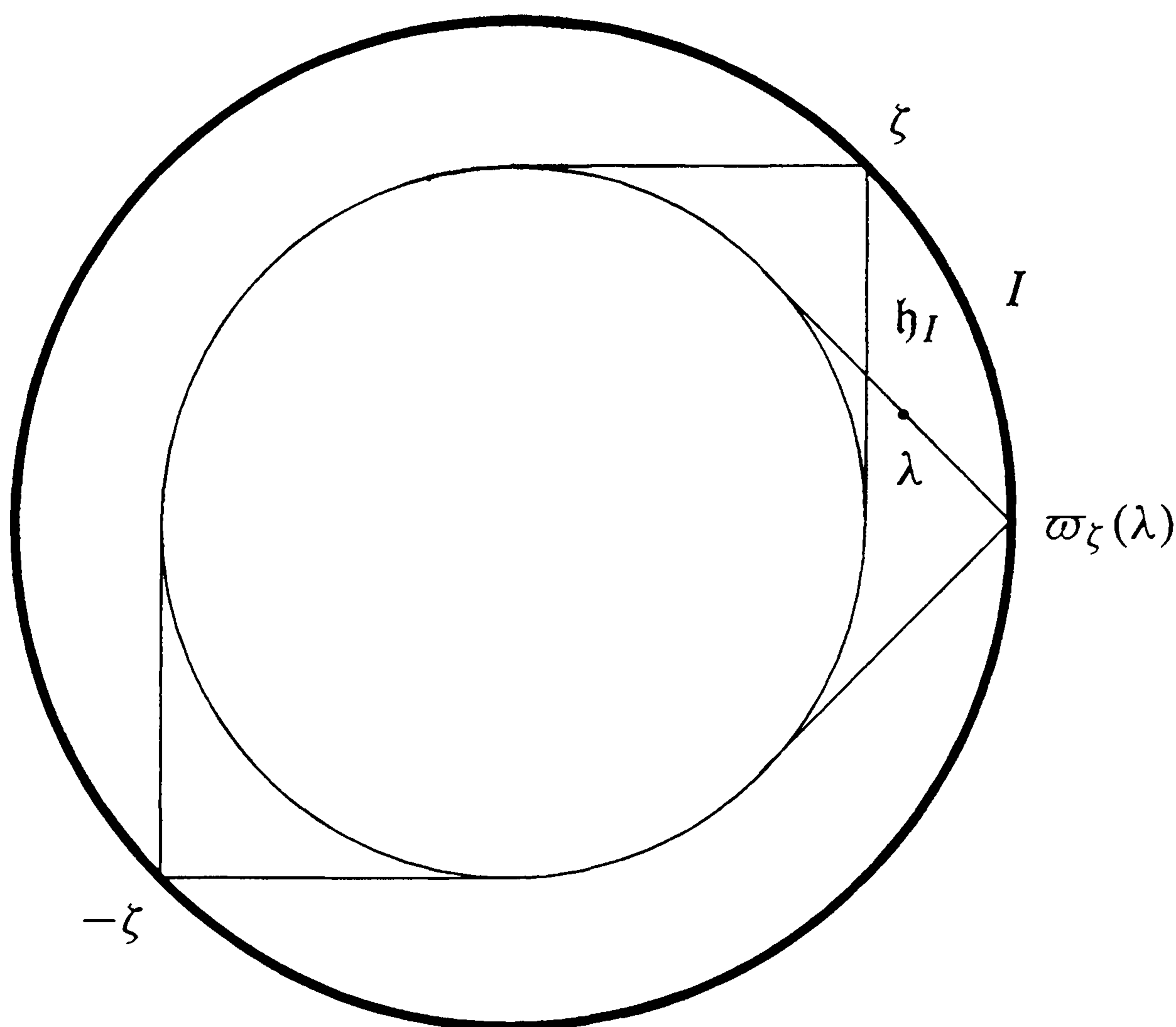
Figure 4.2. The oblique projection \varpi_\zeta(\lambda)
