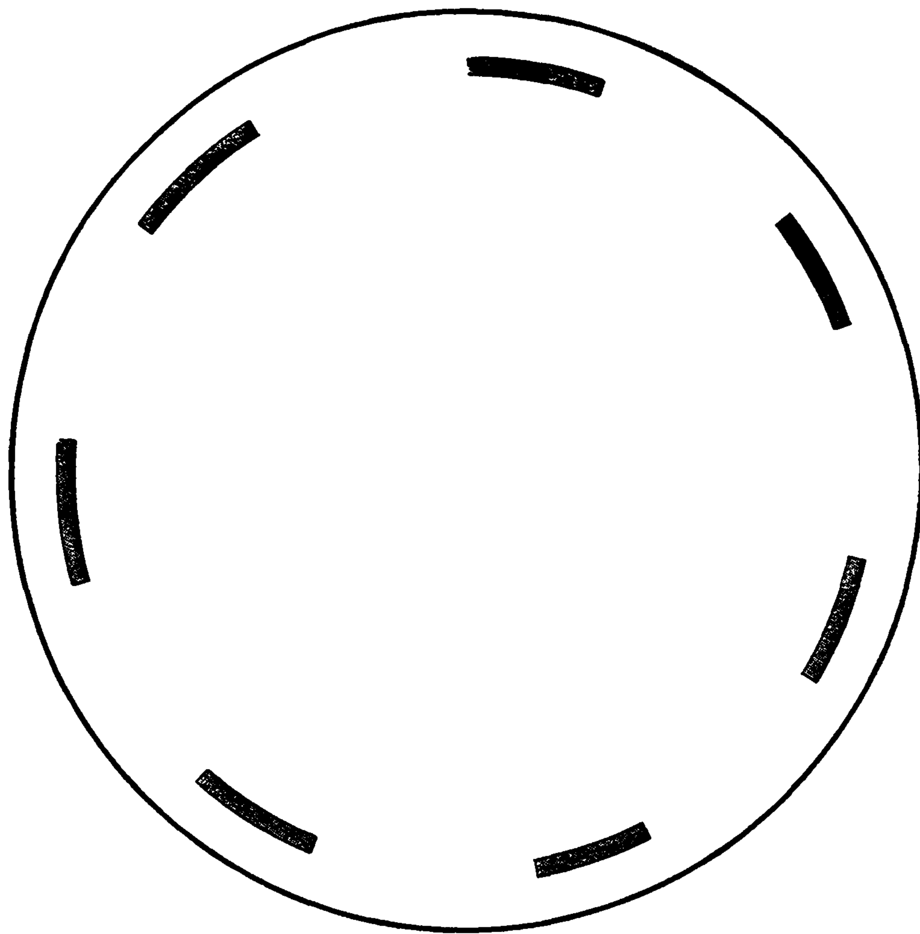
Figure 8.1. The set E^\sharp(N, \alpha)
