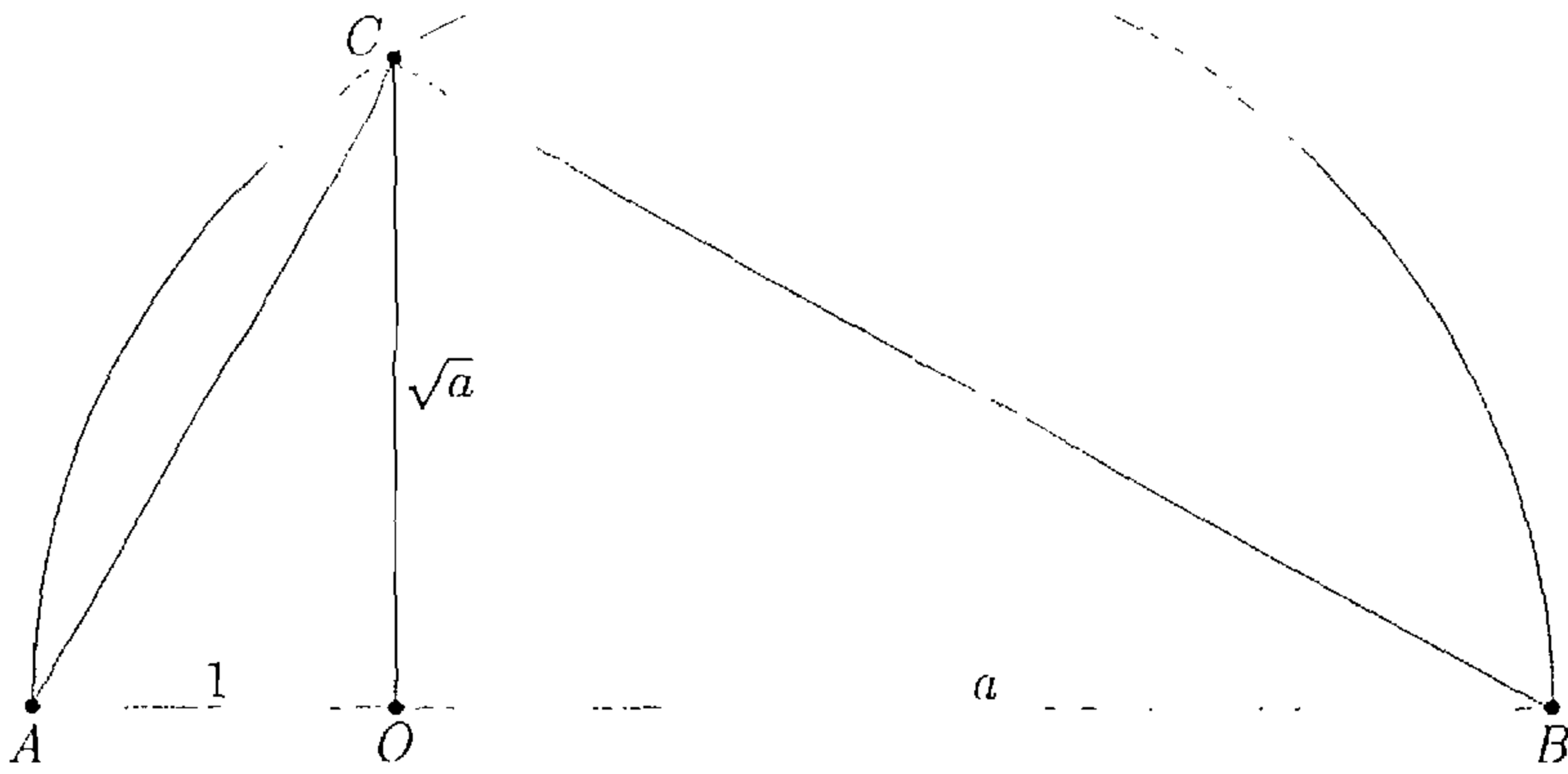
FIGURE 15.5. Construction of \sqrt{a} .
