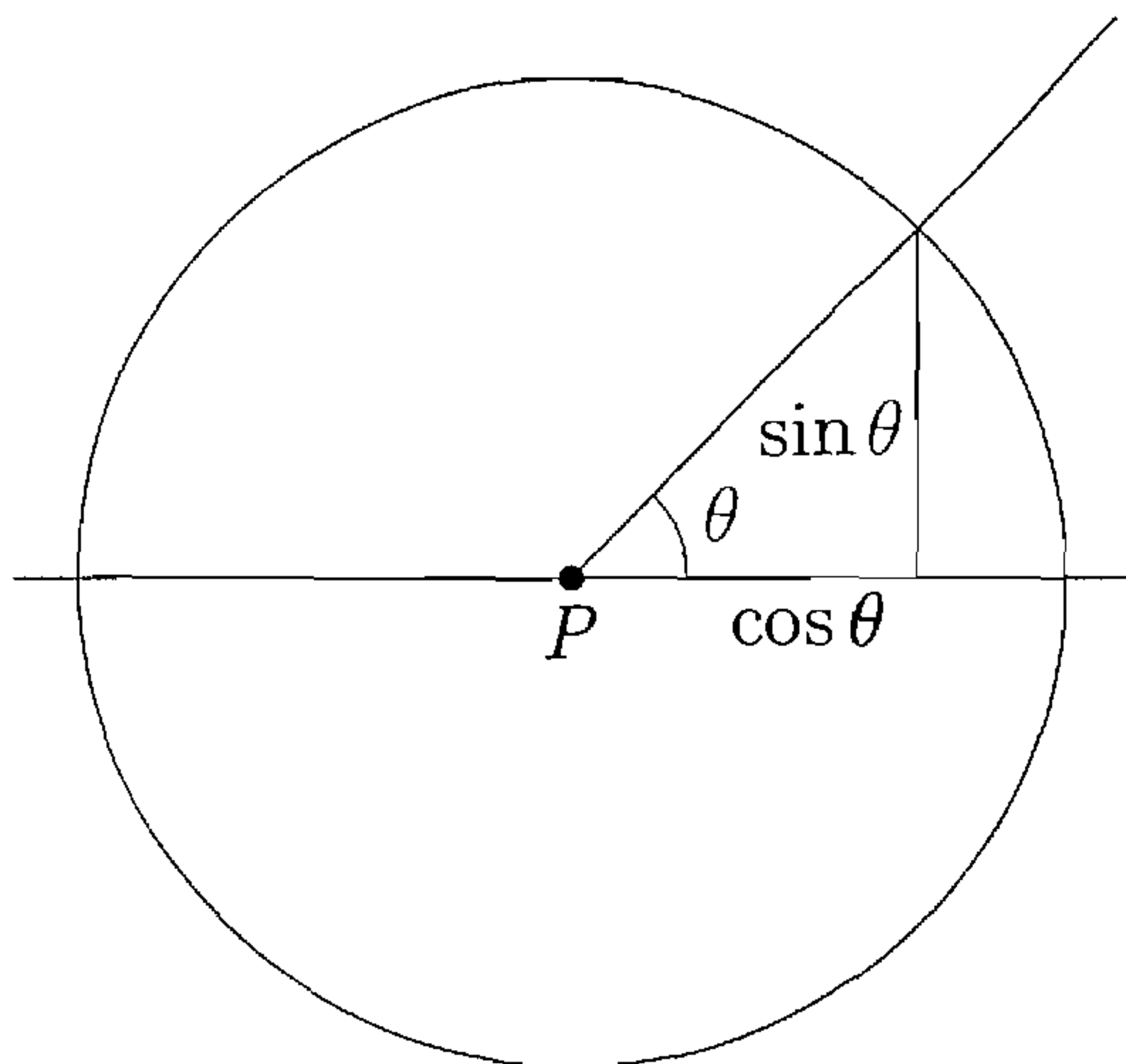
FIGURE 15.6. Construction of sines and cosines.
