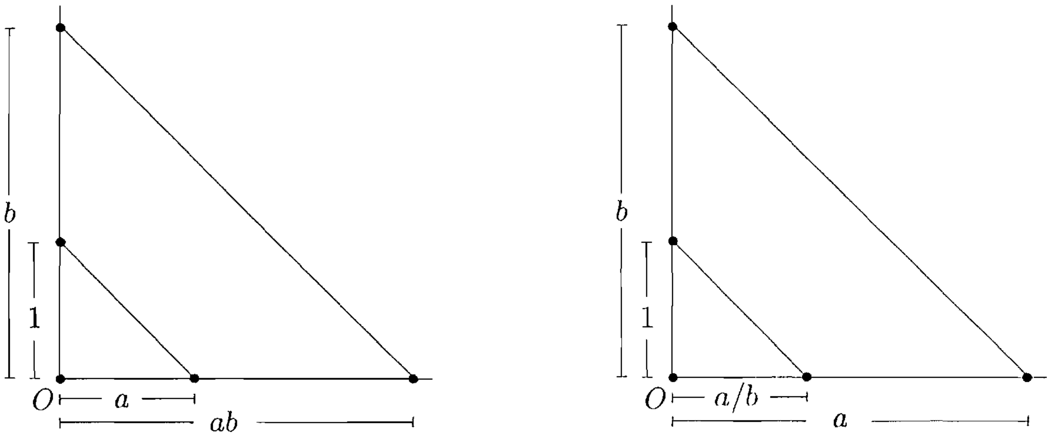
FIGURE 15.4. Construction of ab and a/b .
