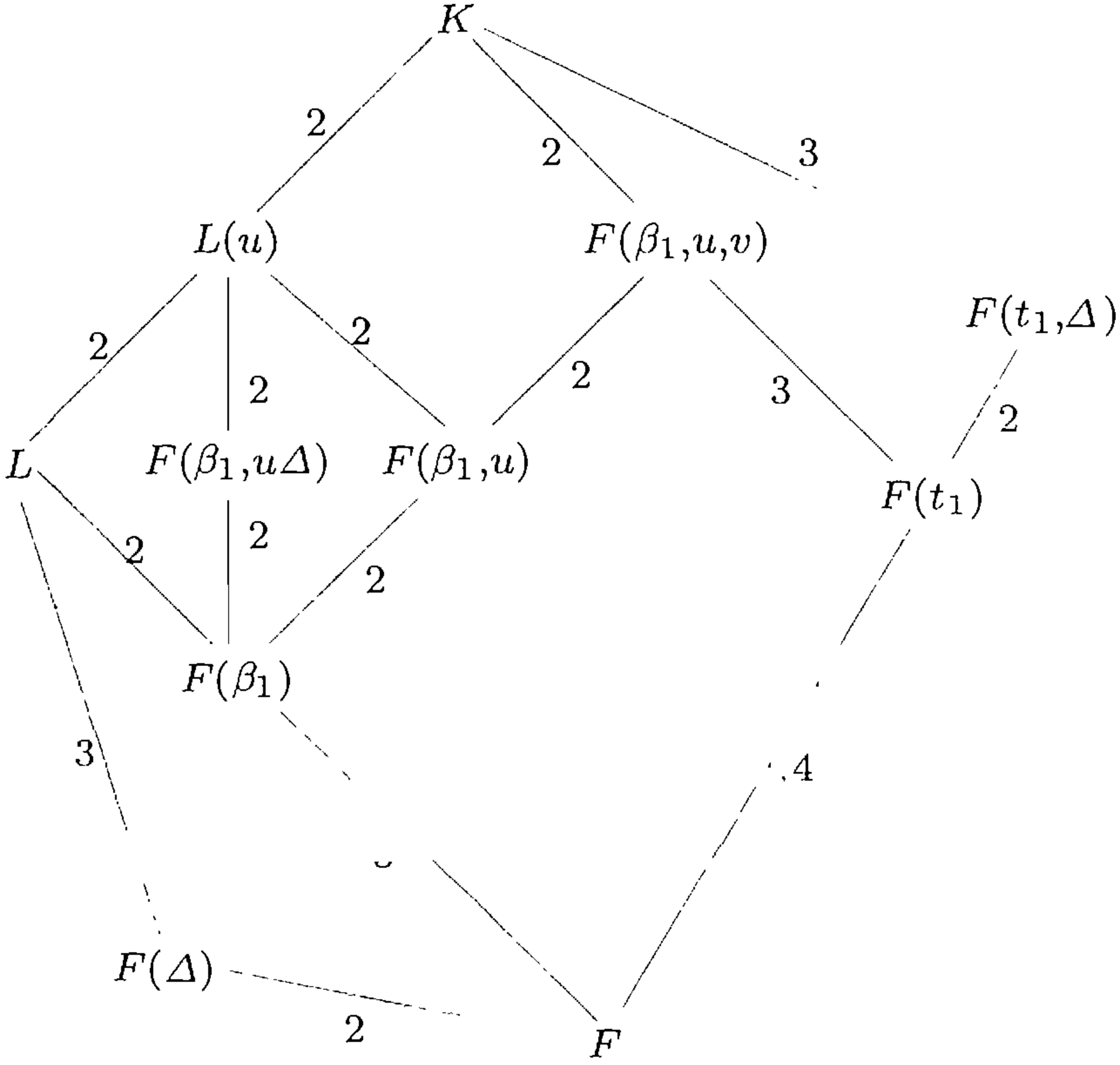
FIGURE 13.1. Field tower for F(t_1, t_2, t_3, t_4)/F .
