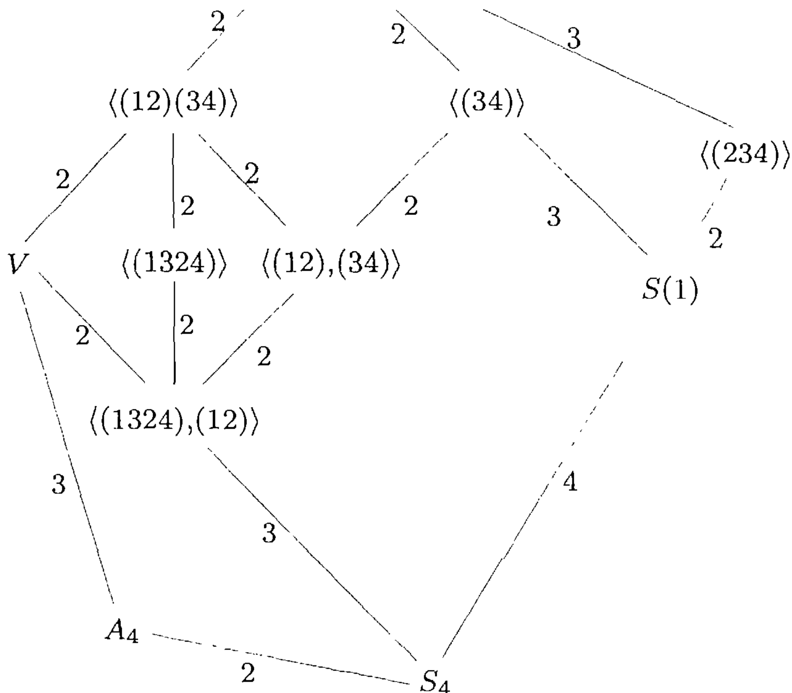
FIGURE 13.2. Group tower for S_4 .
